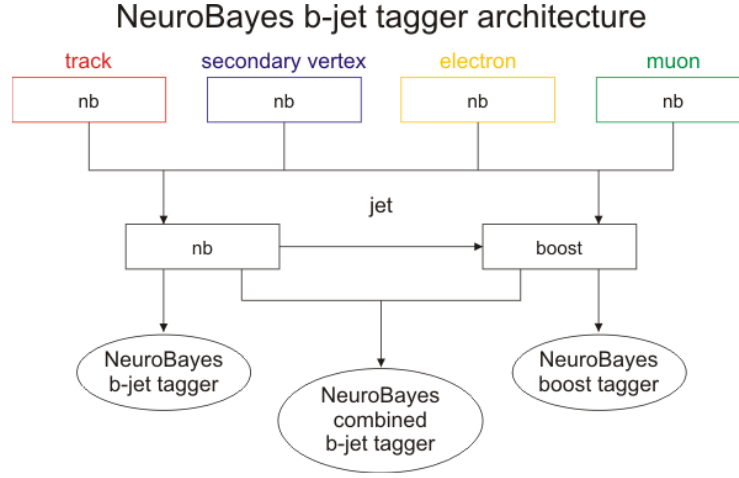
Figure 5.11: Architecture of the NeuroBayes b-jet tagger. Each box stands for a single NeuroBayes calibration. The arrows point up where the result of the expert is used. The colors clarify the different objects.
