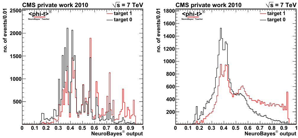
Figure 5.12: Left: the output distribution of the zero iteration mode. The training results in a Gini index of 19.9 calculated in 35.43s. A classification with the same setup parameters plus an additional internal boost results in an output distribution as shown on the right. The Gini index is also 19.9, but the shape is much smoother with a much longer runtime of 290.47s. The explanation of this effect is a different for the monotonous spline fit: NeuroBayes setup parameter DIAG instead of DIA2 5.1.3.
