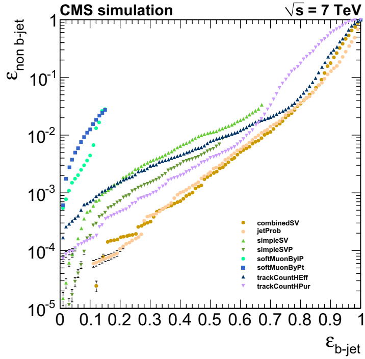
Figure 4.9: Performance of the CMS b-jet taggers. To compare the different taggers, they are plotted in the mistag rate/efficiency phase space. The lower right corner represents a tagger, where all non-b-jet could be suppressed without losing any b-jet. The colors are chosen to distinguish the different kind of taggers. Blue: the muon tagger (SMT), green: the simple secondary vertex tagger (SSV), violet: are track counting tagger (TC), orange: are the two more complex: jet b probability and combined secondary vertex.
