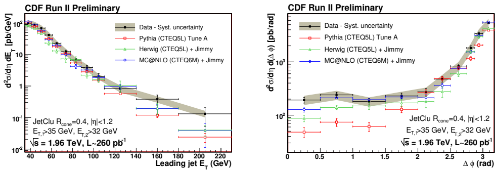
Figure 2.12: The differential b\bar{b} cross section as a function of the leading jet E_T is plotted on the left. On the right the angle between the two b quarks is shown. This distribution is sensitive to the fractions of the three production mechanisms FCR, FEX and GSP.
