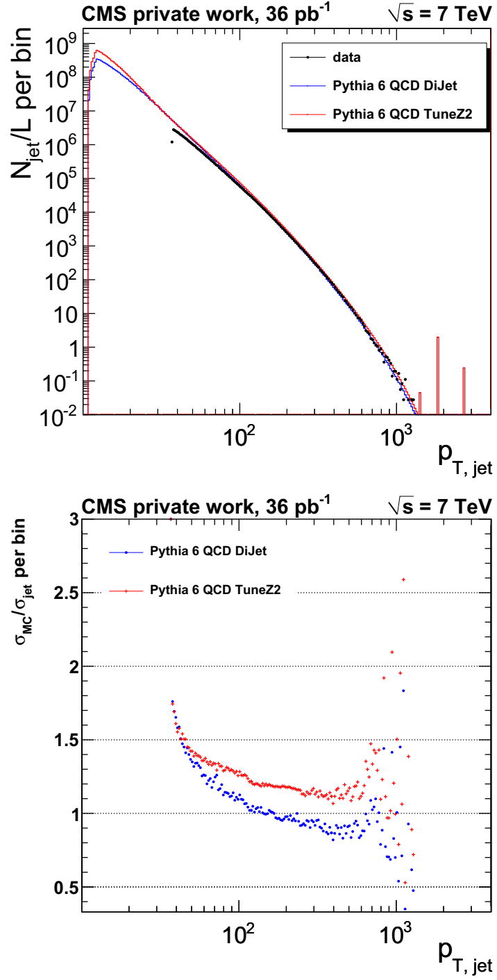
Figure 4.16: Top: the jet spectrum normalized by the integrated luminosity \int \mathcal{L} is shown. It is compared with the two Monte Carlo expectations of the samples used in this thesis. Bottom: relative p_{T, \text{jet}} spectrum. The MC spectra from the top plots are plotted relative to the data distribution.
