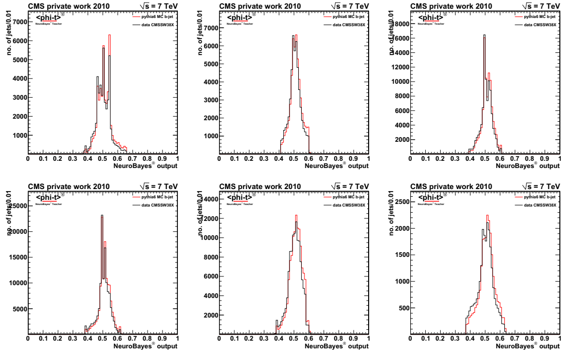
Figure B.5: Result of the comparison of data and MC for jet objects
