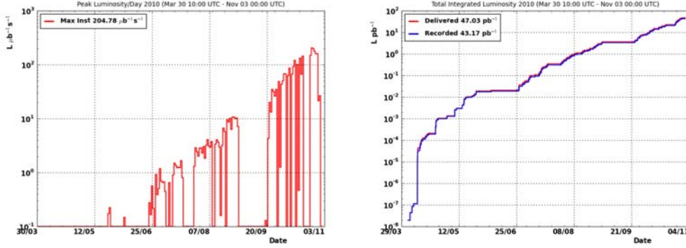
Figure 4.1: Peak luminosity per day for the first year of data taking with the CMS experiment. The period from the first collisions until June is called the commissioning era, the period after Run2010 era. On the right the integrated luminosity is shown. 2
