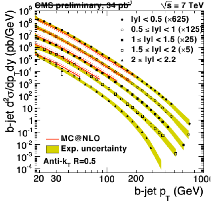
Figure 6.17: The complete analysis of the b-jet cross section measurement was updated. Most subparts are updated. The update of the purity measurement presented here is included. Having all analysis together a similar plot will go for publication.
