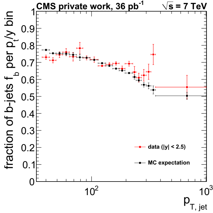
Figure 6.10: Result for the p_T spectrum determined by the flavor content fitter for |y| < 2.5 . The parametrization is chosen to measure directly the b-jet fraction for tagged jets ( p = 1 ). Only statistical errors are shown in this figure.
