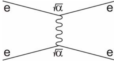
Figure 2.2: Feynman diagram of the electron scattering. A virtual photon is exchanged for the interaction.
