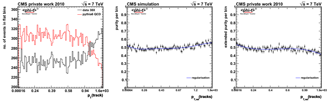
Figure 5.28: The left plot shows the differences between data and MC. In data more tracks with large p_{T,rel} were found than simulated in MC. This effects also the classification of b-jets. The plot in the middle shows the purity of tracks coming from b-jets as calculated by MC, on the right the extended purity of the NBD training is shown.
