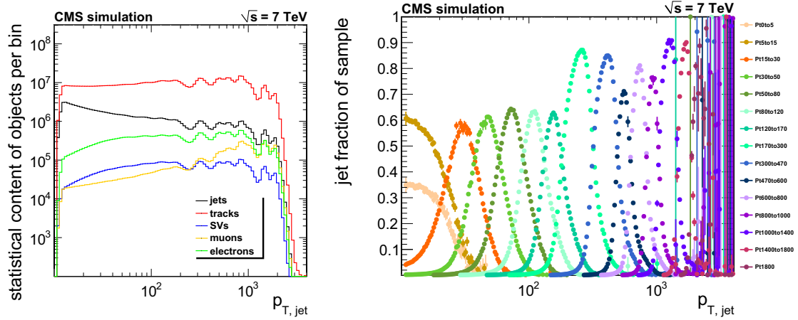
Figure 4.13: Left: Amount of statistics for the different objects, which are used in the analyses. MC samples for different \hat{p}_T bins are available. The different samples must be weighed to get the true p_T spectrum. Right: Composition of the TuneZ2 MC sample created from different samples with different \hat{p}_T bin ranges.
