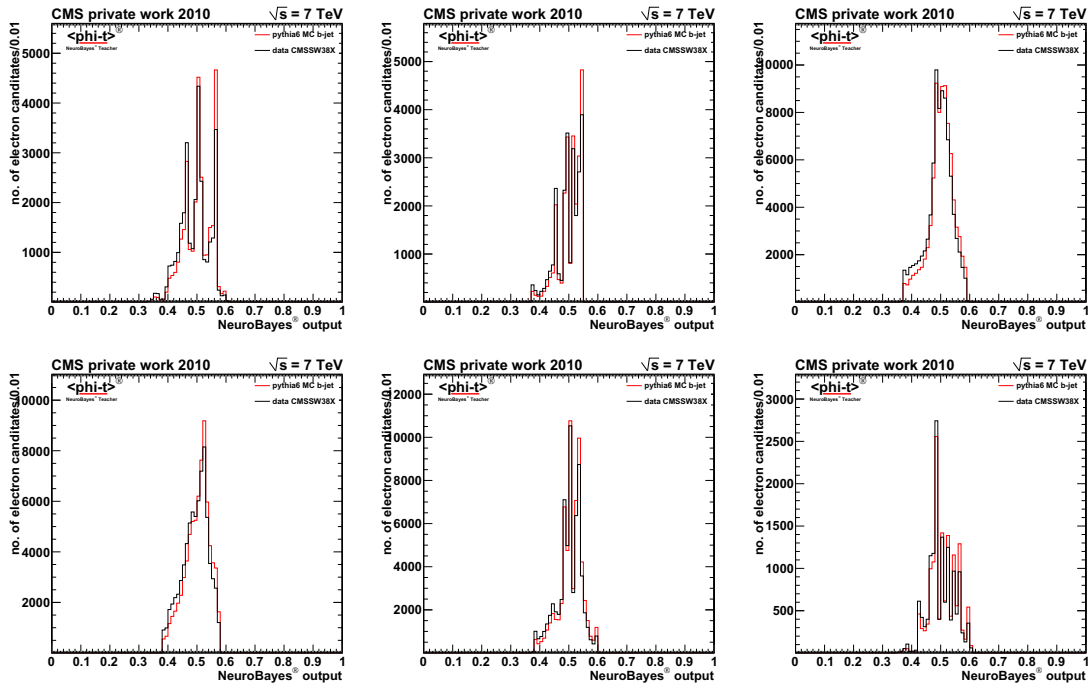
Figure B.3: Result of the comparison of data and MC for electron candidate objects
