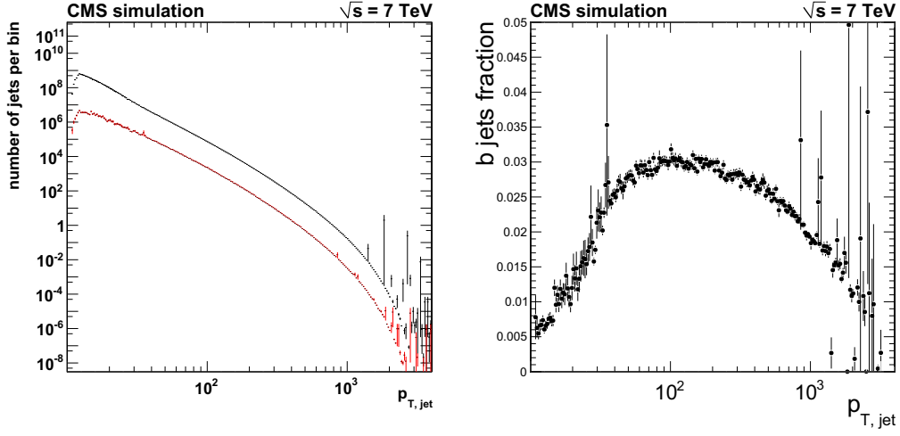
Figure 4.12: p_T spectrum of the all jets in black and b-jets in red (left) and the fraction of b-jets dependent on the jet p_T (right) for the Monte Carlo samples reconstructed in CMSSW version 3.8
