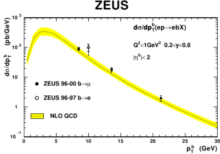
Figure 2.10: Photoproduction of beauty quarks in events with two jets and a muon. The filled points show the ZEUS results from this analysis and the open point is the previous ZEUS measurement in the electron channel [B + 01]. The full error bars are the quadratic sum of the statistical (inner part) and systematic uncertainties. The dashed line shows the NLO QCD prediction with the theoretical uncertainty shown as the shaded band.
