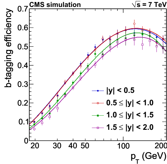
Figure 6.1: b-tagging efficiency in different rapidity bins.
