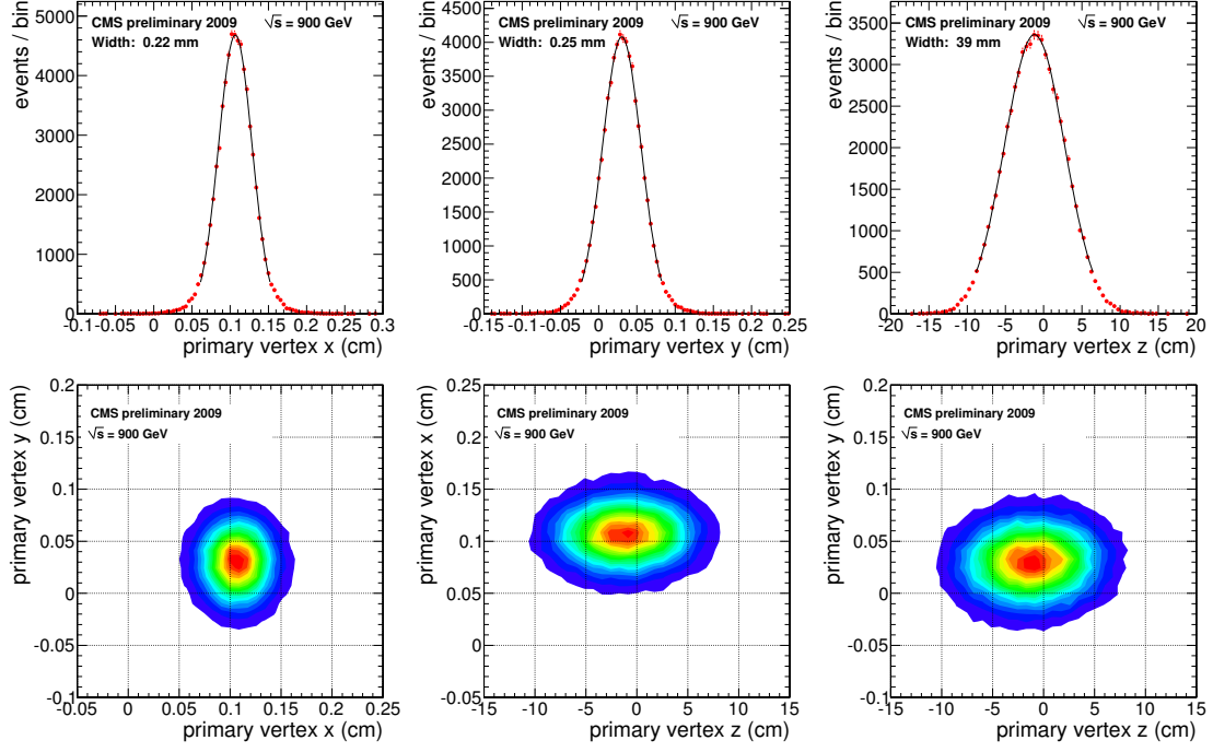
Figure 4.2: Plots of the primary vertex distributions from a single run. 3
