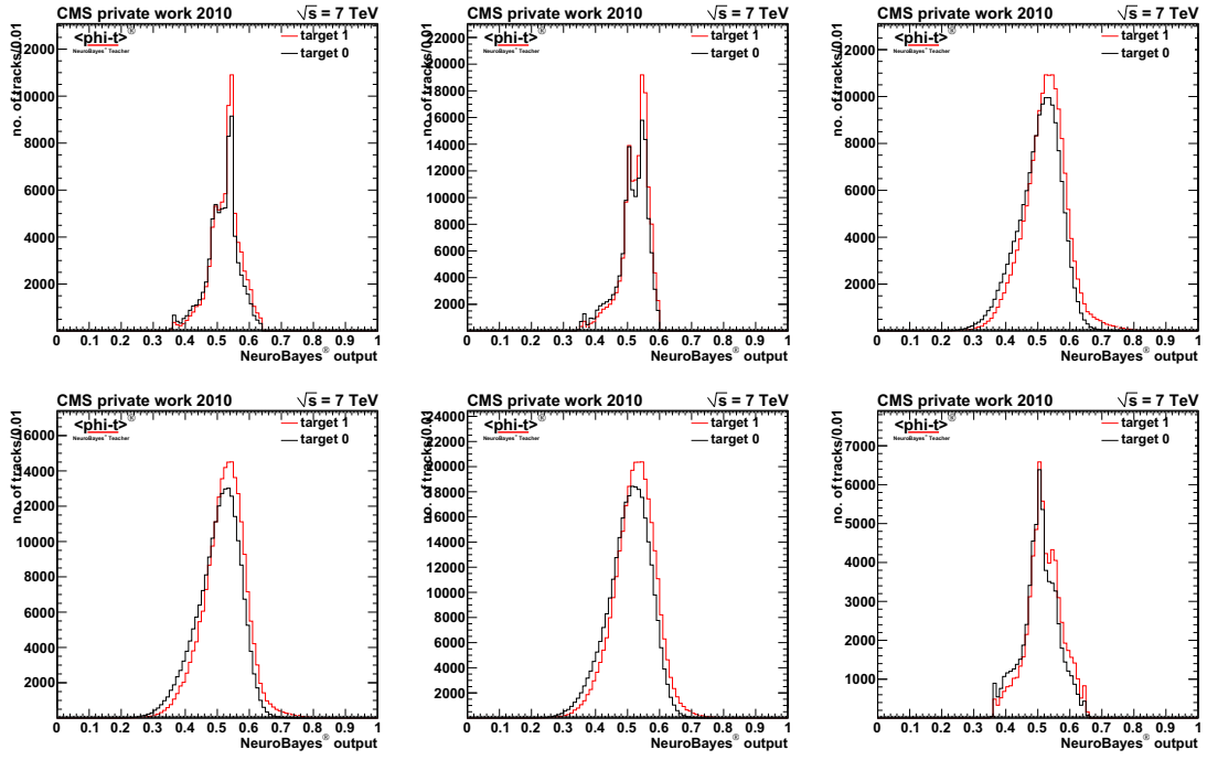
Figure B.1: Result of the comparison of data and MC for track objects
