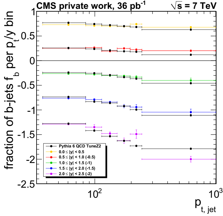
Figure 6.12: The plot show the measured dependencies of the b-jets in p_T and |y| determined by the flavor content fitter. There is a agreement between data and simulations.
