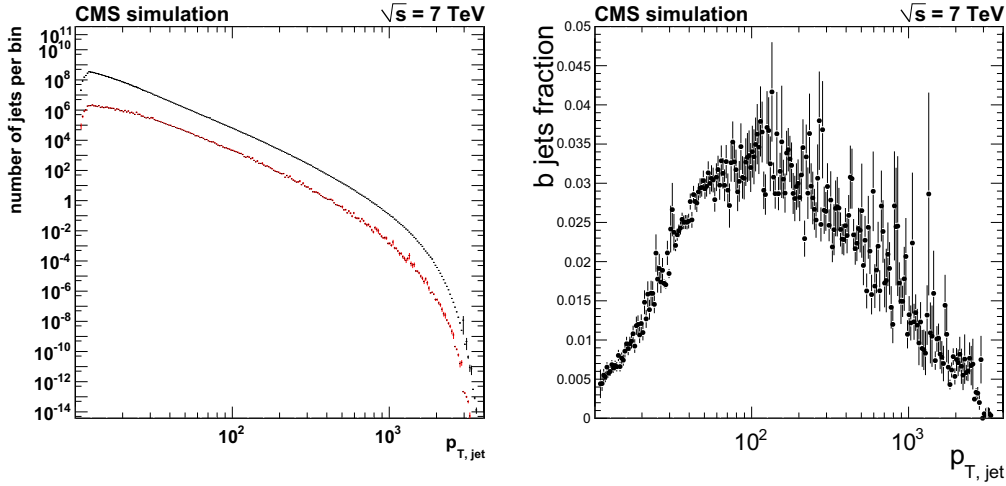
Figure 4.10: p_T spectrum of the all jets in black and b-jets in red (left) and the fraction of b-jets dependent on the jet p_T (right) for the Monte Carlo samples reconstructed in CMSSW version 3.6
