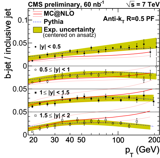
Figure 6.8: Measured b-jet cross section as a ratio to inclusive jet cross section. The NLO theory and Pythia MC predictions are shown for comparison.
