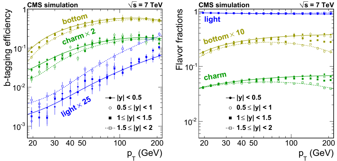
Figure 6.3: The b-tagging efficiency and light, charm mistag rates from MC truth (left). Bottom, charm and light fractions of inclusive jets from MC truth (right).
