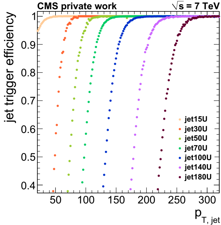
Figure 4.14: Efficiency of the different triggers. As turn on point the position where the trigger becomes 99% efficient is extracted.
