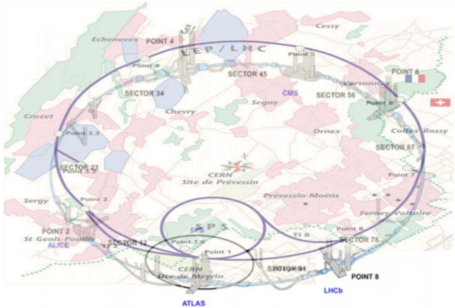
Figure 3.1: Map of the LHC and its hinterland. The red regions correspond to the villages next to CERN. The for experiments are drawn on their location in the accelerator ring.
