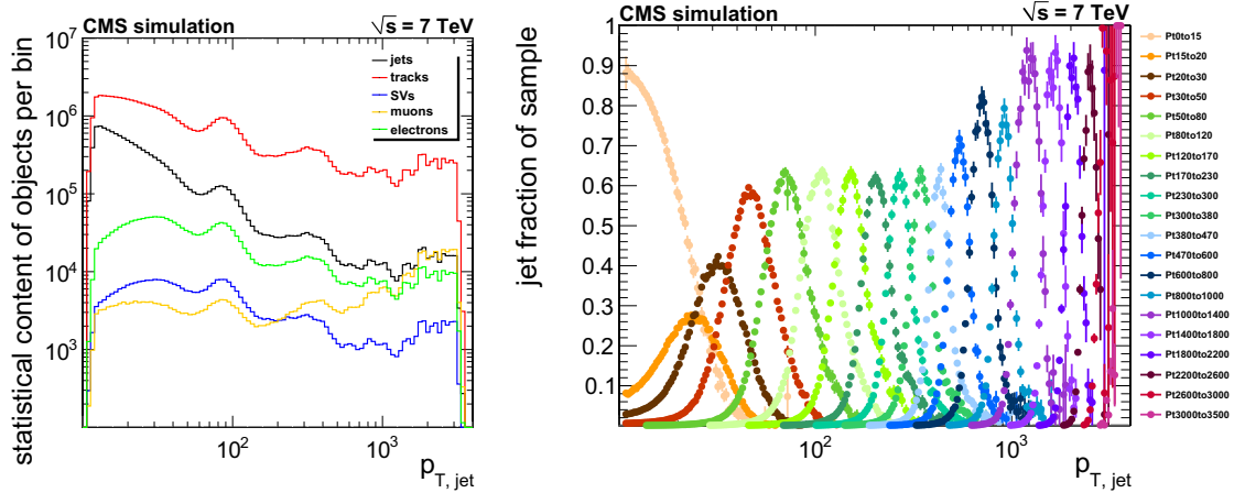
Figure 4.11: Left: Amount of statistics for the different objects, which are used in the analyses. MC samples for different \hat{p}_T bins are available. The different samples must be weighed to get the true p_T spectrum. Right: Composition of the weighed MC created from different samples with different \hat{p}_T bin ranges.
