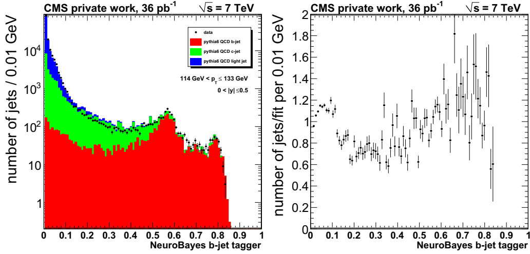
Figure 6.18: Exemplary result of the flavor content fitter. Target distribution is the NeuroBayes b-jet tagger output. On the left the result of the fit to data distribution of the three different classes is shown. The right plot shows the ratio between fitted templates and data distribution.
