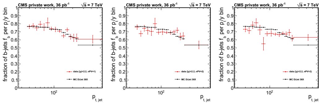
Figure 6.11: Study of the dependency on pile up effects. The histograms show the b-jet fraction of a tagged sample for different numbers of primary vertices. The statistics is too low to claim a final conclusion.
