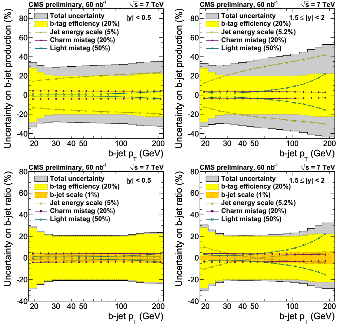
Figure 6.6: Leading sources of systematics uncertainty for the b-jet cross section measurement at |y| < 0.5 (top left) and at 1.5 \leq |y| < 2.0 (top right), and for the ratio of b-jet and inclusive jet cross section measurements at |y| < 0.5 (bottom left), and 1.5 \leq |y| < 2.0 (bottom right). The 11% luminosity uncertainty is not shown.
