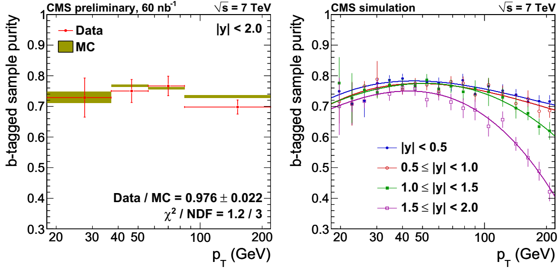
Figure 6.4: The b-tagged sample purity obtained using fits to secondary vertex mass (left). The b-tagged sample purity estimated using b-tagging efficiency and mistag rates from MC (right).
