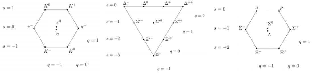
Figure 2.1: The eightfold way is an ordering of the ground state particles as proposed in 1961. The particles are ordered dependent on their quantum numbers S and q . This composition leads to the prediction of the later discovered particle \Omega^{--} and is the base for the later formulated quark model.
