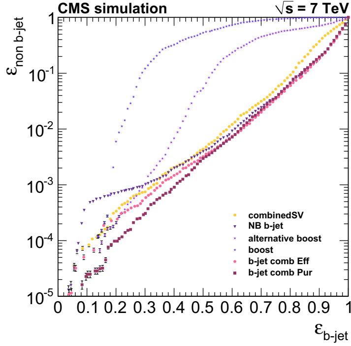
Figure 5.24: Performance of the NeuroBayes b-jet taggers. All new taggers are plotted together with the best existing tagger from CMS.
