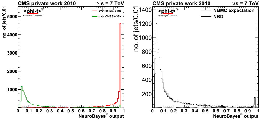
Figure 5.33: Left: the output distribution of the NBD training. This expertise applied on an independent sample results in the distribution plotted on the right. It is similar to the one expected from MC.
