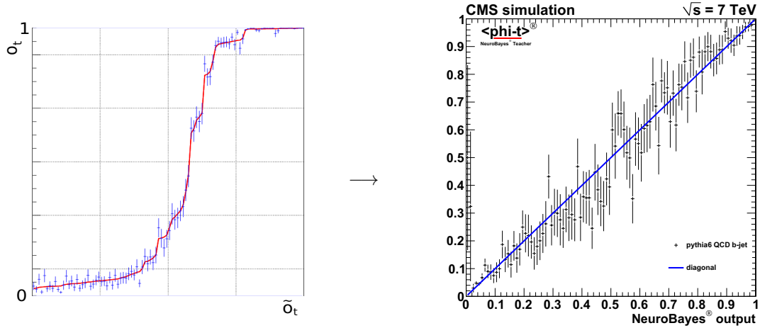
Figure 5.7: Diagonalization of the Zero iteration training. This is needed to get an probability interpretation of the NeuroBayes output. On the left the transformation functions is determined doing a fit of a monotonously rising spline function. On the right the resulting distribution of the target 1 purity P(T1|o_t) to the final output value o_t is plotted. The expected behaviour, shown by the diagonal line is fulfilled.
