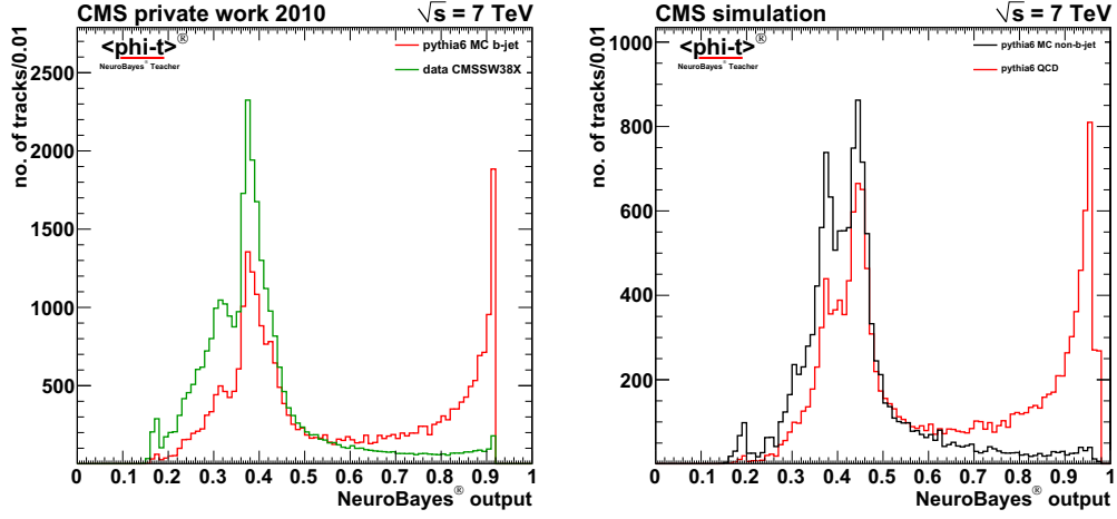
Figure 5.26: The output distributions of the data based training on track level on the left and for a classical MC based training on the right.
