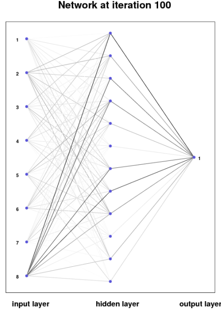
Figure 5.8: Example of an architecture of an artificial neural network calibrated in NeuroBayes. The thickness of the lines corresponds to the absolute values of the weight w^{a \rightarrow b}
