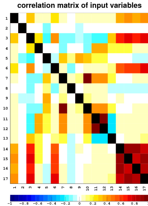
Figure 5.6: Matrix of correlation coefficients \varrho_{ij} . The first column is the target distribution, where target 1 is set to 1 and target 0 is set to 0. In this example there are many highly correlated variables \varrho_{ij} \rightarrow 1 , which are painted in deep red and deep blue colors.
