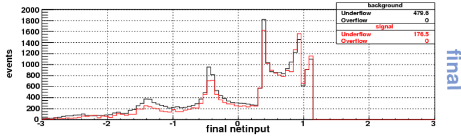
Figure 5.5: Standardization of the estimated signal probability of the variable from figure 5.4. The mean of this distribution is zero with a width of one. This is the final distribution of the transformed input variable after the preprocessing.
