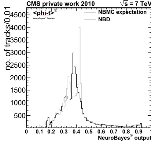
Figure 5.27: The output distribution of the data based training is plotted. Further a comparison of the distribution with the expectations from the NBMC training is shown. The NBMC output distribution (gray) was transformed by the function introduced in the text.
