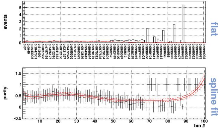
Figure 5.10: Effect of large weights. The bins on the right contain only one event with a large weight. The purity is effected by the target type of this single event. A more reasonable estimate of the purity should be around 0.5 with adequate uncertainty.
