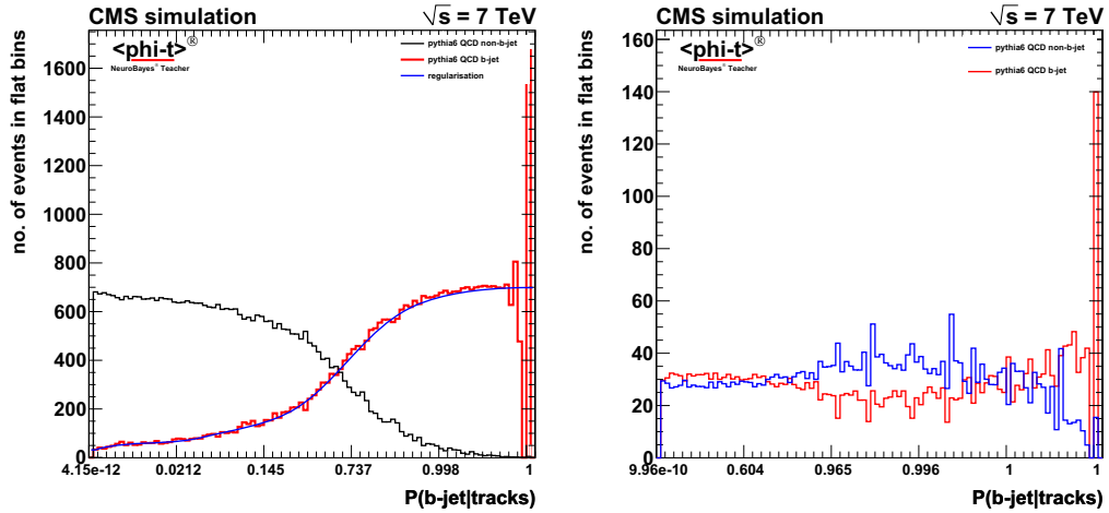
Figure 5.20: The plots show the distribution of the track probability, which is used as input variable, for the unboosted (left) and the boosted NeuroBayes training. The increase of statistics and the reweighing cause a gain of information for an improvement of the b-jet tagger.
