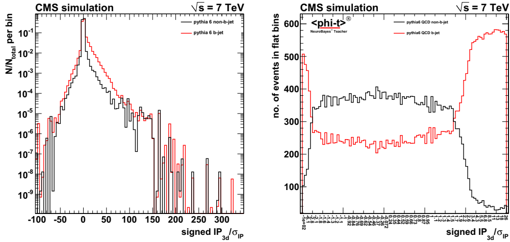
Figure 5.14: Track object training: The most important input variable is the significance of the signed impact parameter. The distribution of this variable is shown in the classical histogram with equidistant bins on logarithmic scale (left) and in probability integral transform (right). The b-jet tracks are plotted in red. The differences to the non-b-jet tracks (black) are clearly visible.
