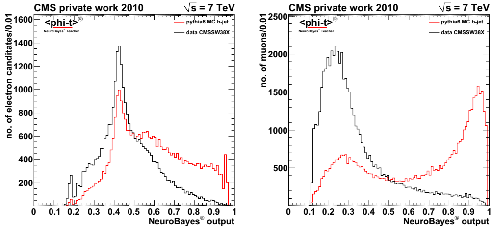
Figure 5.18: NeuroBayes output of the lepton classification. Left: electron candidates. Right: muons. The b-jet objects are plotted in red.
