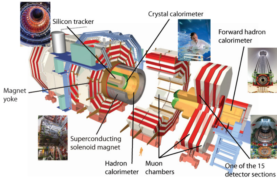
Figure 3.2: model of the CMS detector decorated with pictures of the different detector components 2 .
