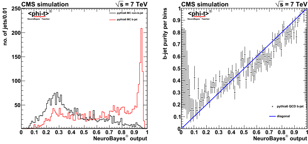
Figure 5.9: On the left the output distribution of an exemplary NeuroBayes calibration is shown. In black is the background and in red the signal distribution. On the right the purity of the signal distribution for each bin is plotted.
