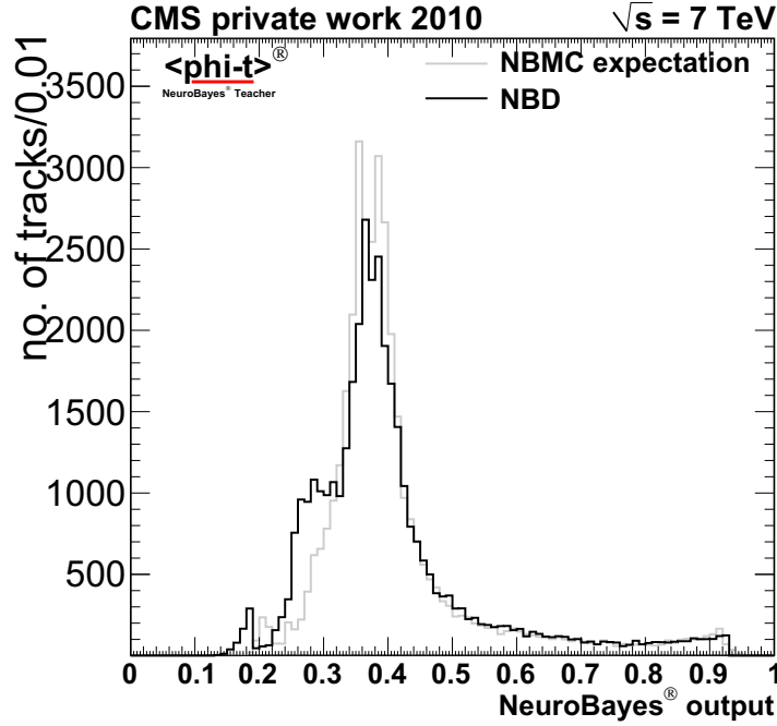
Figure 5.29: The output distribution of the data based training is plotted. For the calibration a correction of the MC distributions was applied. Further a comparison of the distribution with the expectations from the NBMC training is shown. The NBMC output distribution (gray) was transformed by the function introduced in the text.
