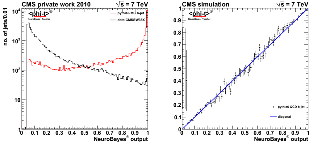
Figure 5.19: NeuroBayes output of the jet classification (left). red: the b-jets, black: other jets. There are no jets in the first 5% of the output distribution. No cut was applied here. B-jets without lepton and small lifetime look like a light jet. In the right plot the purity of the b-jet distribution is shown. If the purity of each bin matches with the value of the NeuroBayes output variable the probability interpretation is fulfilled. This property is required for the boost training.
