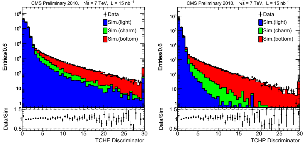
Figure 4.5: Discriminator of the track counting b-jet tagger 9
