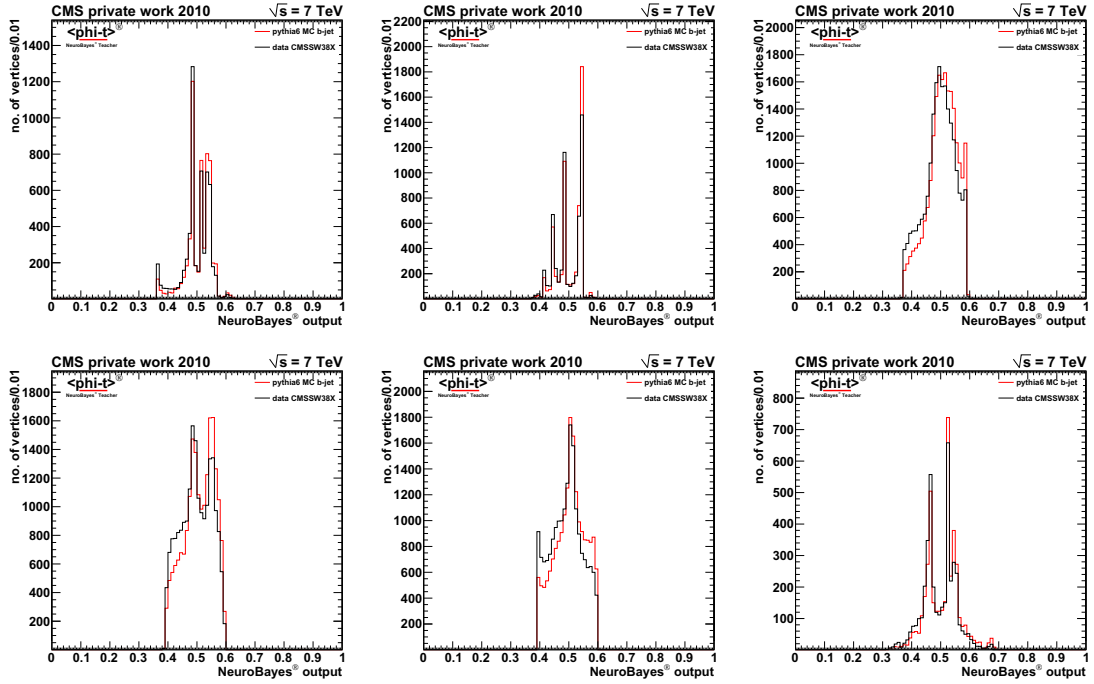
Figure B.2: Result of the comparison of data and MC for vertex objects
