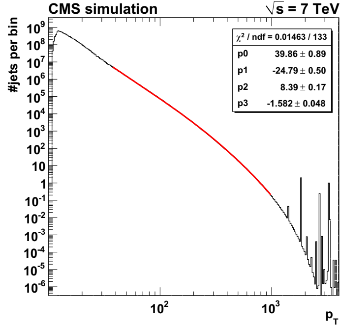
Figure 5.13: To transform the p_{T,jet} spectrum into a flat distribution, it was fitted by a polynomial function at double logarithmic scale. The shown spectrum is calculated out of the available MC events. Therefore different samples must be weighted by a specific value (see 4.4). This causes the binning effects on the right.
