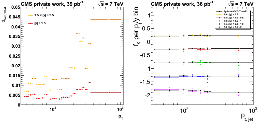
Figure 6.14: The plot on the left shows the variance of the flavor content fit, if the templates were varied within their statistical uncertainties. These contribute to the systematics. On the right the fraction of c-jets f_c is computed and compared to the MC expectations. The good agreement allows a more strict estimate on the uncertainty caused by badly simulated c-jets.
