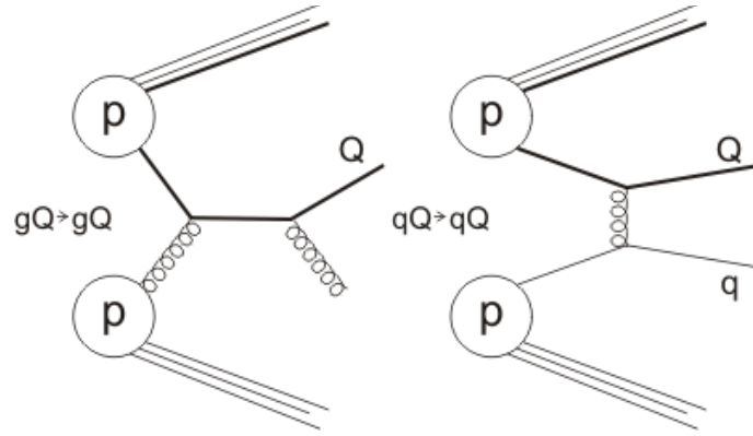
Figure 2.5: At next to leading order the production mechanism are classified in three kinds. Here an example for the flavor excitation (FEX) is illustrated. The processes are assigned to it, if the scattering is accomplished by a heavy quark out of the proton.
