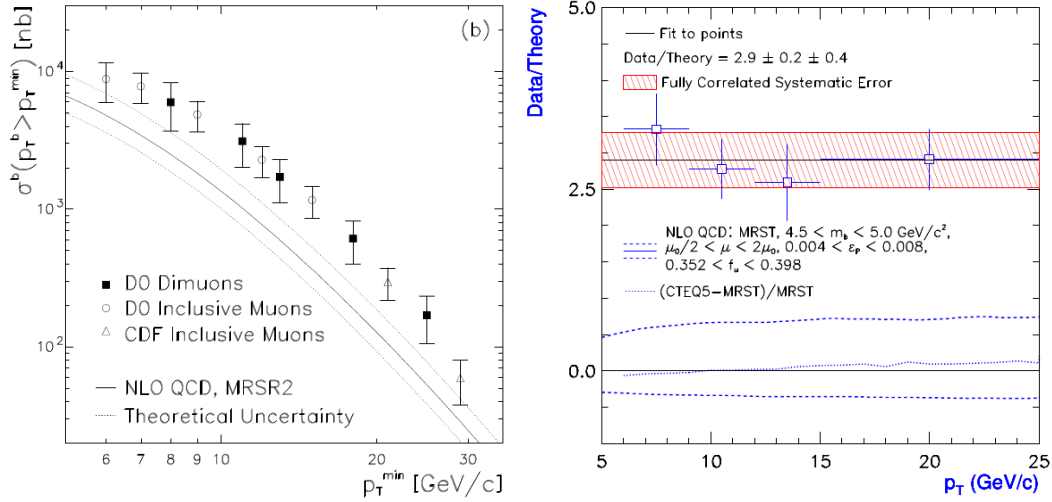
Figure 2.9: b quark production cross section for |y_b| < 1.0 compared with the inclusive single muon results and the NLO QCD prediction. On the right is the result of the B^+ meson differential cross section measurements from CDF normalized to the NLO predictions.
