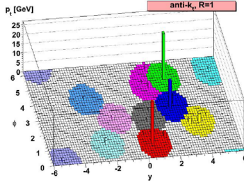
Figure 4.3: Exemplary clustering of the anti-kt jet algorithm. Larger transverse momenta are responsible for more conical clusters 5
