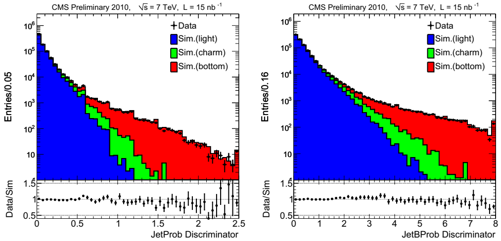
Figure 4.6: Discriminator of the jet probability b-jet tagger 10
