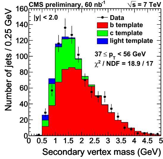
Figure 6.2: Example of secondary vertex mass fits.
