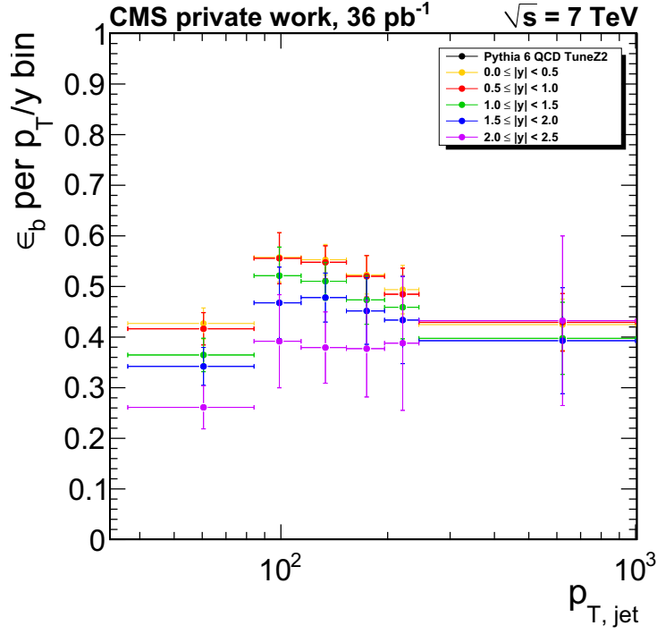
Figure 6.15: Efficiencies for b-jets passing the SSVHP > 2.0 cut by p_T and y . The values are extracted from a Pythia 6 QCD Monte Carlo generator.
