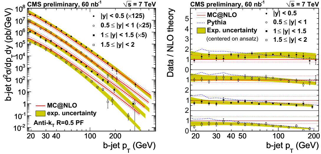
Figure 6.7: Measured b-jet cross section compared to the MC@NLO calculation, overlaid (left) and as a ratio (right). The Pythia prediction is also shown, for comparison.
