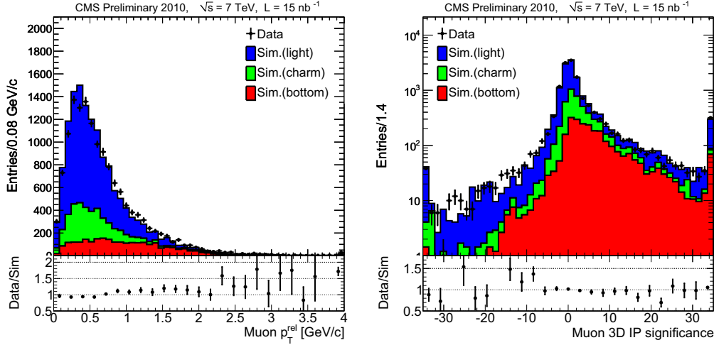
Figure 4.7: Input variables for the soft muon b-jet tagger 11
