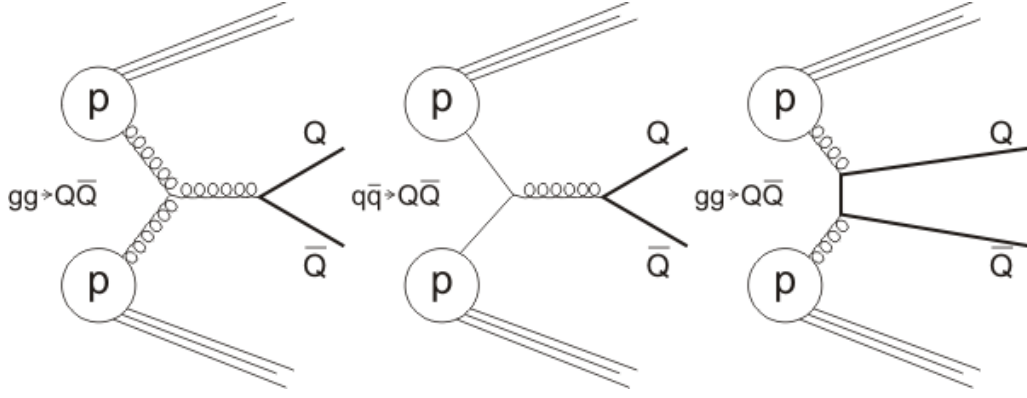
Figure 2.4: Heavy quark Q production mechanisms at leading order (LO). These processes are called flavor creation (FCR).
