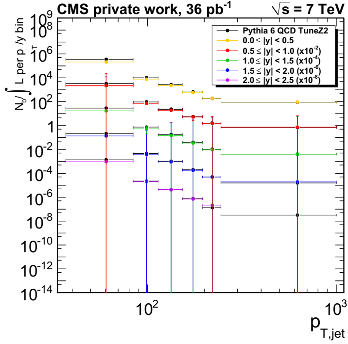
Figure 6.16: Normalized distribution for the number of b-jets extracted by the flavor content fit. The values are compared with a Pythia 6 QCD TuneZ2 expectations. There is good agreement.
