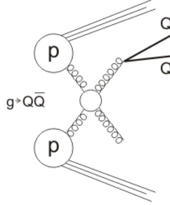
Figure 2.6: The gluons splitting category (GSP) refers to a hard gluon production process which is followed by the intrinsic gluon splitting.
