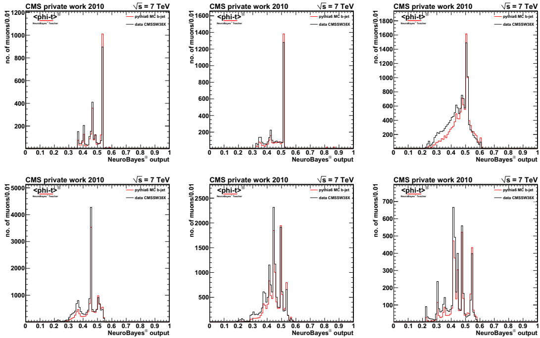
Figure B.4: Result of the comparison of data and MC for muon objects
