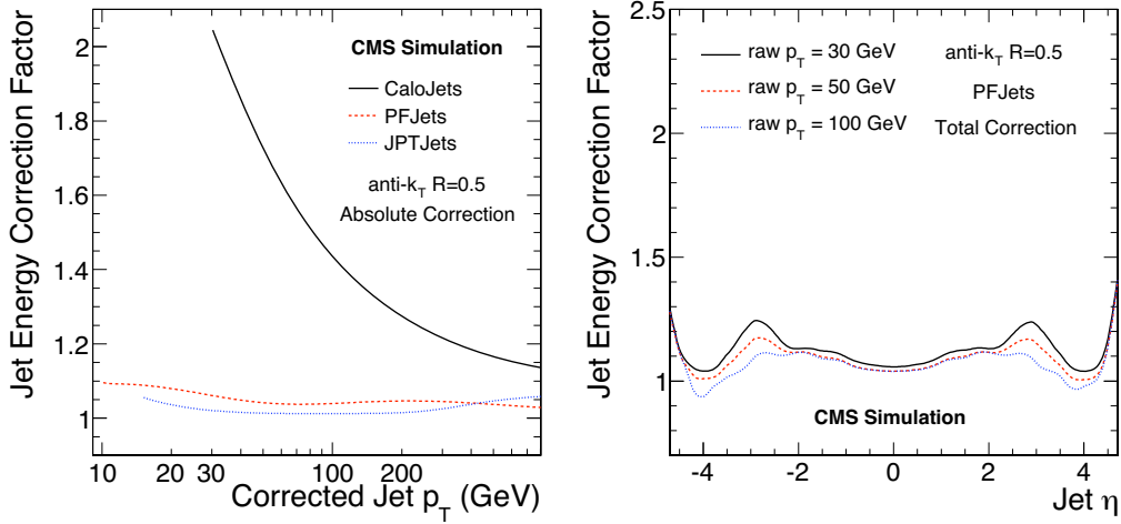
Figure 4.4: Jet energy corrections applied on the PFjets. The multi-step procedure for MC-truth jet energy corrections applies absolute (left), relative corrections (right). 7
