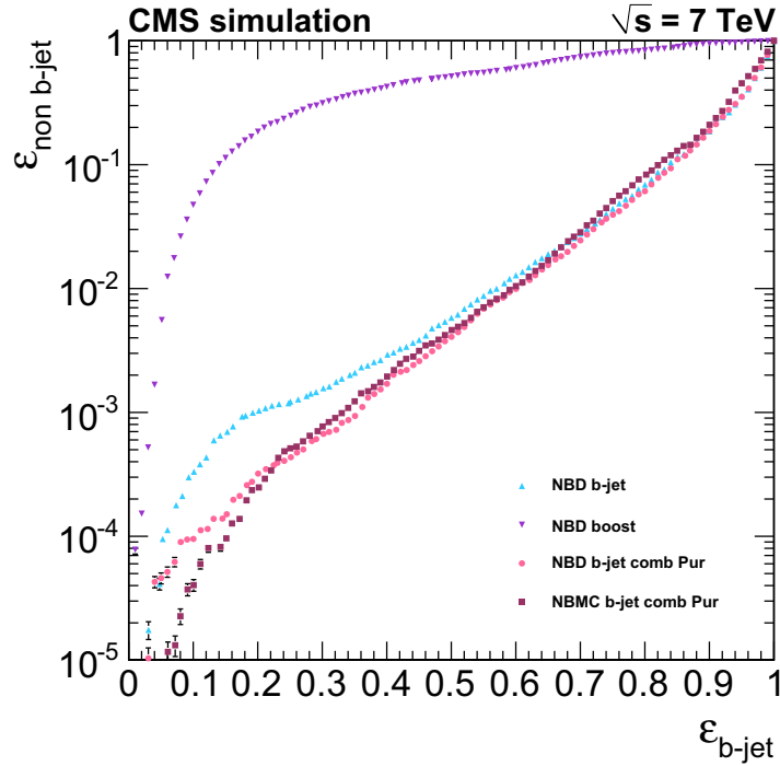
Figure 5.34: Performance of the NeuroBayes data based b-jet tagger. Instead of simulated background events data is used. The performance of this new kind of b-jet tagger is comparable to a MC based.
