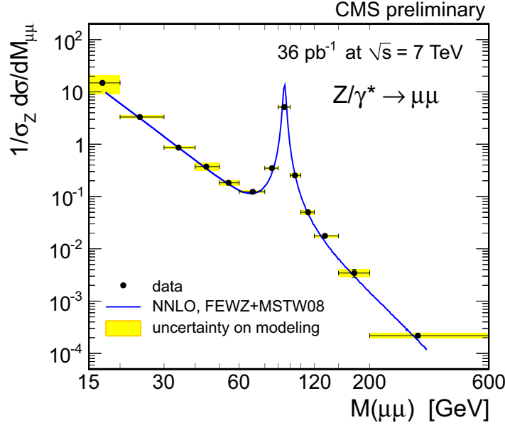
Figure 2.3: The normalized Drell-Yan mass spectrum, (1/\sigma_Z)d\sigma/dM , obtained in the di-muon channel and compared to theoretical predictions. The uncertainty on the modeling accounts for differences in the acceptance corrections obtained with POWHEG and FEWZ. [CMS11]
