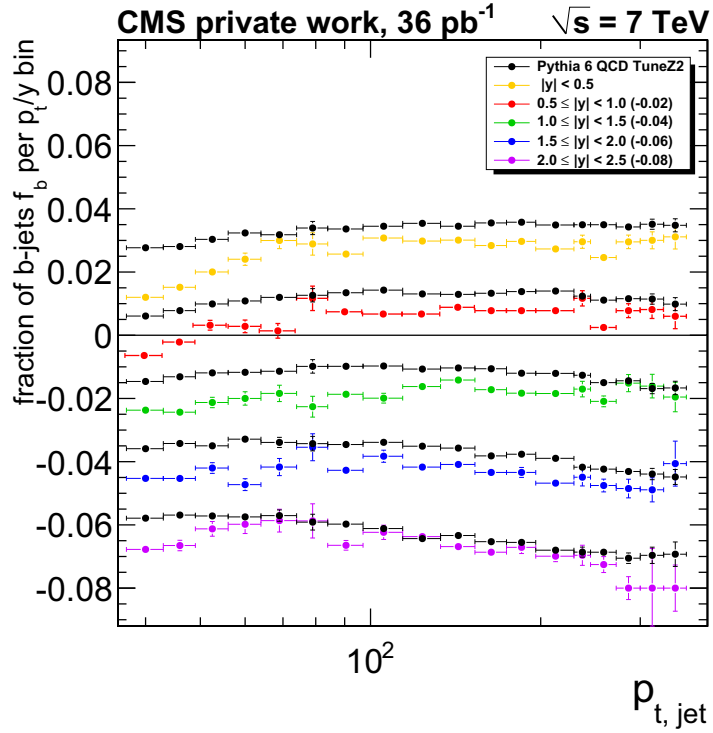
Figure 6.19: The flavour content fitter was used with the NeuroBayes b-jet tagger. the result of the fit in different p_T/y bins is shown. No preselection on the sample was applied. The NeuroBayes variable is sensitive on differences between b-jets and non-b-jets. Due to the differences in the inclusive shapes no convincing fit result is found. The bad application of the fitting procedure points to an insufficient simulation of the jet distributions.
