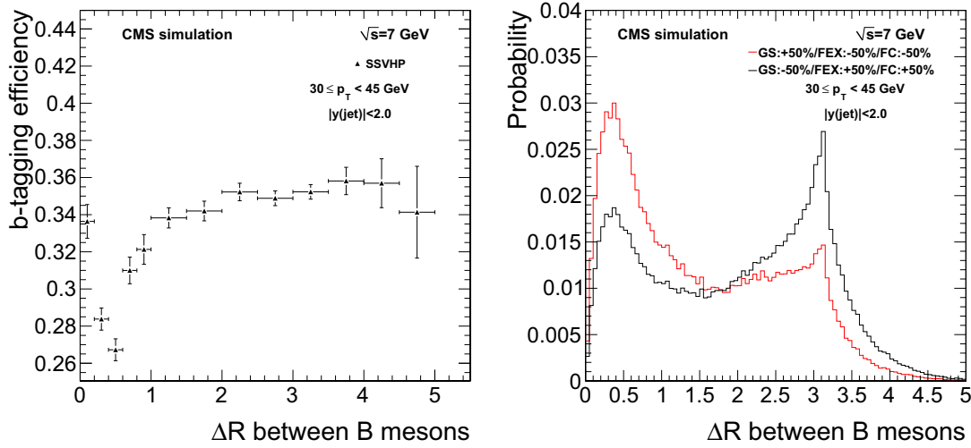
Figure 6.5: The b-tagging efficiency variation versus \Delta R between b-hadrons (left). Distribution of \Delta R between b-hadrons for \pm 50\% variations of GS and FC+FEX (right).
