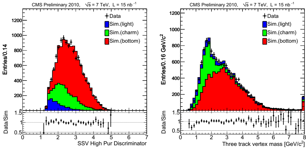
Figure 6.9: Distribution of the simple secondary vertex high purity b-jet tagger and the corresponding vertex mass reconstructed with at least three tracks.
