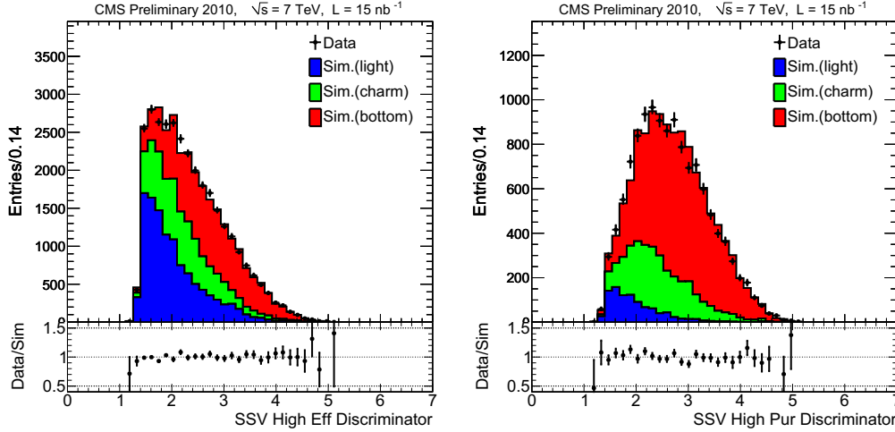
Figure 4.8: Discriminator for the simple secondary vertex b-jet tagger 12
