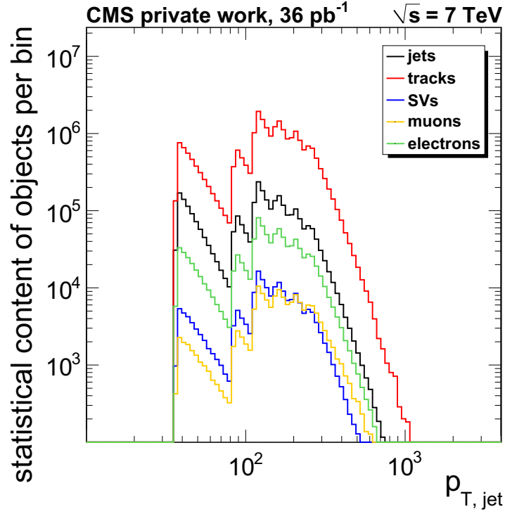
Figure 4.15: Available statistics for different bins in transverse momenta space of the jet. The amount is relevant for the precision of the measurement. Due to trigger prescaling in the low p_T regions, there the statistics are more or less limited perennially to the given number.
