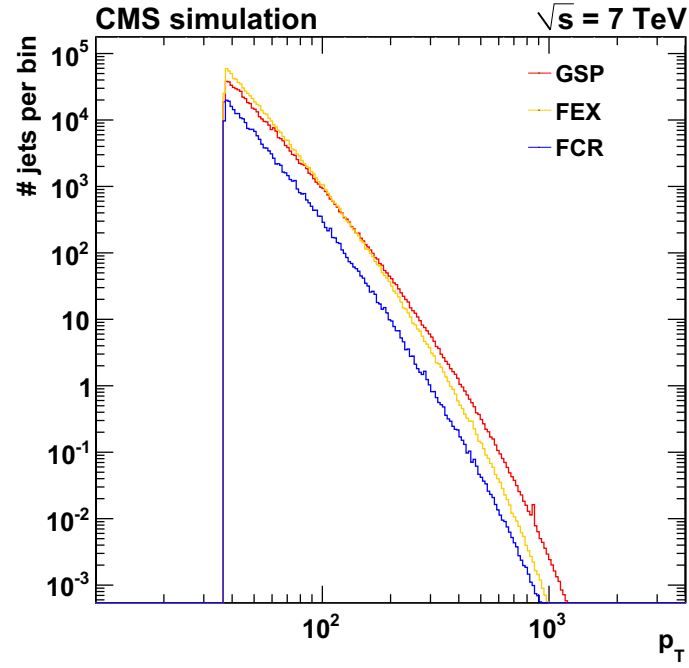
Figure 2.7: Transverse jet momentum spectrum of the different b production mechanisms. For high p_T jets the production is dominated by gluon splitting processes. The plot is done on a Pythia 6 TuneZ2 sample where p_T > 37 GeV.
