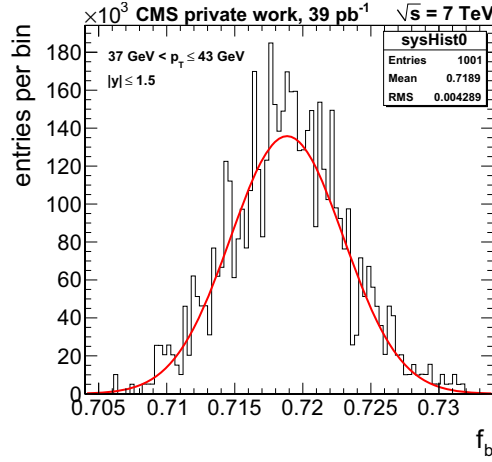
Figure 6.13: The fit results of different f_b estimations with varied templates describe nearly a Gaussian distribution with the mean of the original value. The width of this can be taken as systematic uncertainty \sigma_{tempStat}
