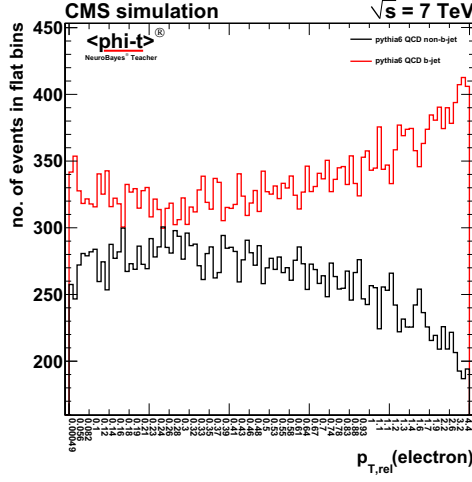
Figure 5.17: Electron candidate object training: Distribution of the transverse momentum of the electron relative to the jet axis.
