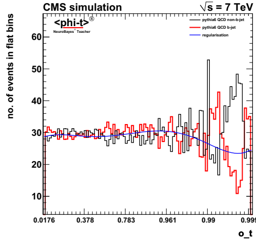
Figure 5.21: The plots show the distribution of the NeuroBayes output of the main expert, which is used as input variable, the boosted NeuroBayes training. The probability interpretation was tested on a well defined binning. The weighting allows us to see the structure within the bins.
