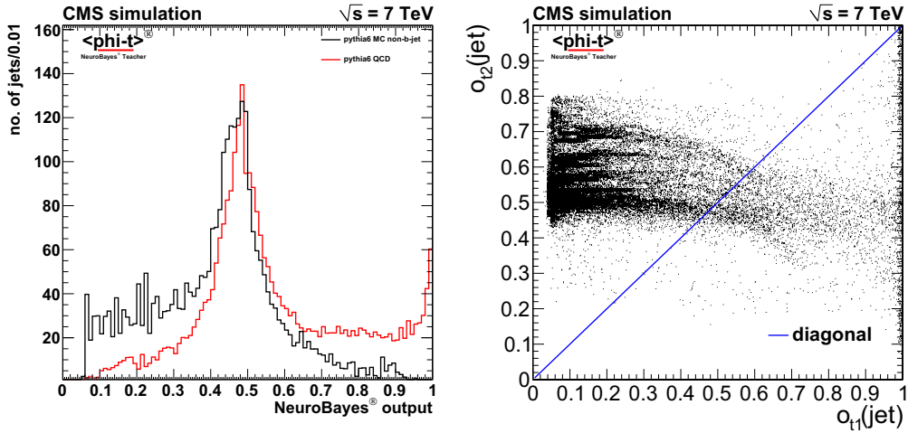
Figure 5.21: The plots show the distribution of the NeuroBayes output of the main expert, which is used as input variable, the boosted NeuroBayes training. The probability interpretation was tested on a well defined binning. The weighting allows us to see the structure within the bins.
