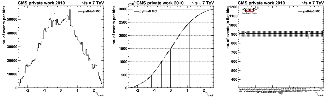
Figure 5.1: Probability integral transform for an exemplary variable. The left histogram shows the original distribution. In middle plot is the cumulative distribution created from the left. Dividing the y-axis in equally sized slices delivers the boundaries of the bins of the right histogram. The content of each bin of the last plot has the same amount of statistics.
