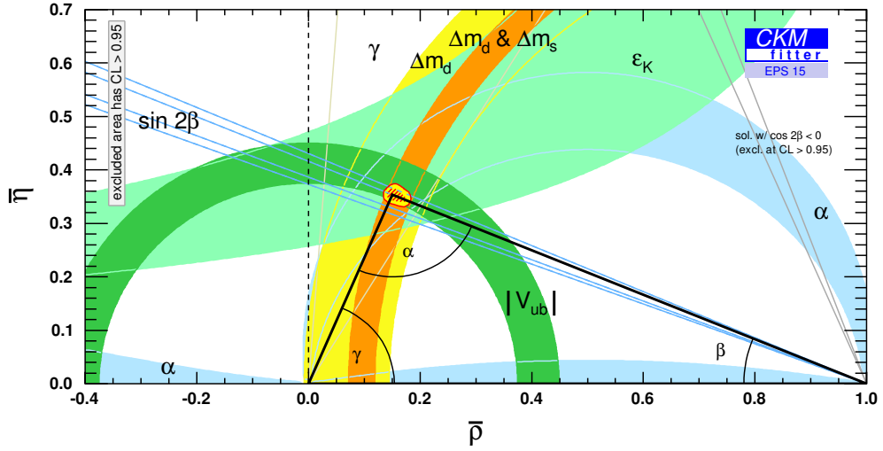
Figure 3.2: Unitarity triangle with constraints from measurements of various quantities [60].
