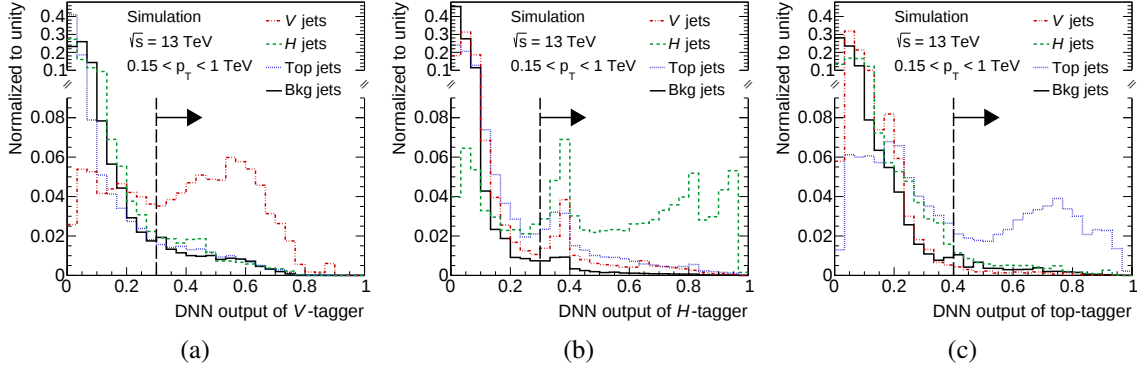
Figure 6.29: DNN output for the standard FLIP V -, H - and top-tagger for the standard FLIP test sample in the RC jet p_T range from 150 GeV to 1 TeV. The arrows show three independent choices of a WP for the V -, H - and top-tagger, possibly leading to ambiguous tags. The four DNN classes V -boson, H -boson, top-quark and background jets are depicted in different colors. All histograms are normalized to unity. For better readability, the vertical axis is split into two intervals.
