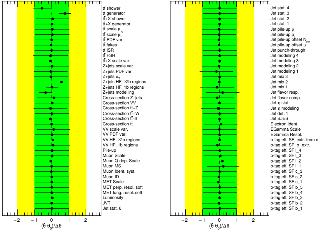
Figure 9.18: Pull plot for the B-only hypothesis used in the observed absence of VLT and VLB quark signal. Pulls of the post-fit mean and post-fit one sigma bands of Gaussian distributed nuisance parameters are illustrated as black dots and horizontal lines on the dots, respectively. A B-only fit is performed for the singlet hypothesis of the VLB quark with m = 1200\text{ GeV} .
