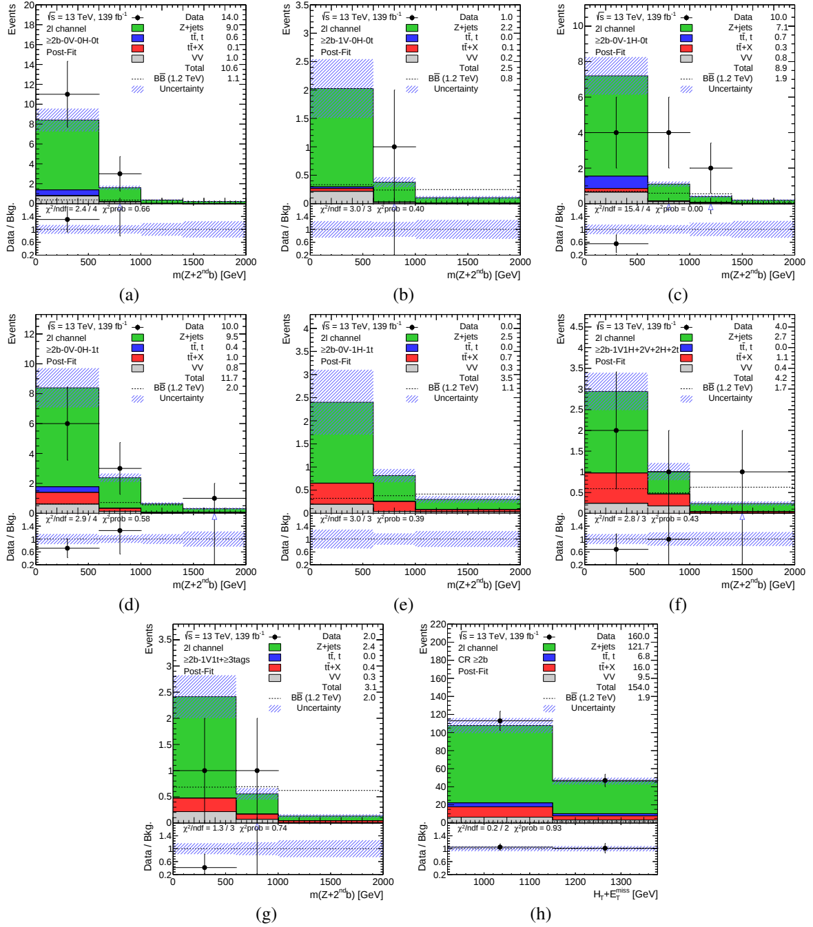
Figure 9.17: Post-fit plots for all categories with at least 2 b -tagged jets with m(Z+2^{\text{nd}}b) as final discriminant. In addition, the CR for at least 2 b -tagged jet with H_T(\text{jets}) + E_T^{\text{miss}} as variable is shown in h). Systematic and statistical uncertainties are included in the uncertainty band. The pre-fit signal for VLB quarks with m = 1200 GeV assuming singlet BRs is overlaid. All backgrounds are depicted and stacked on top of each other. The legend contains the yields of post-fit background, pre-fit VLB signal and data. The subplot shows the ratio of data over the background prediction. Furthermore, the result of a \chi^2 test over the NDF is depicted, as well as the \chi^2 probability.
