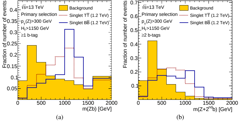
Figure 9.6: Depiction of a) m(Zb) for at least one b -tagged jet and (b) m(Z + 2^{\text{nd}} b) for at least two b -tagged jets in the event. Furthermore, the primary selection and the requirements on p_T(Z) > 300\text{ GeV} and H_T(\text{jets}) > 1150\text{ GeV} are applied. Both pair-production benchmark signal masses for VLT and VLB quarks at 1200 GeV are shown, as well as a sum of all background processes. The under- and overflow bins are included.
