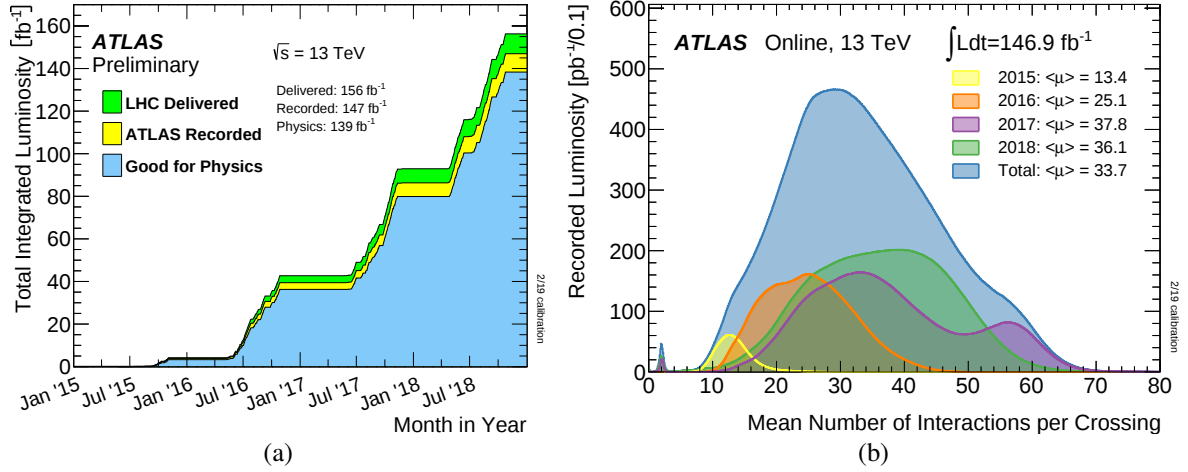
Figure 4.1: Illustration of a) the integrated luminosity recorded during Run-2 and b) the average number of pile-up events \langle\mu\rangle per bunch-crossing for all years of data taking during Run-2 of the ATLAS detector [76].
