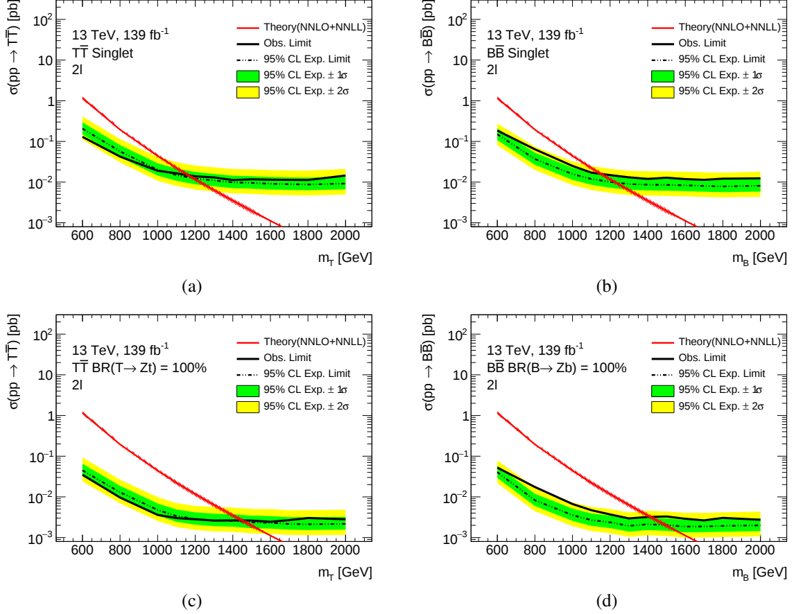
Figure C.4: Expected and observed limits on the cross-section for T\bar{T} and B\bar{B} production from the 2\ell channel of the Z(\ell\ell)t/b + X analysis at 95% CL using 139\text{ fb}^{-1} . The limits for VLT quarks are illustrated for a) the singlet model and c) the 100% BR into Zt . The limits for VLB quarks are depicted for b) singlet model and d) BR( B \rightarrow Zb ) \rightarrow 100%. The \pm 1(2)\sigma band of the 95% CL limit are depicted in green (yellow). The theory curve is shown in red.
