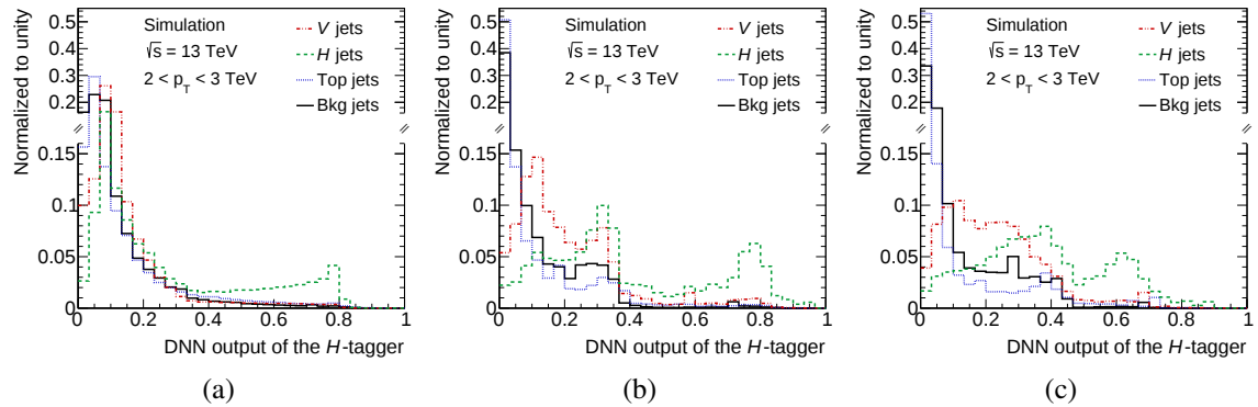
Figure A.2: DNN output distributions of the H -tagger for a) the NFLIP tagger, b) the standard FLIP tagger and c) the b -tag enriched FLIP tagger from 2–3 TeV. The four DNN classes V -boson, H -boson, top-quark and background jets are depicted in different colors. All histograms are normalized to unity. For better readability, the vertical axis is split into two intervals.
