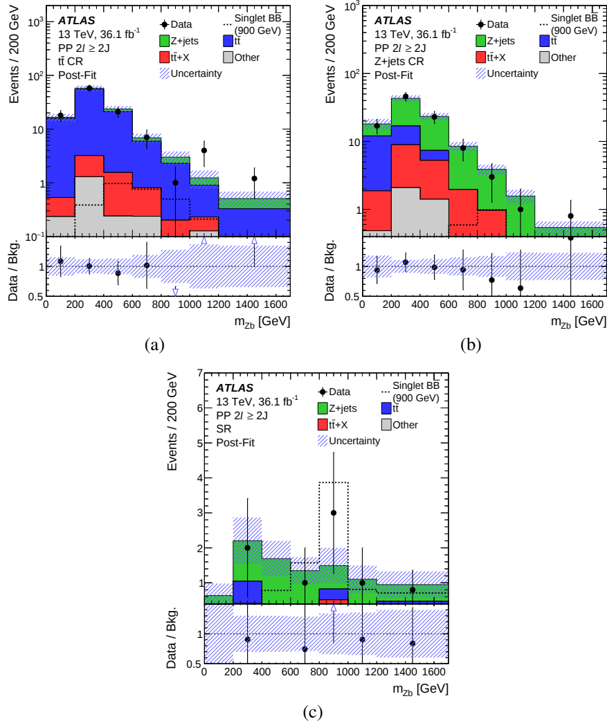
Figure 8.9: Post-fit distributions [3] for the final discriminant m(Zb) in the a) t\bar{t} CR, b) Z + \text{jets} CR and c) SR. Signal according to the pre-fit hypothesis is overlaid. All systematic uncertainties are included. The background is modeled according to the B-only hypothesis. The lower plot shows the ratio of data over the background expectation.
