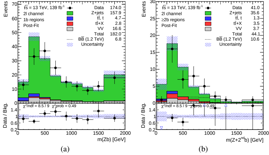
Figure 9.15: Post-fit distributions of a) m(Zb) for exactly one b -tagged jet and b) m(Z + 2^{\text{nd}} b) after requiring at least two b -tagged jets. The full selection is applied for both distributions. The VLB quark signal at 1.2 TeV with singlet BRs according to the pre-fit hypothesis is overlaid. Systematic and statistical uncertainties are included in the uncertainty band. The background is modeled according to the B-only hypothesis. The subplot shows the ratio of data over the background prediction. Furthermore, the results of a \chi^2 test over the NDF are depicted, as well as the \chi^2 probabilities.
