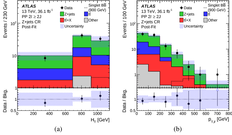
Figure 8.7: Post-fit distributions for a) H_T(\text{jets}) [3] and b) p_T(Z) [154] in the Z + jets CR. Signal according to the pre-fit hypothesis is overlaid. All systematic uncertainties are included. The background is modeled according to the B-only hypothesis. The lower plot shows the ratio of data over the background expectation.
