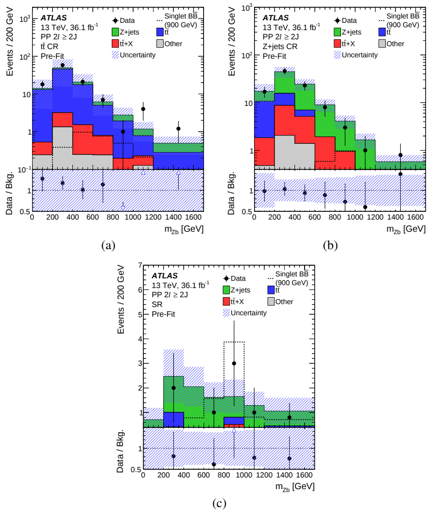
Figure B.1: Pre-fit distributions [154] for m(Zb) in all three regions. The t\bar{t} CR and Z +jets CR are shown in a) and b), respectively, while the SR is shown in c). Signal according to the pre-fit hypothesis is overlaid. All systematic uncertainties are included. The background is modeled according to the B-only hypothesis. The lower plot shows the ratio of data over the background expectation.
