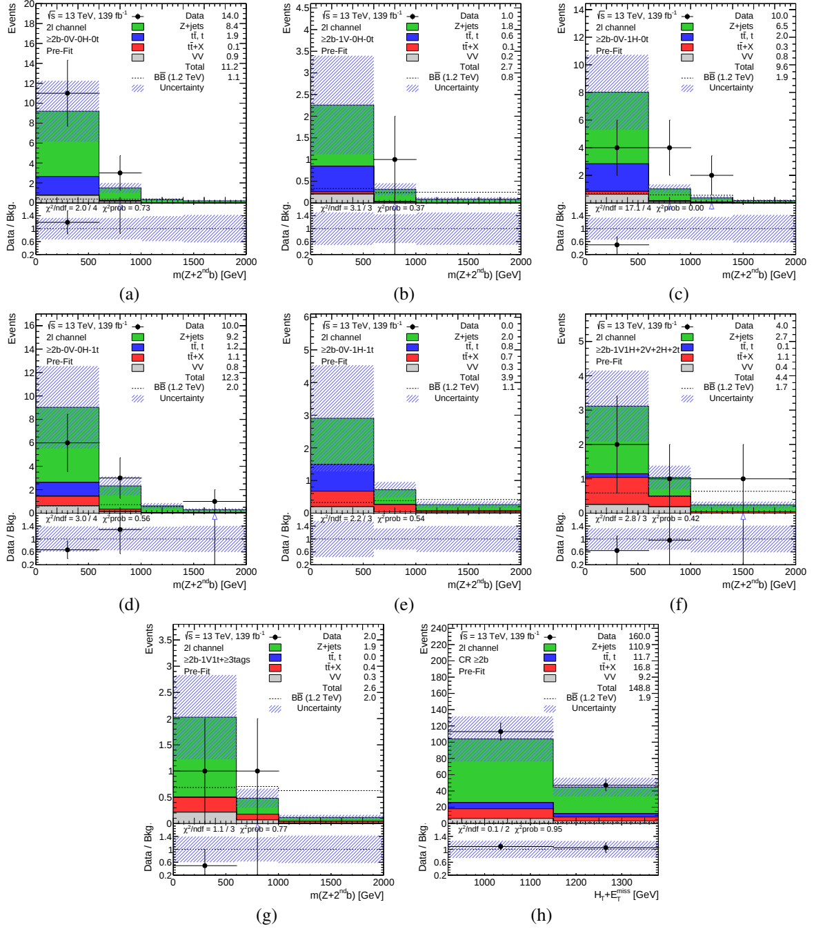
Figure C.3: Pre-fit plots for all categories with at least 2 b -tagged jets with m(Z+2^{\text{nd}}b) as final discriminant. In addition, the CR for at least 2 b -tagged jet with H_T(\text{jets}) + E_T^{\text{miss}} as variable is shown in h). Systematic and statistical uncertainties are included in the uncertainty band. The pre-fit signal for VLB quarks with m = 1200 \text{ GeV} assuming singlet BRs is overlaid. All backgrounds are depicted and stacked on top of each other. The legend contains the yields of pre-fit background, pre-fit VLB signal and data. The subplot shows the ratio of data over the background prediction. Furthermore, the result of a \chi^2 test over the NDF is depicted, as well as the \chi^2 probability.
