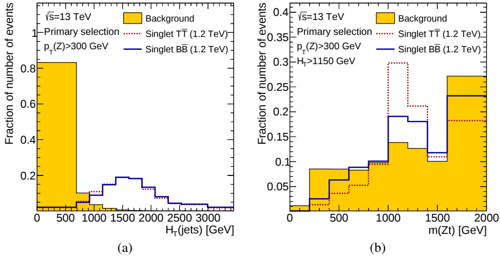
Figure 9.7: Depiction of a) H_T(\text{jets}) after applying the p_T(Z) > 300 GeV cut and b) m(Zt) after applying the p_T(Z) > 300 GeV and H_T(\text{jets}) > 1150 GeV cuts. Both pair-production benchmark signal masses for VLT and VLB quarks at 1200 GeV are shown, as well as a sum of all background processes. The under- and overflow bins are included.
