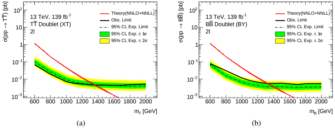
Figure 9.20: Expected and observed limits at 95% CL on the cross-section for a) T\bar{T} and b) B\bar{B} production with BRs according to the doublet models ( X, T ) (or (T, B) ) and (B, Y) , respectively. The 2\ell channel of the Z(\ell\ell)t/b + X analysis using 139\text{ fb}^{-1} is shown. The \pm 1(2)\sigma bands of the expected limit at 95% CL are depicted in green (yellow). The theory curve is shown in red.
