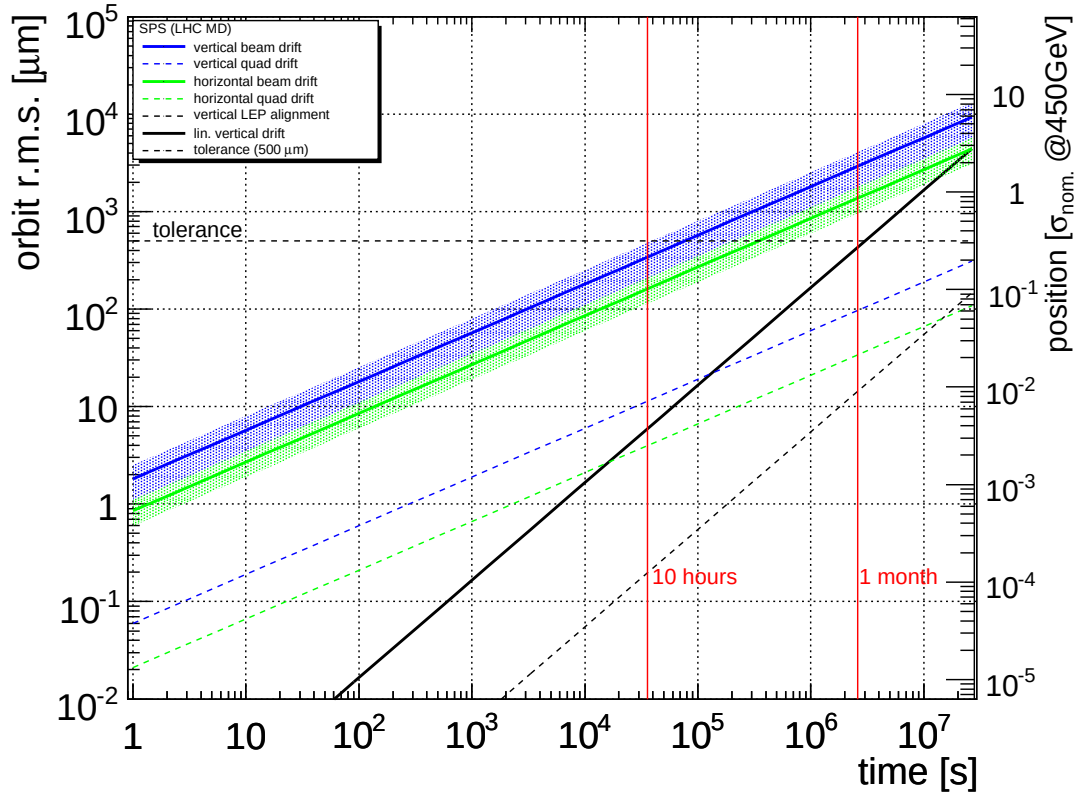
Figure 4.21: Expected SPS r.m.s. orbit drift due to random ground motion. The corresponding drift in units of nominal beam size \sigma ( 3.75 \mu\text{m} rad emittance and for 450 \text{ GeV} ) is given on the right scale. The range corresponds to the parameter \kappa spread of the model. The tolerance corresponds to the maximum permissible orbit shift at the extraction point to the LHC.
