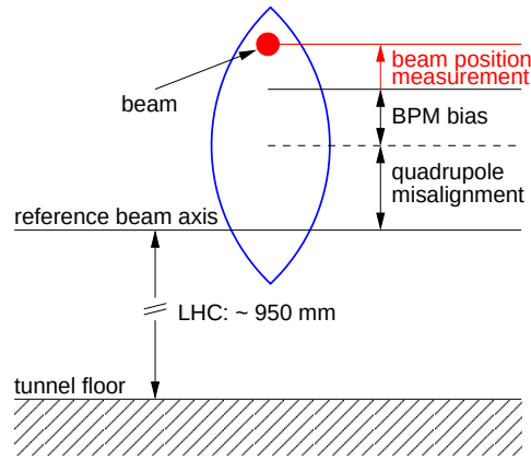
Figure 5.11: Local reference system. Not to scale.
