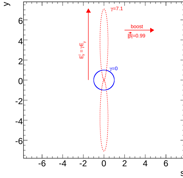
Figure 2.1: Equipotential surface in charged particle's frame of rest (blue) and as observed in \beta = v_s/c = 0.99 boosted frame of reference. The transverse field enhancement by \gamma = 7.1 is visible. For LHC energies ( \gamma > 400 ), the electrical field is compressed into discs travelling along the individual protons.
