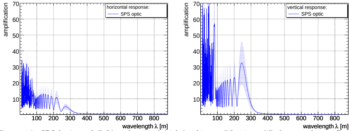
Figure 4.3: SPS horizontal (left) and vertical (right) orbit amplification \kappa(f) due to coherent P- and S-wave oscillations. The amplification is shown as a function of wavelength. The first resonance once the wavelength drops below the betatron-wavelength of about 264 m is visible.
