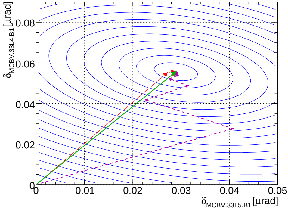
Figure 6.10: SVD error contour: The perfect correction (solid green), the correction with optics error (dotted red) and COD calibration errors (dashed violet) are indicated. The contours represent constant values of the residual orbit error. Independent of the type of error, the corrections converge to the same optimal setting. However, the number of iterations required varies.
