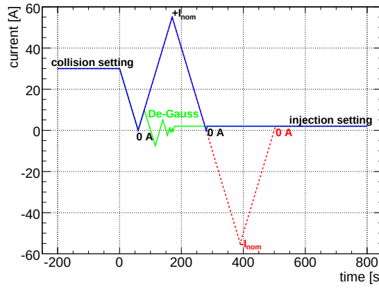
Figure 4.33: Schematic COD pre-cycles: cycle through positive saturation only (blue curve), through positive and negative saturation (red curve), or using a De-Gauss cycle with reducing amplitude (green curve).
