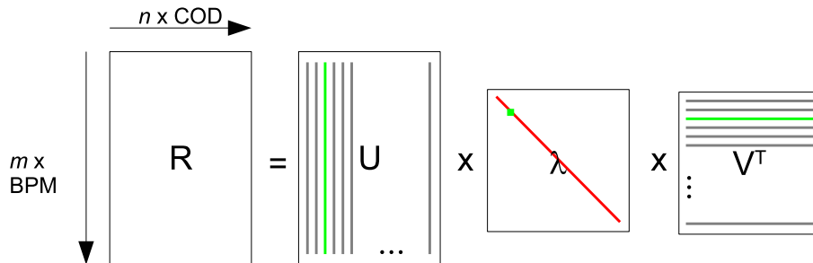
Figure 6.4: Schematic of the Singular Value Decomposition (SVD): An arbitrary real matrix \mathbf{R} with dimension m \times n can be decomposed into a rectangular matrix \mathbf{U} \in \mathbb{R}^{m \times n} , diagonal eigenvalue matrix \boldsymbol{\lambda} = \text{diag}(\lambda_1, \dots, \lambda_n) \in \mathbb{R}^{n \times n} and transpose eigenvector matrix \mathbf{V}^T \in \mathbb{R}^{n \times n} .
