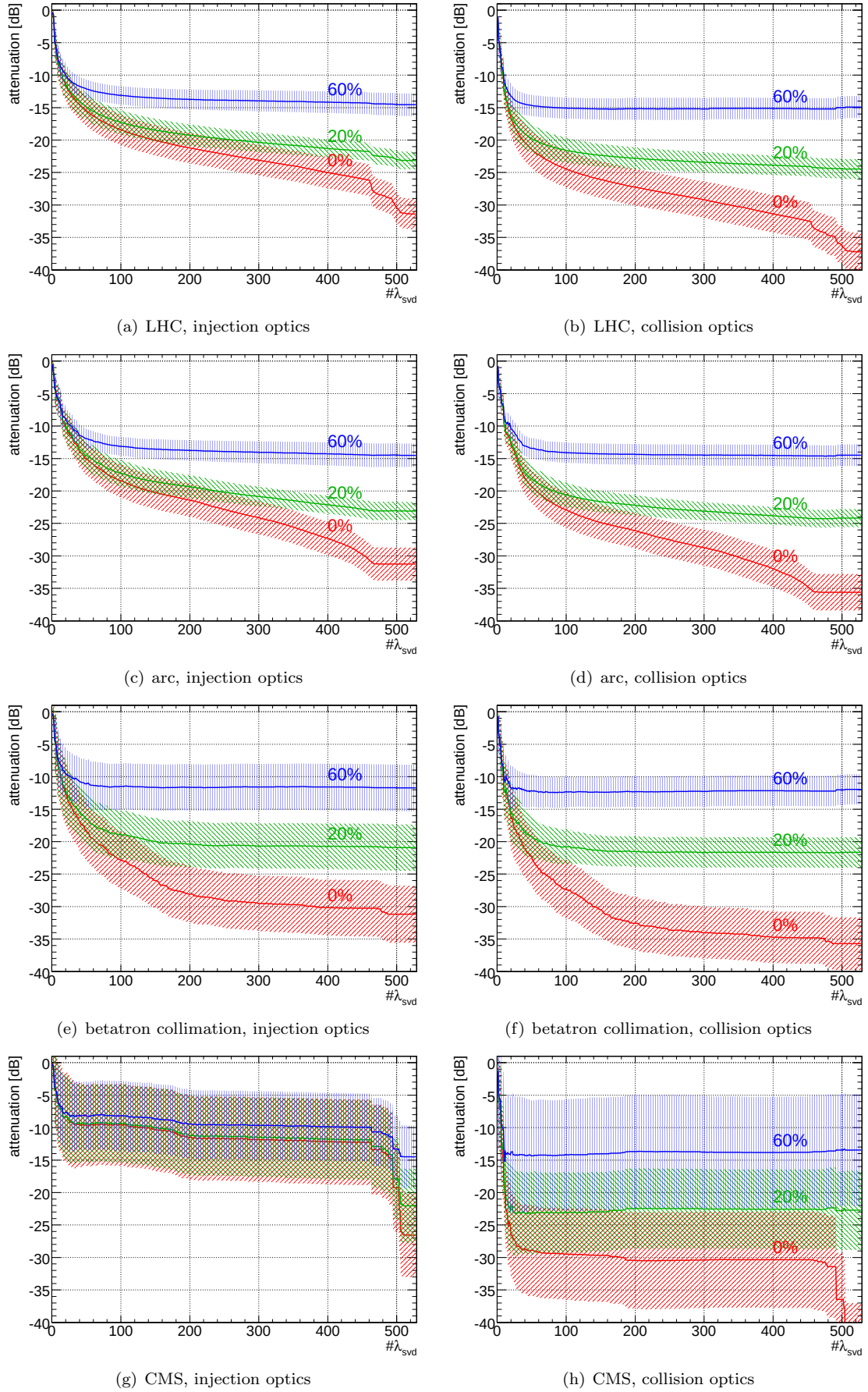
Figure 6.12: Attenuation of SVD-based orbit correction as a function of used eigenvalues \#\lambda_{\text{svd}} for 0, 20 and 60% peak-to-peak beta-beat. The correction is based on all available correctors and monitors.
