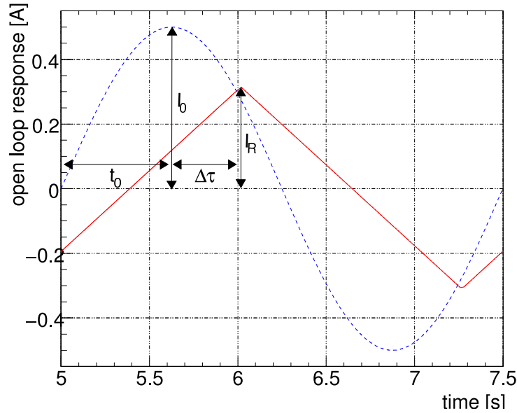
Figure 5.17: Rate limiter response. The additional delay due to the rate limiter is visible.
