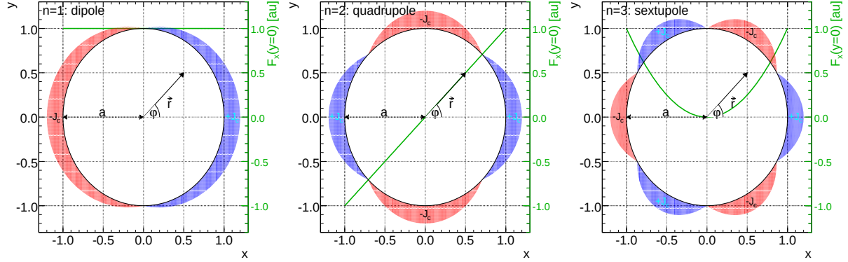
Figure 1.9: The \cos(n\phi) current distributions for superconducting dipoles (dipoles), quadrupoles (middle) and sextuples (right) are shown. The colours ( \pm signs) indicate whether the polarity of the current density J_c is going 'in' (red, '-') or coming 'out' (blue, '+') of the drawing plane.
