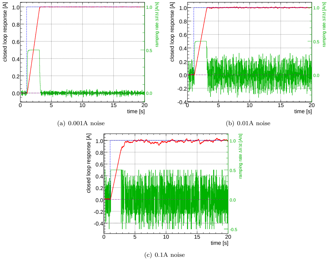
Figure 6.34: Measurement noise rejection. The equivalent BPM noise levels are \pm 13 \mu ( 0.1 \text{ A} ), \pm 1.3 \mu ( 0.01 \text{ A} ) and \pm 0.13 \mu ( 0.001 \text{ A} ). The minimum relative noise reduction is about a factor of two for a signal-to-noise ratio of 20 \text{ dB} .
