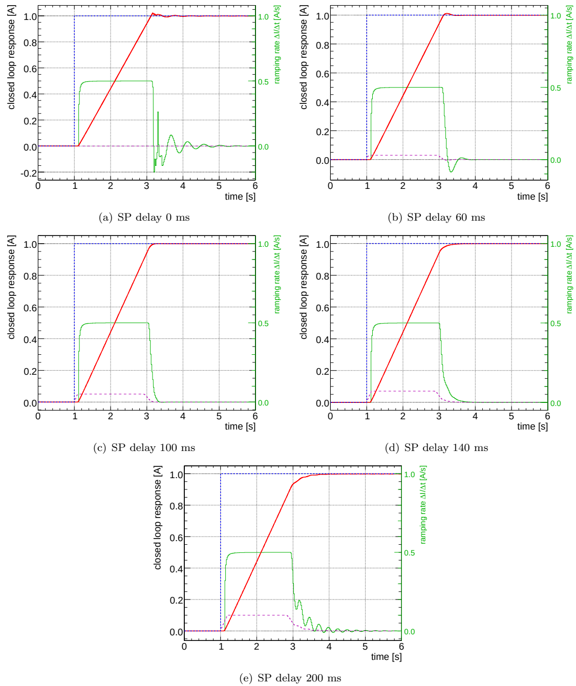
Figure 6.27: Effect of the the Smith predictor under various compensated delay mismatches. The true open-loop delay is 100 ms.
