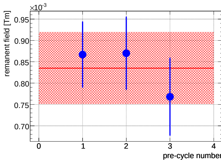
Figure 4.34: Field reproducibility at 0 A after pre-cycling the magnet through saturation. The plotted error bars (area) correspond to 1 \sigma r.m.s.
