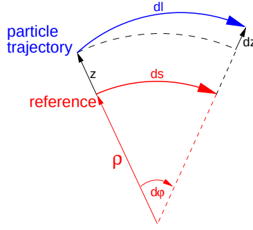
Figure 2.7: Pathlength difference of the perturbed orbit with respect to the design orbit over a short angular segment d\phi of the accelerator.
