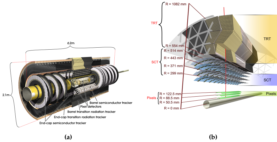
Figure 2.6: Schematic view of the ATLAS Inner Detector (a) and details of its barrel section (b) [84].
