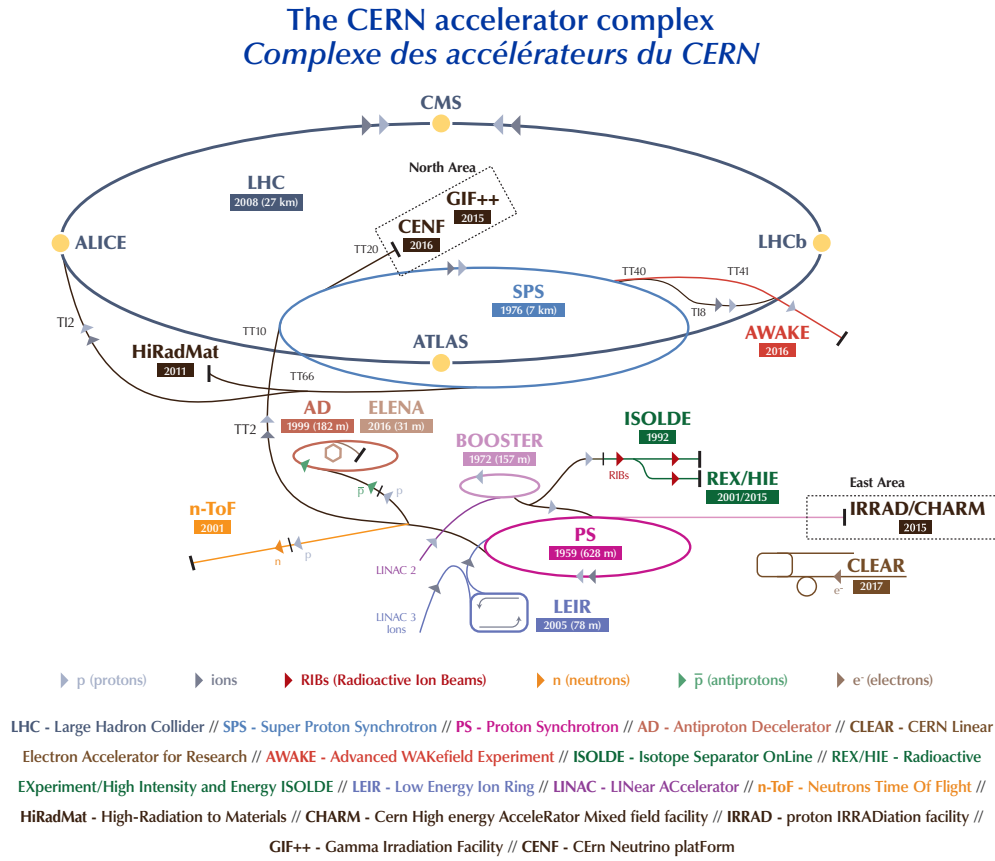
Figure 2.1: Schematics of the CERN accelerator complex, with the different accelerators and detectors [75].
