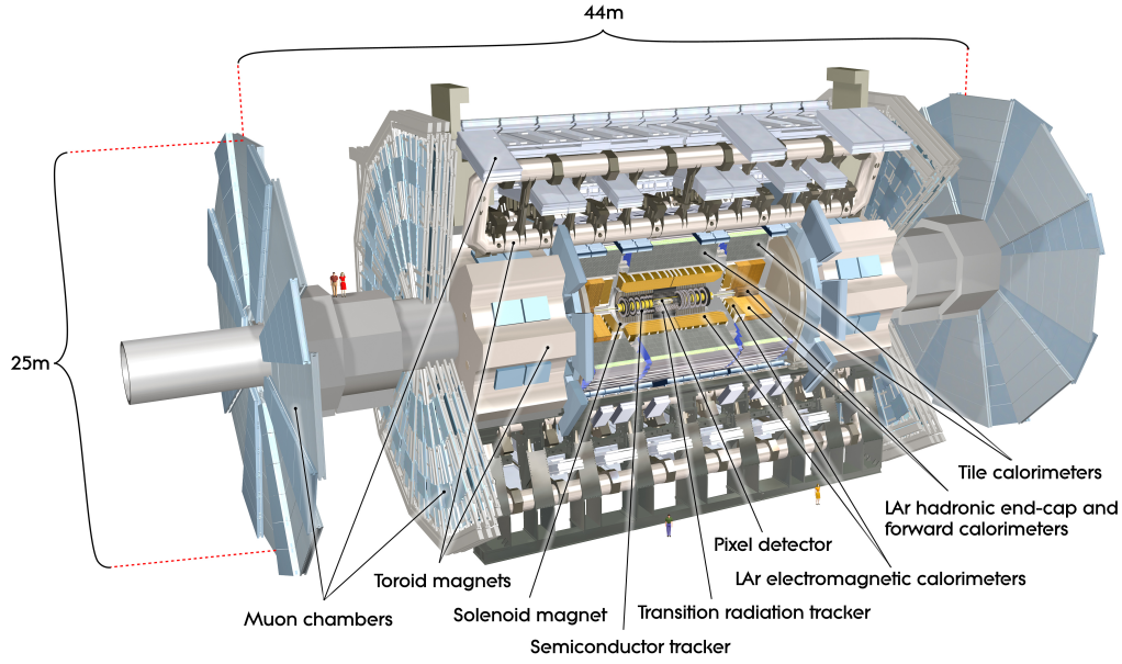
Figure 2.4: Schematic overview of the ATLAS detector [84].
