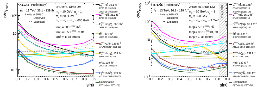
Figure 7.17: Observed (solid lines) and expected (dashed lines) exclusion limits at 95% CL for the 2HDM+a model as a function of \sin\theta with m_A = 600 GeV, m_a = 200 GeV (left) and m_A = 1 TeV, m_a = 350 GeV (right). The results are shown for several individual searches as well as the combination of the E_T^{\text{miss}} + Z(\ell^+\ell^-) and E_T^{\text{miss}} + h(b\bar{b}) searches.
