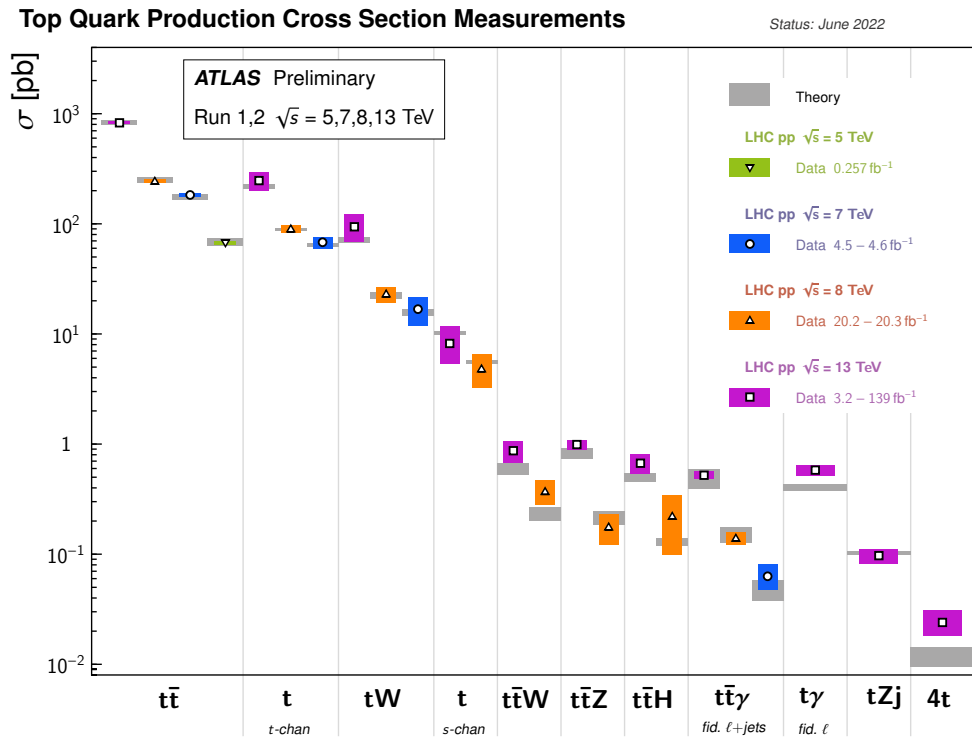
Figure 1.6: Summary of several top-quark related production cross-section measurements, compared to the corresponding theoretical expectations. All theoretical expectations were calculated at NLO or higher [34].
