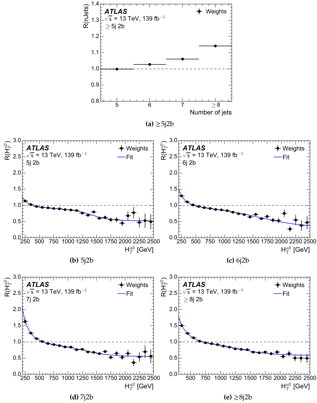
Figure 6.6: Reweighting factors (weights) obtained from the comparison between data and simulation of the number of jets (a) and H_T^{all} for various jet multiplicity selections (b) to (e). The errors in the data points include the statistical uncertainties in data and MC predictions.
