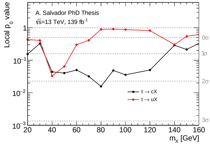
Figure 9.5: p_0 values for the fitted signal strength as a function of the mass of X for the t \rightarrow cX (black) and t \rightarrow uX (red) signal fits.
