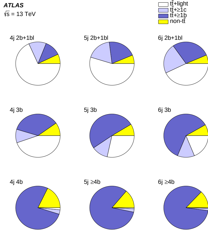
Figure 8.2: Background composition in the various analysis regions.
