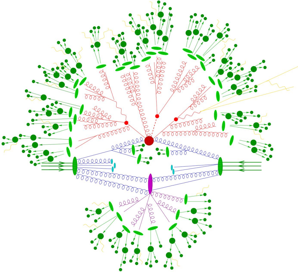
Figure 3.1: Illustration of a proton-proton collision as simulated by a Monte-Carlo event generator. The hard interaction (red blob in the center) is produced from the initial-state partons from the protons (blue), followed by the decay of two top-quarks and a Higgs boson (small red blobs). Additional QCD radiation is produced both before (red) and after (dark green) the final-state partons hadronise. The light green blobs correspond to the hadronisation process of the produced particles and the cyan blobs correspond to the hadronisation of the partons from the proton that did not interact. Also, a secondary interaction (purple) and photon radiation (yellow) are represented. No pile-up effects are illustrated [103].
