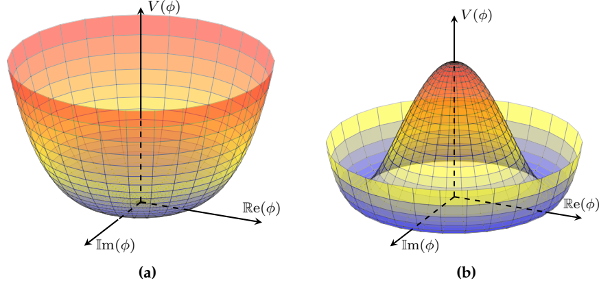
Figure 1.2: Shape of the potential V(\phi) for \lambda > 0 and (a) \mu^2 > 0 or (b) \mu^2 < 0 .
