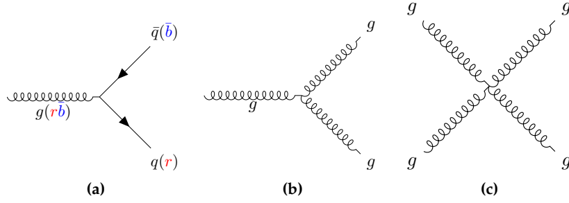
Figure 1.1: Vertices allowed in QCD: (a) quark-gluon coupling, (b) three-point gluon self-coupling, and (c) four-point gluon self-coupling. The colour charge is shown in the quark-gluon vertex to depict an example of the interaction.
