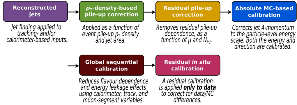
Figure 4.3: Stages of jet energy scale calibrations, all applied to the four-momentum of the jet [141].
