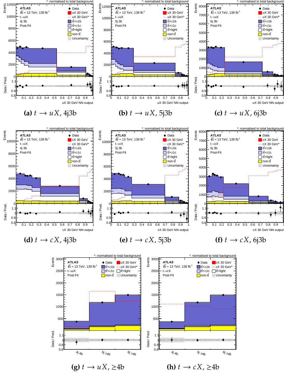
Figure 9.1: Comparison between the data and prediction for the NN output in the 3b regions for the t \rightarrow uX ((a) to (c)) and the t \rightarrow cX ((d) to (f)) processes, and the yields in the \geq 4b regions for the t \rightarrow uX (g) and the t \rightarrow cX (h) processes after the signal-plus-background fit to data under the 30 GeV X scalar mass hypothesis.
