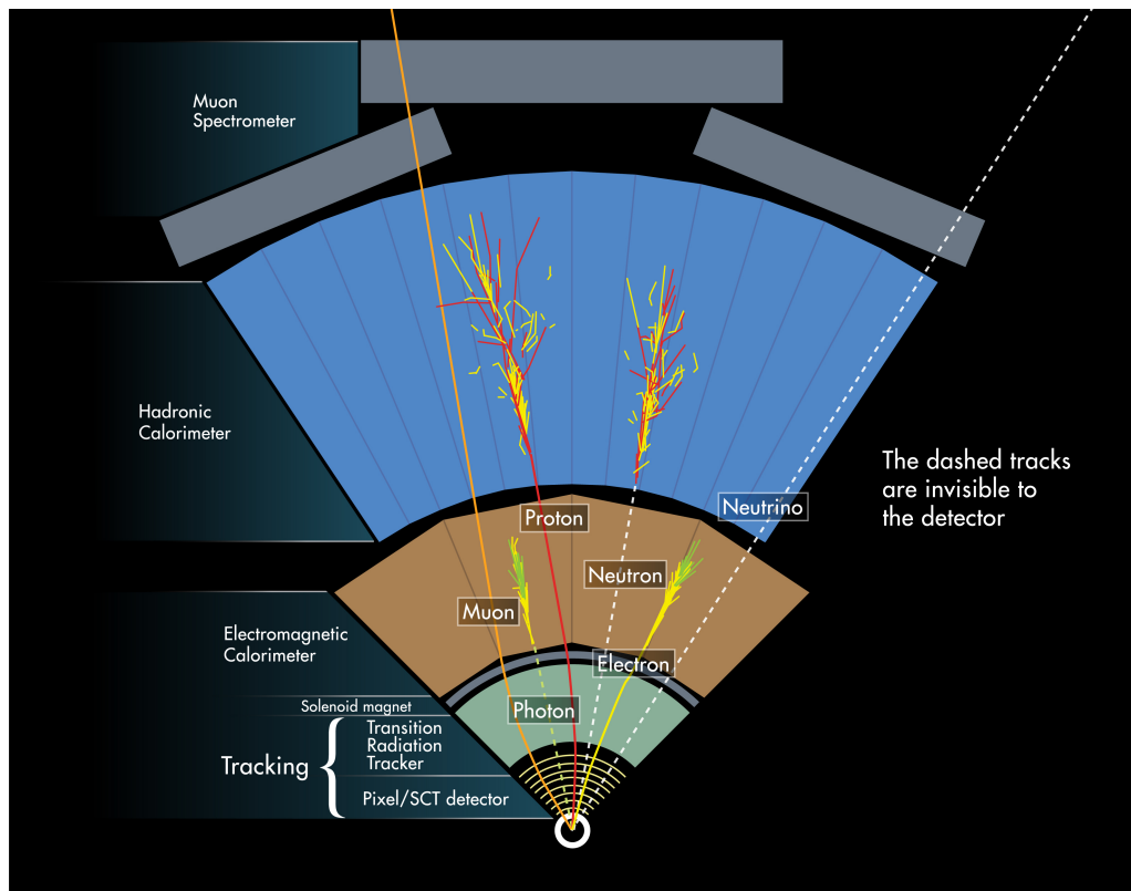
Figure 4.1: Illustration of a section of the ATLAS detector showing the interaction of particles with the different sub-detectors [137].
