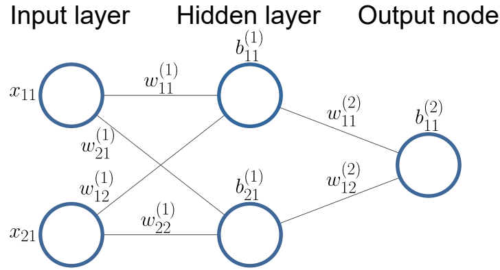
Figure 5.2: Fully connected feed-forward neural network with two input nodes, one hidden layer with two nodes and one output node.
