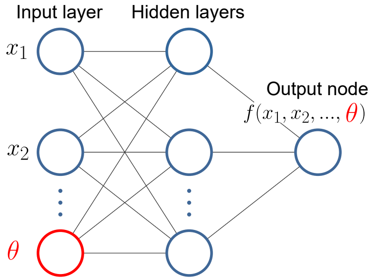
Figure 5.3: Simple schematic of a fully connected feed-forward Neural network with input features x_1, x_2, \dots as well as an input parameter \theta , such that the response f depends on it.
