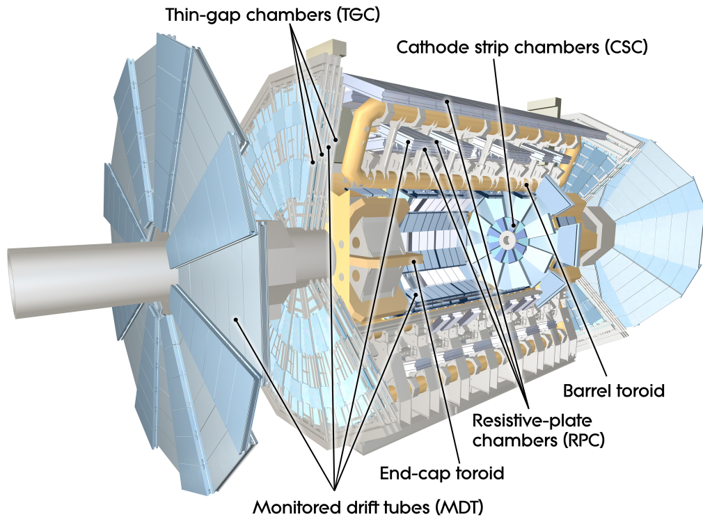
Figure 2.8: Schematic overview of the ATLAS muon spectrometer [84].
