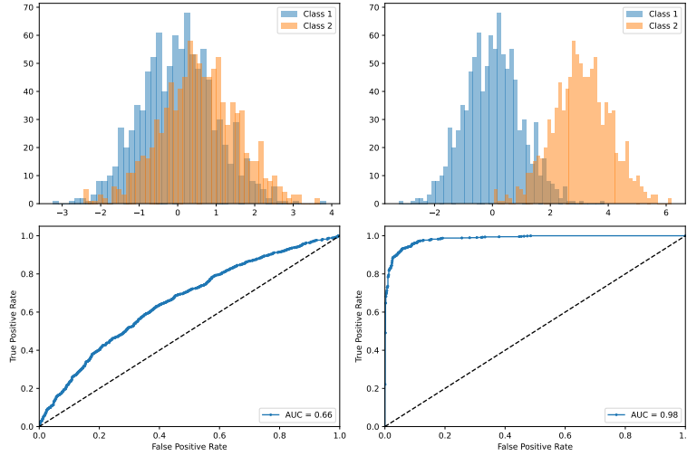
Figure 5.1: Comparison of two Gaussian distributions and their corresponding ROC curves to illustrate the behaviour of the ROC curve and the AUC.
