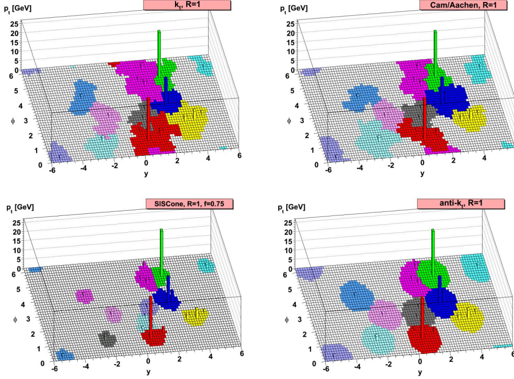
Figure 4.2: Illustration of different clustering algorithms. The anti- k_t (bottom right) shows cone-like structure around the track with the highest momentum [138].
