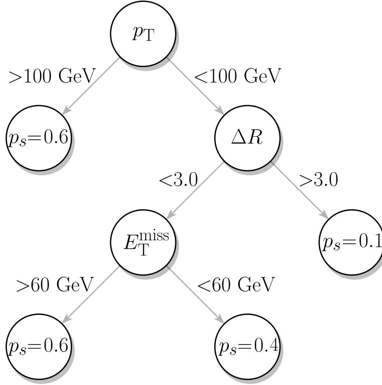
Figure 5.4: Schematic representation of a decision tree trained on a dataset composed of signal and background events with example training variables and cuts. The output of the tree is the probability that each event has of being generated by signal. Values above (below) 0.5 correspond to signal-like (background-like) events.
