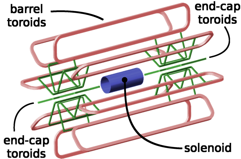
Figure 2.9: Schematic overview of the ATLAS magnet system [99].
