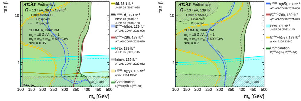
Figure 7.16: Observed (solid lines) and expected (dashed lines) exclusion regions at 95% CL in the m_a - \tan\beta plane with \sin\theta = 0.35 (left) and \sin\theta = 0.7 (right). The results are shown for several individual searches as well as the combination of the E_T^{\text{miss}} + Z(\ell^+\ell^-) and E_T^{\text{miss}} + h(b\bar{b}) searches. The dashed grey regions indicate the region where the width of the Higgs bosons exceeds 20% of its mass.
