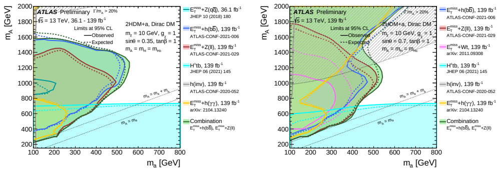
Figure 7.14: Observed (solid lines) and expected (dashed lines) exclusion regions at 95% CL in the m_a - m_A plane with \sin \theta = 0.35 (left) and \sin \theta = 0.7 (right). The results are shown for several individual searches as well as the combination of the E_T^{\text{miss}} + Z(\ell^+ \ell^-) and E_T^{\text{miss}} + h(b\bar{b}) searches. The dashed grey regions indicate the region where the width of the Higgs bosons exceeds 20% of its mass.
