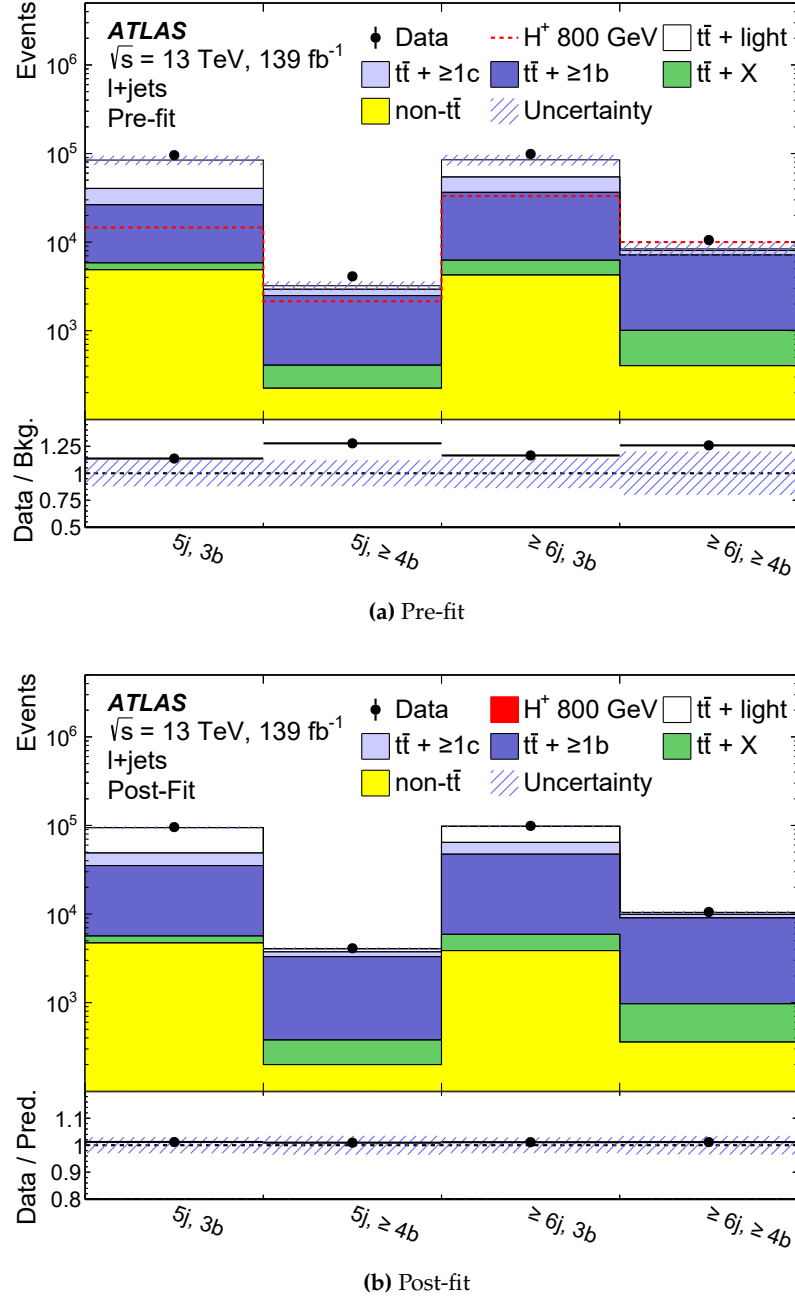
Figure 7.1: Comparison of predicted and observed event yields before (a) and after (b) the fit in each of the signal regions for the 800 GeV hypothesis. The lower panel displays the ratio of the data to the total prediction and the hatched band shows the uncertainties. The pre-fit yields of a charged Higgs boson with a mass of 800 GeV corresponding to a cross-section of 10 pb are overlaid in red in the figure before the fit.
