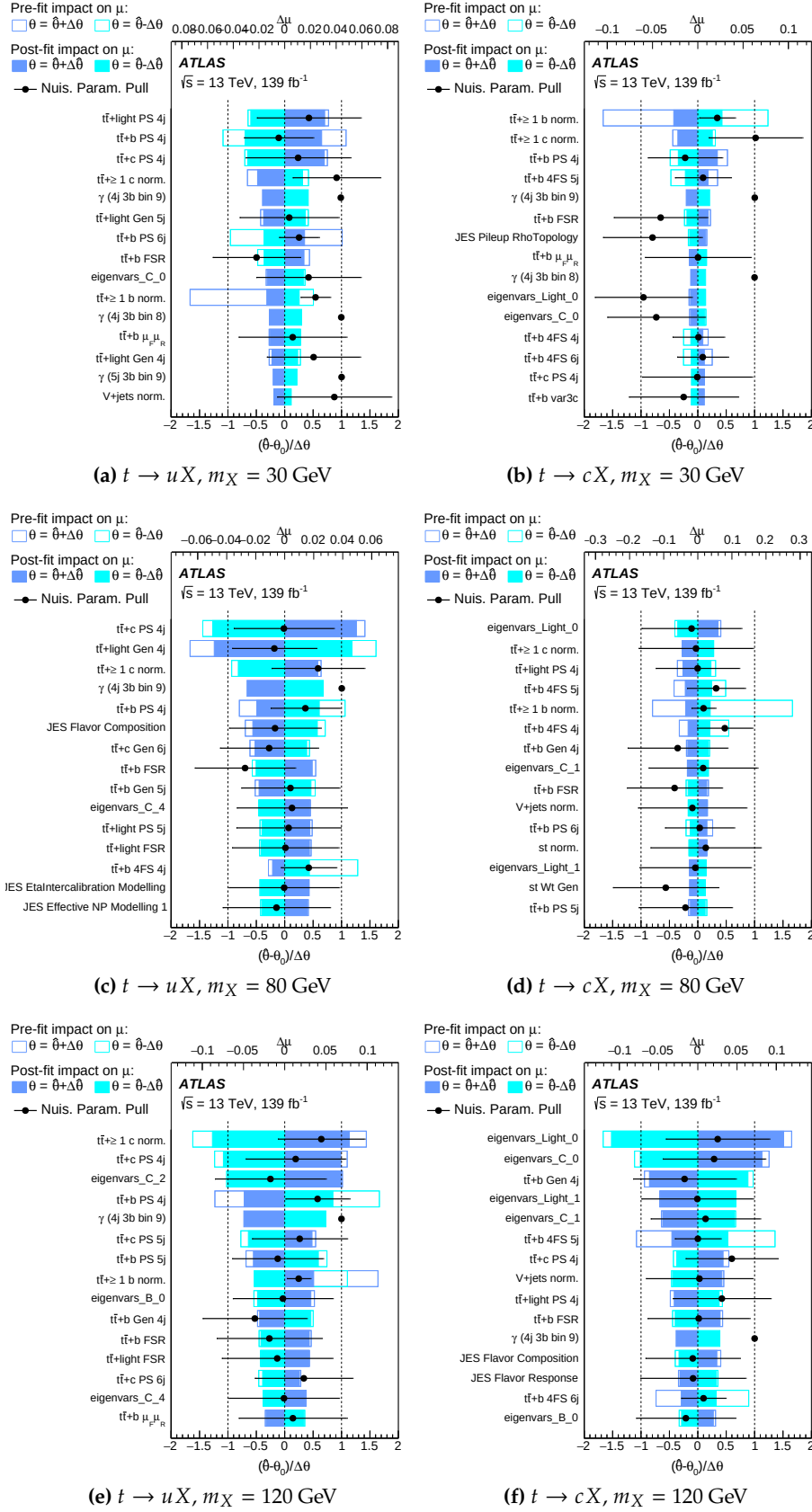
Figure 9.6: Ranking of the 15 systematic uncertainties with the largest impact on \mu for the fits performed with the 30 GeV (top), 80 GeV (middle), 120 GeV (bottom) m_X hypotheses and for the t \rightarrow uX (left) and t \rightarrow cX (right) processes. The empty (filled) rectangles correspond to the pre-fit (post-fit) impact on \mu . The black points represent the post-fit pulls of the nuisance parameters relative to the nominal values, \theta_0 . Statistical uncertainties ( \gamma ) are shown pulled with respect to 1.
