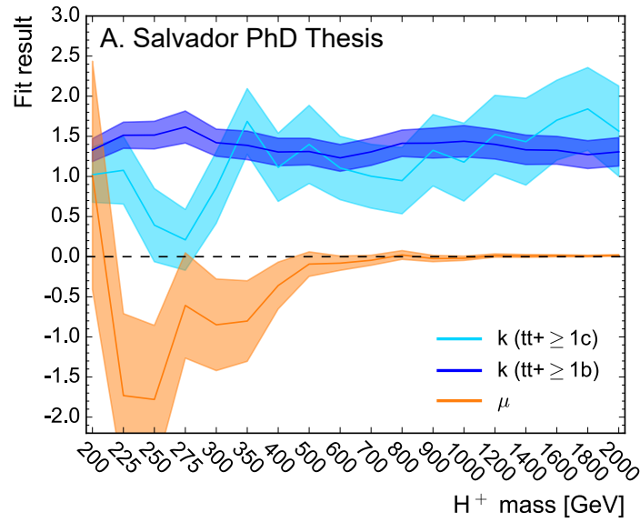
Figure 7.6: Signal strength and t\bar{t} +HF normalisation factors after the fit as a function of the H^+ mass with the corresponding uncertainties. The signal cross-section is normalised to 1 pb.
