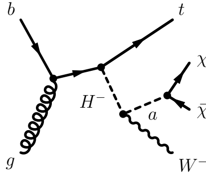
Figure 7.10: Representative Feynman diagram for the dominant gluon-induced production and decay mode in the 2HDM+a involving a charged Higgs boson, the DM particle, \chi and the pseudo-scalar mediator, a .
