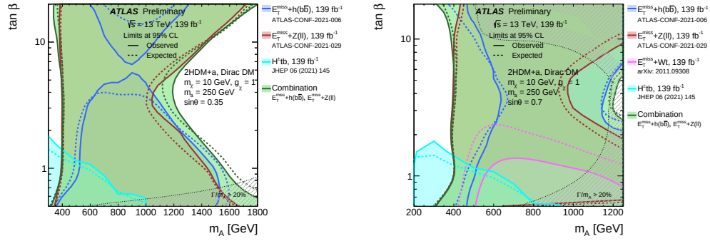
Figure 7.15: Observed (solid lines) and expected (dashed lines) exclusion regions at 95% CL in the m_A - \tan\beta plane with \sin\theta = 0.35 (left) and \sin\theta = 0.7 (right). The results are shown for several individual searches as well as the combination of the E_T^{\text{miss}} + Z(\ell^+\ell^-) and E_T^{\text{miss}} + h(b\bar{b}) searches. The dashed grey regions indicate the region where the width of the Higgs bosons exceeds 20% of its mass.
