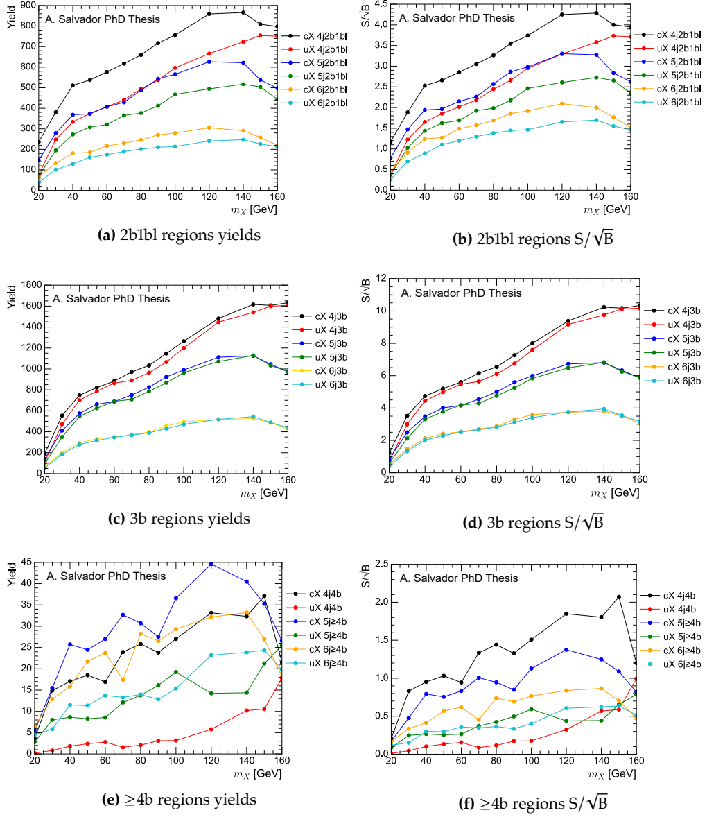
Figure 8.3: Signal yields (left) and S/\sqrt{B} (right) for the 2b+1bl (top), 3b (middle) and \geq 4b (bottom) regions after applying reweighting as a function of the mass of X for both t \rightarrow cX and t \rightarrow uX processes, assuming a branching fraction of 0.1% and an integrated luminosity of 139 \text{ fb}^{-1} .
