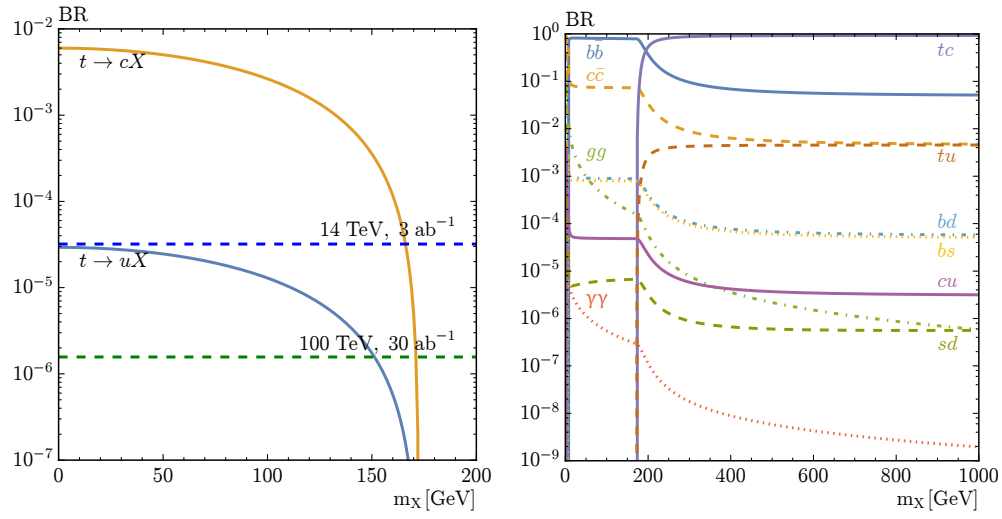
Figure 1.7: Branching fraction of the top-quark into a flavon and either u - or c -quarks (left) and flavon branching ratios for decays to quarks (right) as a function of the flavon mass, m_X [72]. The top-quark branching fraction are computed assuming a fixed VEV of 500 GeV.
