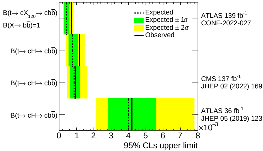
Figure 9.10: Expected and observed upper limits for the branching ratio of different t \rightarrow cX/cH results. The results shown include the t \rightarrow cX results for the 120 GeV mass hypothesis, the t \rightarrow cH result presented in this section and the t \rightarrow cH published result from FCNC searches performed by CMS using 137 \text{fb}^{-1} and by ATLAS using 36 \text{fb}^{-1} . The bands surrounding the expected limits show the 68% and 95% confidence intervals.
