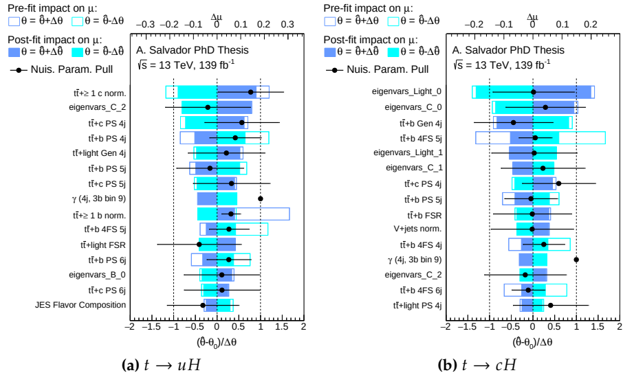
Figure 9.8: Ranking of the 15 systematic uncertainties with the largest impact on \mu for the fits performed with the SM Higgs hypothesis for the t \rightarrow uH (left) and t \rightarrow cH (right) processes. The empty (filled) rectangles correspond to the pre-fit (post-fit) impact on \mu . The black points represent the post-fit pulls of the nuisance parameters relative to the nominal values, \theta_0 . Statistical uncertainties ( \gamma ) are shown pulled with respect to 1.
