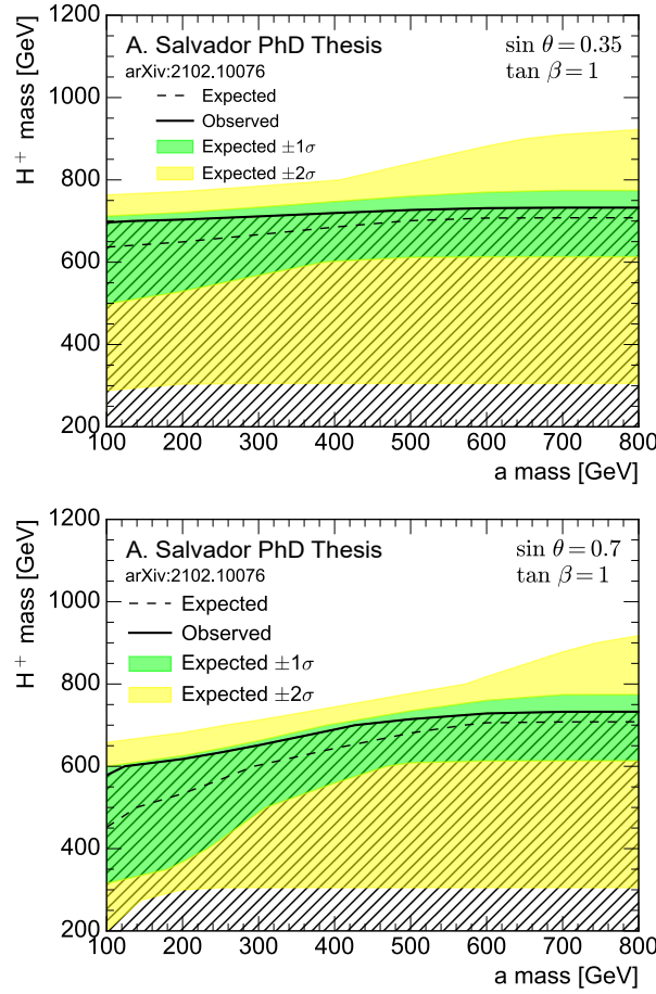
Figure 7.13: Observed and expected exclusion plots in the H^+ - a mass plane of the production of H^+ \rightarrow tb for \sin \theta = 0.35 (0.7) at the top (bottom).
