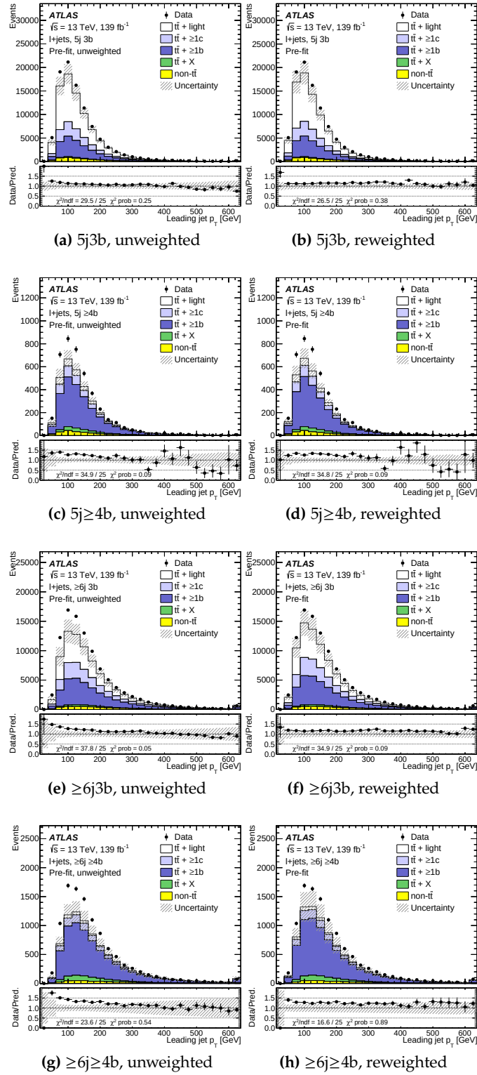
Figure 6.7: Comparison of the data and predicted leading jet p_T distributions before (left) and after (right) the reweighting is applied. The uncertainty bands include both statistical and systematic uncertainties, except for the cross-sections of the t\bar{t} + \geq 1b and t\bar{t} + \geq 1c backgrounds. The lower panels show the ratio of the data to the total prediction. The hatched bands show the uncertainties before the fit to the data, which are dominated by systematic uncertainties. The \chi^2 per number of degrees of freedom ( \chi^2/\text{ndf} ) and the \chi^2 probability are also shown. Statistical uncertainties on MC predictions and data are uncorrelated across bins, while systematic uncertainties on the predictions are correlated.
