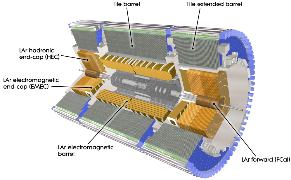
Figure 2.7: Schematic overview of the ATLAS calorimeter system [84].
