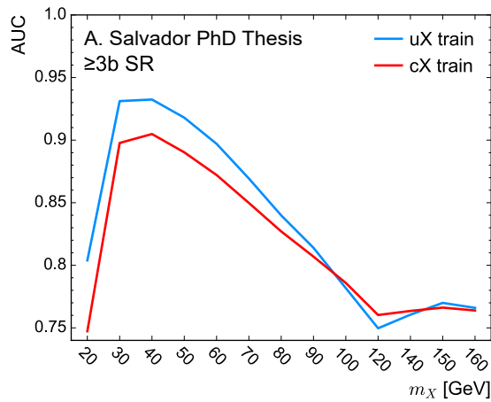
Figure 8.9: Comparison of the performance, measured as the area under the ROC curve as a function of the mass of the scalar X for the \geq 3b regions. The NNs are trained using either the t \rightarrow uX (blue) or t \rightarrow cX (red) signal samples, and evaluated accordingly.
