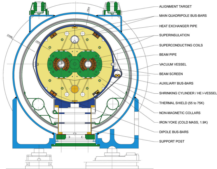
Figure 2.2: Diagram showing the cross-section of an LHC dipole magnet [76].
