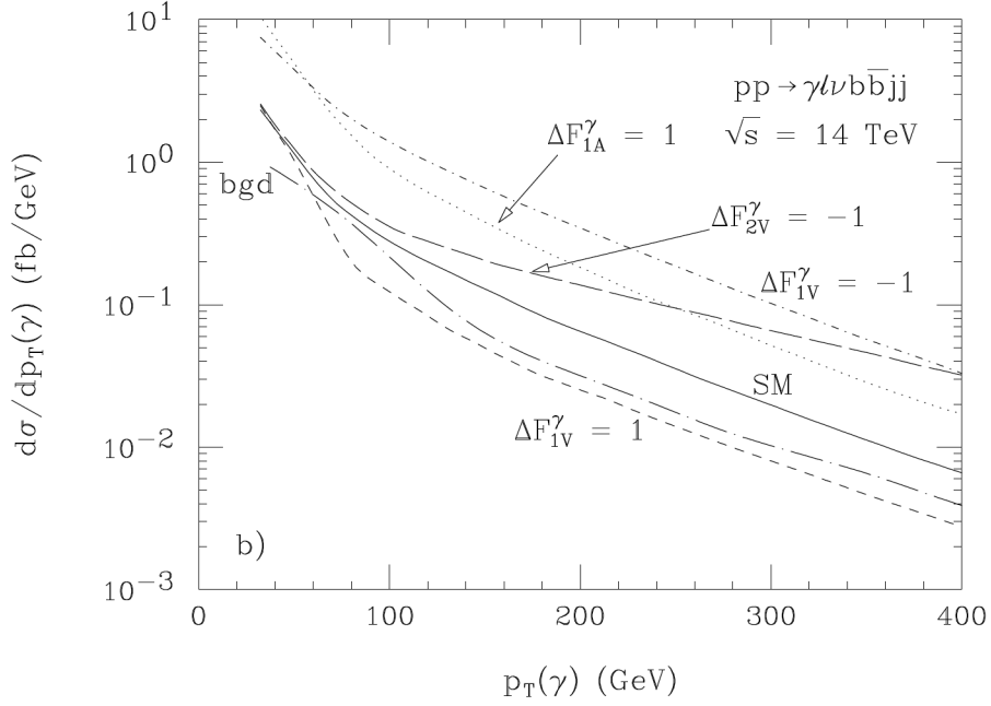
Figure 2.9.: Differential cross-section of t\bar{t}\gamma production in the semileptonic channel as a function of the photon transverse momentum for at the LHC at \sqrt{s}=14 TeV [39]. The continuous curve labelled as SM corresponds to the Standard Model prediction of the t\bar{t}\gamma cross-section, while the dotted and dashed curves correspond to the t\bar{t}\gamma cross-section with anomalous t\gamma couplings. For each curve only, one coupling is allowed to deviate and the labels \Delta F_{1(2),V}^\gamma(\Delta F_{1(2),A}^\gamma) indicate the differences with respect to the SM of the vector (axial-vector) form-factors F_{1(2),V}^\gamma(F_{1(2),A}^\gamma) .
