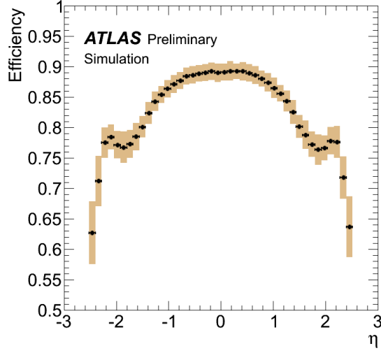
Figure 7.5.: Track reconstruction efficiency as a function of \eta obtained using the GEO-20 detector model, for tracks with p_T > 500 MeV. The systematic uncertainties were determined by comparison to a model with +10% additional material in the whole ID [88].
