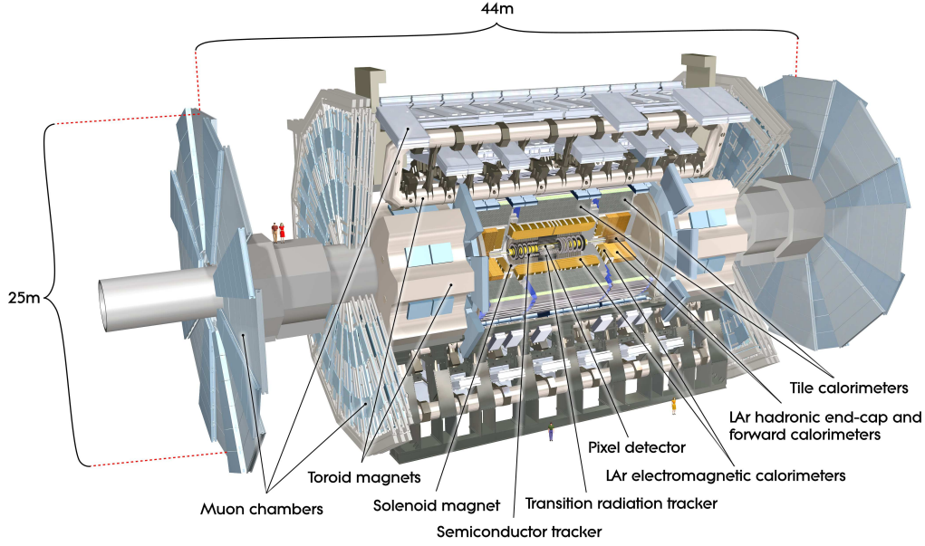
Figure 3.5.: Cut-away view of the ATLAS detector. The dimensions of the detector are 25 m in height and 44 m in length. The overall weight of the detector is approximately 7000 tons. [10]
