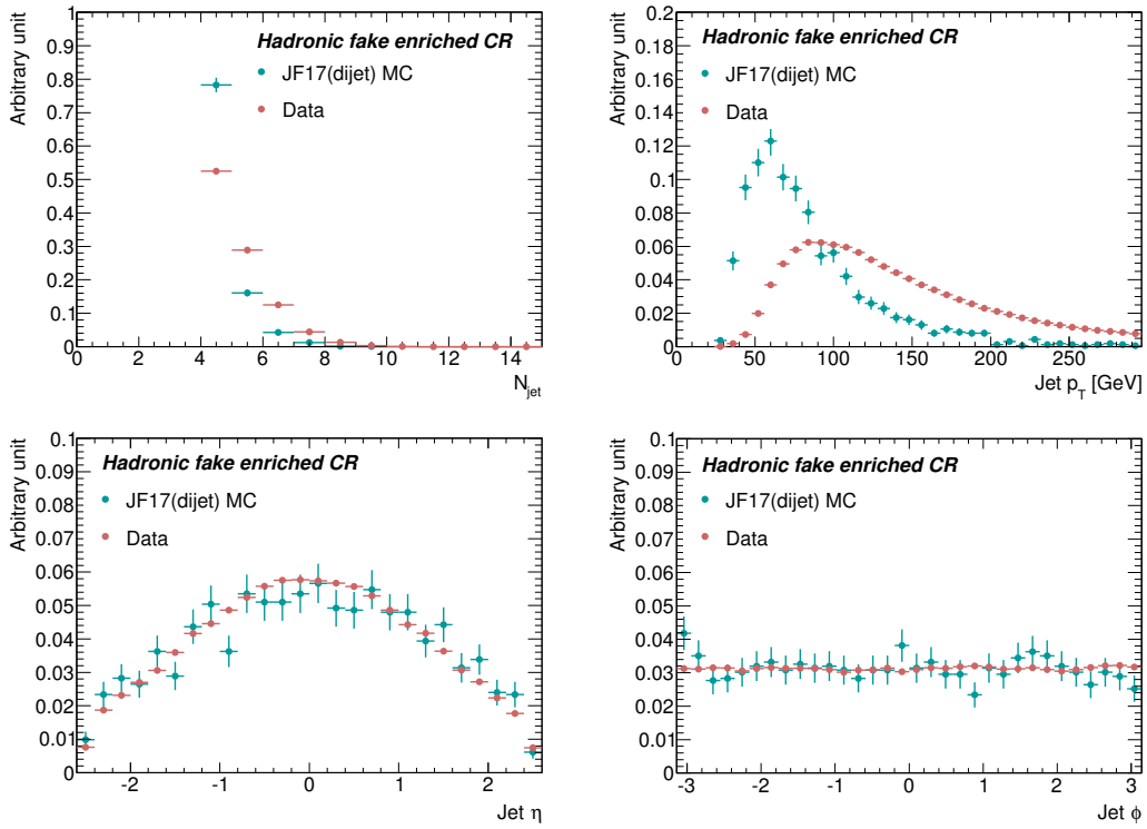
Figure 7.9.: Comparison of data and JF17 di-jet MC sample in terms of jet kinematics. It can be seen that the MC does not describe the data well. The sample is therefore not suitable to be used for evaluating the systematic uncertainty for prompt photon contamination.
