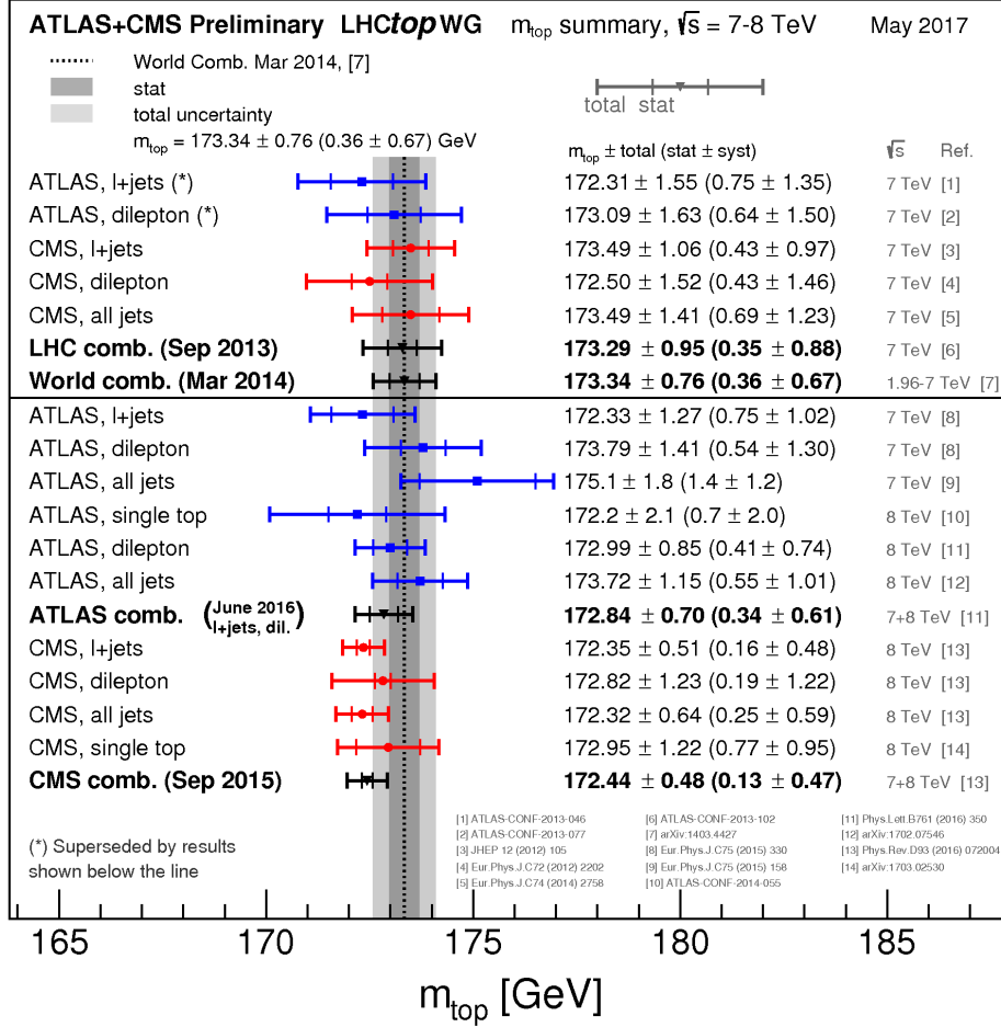
Figure 2.6.: Summary of the ATLAS and CMS direct m_{\text{top}} measurements. The results are compared with the LHC and Tevatron+LHC m_{\text{top}} combinations. For each measurement, the statistical uncertainty, the jet scale factor (JSF) and b-jet scale factor (bJSF) contributions (when applicable) as well as the sum of the remaining uncertainties are reported separately. The JSF, bJSF contributions are statistical in nature and apply to analyses performing in-situ (top quark pair base) jet energy calibration procedures. The results below the line are results produced after the LHC and Tevatron+LHC combinations were performed. [22]
