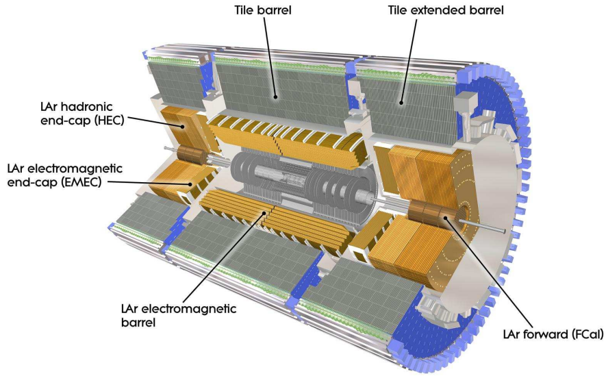
Figure 3.7.: An overview of the calorimetry at the ATLAS detector. [10]
