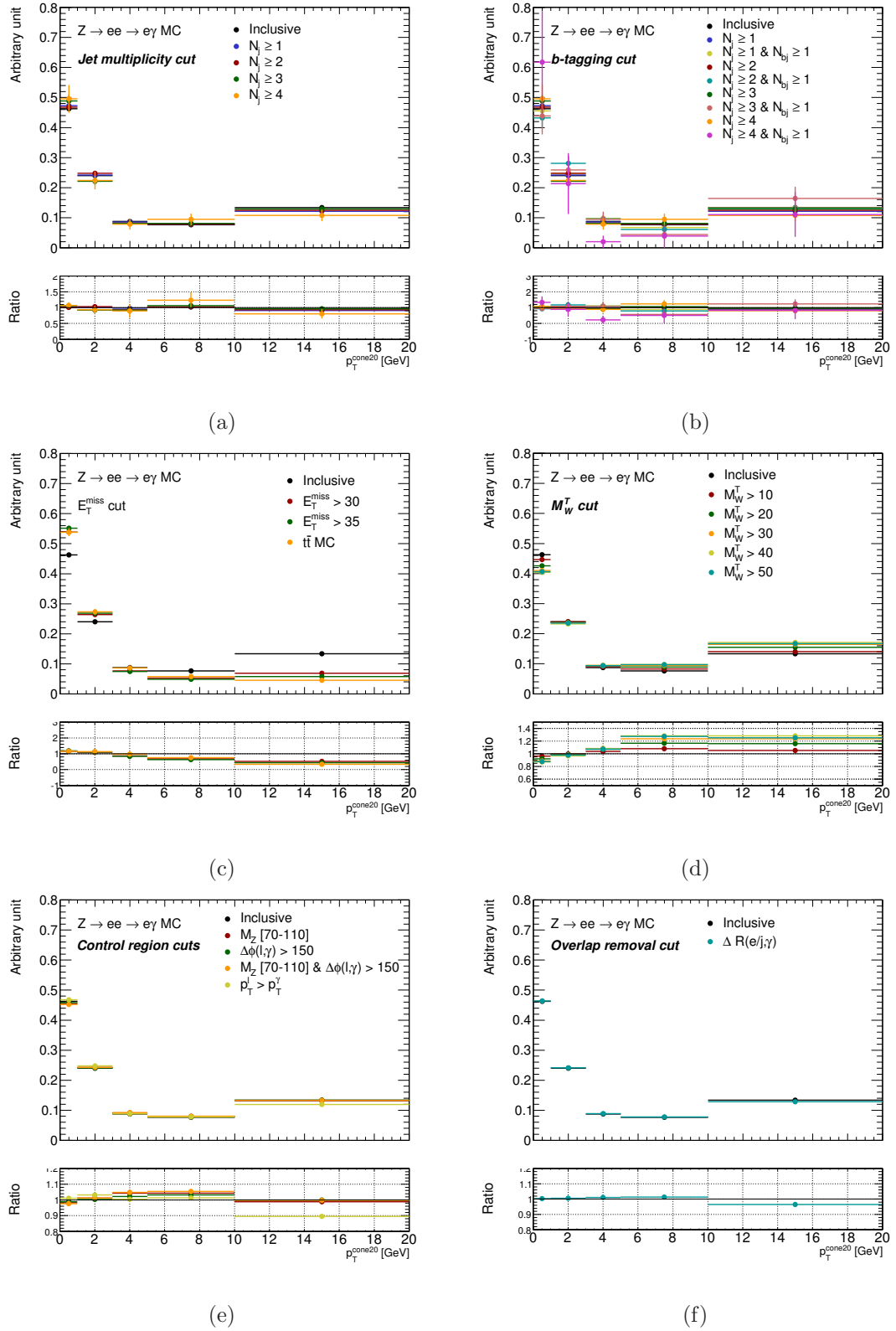
Figure 7.21.: Photon isolation distributions where the effects of several SR and CR cuts are investigated: (a) is the check for jet multiplicity, (b) for b -tagging, (c) for E_T^{\text{miss}} , (d) for M_W^T , (e) for control region cuts and (f) for the overlap removal between the photon and other objects.
