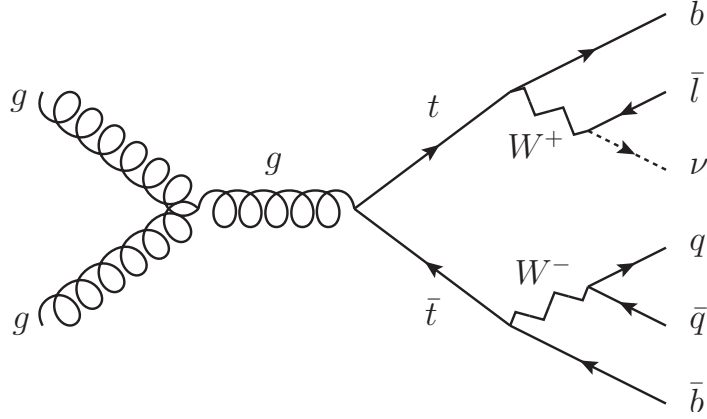
Figure 2.4.: A representative feynman diagram for the semileptonic decay channel of a t\bar{t} pair.
