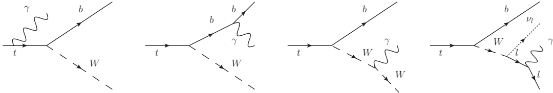
Figure 2.8.: Representative Feynman diagrams for radiative top-quark decay.
