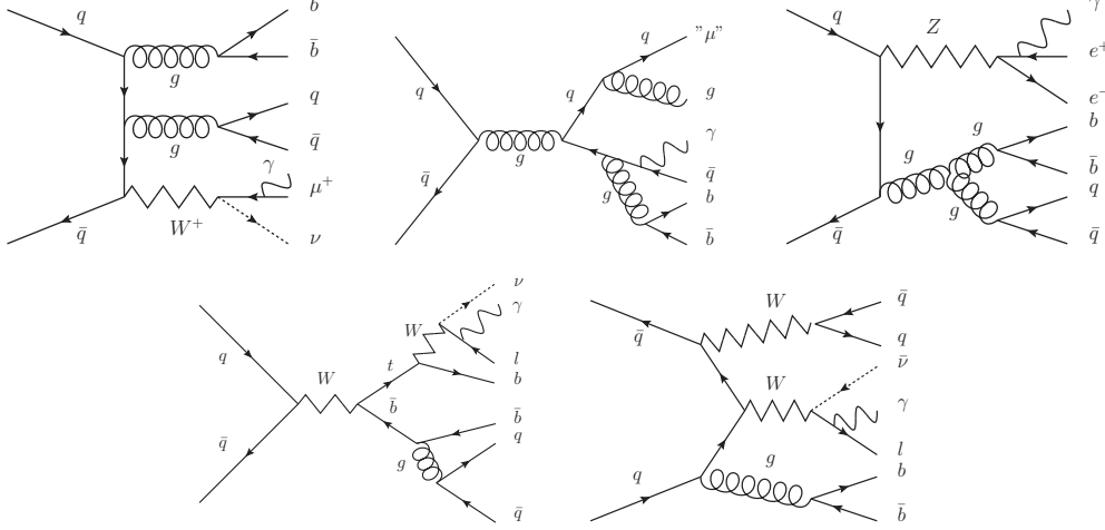
Figure 7.24.: Example representative Feynman diagrams for the background processes with a prompt photon.
