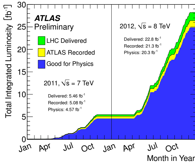
Figure 3.3.: Cumulative luminosity versus time delivered (green), recorded by ATLAS (yellow), and certified to be good quality data (blue) during stable beams and for pp collisions at 7 and 8 TeV centre-of-mass energy in 2011 and 2012. [57]
