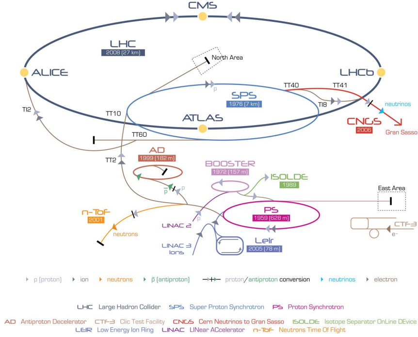
Figure 3.2.: The CERN accelerator complex, showing all particle accelerators situated at CERN. The LHC accelerator chain comprises (with increasing energy): Linac2 → Proton Synchrotron Booster → Proton Synchrotron Super Proton → Synchrotron LHC [48].
