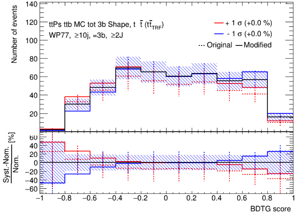
Figure 6.17: Pre-fit uncertainties associated to t\bar{t} parton shower in the 10j i3b e2J i sub-region without the smoothing. Red points refer to the original variation, with associated statistical error. The red solid line is obtained by smoothing the uncertainty consistently with the statistical uncertainty of the variation. The blue solid line is obtained by symmetrising the red one. Red and blue solid lines give the uncertainty on the prediction.
