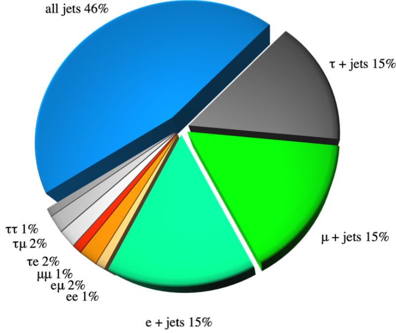
Figure 1.5: Top quark pair branching fractions.
