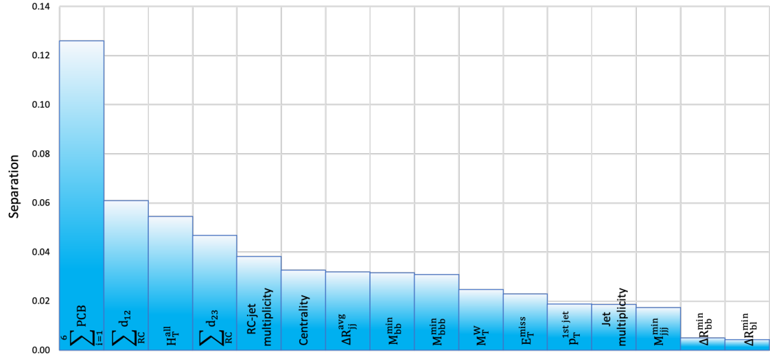
Figure C.11: Ranking of input variables in terms of separation in the 10ji3be region for the training done on odd events according to TMVA.
