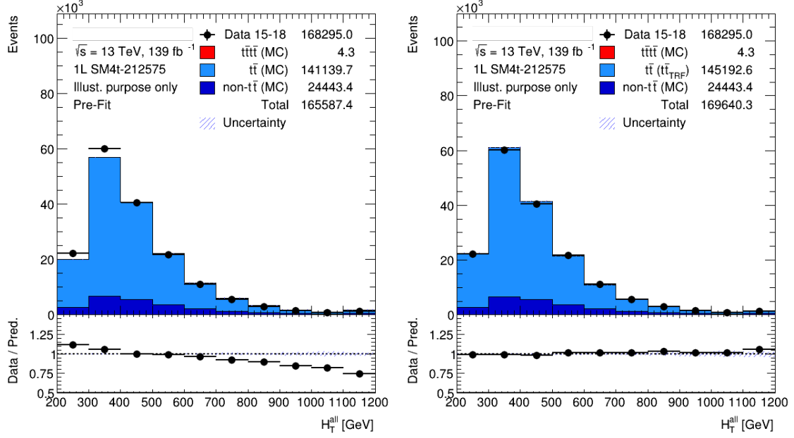
Figure 4.4: Illustrative example of the effect of the TRF_{t\bar{t}} method in the region 5je3be . On the left, the light-blue background is the simple MC prediction for t\bar{t} +jets. On the right, the same background is estimated using the TRF_{t\bar{t}} method, resulting in a much better agreement with the data.
