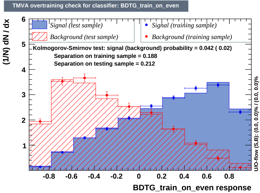
Figure 5.6: Training response for the BDT in the 10ji4bi region for the training done on even events.
