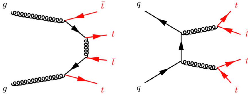
Figure 1.6: Leading order Feynman diagrams for the t\bar{t}t\bar{t} production in case of gg fusion and q\bar{q} annihilation.
