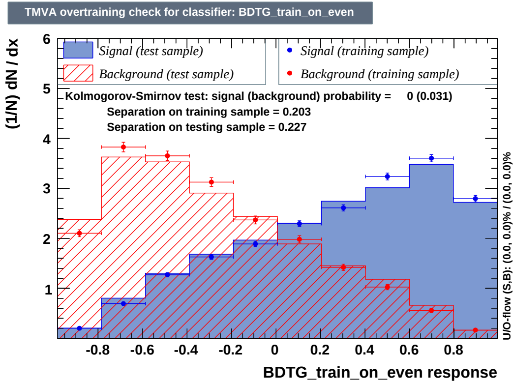
Figure C.2: Training response for the BDT in the 9je3be region for the training done on even events.
