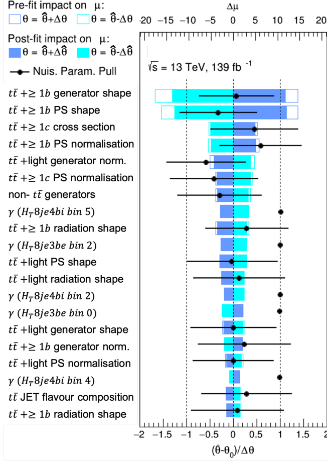
Figure 6.7: Ranking plot from the fit to data in control regions under the signal-plus-background hypothesis. The \gamma parameters refer to statistical uncertainty on the background model and are assumed to be Poisson-distributed NPs.
