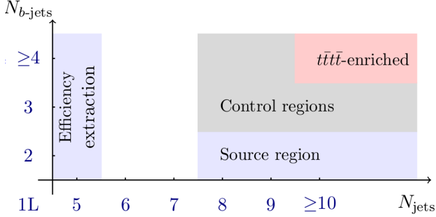
Figure 3.2: Schematic view of the regions definition.
