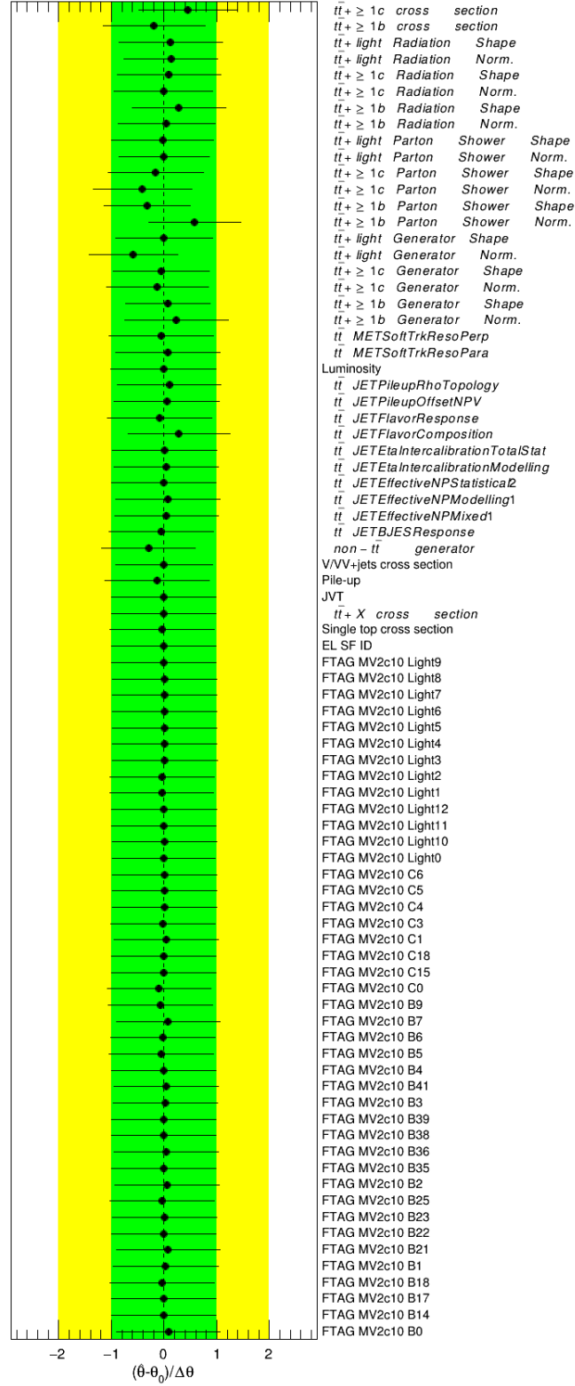
Figure 6.6: Fitted nuisance parameters under the signal-plus-background hypothesis in the control regions only.
