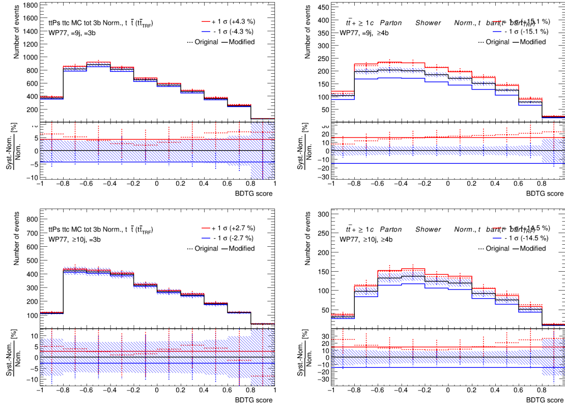
Figure 6.26: Pre-fit uncertainties associated to the parton shower generator on t\bar{t} + \geq 1c normalisation in the signal regions. Red points refer to the original variation, with associated statistical error. The red solid line is obtained by smoothing the uncertainty consistently with the statistical uncertainty of the variation. The blue solid line is obtained by symmetrising the red one. Red and blue solid lines give the uncertainty on the prediction.
