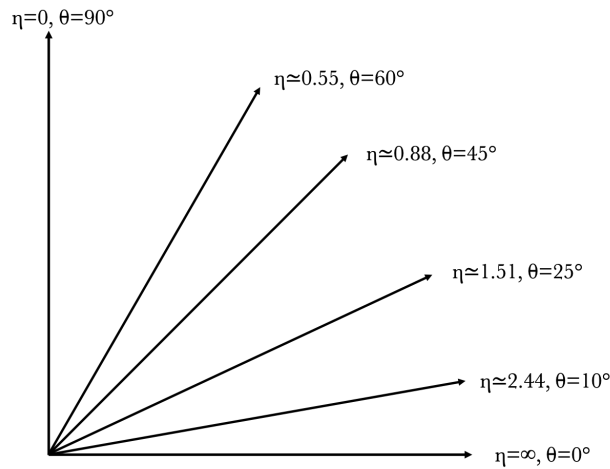
Figure 2.4: Variation of the pseudorapidity as a function of \theta .
