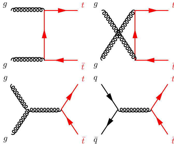
Figure 1.3: Leading order Feynman diagrams for t\bar{t} production in case of gg fusion and q\bar{q} annihilation.
