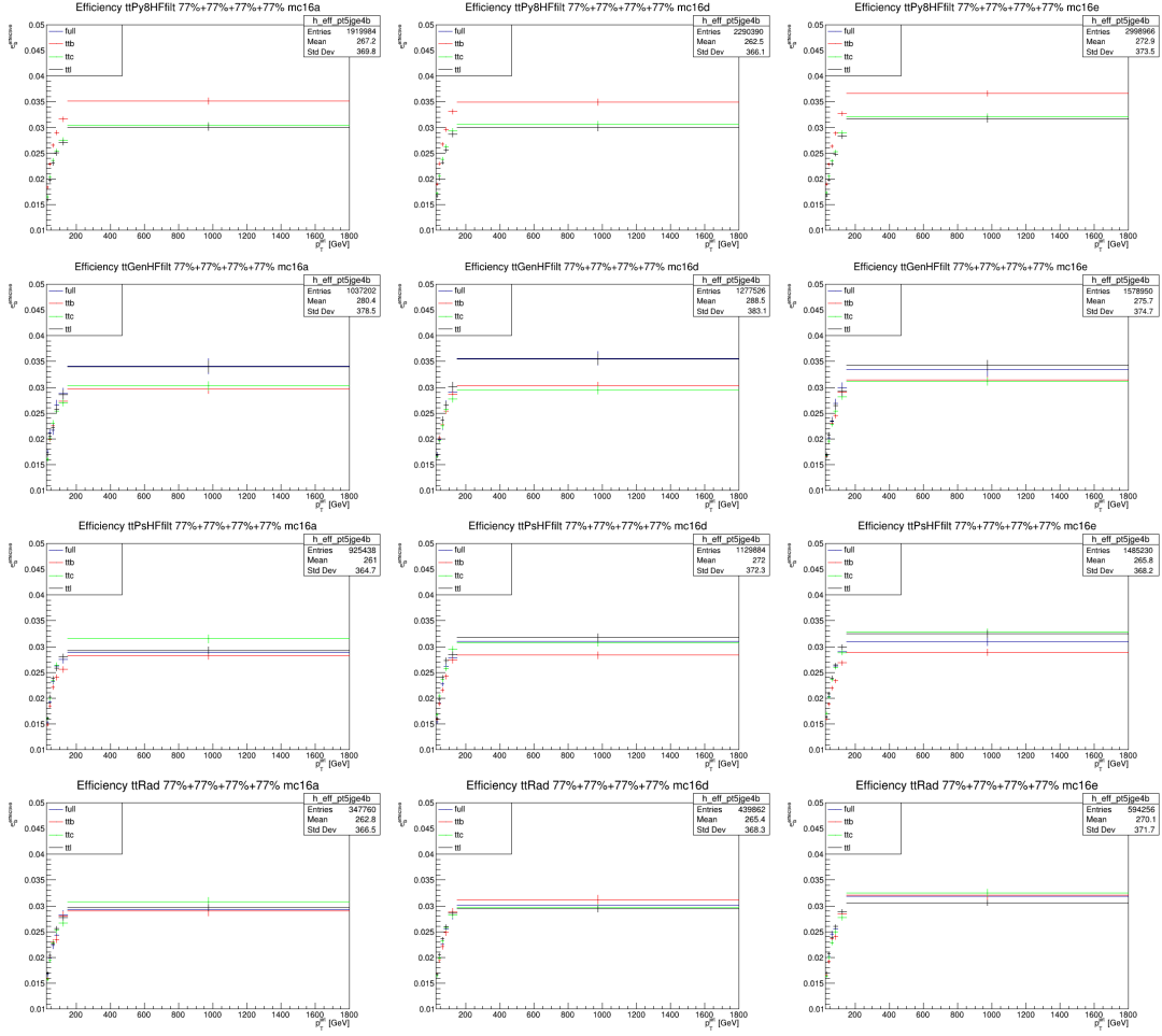
Figure B.2: Efficiencies for TRF_{t\bar{t}} method for \geq 4b regions as a function of jet p_T .
