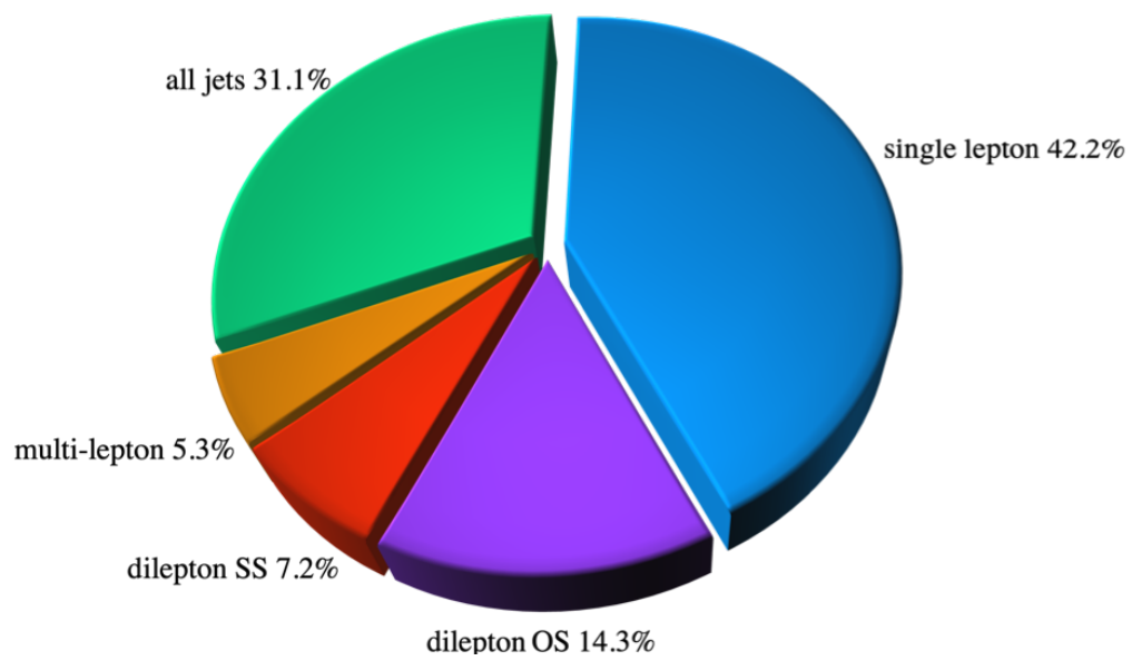
Figure 1.7: Branching ratio for the decays of t\bar{t}t\bar{t} .
