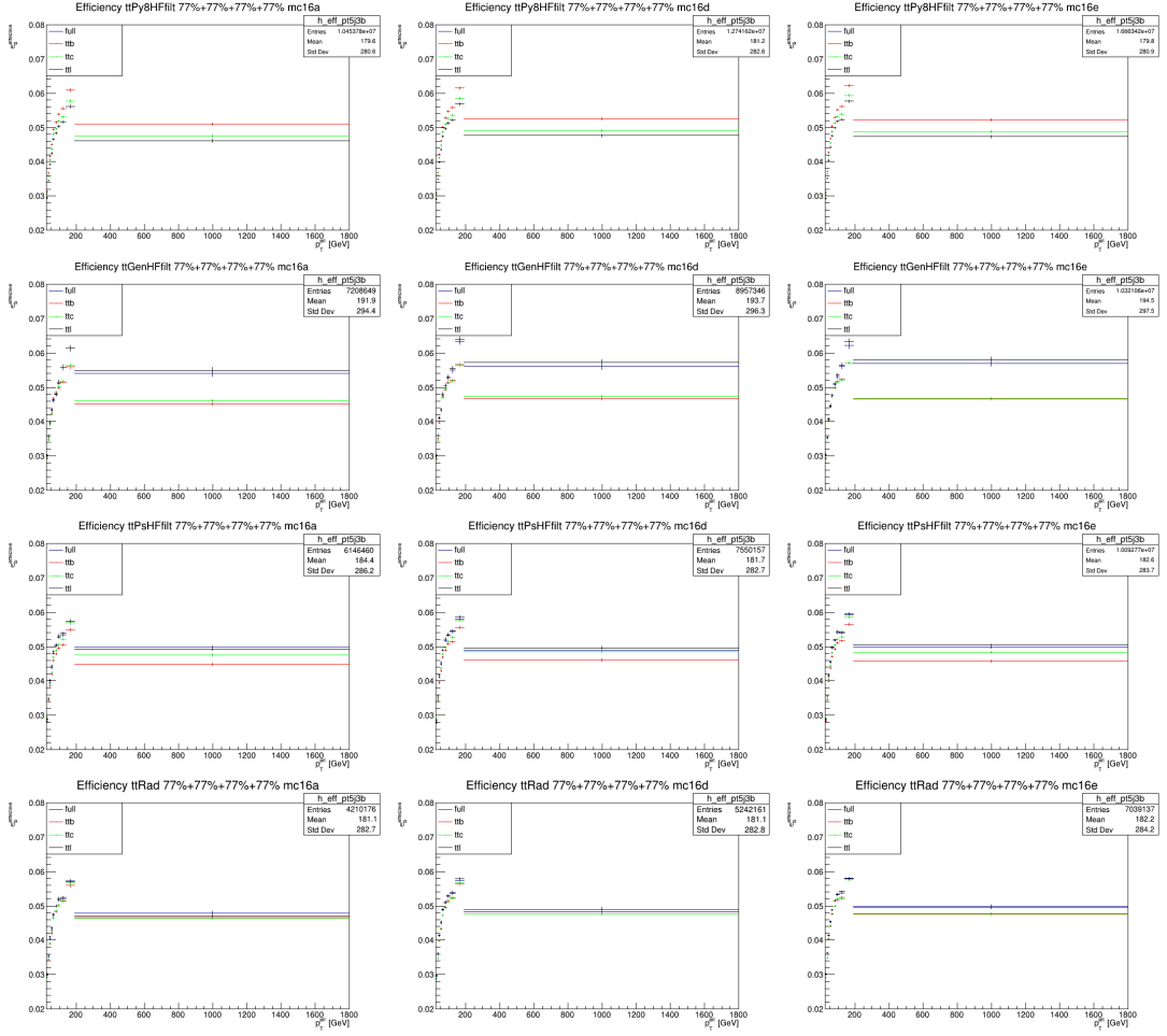
Figure B.1: Efficiencies for TRF_{t\bar{t}} method for 3b regions as a function of jet p_T .
