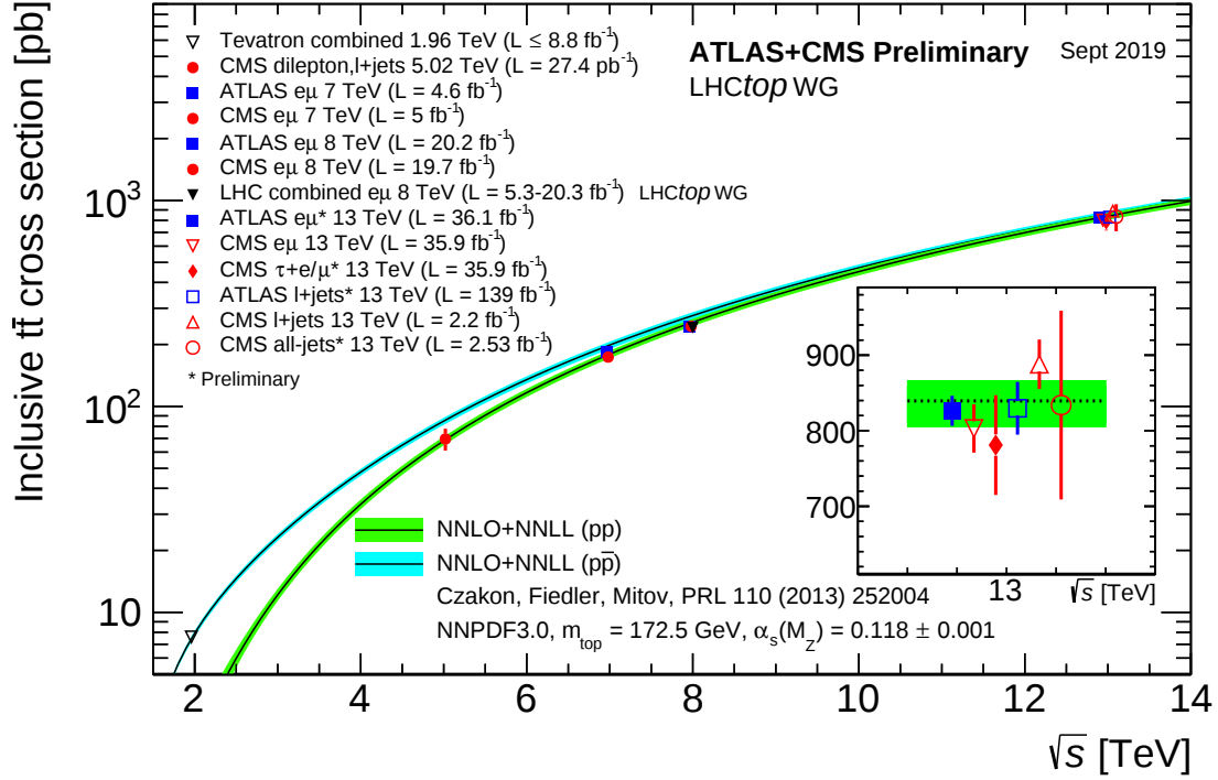
Figure 1.4: Summary of LHC and Tevatron measurements of the t\bar{t} production cross section as a function of the centre of mass energy compared to theoretical calculations [17].
