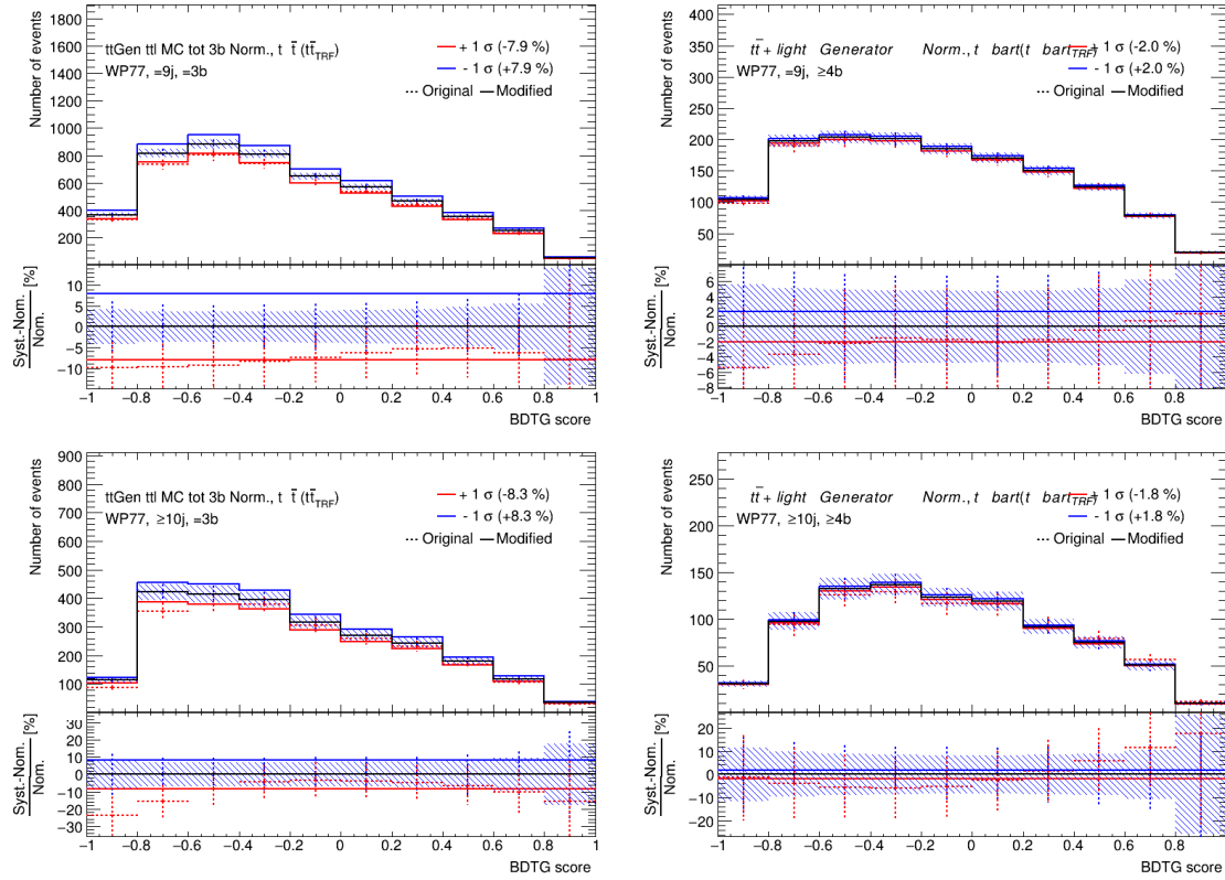
Figure 6.30: Pre-fit uncertainties associated to the matrix element generator on t\bar{t} +light normalisation in the signal regions. Red points refer to the original variation, with associated statistical error. The red solid line is obtained by smoothing the uncertainty consistently with the statistical uncertainty of the variation. The blue solid line is obtained by symmetrising the red one. Red and blue solid lines give the uncertainty on the prediction.
