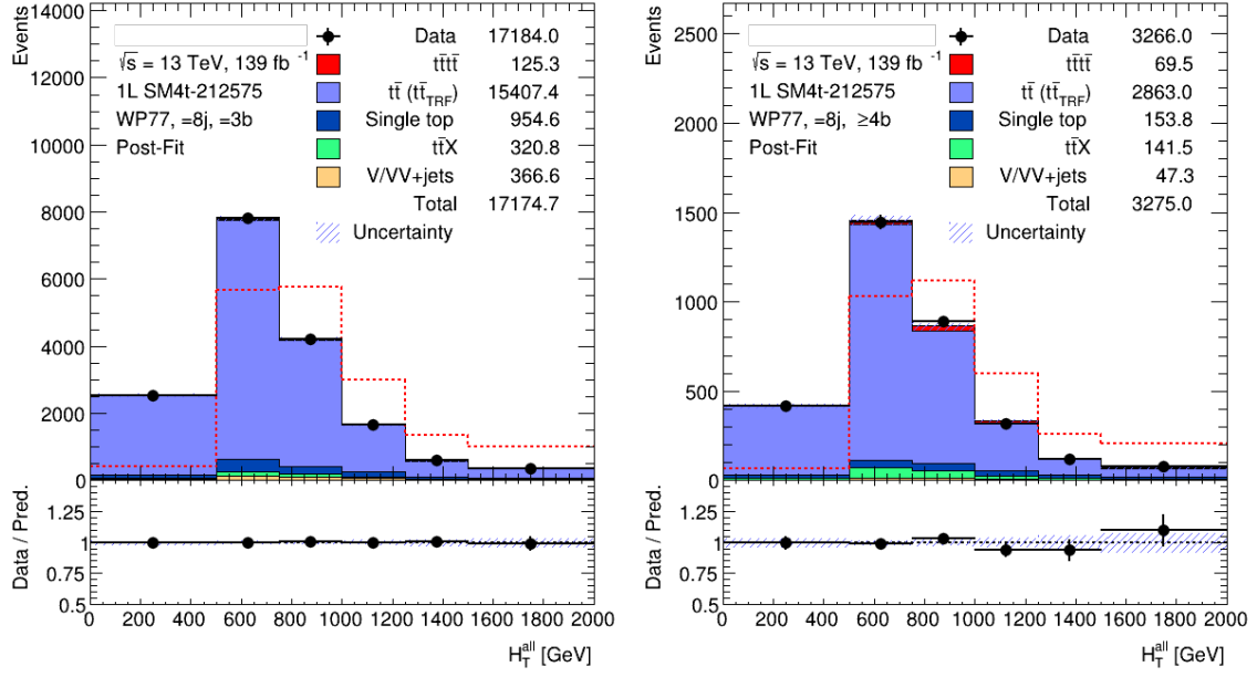
Figure 6.4: Comparison between data and prediction of the H_T distributions in the control regions after the fit to data. The t\bar{t} +jet background is estimated through the data-driven method, with the MC-correction applied. The hashed area represents the combination of the statistical and systematic uncertainties on the background prediction. The last bin in all figures contains the overflow.
