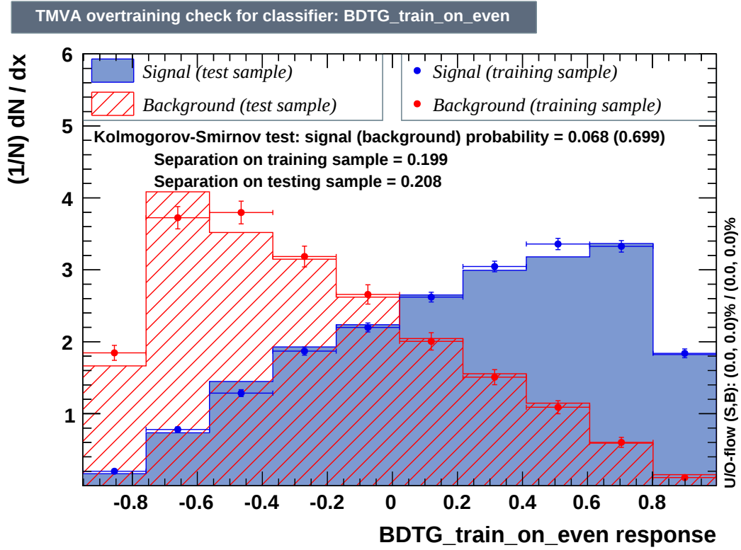
Figure C.10: Training response for the BDT in the 10ji3be region for the training done on even events.
