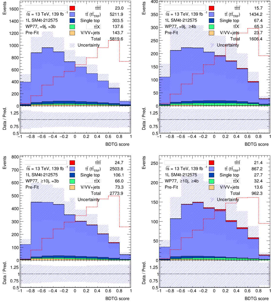
Figure 6.9: Comparison between Asimov data set and prediction of the BDT distributions in the signal regions prior to the fit to data. The t\bar{t} +jet background is estimated through the data-driven method, with the MC-correction applied. The hashed area represents the combination of the statistical and systematic uncertainties on the background prediction.
