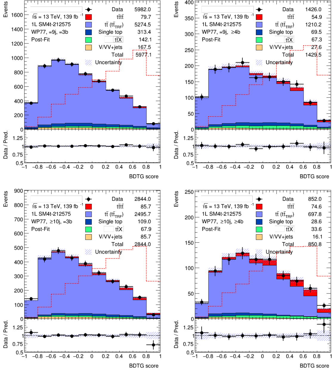
Figure 6.20: Comparison between data and prediction of the BDT distributions in the signal regions after the fit to data. The t\bar{t} +jet background is estimated through the data-driven method, with the MC-correction applied. The hashed area represents the combination of the statistical and systematic uncertainties on the background prediction.
