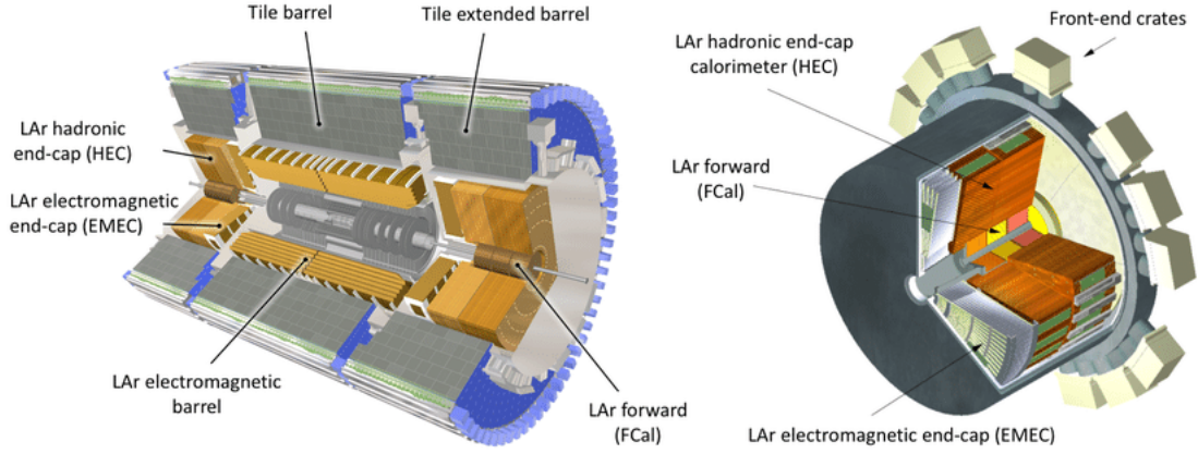
Figure 2.8: Schematic view of the ATLAS calorimeter system [23].
