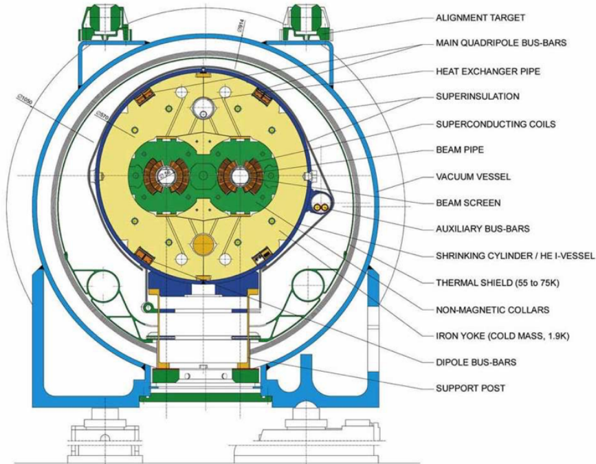
Figure 2.2: Section of one of the magnetic dipoles used to bend and stabilise the beam orbit [22].
