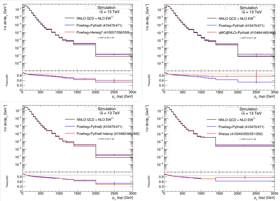
Figure A.3: Normalised t\bar{t} differential cross section as a function of top quark p_T for different NLO t\bar{t} simulation samples, compared to the nominal MC sample and the NNLO QCD + NLO EW prediction.
