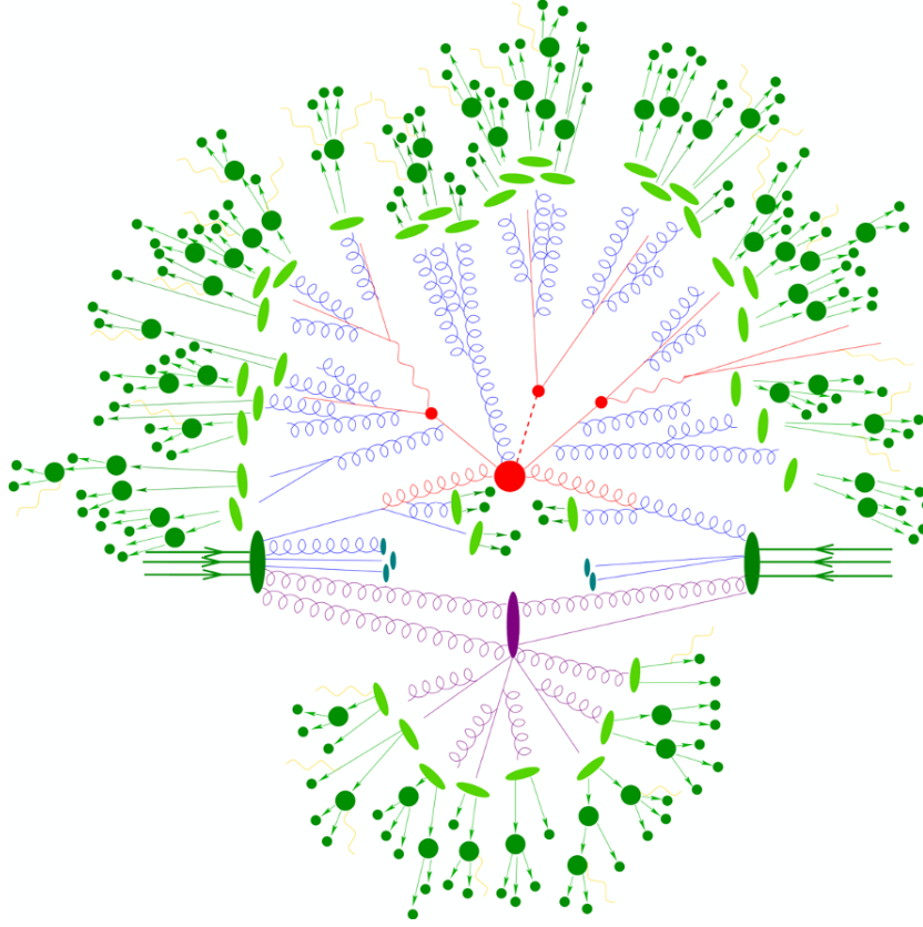
Figure 4.1: Schematic representation of an event as produced by a MC simulation [48].
