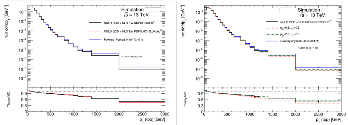
Figure A.2: Normalised t\bar{t} differential cross section as a function of top quark p_T in case of PDF variations (on the left) and scale variations (on the right) of the NNLO QCD + NLO EW prediction compared to the nominal NLO t\bar{t} simulation sample (POWHEG + PYTHIA 8).
