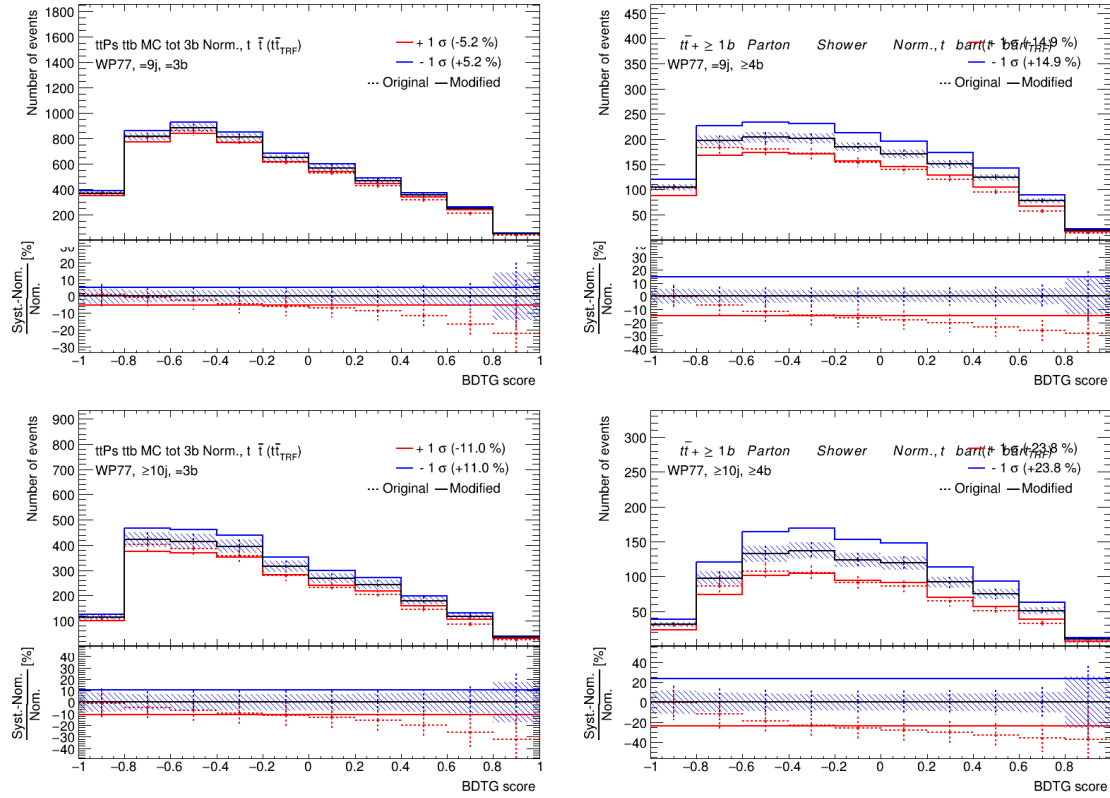
Figure 6.28: Pre-fit uncertainties associated to the parton shower generator on t\bar{t} + \geq 1b normalisation in the signal regions. Red points refer to the original variation, with associated statistical error. The red solid line is obtained by smoothing the uncertainty consistently with the statistical uncertainty of the variation. The blue solid line is obtained by symmetrising the red one. Red and blue solid lines give the uncertainty on the prediction.
