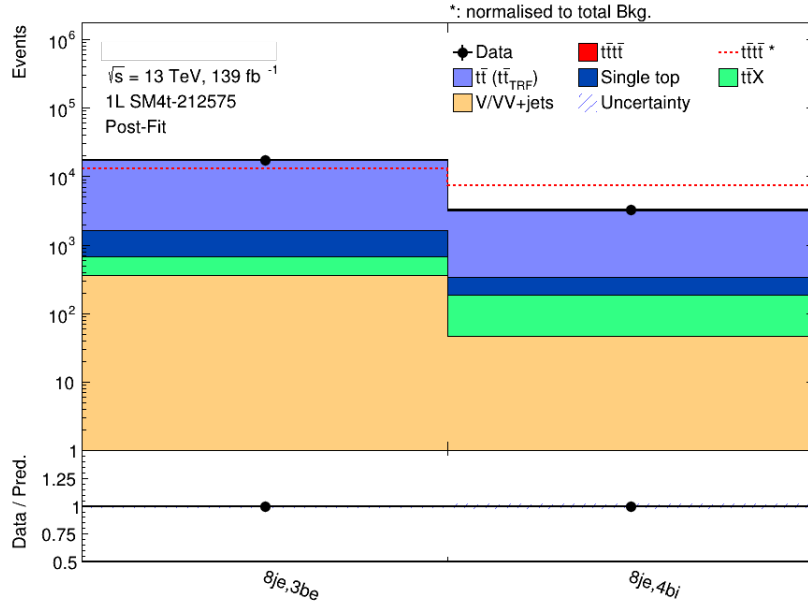
Figure 6.5: Comparison of prediction to data in control regions after the fit to data. The t\bar{t} +jet background is estimated through the data-driven method. The hashed area represents the combination of the statistical and systematic uncertainties on the background prediction. The bottom panel displays the ratio of data to the total prediction.
