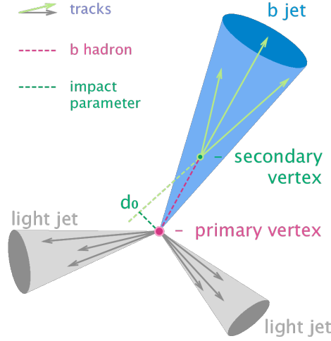
Figure 3.1: Schematic view of a b -hadron decay inside a jet coming from a secondary vertex.
