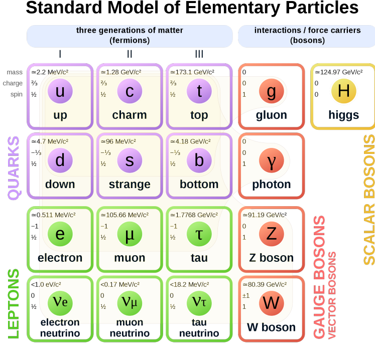
Figure 1.1: Scheme of the elementary particles described in the SM.
