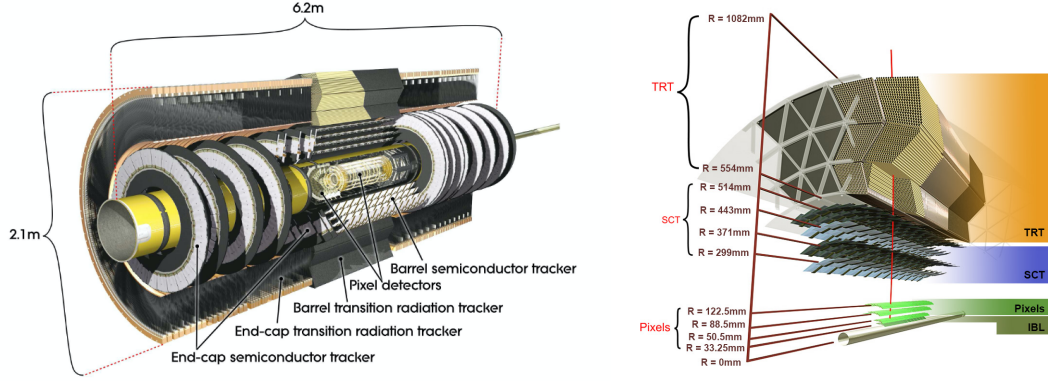
Figure 2.7: Schematic view of the ATLAS Inner Detector [23], [32].
