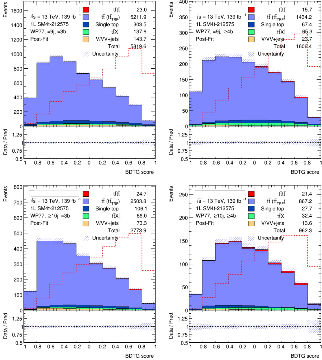
Figure 6.10: Comparison between Asimov data set and prediction of the BDT distributions in the signal regions after the fit to data. The t\bar{t} +jet background is estimated through the data-driven method, with the MC-correction applied. The hashed area represents the combination of the statistical and systematic uncertainties on the background prediction.
