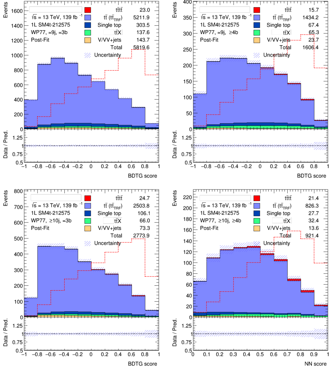
Figure D.2: Comparison between data and prediction of the BDT/NN distributions in the signal regions after the fit to data. The t\bar{t} +jet background is estimated through the data-driven method, with the MC-correction applied. The hashed area represents the combination of the statistical and systematic uncertainties on the background prediction.
