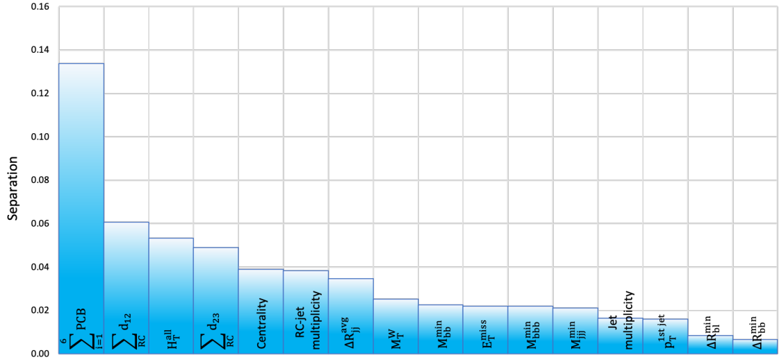
Figure 5.5: Ranking of input variables in terms of separation in the 10ji4bi region for the training done on even events according to TMVA.
