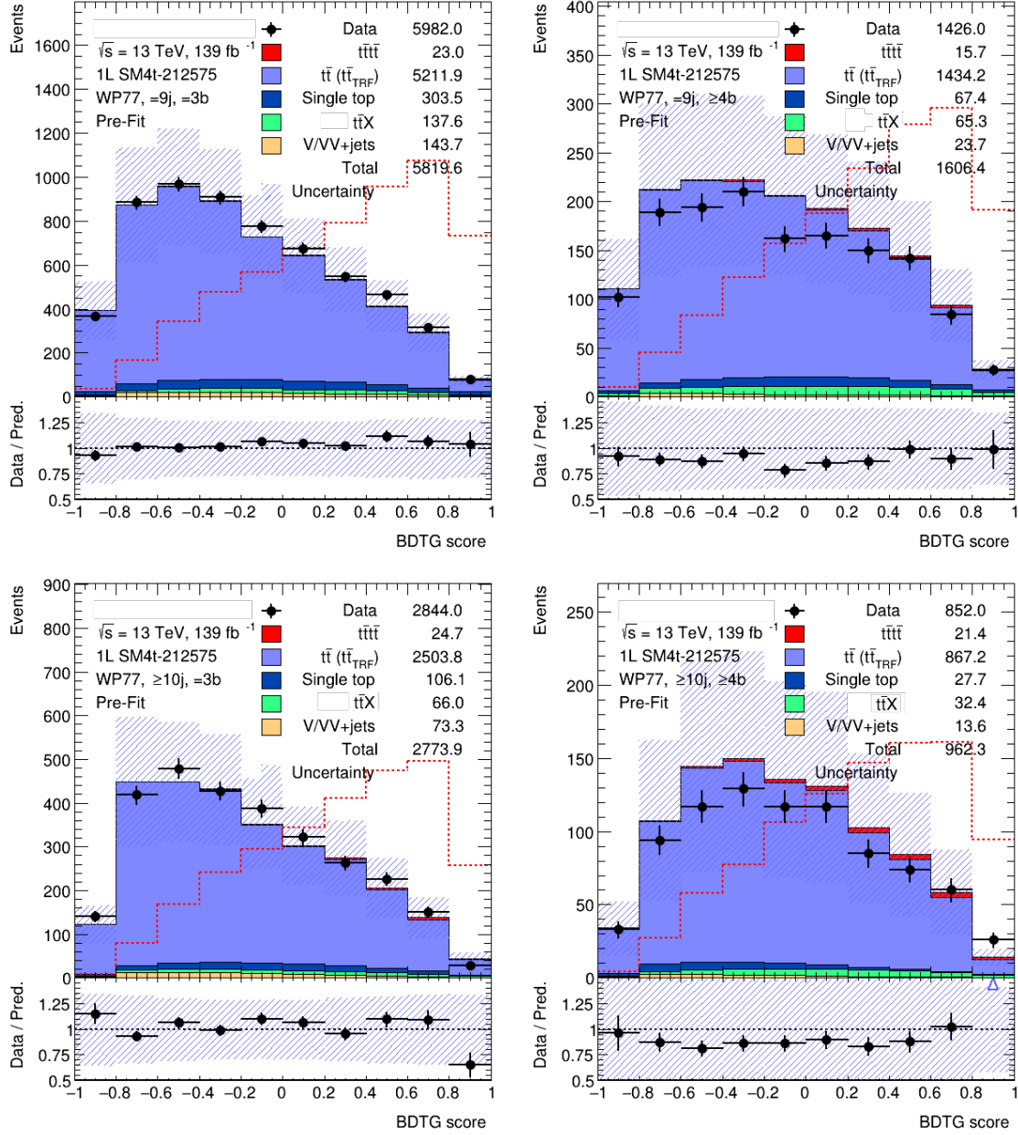
Figure 6.19: Comparison between data and prediction of the BDT distributions in the signal regions prior to the fit to data. The t\bar{t} +jet background is estimated through the data-driven method, with the MC-correction applied. The hashed area represents the combination of the statistical and systematic uncertainties on the background prediction.
