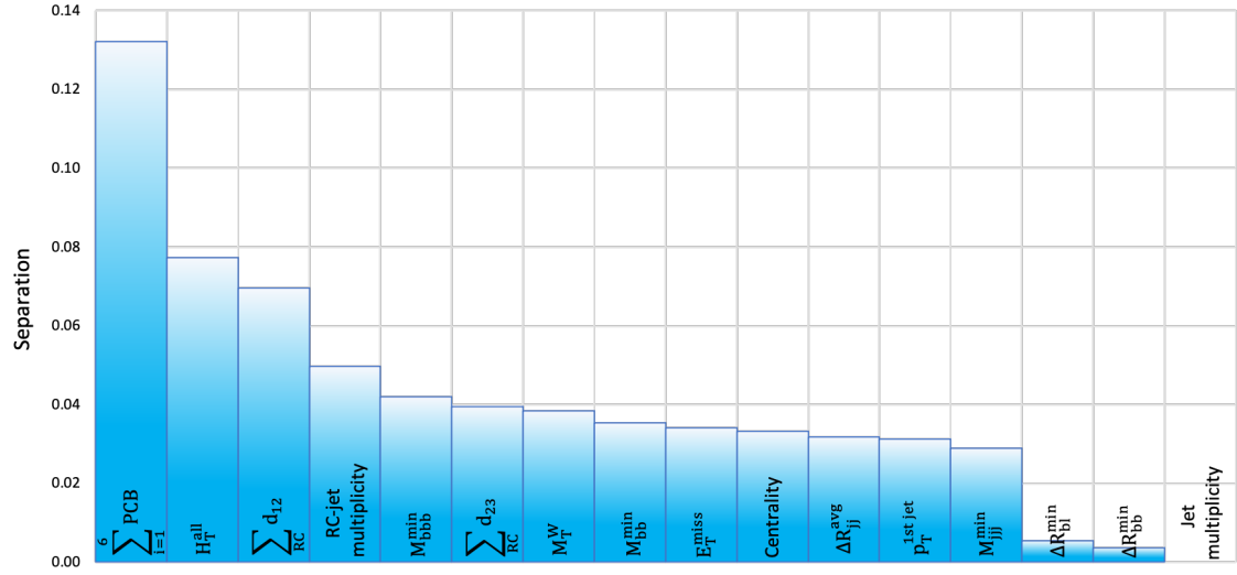
Figure C.1: Ranking of input variables in terms of separation in the 9je3be region for the training done on even events according to TMVA.
