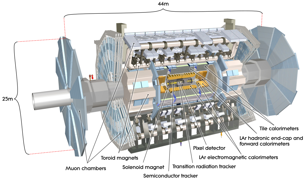
Figure 2.5: Digital view of the ATLAS detector with the indications of the various sub-detectors [23].
