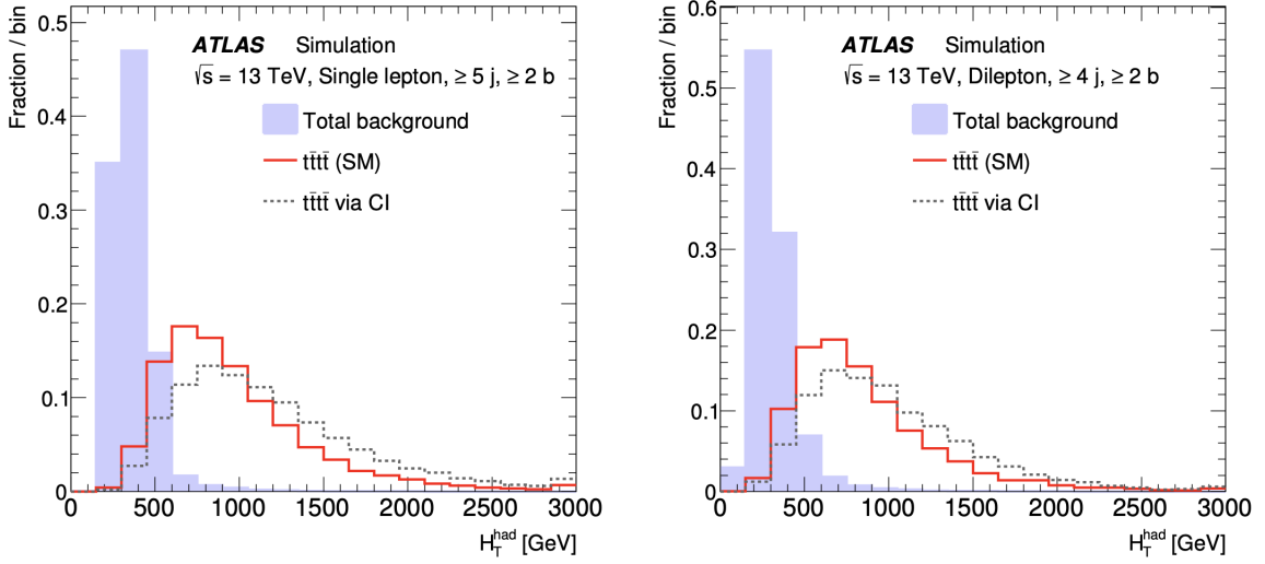
Figure 5.1: Examples of the H_T distributions in the first round of the analysis, after preselection, for the total predicted background with the t\bar{t} +jets background estimated via MC simulation (shaded histogram) and signals for the 1L ( 5ji2bi region) and the 2LOS ( 4ji2bi region) channels. The signals shown correspond to t\bar{t}t\bar{t} production with SM kinematics (solid) and t\bar{t}t\bar{t} production involving a four-fermion contact interaction (dashed). The distributions are normalised to unit area [20].
