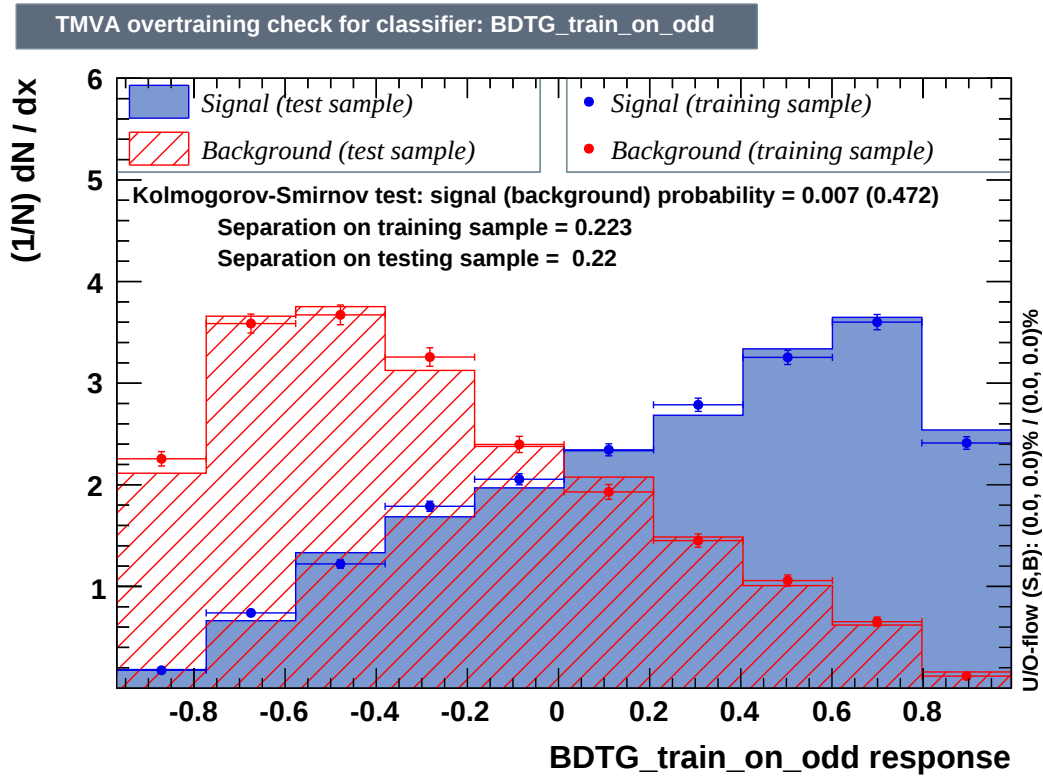
Figure C.4: Training response for the BDT in the 9je3be region for the training done on odd events.
