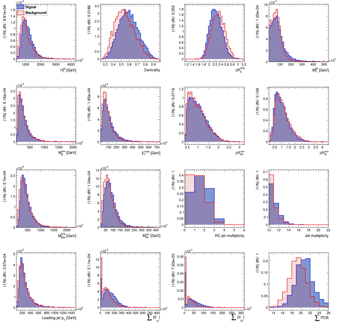
Figure 5.4: Separation of the variables used for the training in the 10ji4bi region.
