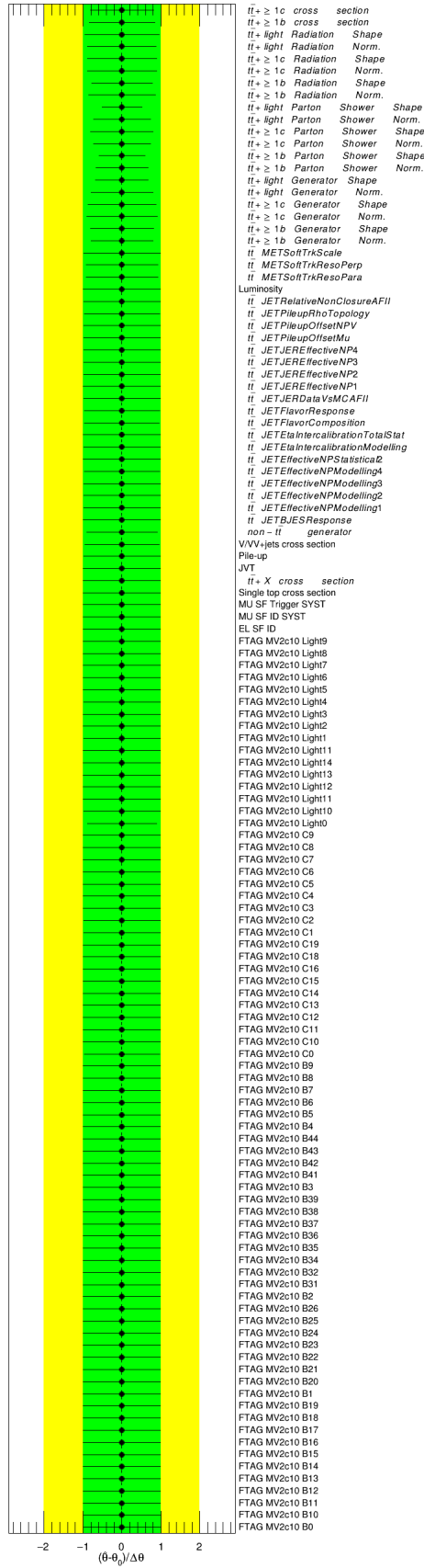
Figure D.3: Fitted nuisance parameters on data under the signal-plus-background hypothesis in the signal regions.
