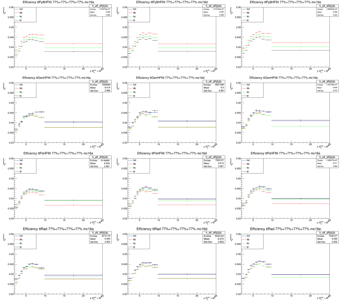
Figure B.3: Efficiencies for TRF_{t\bar{t}} method for 3b regions as a function of \Delta R_{j1}^{min} \times N_j .
