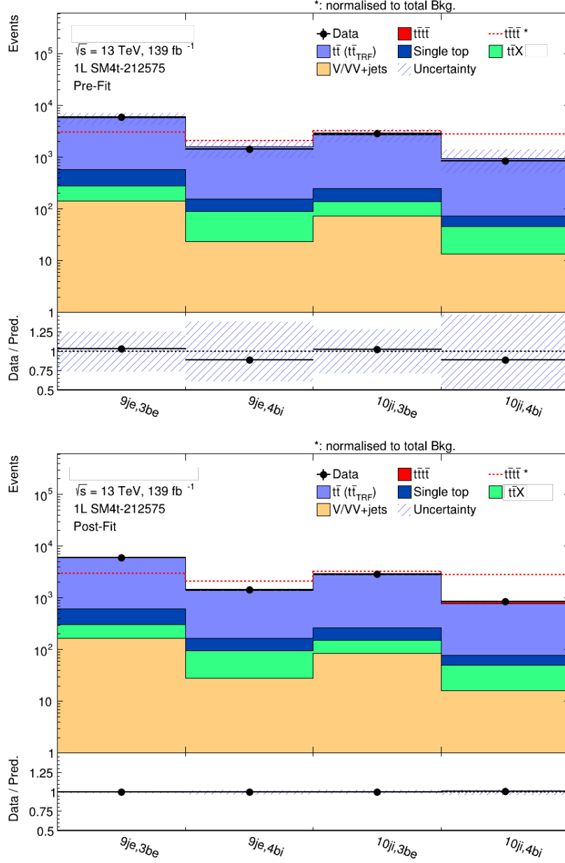
Figure 6.18: Comparison of prediction to data in the four signal regions prior and after the fit to data. The t\bar{t}+jet background is estimated through the data-driven method. The hashed area represents the combination of the statistical and systematic uncertainties on the background prediction. The bottom panels display the ratio of data to the total prediction.
