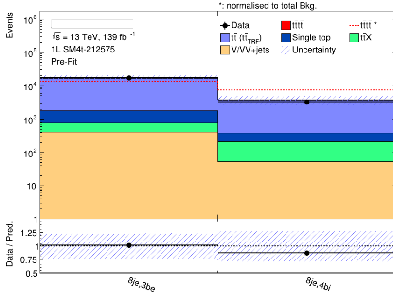
Figure 6.3: Comparison of prediction to data in control regions prior to the fit to data. The t\bar{t} +jet background is estimated through the data-driven method. The hashed area represents the combination of the statistical and systematic uncertainties on the background prediction. The bottom panel displays the ratio of data to the total prediction.
