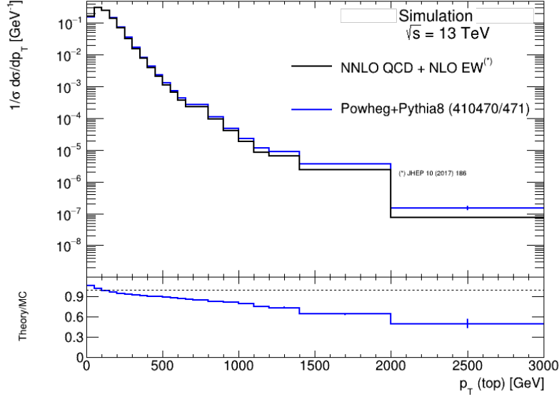
Figure A.1: Normalised t\bar{t} differential cross section as a function of top quark p_T as predicted by the NNLO QCD + NLO EW calculations compared to the nominal NLO t\bar{t} simulation sample (POWHEG + PYTHIA 8).
