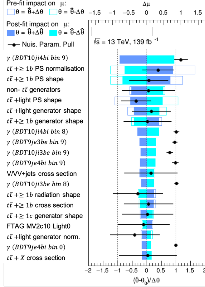
Figure 6.22: Ranking plot from the fit on data under the signal-plus-background hypothesis. The \gamma parameters refer to statistical uncertainty on the background model and are assumed to be Poisson-distributed NPs.
