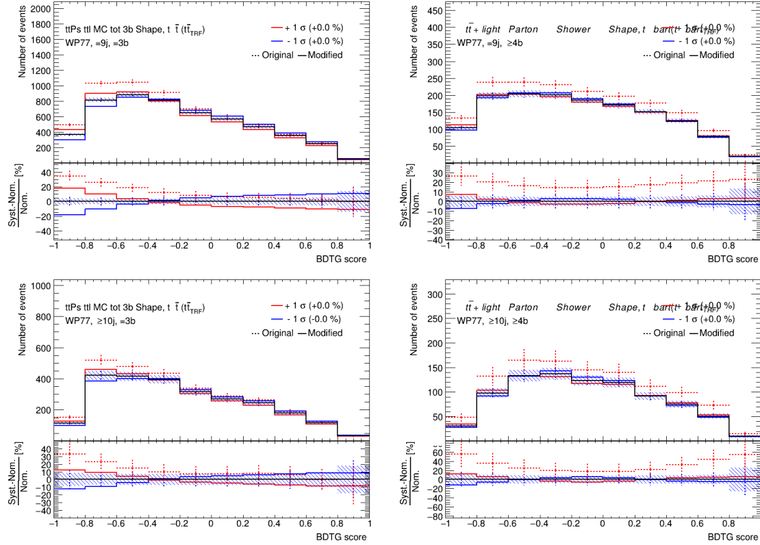
Figure 6.25: Pre-fit uncertainties associated to the parton shower generator on t\bar{t} +light shape in the signal regions. Red points refer to the original variation, with associated statistical error. The red solid line is obtained by smoothing the uncertainty consistently with the statistical uncertainty of the variation. The blue solid line is obtained by symmetrising the red one. Red and blue solid lines give the uncertainty on the prediction.
