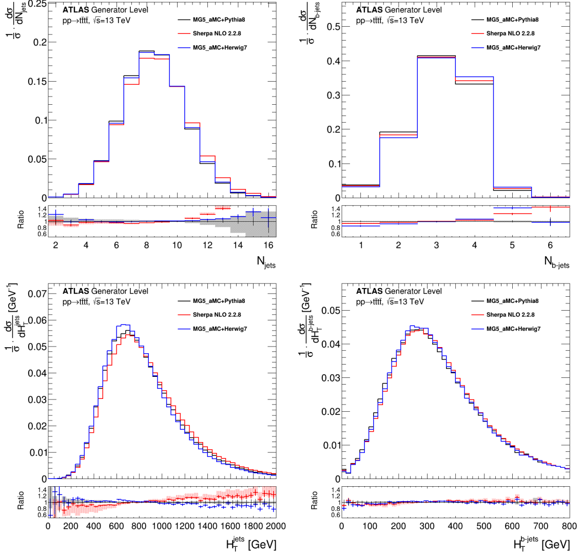
Figure 4.2: Distributions of the jet and b -jet multiplicities, the scalar sum of jets and b -jets p_T ( H_T ) from MADGRAPH5_AMC@NLO + PYTHIA, SHERPA and MADGRAPH5_AMC@NLO + HERWIG t\bar{t}t\bar{t} generation at NLO. All distributions are normalised to one. The lower ratio is calculated with respect to the MADGRAPH5_AMC@NLO + PYTHIA NLO distribution. The uncertainties shown reflect the finite sample statistics (solid lines) and the effect of the different choices of factorisation and renormalisation scales (shaded bands) [70].
