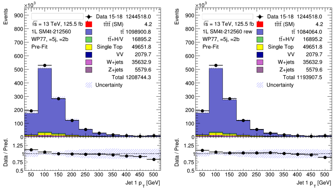
Figure A.5: Comparison between data and prediction of leading-jet p_T before any fit to data. The hashed area represents the combined statistical and systematic (on t\bar{t} modelling) uncertainties of the prediction. Distributions are shown before (left) and after (right) the correction procedure. The comparison is done in the 5je2be region of the 1L channel of the t\bar{t}t\bar{t} analysis.
