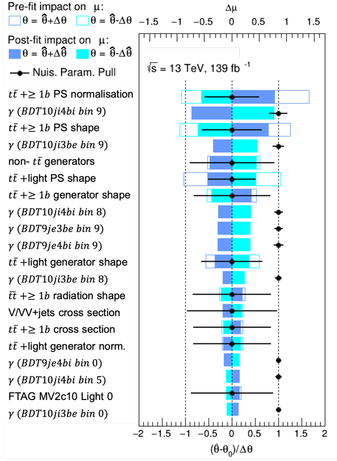
Figure 6.12: Ranking plot from the fit on Asimov data set under the signal-plus-background hypothesis. The \gamma parameters refer to statistical uncertainty on the background model and are assumed to be Poisson-distributed NPs.
