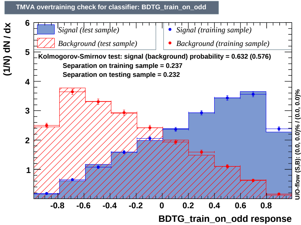
Figure C.8: Training response for the BDT in the 9je4bi region for the training done on odd events.
