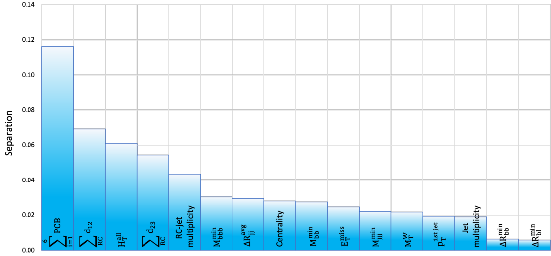
Figure C.9: Ranking of input variables in terms of separation in the 10ji3be region for the training done on even events according to TMVA.
