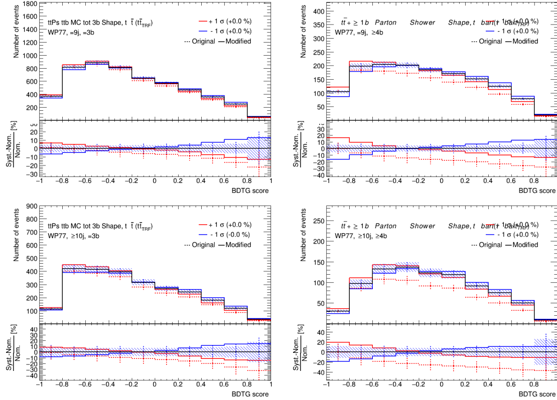
Figure 6.27: Pre-fit uncertainties associated to the parton shower generator on t\bar{t} + \geq 1b shape in the signal regions. Red points refer to the original variation, with associated statistical error. The red solid line is obtained by smoothing the uncertainty consistently with the statistical uncertainty of the variation. The blue solid line is obtained by symmetrising the red one. Red and blue solid lines give the uncertainty on the prediction.
