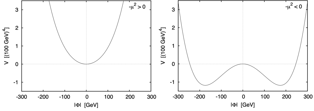
Figure 1.2: Examples of a potential of the type V(|\varphi|^2) = -\mu^2|\varphi|^2 + \lambda|\varphi|^4 , with \lambda > 0 and two different choices for -\mu^2 [9].
