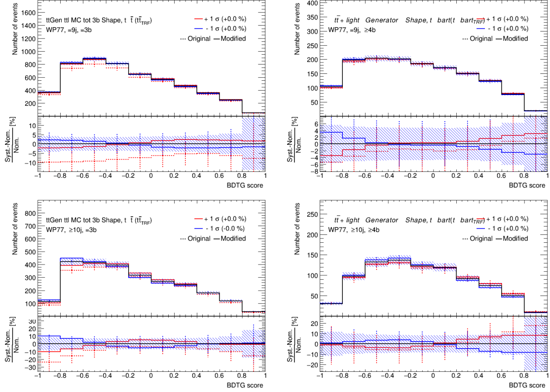
Figure 6.29: Pre-fit uncertainties associated to the matrix element generator on t\bar{t} +light shape in the signal regions. Red points refer to the original variation, with associated statistical error. The red solid line is obtained by smoothing the uncertainty consistently with the statistical uncertainty of the variation. The blue solid line is obtained by symmetrising the red one. Red and blue solid lines give the uncertainty on the prediction.
