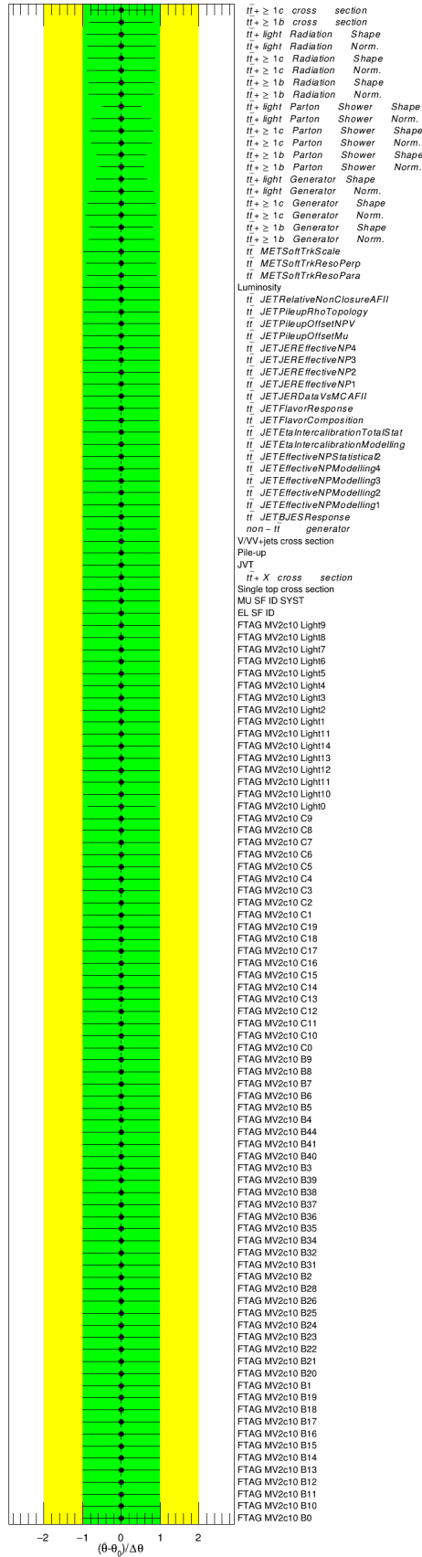
Figure 6.11: Fitted nuisance parameters on Asimov data set under the signal-plus-background hypothesis in the signal regions only.
