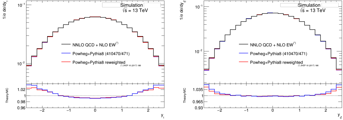
Figure A.4: Normalised t\bar{t} differential cross section as a function of top quark rapidity (on the left) and rapidity of the t\bar{t} system (on the right) before and after the correction of top quark p_T to the NNLO QCD + NLO EW prediction.
