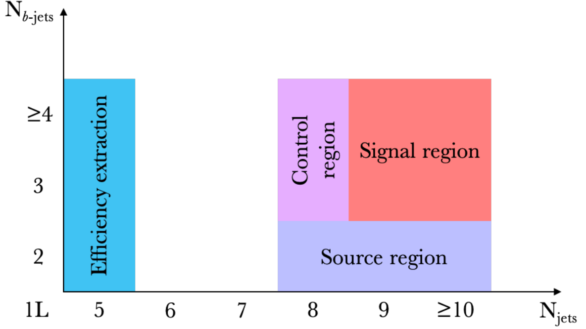
Figure 4.3: Schematic view of the regions definition.
