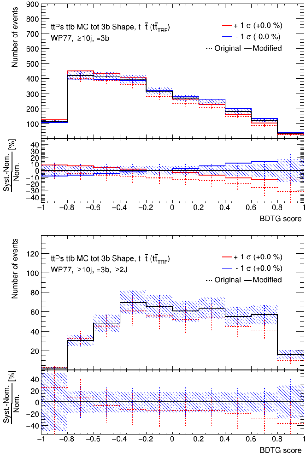
Figure 6.16: Pre-fit uncertainties associated to t\bar{t} parton shower in 10ji3be region (on the top) and 10ji3be2Ji sub-region (on the bottom). Red points refer to the original variation, with associated statistical error. The red solid line is obtained by smoothing the uncertainty consistently with the statistical uncertainty of the variation. The blue solid line is obtained by symmetrising the red one. Red and blue solid lines give the uncertainty on the prediction.
