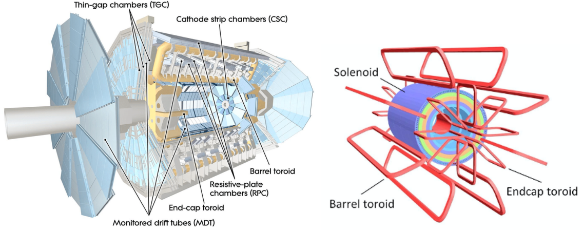
Figure 2.10: Schematic view of the ATLAS Muon Spectrometer and of the magnet system [23].
