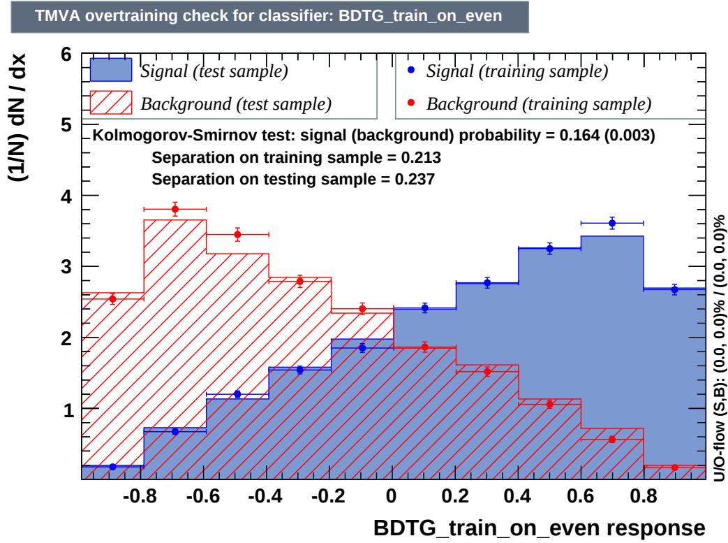
Figure C.6: Training response for the BDT in the 9je4bi region for the training done on even events.
