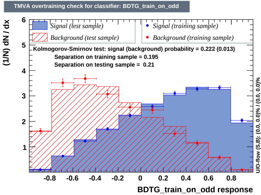
Figure C.14: Training response for the BDT in the 10ji4bi region for the training done on odd events.
