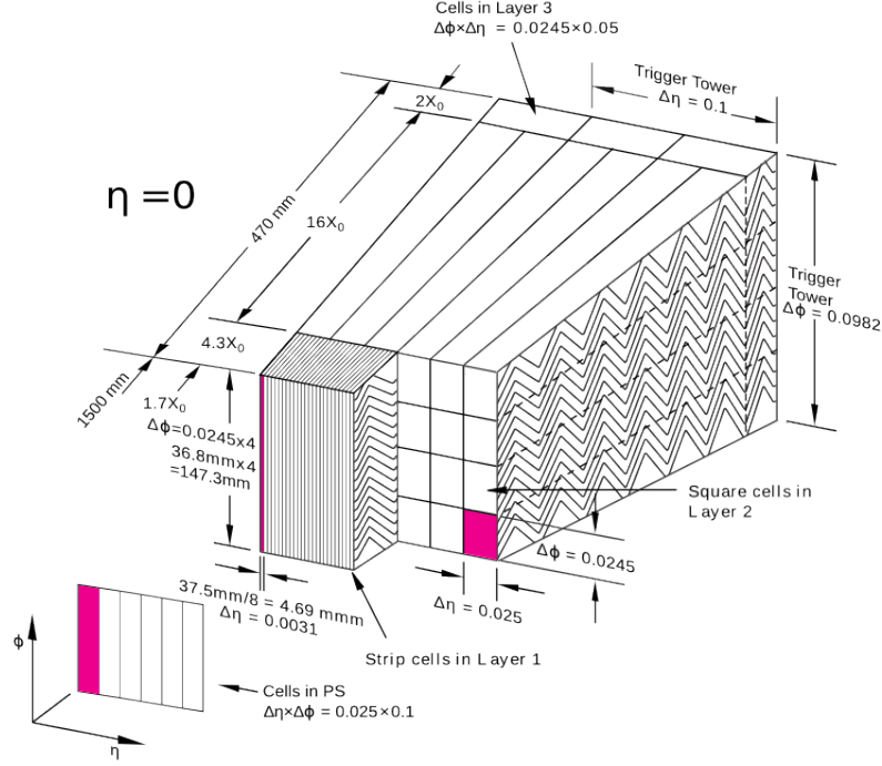
Figure 2.9: Sketch of an EM barrel module with the three different layers. The granularity of the cells is also shown [23].
