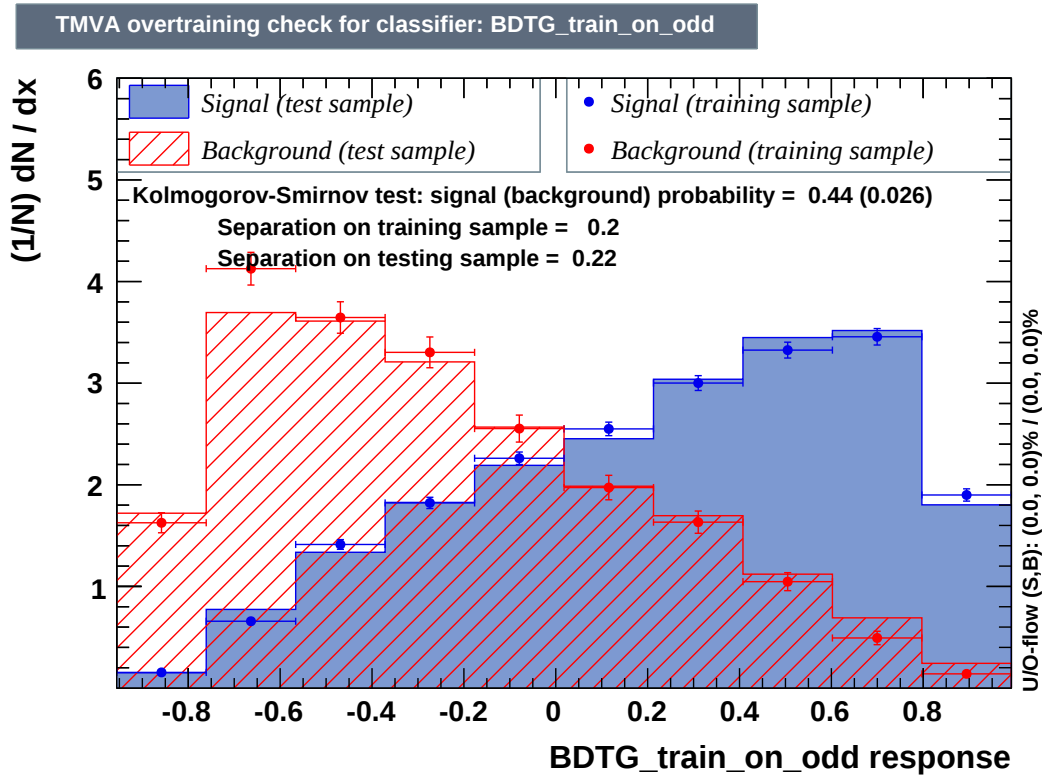
Figure C.12: Training response for the BDT in the 10ji3be region for the training done on odd events.
