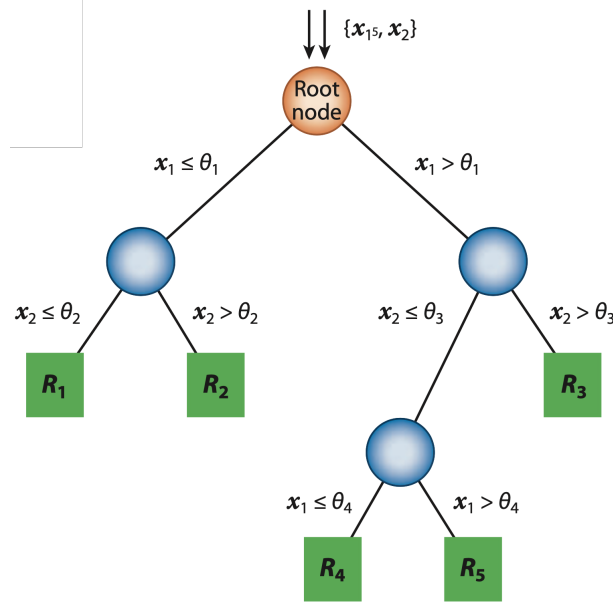
Figure 5.3: A schematic representation of a binary decision tree with two input variables x_1 and x_2 [75].
