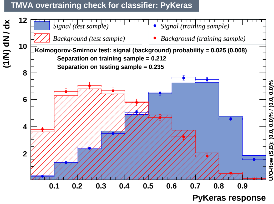
Figure D.1: Training response for the neural network in the 10j4bi region.
