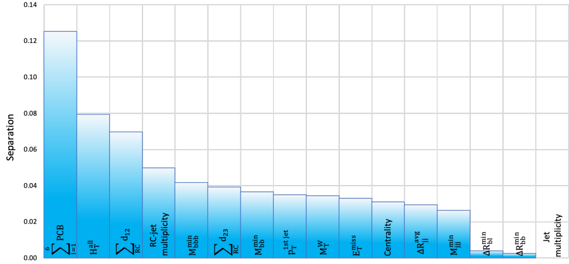
Figure C.3: Ranking of input variables in terms of separation in the 9je3be region for the training done on odd events according to TMVA.
