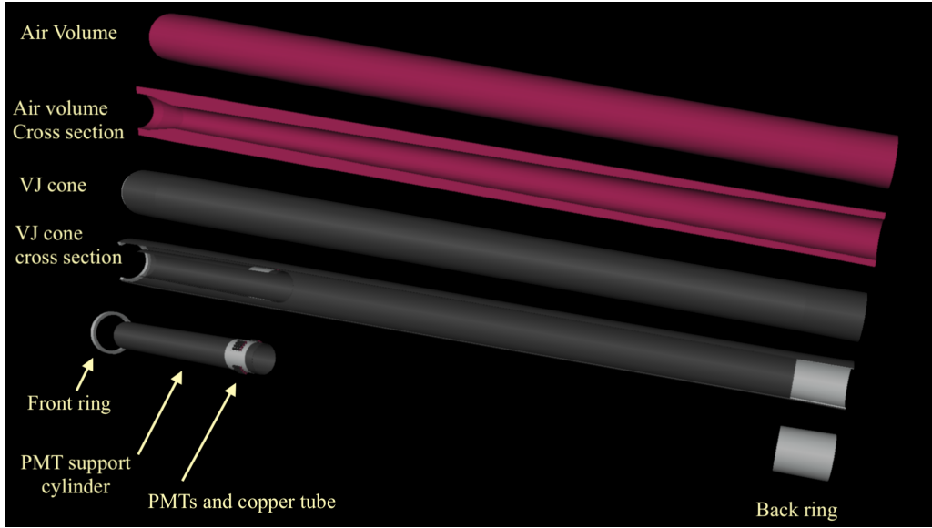
Figure 3.3: Visualization of the layers of the simulated LUCID-2 detector
