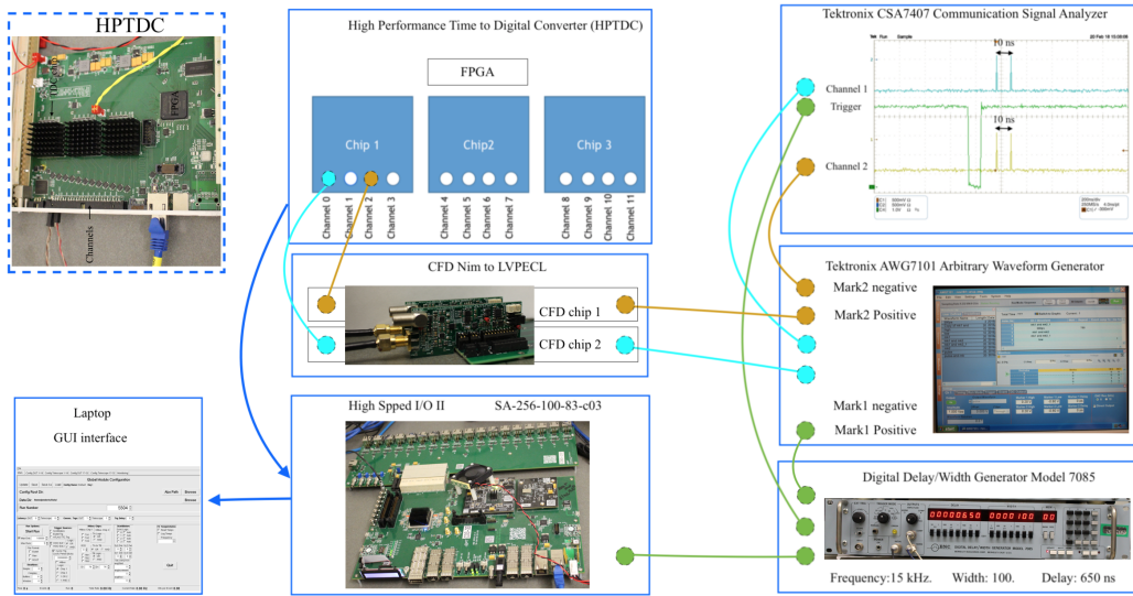
Figure 4.13: A general view of the setup for testing HPTDC channels calibration and precision.
