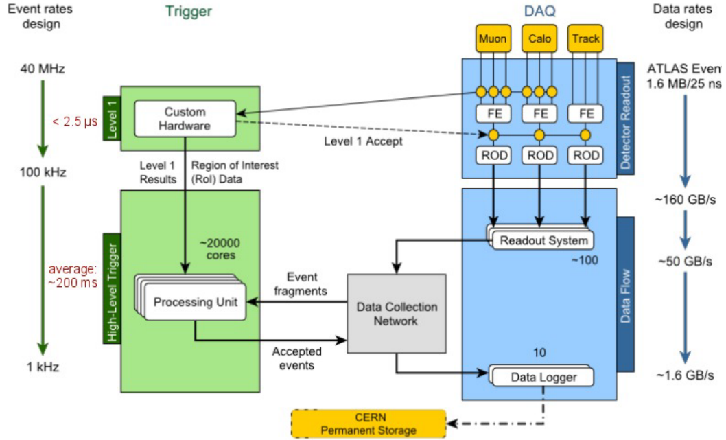
Figure 1.14: Overview of the ATLAS TDAQ system during Run 2.
