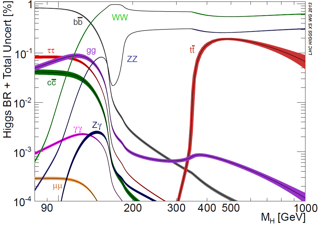
Figure 2.5: Predictions for the probabilities of various decays of the Standard Model Higgs, as a function of the Higgs mass.
