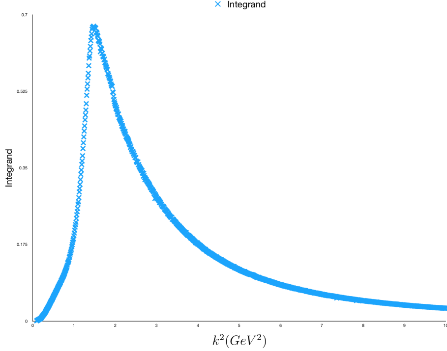
Figure 6.4: The integrand of the k integrand in equation \int d^2\bar{k} \int_0^1 d\alpha_l \int_0^1 d\tau \alpha_s^3(\bar{k}^2) \sum_q (F_1 + F_2) . F_1 and F_2 are defined in equation 6.7.
