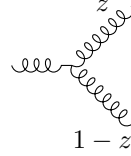
Figure 5.8: Leading order DGLAP splitting functions. C_F = \frac{4}{3} , C_A = 3 , and T_F = \frac{1}{2} are the QCD color factors
