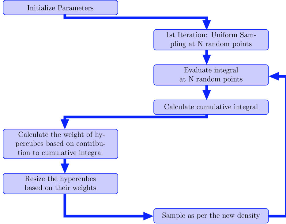
Figure 6.3: VEGAS flowchart
