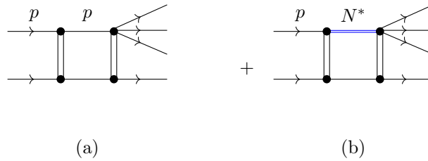
Figure 5.5: The double pomeron exchange contribution to a single diffractive production in the simple two-channel model. (a) Only elastic interaction can happen (b) the intermediate interaction can be inelastic as long as the final interaction is inelastic. Black parallel lines represent the pomeron exchange.
