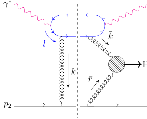
Figure 6.1: Utilization of Cutkosky cutting rules to calculate the imaginary part of the CEDP amplitude. The dotted line indicates the cut which separates the left and right side of the process.
