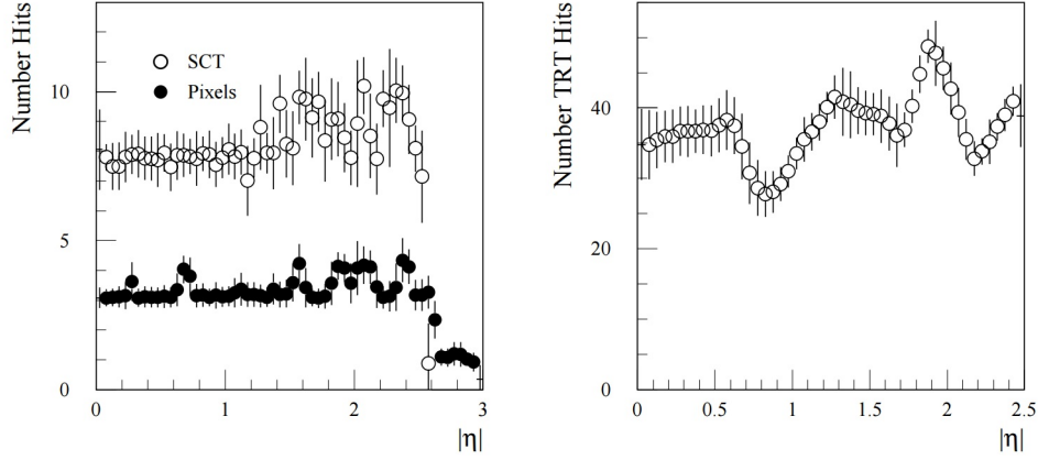
Figure 1.8: Number of Hits per track in the precision detectors and TRT.
