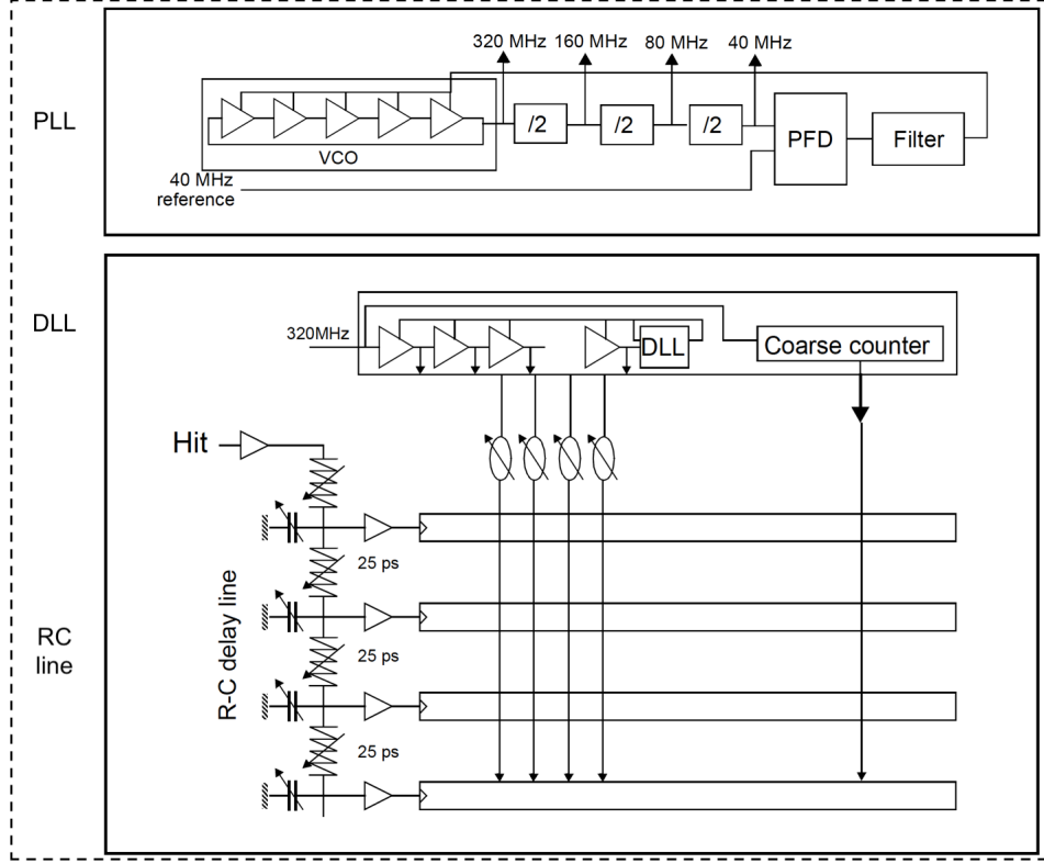
Figure 4.9: HPTDC timing unit [75].
