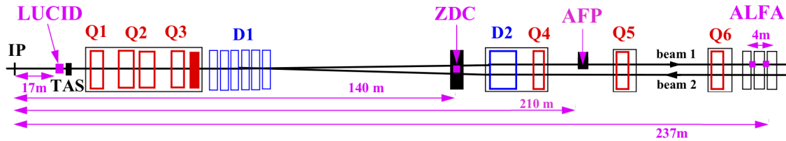
Figure 1.13: A sketch of the ATLAS Forward map, not to scale, showing the positions of ATLAS detectors in the forward region on one side of the interaction point of ATLAS.
