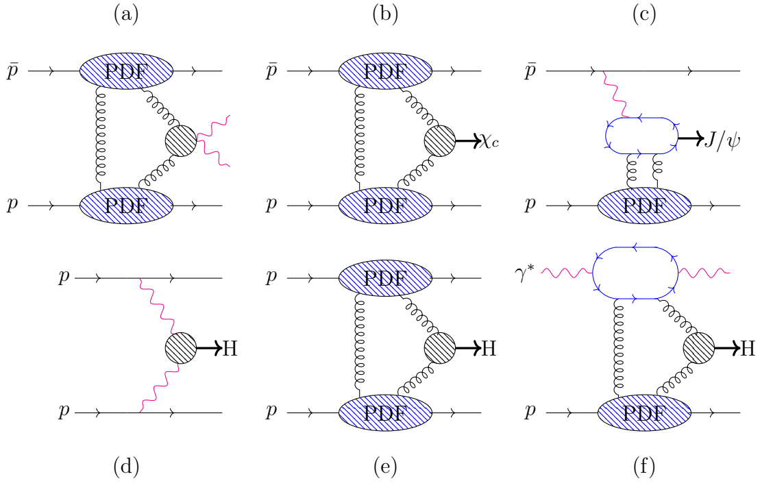
Figure 5.9: The dominant Feynman diagrams for some relevant example CED processes. First row: (a) p\bar{p} \rightarrow p + \gamma\gamma(l^+l^-) + \bar{p} , (b) p\bar{p} \rightarrow p + \chi_c + \bar{p} , (c) Elastic photo-production of J/\psi , p\bar{p} \rightarrow p + J/\psi + \bar{p} , (d) pp \rightarrow p + H + p , (e) Double Pomeron exchange(DPE), pp \rightarrow p + H + p , (f) \gamma p \rightarrow \gamma + H + p .
