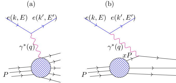
Figure 5.6: (a) Deep inelastic electron-proton scattering of an electron from a proton, (b) Deep inelastic scattering of an electron from a quark constituent of the proton in the parton model.
