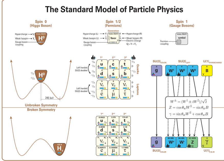
Figure 2.1: The diagram shows the elementary particles of the Standard Model, the Higgs boson, the three generations of quarks and leptons, and the gauge bosons, including their name, mass, spin, charge, chirality, and interactions with the strong, weak and electromagnetic forces. It also shows how the properties of the various particles differ in the symmetric phase and broken-symmetry phase
