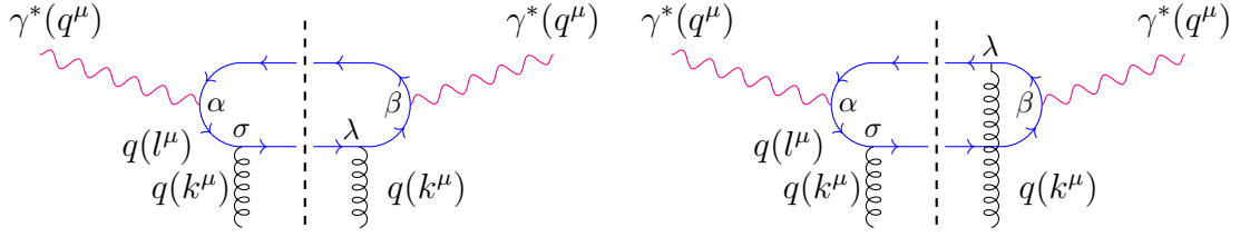
Figure 5.1: We make use of the Cutkosky cutting rules to calculate the imaginary part of the amplitude. The dotted line indicates the cut which separated the left and right side of the process. By applying the optical theorem, the imaginary part of the amplitude is the convolution of the amplitude of the right process and the left process in a three body phase space.
