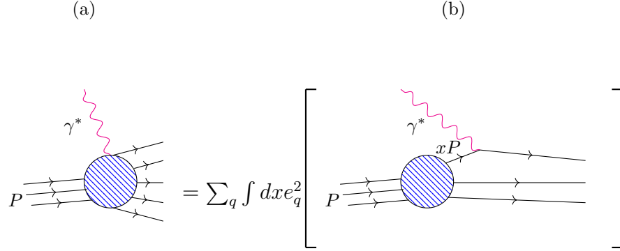
Figure 5.7: (a) The hadronic part of the DIS of an electron from a proton. \gamma^* is the emitted virtual photon that interacts with the other beam proton. (b) Under the assumption that proton consist of uncorrelated point-like quarks, the hadronic cross-section of the DIS can be expressed through the sum of all partonic contribution of the hadron. In this case, the partonic contribution is the DIS of an electron from a quark constituent of the proton.
