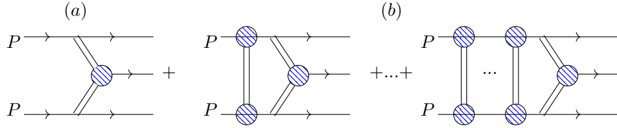
Figure 5.4: The effective amplitude, \mathcal{M}_{eff} , of a diffractive event is the summation of its bare amplitude, \mathcal{M} , shown in Feynman diagram in figure (a), with all the higher order rescattering amplitudes \mathcal{M}_{res} , shown in figure (b).
