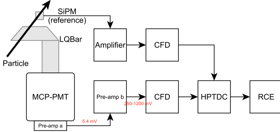
Figure 4.6: AFP electronic readout layout.
