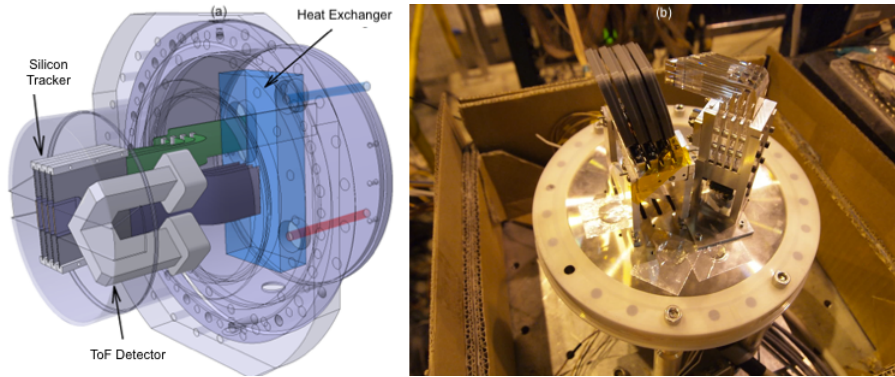
Figure 4.1: (Left) Schematic view of Roman Pot and shows the position of ToF detector and the silicon tracker detector. (Right) Shows the prototype of the ToF detector and the silicon tracker installed inside the Roman Pot.
