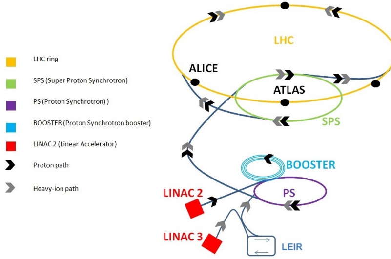
Figure 1.1: The schematic view of the LHC injection chain.
