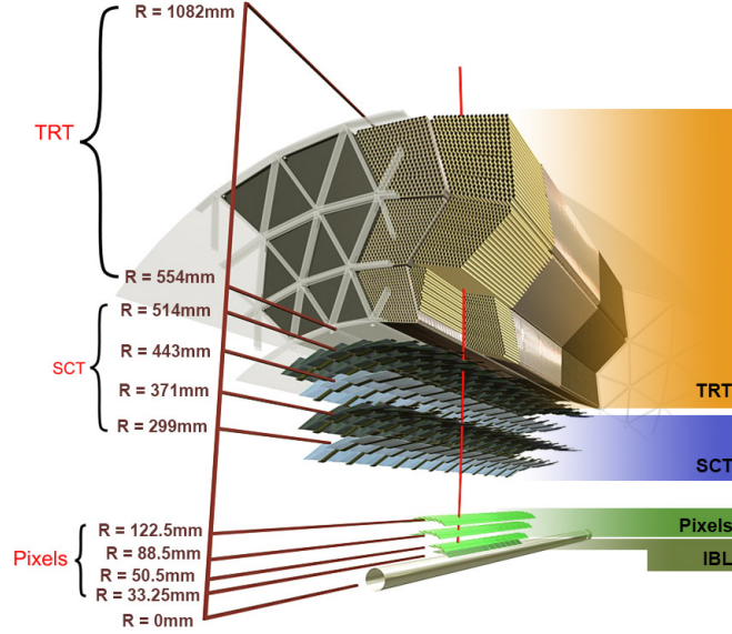
Figure 1.6: Schematic view of the Inner Detector (ID), including the new Insertable B-Layer, the Pixel barrel and end-cap, SCT barrel and end-cap and TRT barrel.
