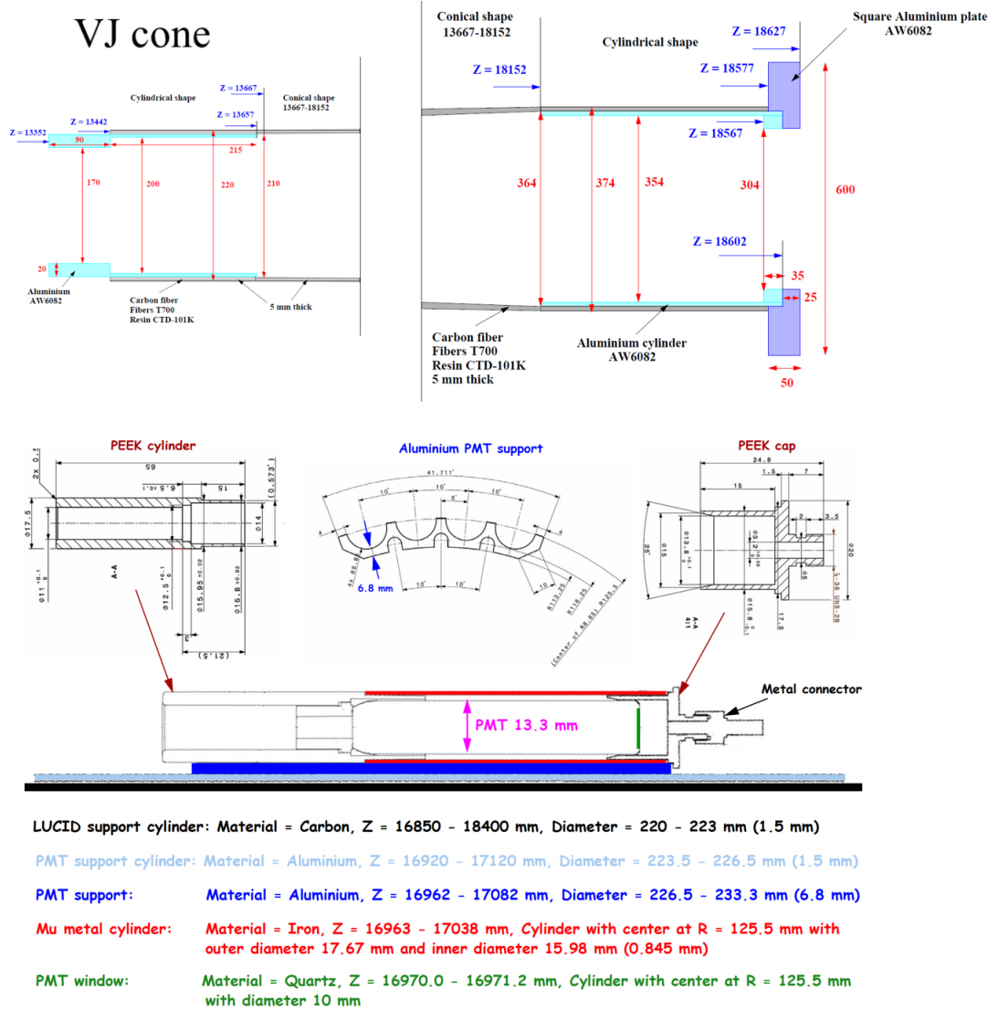
Figure 3.5: Schematic description of the VJ cone, PMT support, muon shield and PEEK cap in the LUCID-2 design
