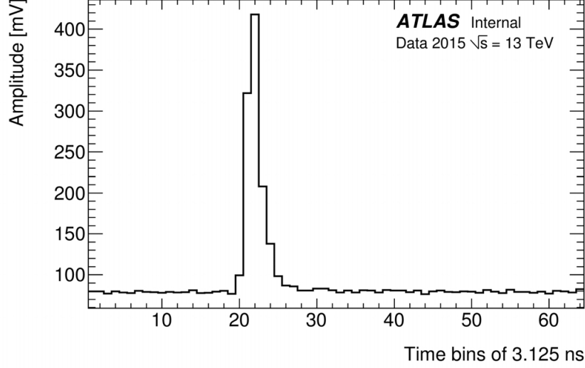
Figure 3.1: Digitized pulse shape of a signal from one of the PMTs in A-arm of the LUCID detector during a 50 ns run in June 2015 at CM energy of 13 TeV. Each time bin represent 3.125 ns long which means the duration of the pulse is less than 25 ns.
