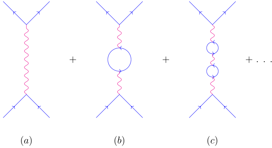
Figure 5.1: (a) First order Feynman diagram of electron-positron pair production via a photon mediator. Diagrams (b) and (c) show the same process in higher order with one loop and more.
