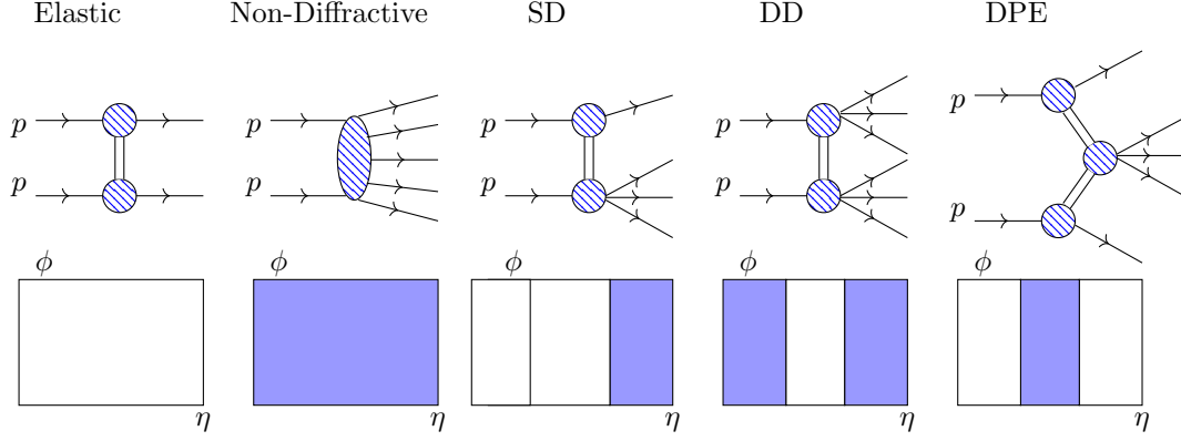
Figure 5.3: Event topologies in \eta vs \phi for elastic and diffractive p-p interactions. Shaded areas represent particle production region and empty areas show rapidity gap regions.
