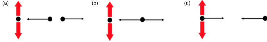
Figure 4.4: A schematic diagram of overlap backgrounds to central exclusive production
