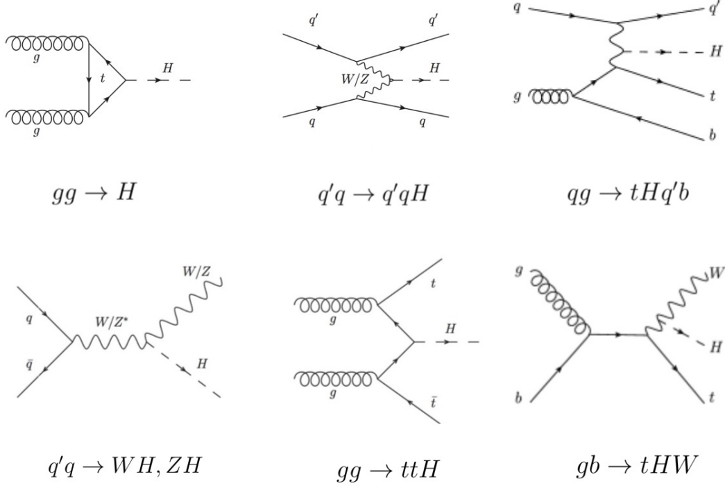
Figure 2.3: Leading order diagrams for Higgs boson production mechanisms at the LHC.
