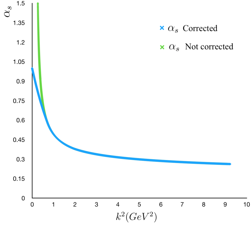
Figure 6.5: Values of \alpha_s MSTW08NLO PDF set and “analytic” model. The green line is the plot of \alpha_s related to MSTW08NLO PDF set. The blue line represents the “analytic” model fitted to the \alpha_s plot from MSTW08NLO at k^2 < 1 \text{ GeV}^2 .
