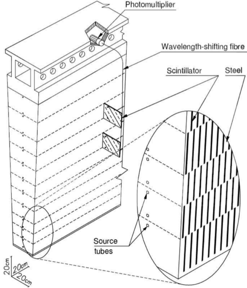
Figure 1.11: Schematic diagram of Tile calorimeter.
