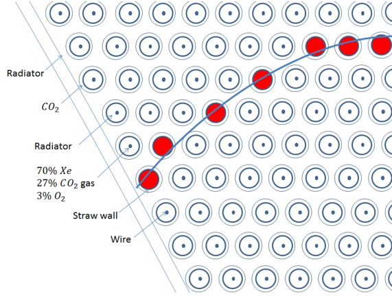
Figure 1.7: Schematic diagram of portion of the TRT detector with an indication of a track of charged particle which is slightly curved due to the magnetic field of solenoid.
