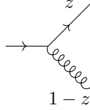
Figure 5.8: Leading order DGLAP splitting functions. C_F = \frac{4}{3} , C_A = 3 , and T_F = \frac{1}{2} are the QCD color factors
