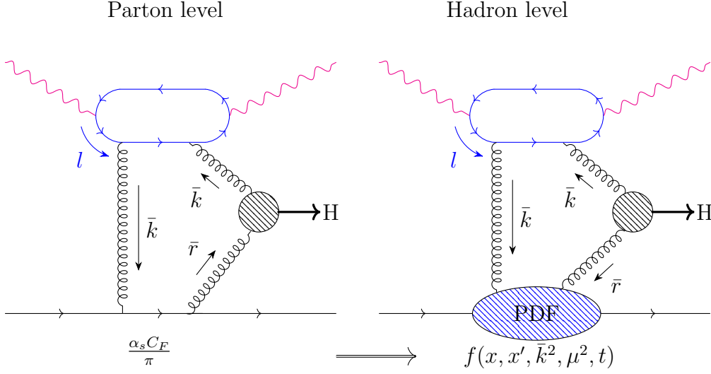
Figure 6.2: Converting parton-level amplitude into the hadron-level amplitude by replacing a factor of \alpha_s C_F / \pi in the amplitude by f(x, x', \bar{k}^2, \mu^2, t) .
