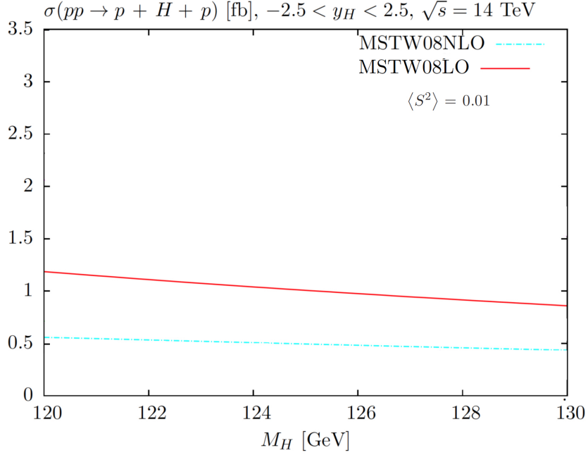
Figure 6.6: Cross-section of the DPE processes in centre of mass energy of 14 TeV, integrated over the rapidity interval -2.5 < y < 2.5 , for a range of PDFs MSTW08LO and NLO [133].
