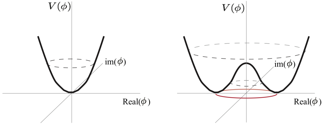
Figure 2.2: (Left) For \mu^2 > 0 there is a unique ground state at \phi = 0 . (Right) For \mu^2 < 0 the ground state is degenerate.
