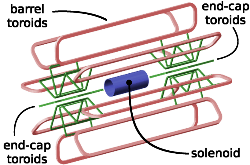
Figure 1.5: Overview of the ATLAS magnet systems.
