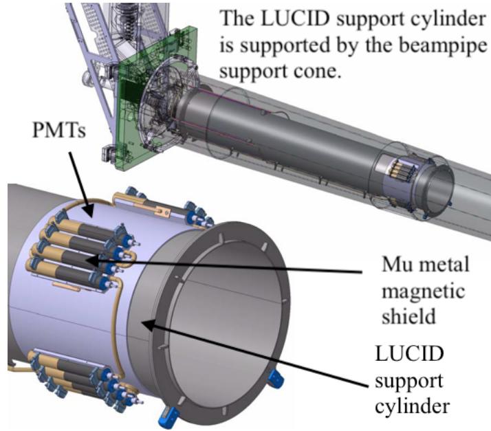
Figure 3.2: Schematic view of LUCID-2 detector.
