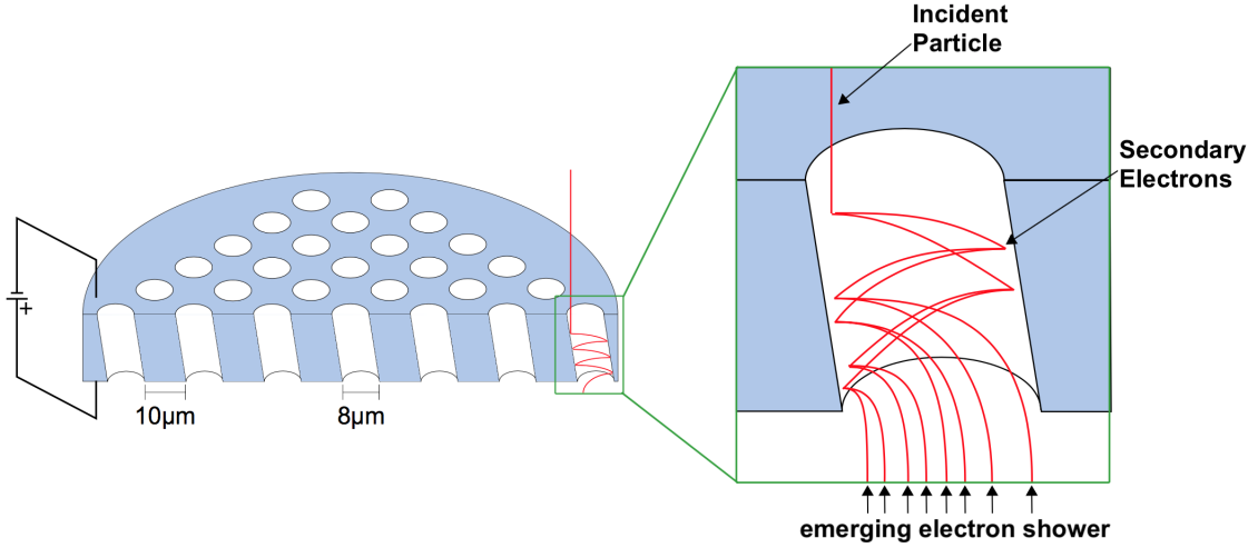
Figure 4.7: Schematic view of a MCP
