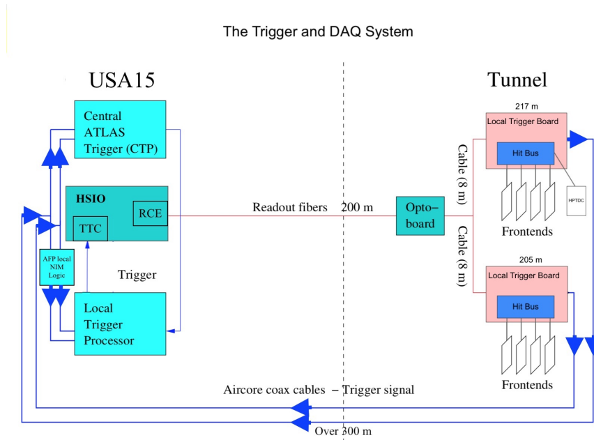
Figure 4.10: AFP Trigger setup
