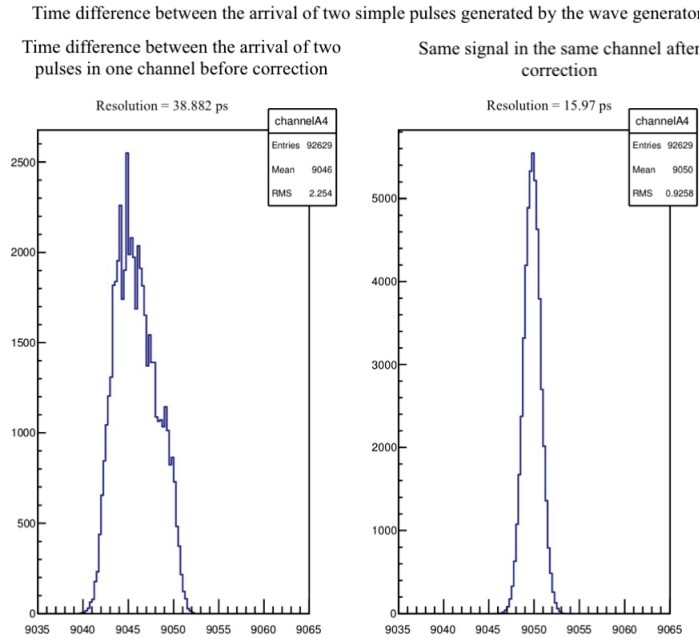
Figure 4.15: HPTDC channel calibration. (Left plot) shows the time difference between the arrival of two pluses in one channel without LSB correction. (Right plot) same distribution after applying Applying the LSB correction.
