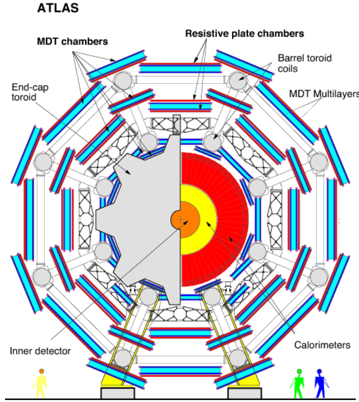
Figure 1.12: Schematic view of a cross-section of the Muon Spectrometer.
