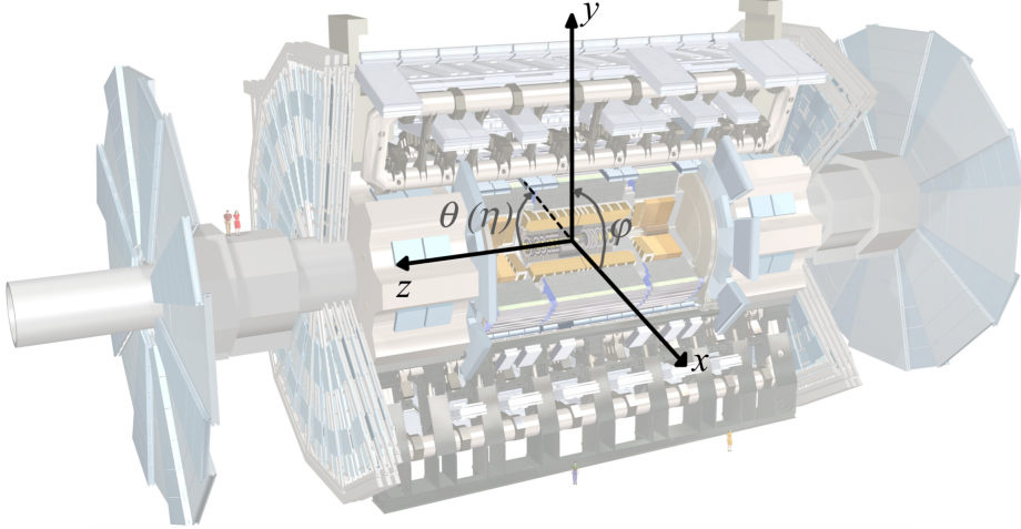
Figure 1.4: ATLAS coordinate system
