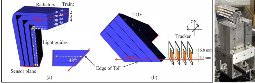
Figure 4.5: The left hand picture is the schematic view of the 4 \times 4 row of LQbar radiators of the ToF detector. It shows the passage of a Cherenkov photon emitted from a proton through the Silicon Tracker detector and LQbars in ToF detector. The right hand picture is a prototype of the new LQbar-mounting made in the University of Alberta.
