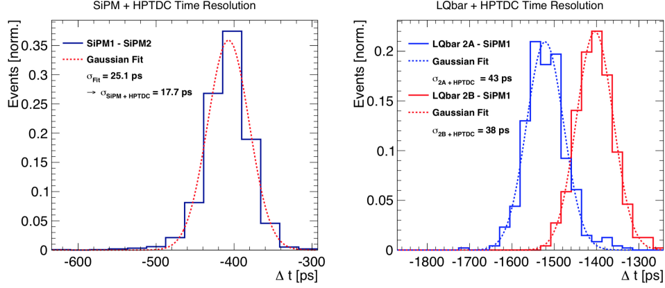
Figure 4.11: Time differences measured with the HPTDC-RCE readout. (Left plot) shows the time differences between the two SiPM channels measured by the HPTDC. (Right plot) shows the time differences between the LQbars and the SiPM reference channel.
