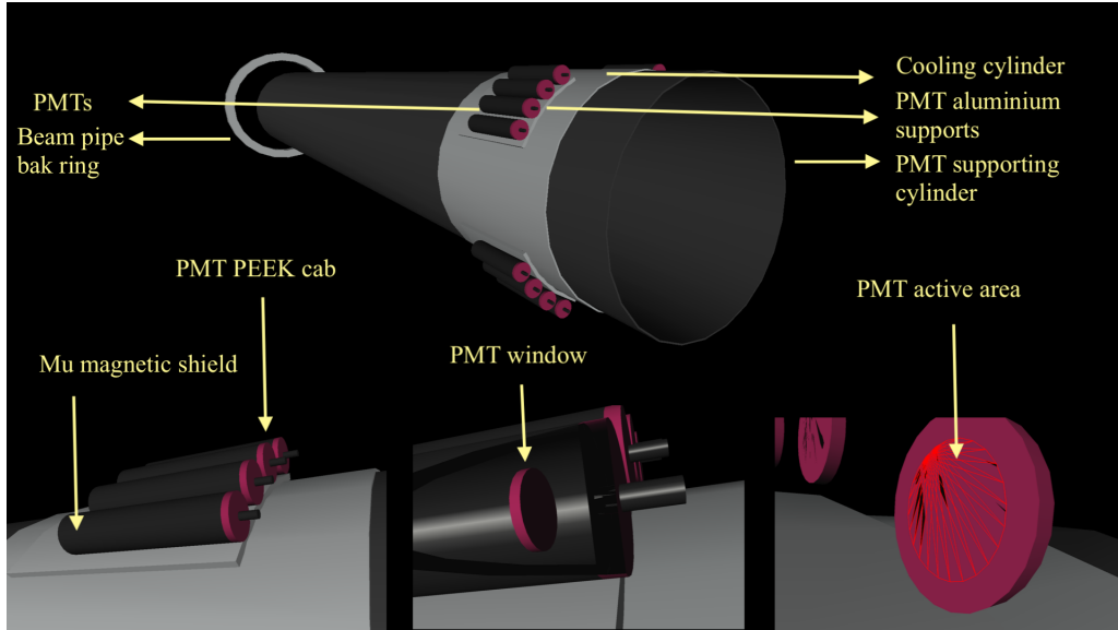
Figure 3.4: Visualization of the PMTs in the simulated LUCID-2 detector
