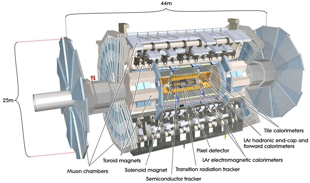
Figure 1.3: Overview of the full ATLAS detector showing the magnet systems and the four major sub-detectors.
