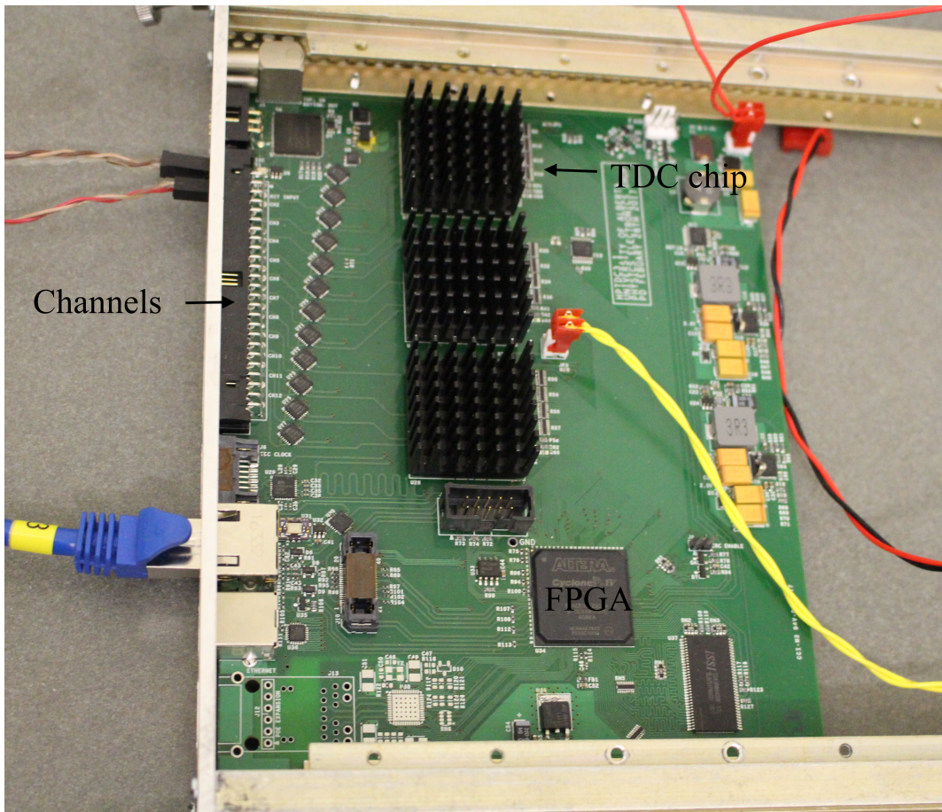
Figure 4.12: The University of Alberta HPTDC board.
