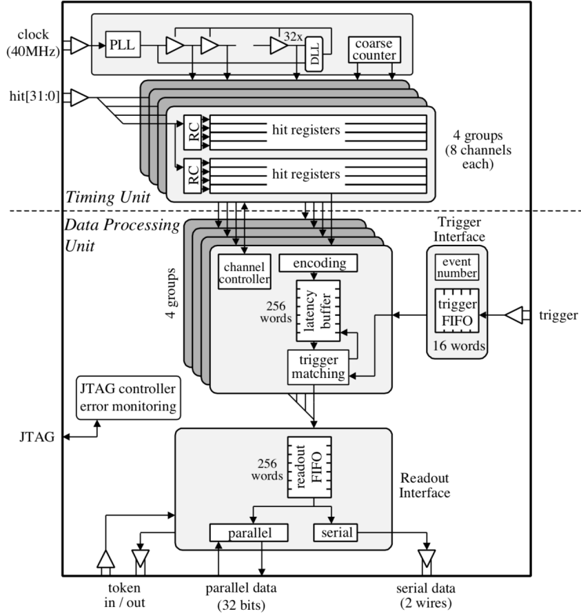
Figure 4.8: The architecture of the HPTDC chip [75].
