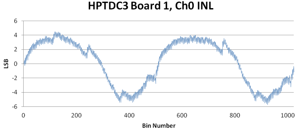
Figure 4.14: Shows the HPTDC bin offset: (bin_i = \frac{2^{10}A}{B} - 1 + \sum_i bin_{(i-1)}) where A is the hit number in bin_i and B is the total number of hits
