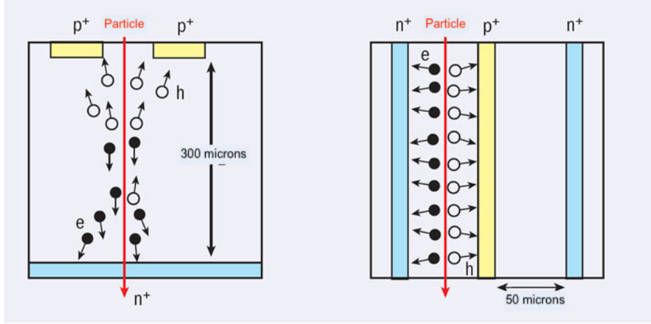
Figure 4.3: Schematic cross-sections of (left) a planar sensor design and (right) a 3D sensor, showing the charge collection in the two designs.
