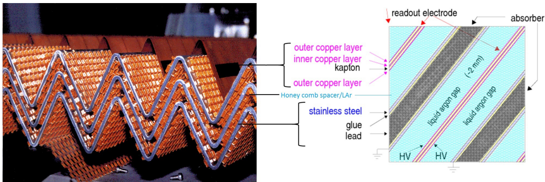
Figure 1.9: Schematic diagram of Electromagnetic barrel accordion calorimeter and a cut away view of inside the accordion geometry.
