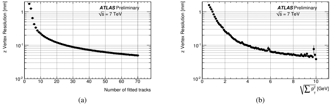
Figure 3.5.: Estimated vertex resolution \sigma_{z_{PV}, \text{true}} in 7 TeV data as a function of the number of tracks N_{\text{trk}} (a) and as function of the value of \sqrt{\sum_{\text{trk}} p_T^2} (b) [89].
