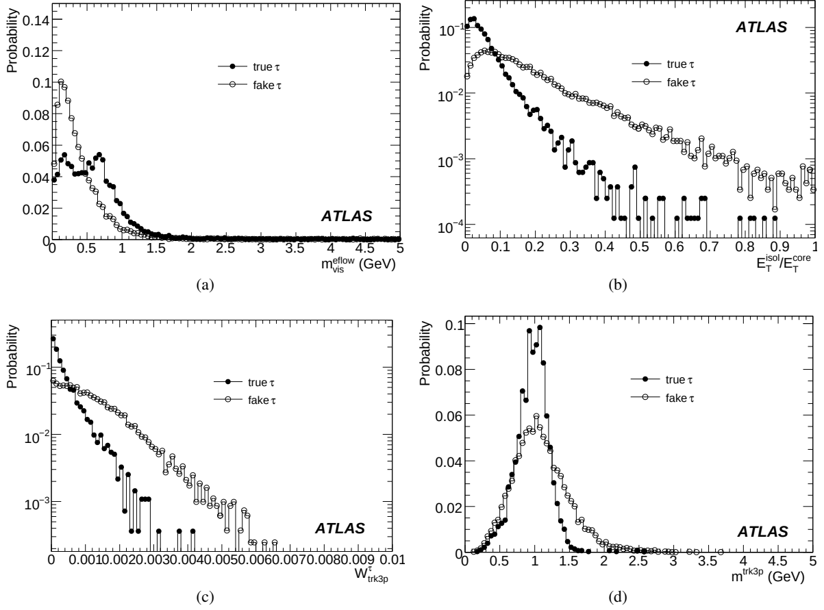
Figure 5.7.: Distribution for signal and background (with a transverse energy range of E_T = 20 - 40 GeV) for the visible mass m_{\text{vis}}^{\text{eff}} and ratio of the transverse energy in the isolation and core region E_T^{\text{isol}}/E_T^{\text{core}} for 1-prong \tau candidates, and the track width W_{\text{trk3p}}^{\tau} and the invariant mass m_{\text{trk3p}} for 3-prong \tau candidates [149].
