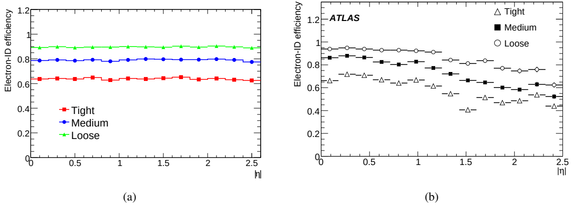
Figure 4.4.: Electron efficiency for loose (green triangles), medium (blue circles), and tight (red squares) selection as function of \eta with the DELPHES reconstruction and identification simulation (left) and electron identification efficiency as a function of \eta for electrons with E_T > 5 GeV from H \rightarrow eee decays taken from [150].
