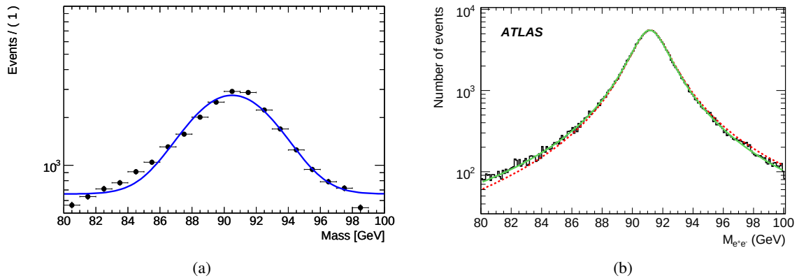
Figure 4.10.: Z boson peak for the decay Z \rightarrow ee for the matrix element ME_{qq2gZZff} , simulated with DELPHES(a), and Z boson mass distribution for PYTHIA events fitted with a Breit-Wigner distribution with (solid line) and without (dashed line) the parton luminosity factor for electrons (b). The blue line in (a) represents a Breit-Wigner fit convoluted with a Gauss fit.
