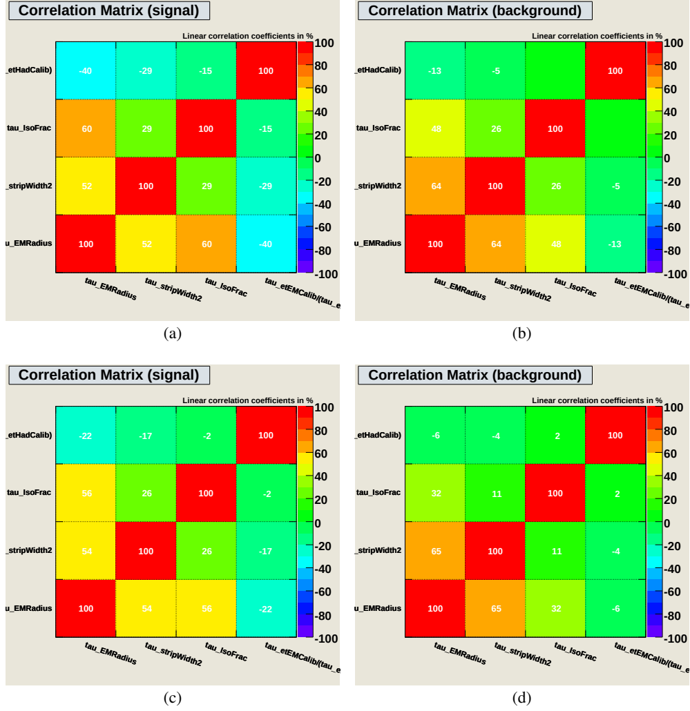
Figure 6.5.: Correlation matrix of calorimeter-based approach for 1-prong \tau candidates and multi-prong \tau candidates for signal (a, c) and background (b, d) for a E_T^{\text{vis}} range of 25 – 45 GeV.
