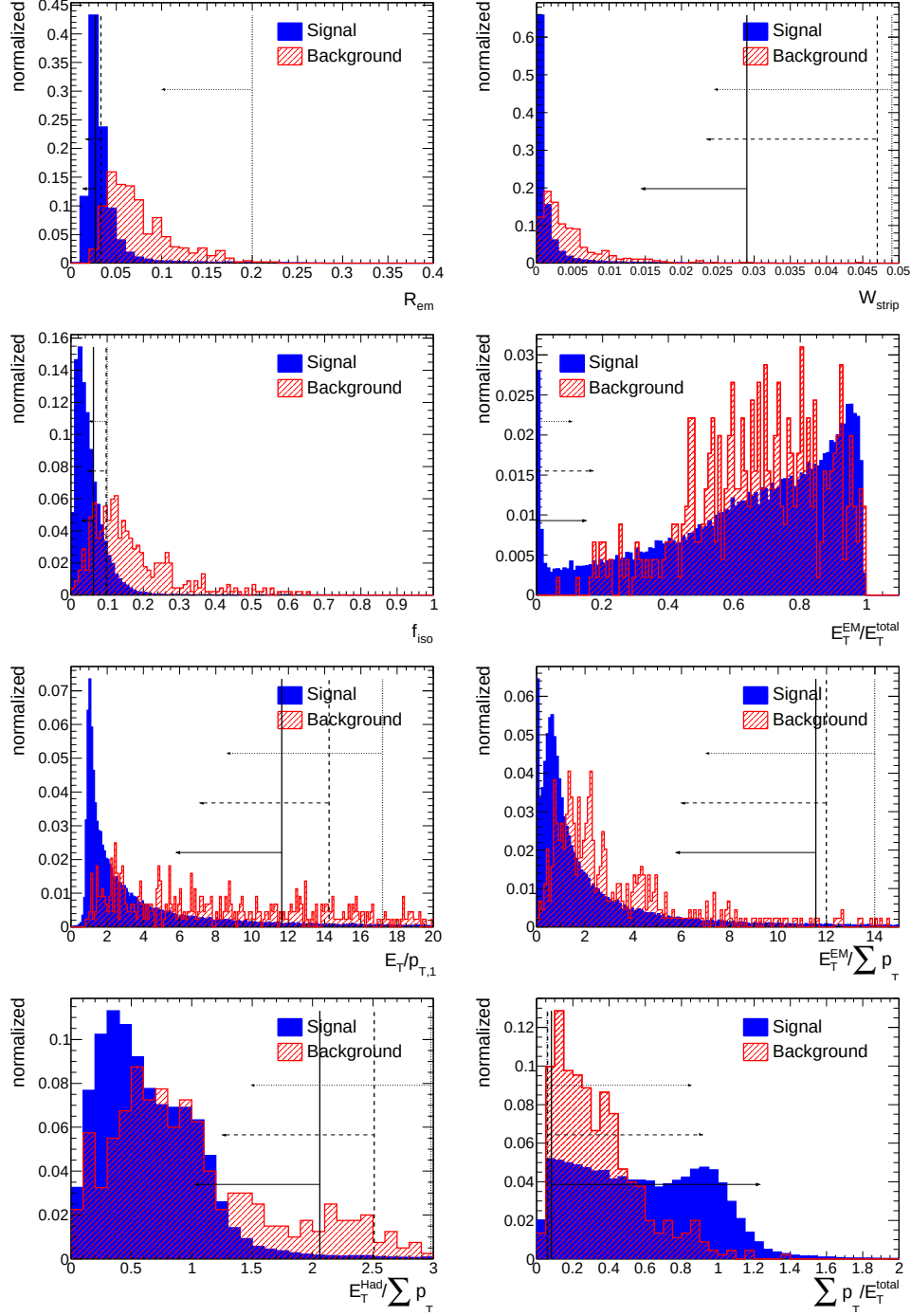
Figure A.12.: Distribution of calorimeter and tracking variables for 1-prong \tau -lepton candidates within a p_T range of > 100 GeV, position of tight (solid line), medium (dashed line), and loose (dotted line) cuts are shown.
