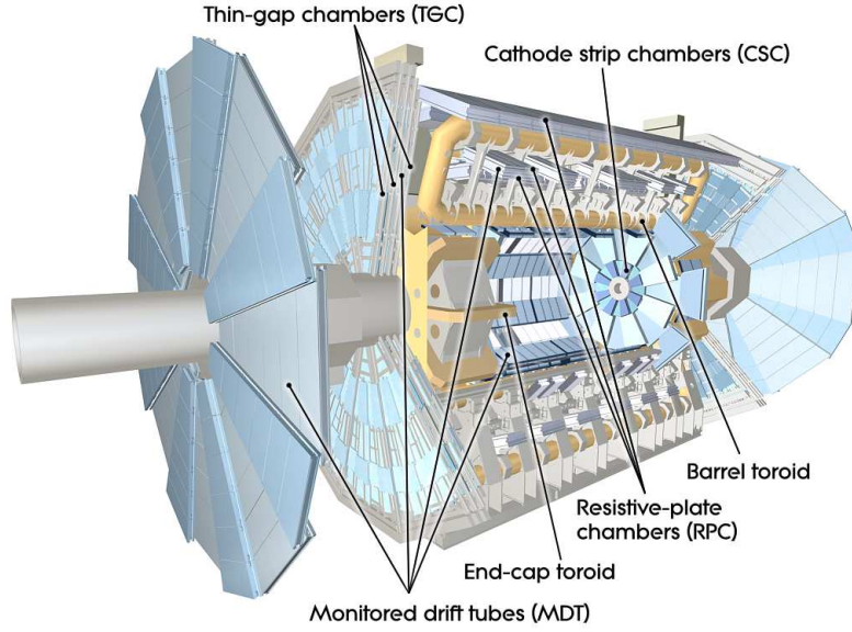
Figure 3.14.: Cut-away view of the ATLAS muon system [78].
