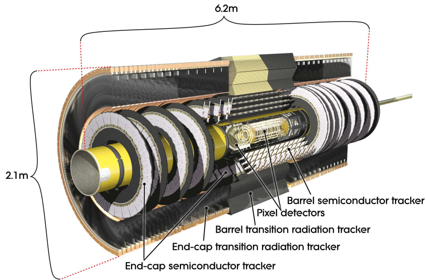
Figure 3.4.: Cut-away view of the ATLAS Inner Detector [78].
