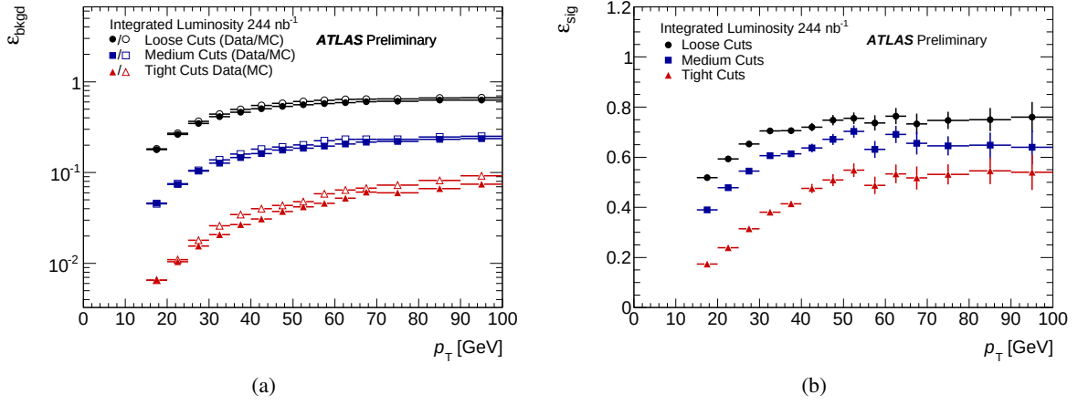
Figure 5.10.: Background efficiencies obtained from data and MC samples as a function of the reconstructed p_T^{\tau} (a) and signal efficiencies predicted by a Z \rightarrow \tau\tau MC sample as a function of the reconstructed p_T^{\tau} (b) [168].
