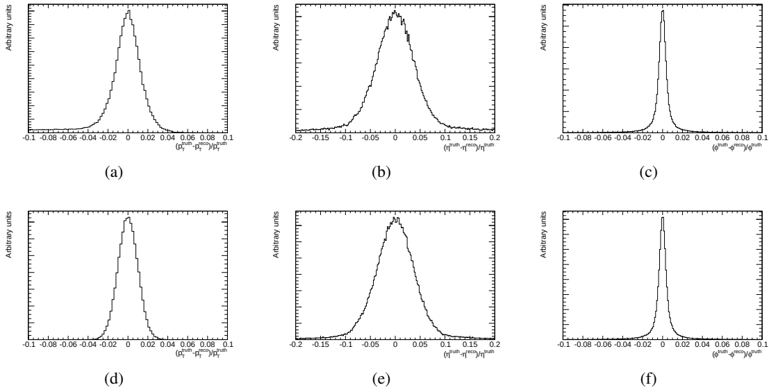
Figure 4.8.: Relative resolution of p_T , \eta , and \phi for electrons and muons for Monte Carlo events, generated with the HERWIG++ matrix element ME_{qq2gZ2ff} and passed through DELPHES and the reconstruction and identification simulation.
