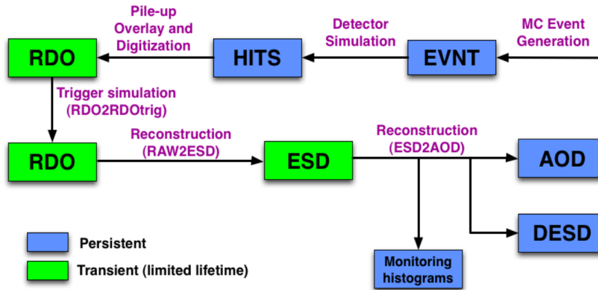
Figure 4.1: Simulation workflow in ATLAS. EVNT files contain events from generators that are propagated through the detector. Resulting HITS are digitized and overlaid with other HITS to simulate the detector response. The resulting RDO format is used as if it were the RAW data coming from the detector (including “Truth” information) [Bir+14].
