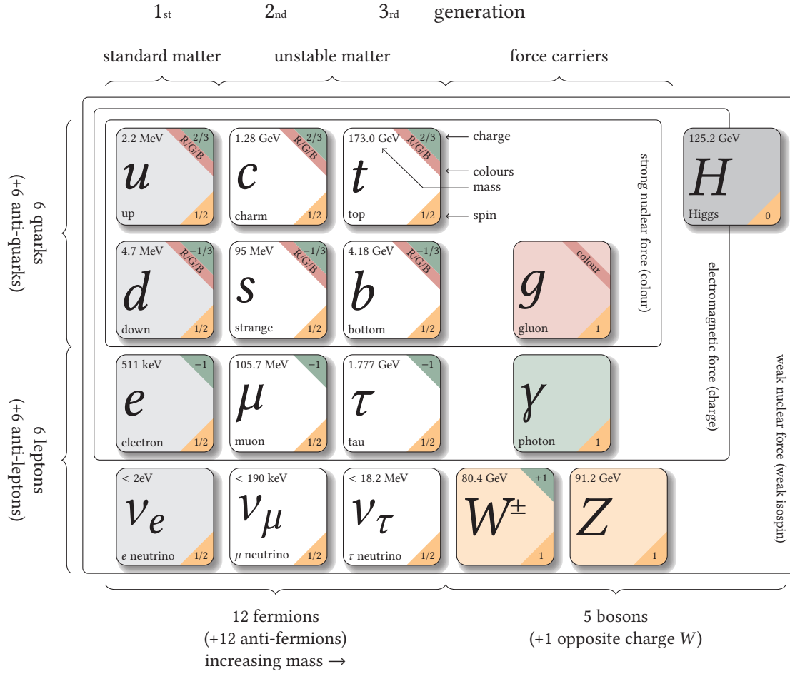
Figure 1.1: All fundamental particles of the Standard Model. Modified version of “ Standard model of physics ” [GB16], updated mass measurements according to “Review of Particle Physics” [Tan+18] in natural units.
