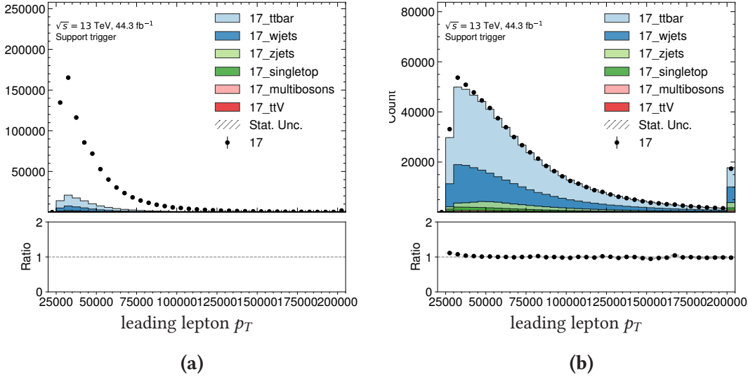
Figure 7.14: Leading lepton p_T for baseline-not-signal (7.14a) and signal (7.14b) 2017 muon events.
