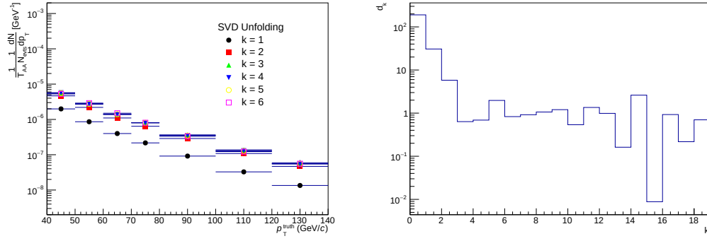
Figure 3.41: Left: Unfolded result for R = 0.2 jets as a function of k . Right: D-vector for R = 0.2 jets.
