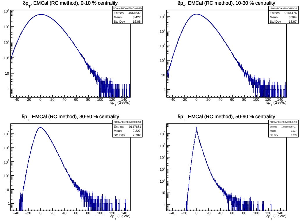
Figure 3.20: \delta p_T as a function of centrality for R = 0.4 jets, using the random cone method.
