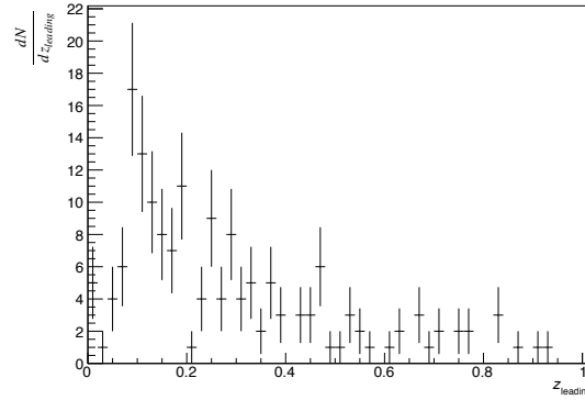
Figure 3.22: Charged track z_{leading} distribution in Pb–Pb data for jets with 120 < p_{T,det}^{jet} < 140 GeV/c, for R = 0.2 in 0-10% centrality. Jets with z_{leading} larger than \approx 0.8 on this plot would be removed by the 100 GeV/c track cut (and approximately corrected for by the jet reconstruction efficiency).
