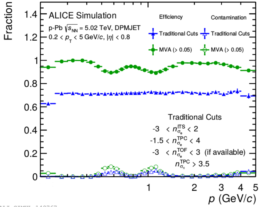
Figure 7.3: Electron PID efficiency and contamination compared between the BDT algorithm outlined in the text and a traditional PID approach whose selection criteria are listed in the lower right box.
