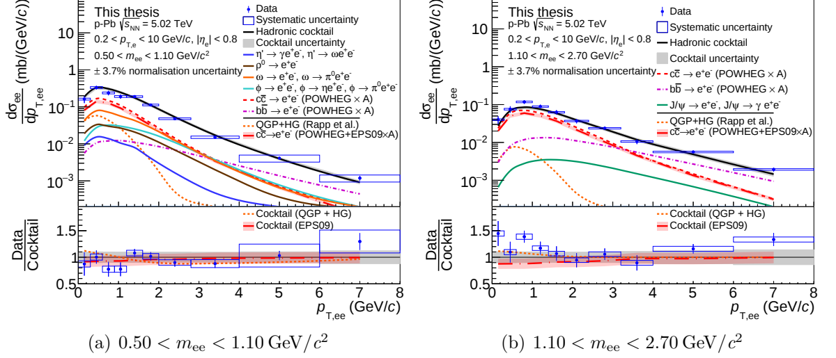
Figure 5.6: The differential dielectron cross section measured in p -Pb collisions at \sqrt{s_{\text{NN}}} = 5.02 TeV as function of p_{\text{T},\text{ee}} in two separate mass intervals. The data are compared to a hadronic cocktail with the heavy-flavour contributions, generated with POWHEG, fit to the cross sections measured in pp collisions [83] and scaled with the atomic mass number of the Pb nucleus ( A = 208 ). Additional models including thermal sources of dielectrons (QGP + HG) [63] and a suppression of the open charm hadron production rate (POWHEG+EPS09) [69] are also presented. In the lower ratio panel all three calculations are compared to the data. The grey band represents the systematic uncertainty of the hadronic cocktail, and the red band represents the uncertainty of the nPDF calculation.
