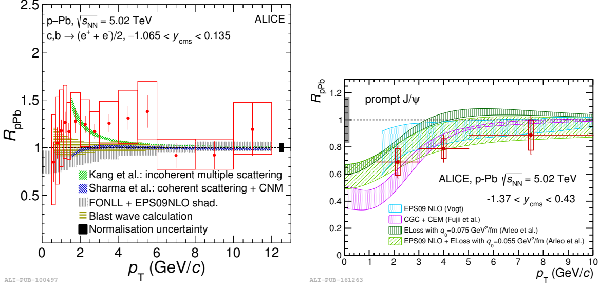
Figure 2.15: Left: Nuclear modification factor ( R_{pPb} ) of electrons from heavy-flavour hadron decays as a function of p_T measured in p-Pb collisions at \sqrt{s_{NN}} = 5.02 TeV [89]. Right: prompt J/\psi R_{pPb} as a function of p_T measured by ALICE in collisions at \sqrt{s_{NN}} = 5.02 TeV [92].
