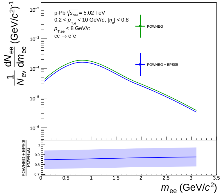
Figure 4.29: The expected dielectron yield from open-charm hadron decays in p\text{-Pb} collisions at \sqrt{s_{\text{NN}}} = 5.02 \text{ TeV} . The vacuum expectation from POWHEG (green) is compared to calculations incorporating the EPS09 nPDF (blue). The blue band in the ratio represents the uncertainty on the nPDF.
