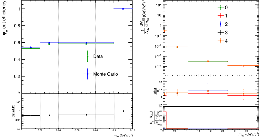
Figure 4.17: Left: \phi_V selection criteria efficiency compared between data (green) and MC simulations (blue) using DPMJet-III. Right: Corrected dielectron yields with differing number of shared hits in the ITS (indicated in by the legend) compared, with the resulting ratio and significance tests plotted below. The blue line the lowest ratio plot indicates the 3\sigma significance level.
