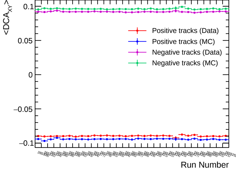
Figure 4.10: The mean DCA_{xy} ( \langle DCA_{xy} \rangle ) as a function of run number compared between data (positron candidates in red and electron candidates in purple) and simulation (positron candidates in blue and electron candidates in teal). The simulated data in this example were produced with DPMJET-III, propagated through the detector with GEANT 3, and all track and PID criteria outlined in Section 4.2 were applied.
