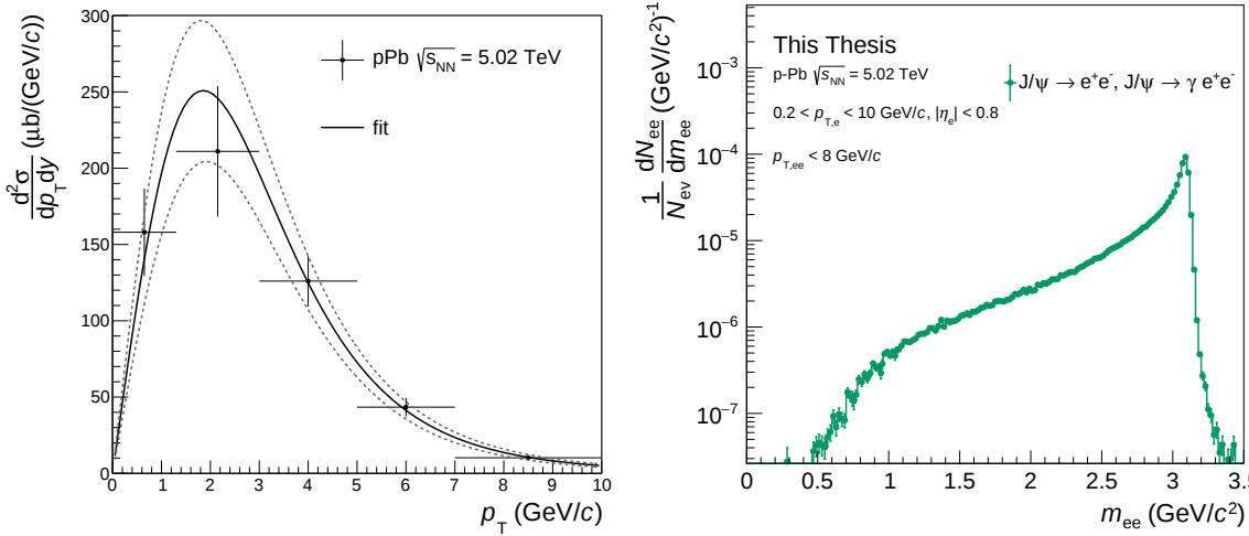
Figure 4.25: The fit to the measured J/ψ p_T spectrum (left) in p–Pb collisions at \sqrt{s_{NN}} = 5.02 TeV [144] used as input to generate the contribution to the dielectron yield (right). The J/ψ decay is performed with PHOTOS [145] and also accounts for the radiative decay ( J/\psi \rightarrow \gamma e^+ e^- ).
