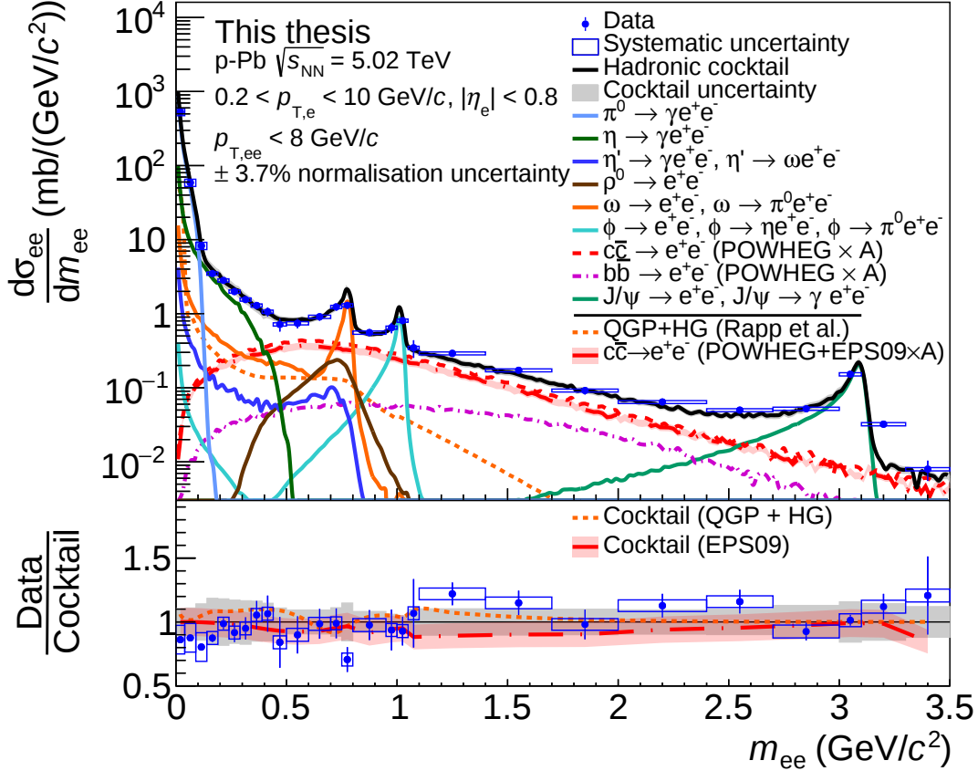
Figure 5.5: The differential dielectron cross section measured in p -Pb collisions at \sqrt{s_{NN}} = 5.02 TeV as function of m_{ee} integrated over the range 0 < p_{T,ee} < 8 GeV/ c . The data are compared to a hadronic cocktail with the heavy-flavour contributions, generated with POWHEG, fit to the cross sections measured in pp collisions [83] and scaled with the atomic mass number of the Pb nucleus ( A = 208 ). Additional models including thermal sources of dielectrons (QGP + HG) [63] and a suppression of the open charm hadron production rate (POWHEG+EPS09) [69] are also presented. In the lower ratio panel all three calculations are compared to the data. The grey band represents the systematic uncertainty of the hadronic cocktail, and the red band represents the uncertainty of the n PDF calculation.
