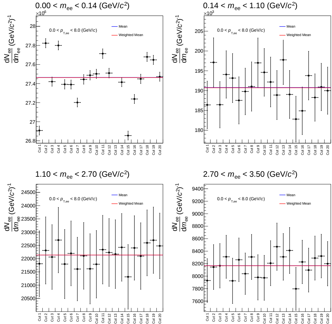
Figure 4.18: Dielectron yields in course m_{ee} bins integrated over 0 < p_{T,ee} < 8 \text{ GeV}/c for the 20 different track and PID selection criteria listed in Tables 7.2 and 7.3 . The mean of the yields is shown in blue and the mean weighted by the statistical uncertainty of each yield is shown in red.
