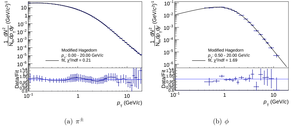
Figure 4.22: \pi^\pm (left) and \phi (right) p_T spectra measured in p -Pb collisions at \sqrt{s_{NN}} = 5.02 TeV by the ALICE collaboration [125, 137]. The fit was performed using a modified Hagedorn function (Eq. 4.18).
