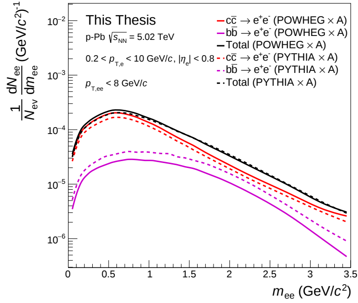
Figure 4.24: The expected dielectron yield per event in p -Pb collisions at \sqrt{s_{\text{NN}}} = 5.02 TeV from c\bar{c} (red) and b\bar{b} (pink) decays as a function of m_{ee} . The simulated yields, performed with POWHEG (solid) and PYTHIA 6.4 (dashed), are scaled to the dielectron cross section measured in pp collision at \sqrt{s_{\text{NN}}} = 5.02 TeV [83], and multiplied by the atomic number of the Pb ion ( A = 208 ).
