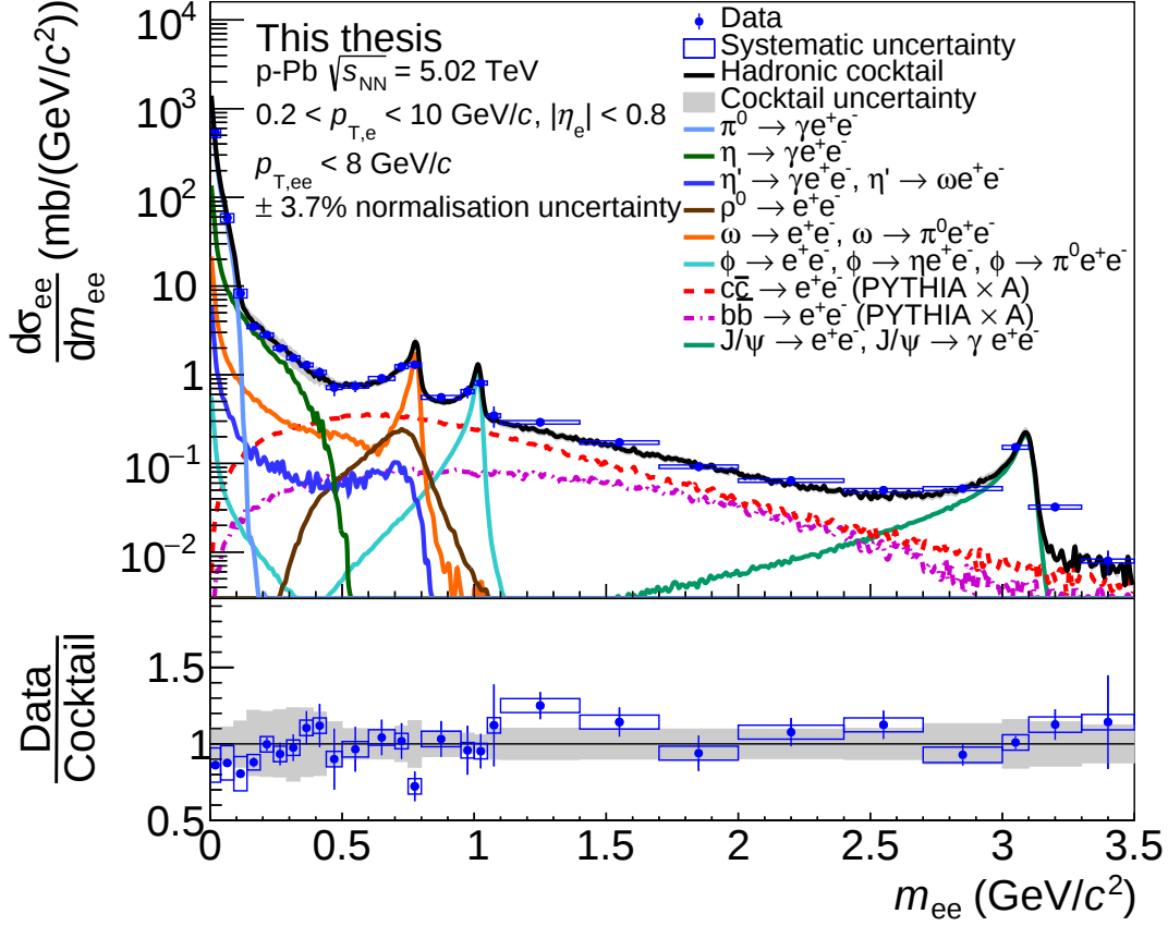
Figure 5.2: The differential dielectron cross section measured in p\text{-Pb} collisions at \sqrt{s_{NN}} = 5.02 \text{ TeV} as function of m_{ee} integrated over the range 0 < p_{T,ee} < 8 \text{ GeV}/c . The data are compared to a hadronic cocktail with the heavy-flavour contributions, generated with PYTHIA 6, fit to the cross sections measured in pp collisions [83] and scaled with the atomic mass number of the Pb nucleus ( A = 208 ). The grey band represents the systematic uncertainty of the hadronic cocktail. The lower panel shows the ratio of the data over the hadronic cocktail.
