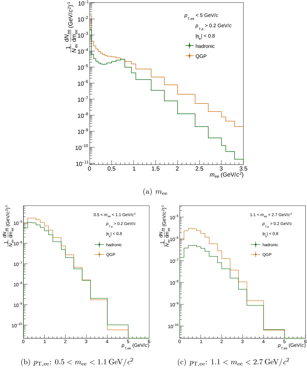
Figure 4.27: Differential thermal dielectron production calculations for p - Pb collisions at \sqrt{s_{NN}} = 5.02 \text{ TeV} as a function of m_{ee} , as well as p_{T,ee} for two mass ranges, shown separately for the partonic (orange) and hadronic (green) phases. The model parameters are outlined in the text and the full procedure is presented in detail in [63].
