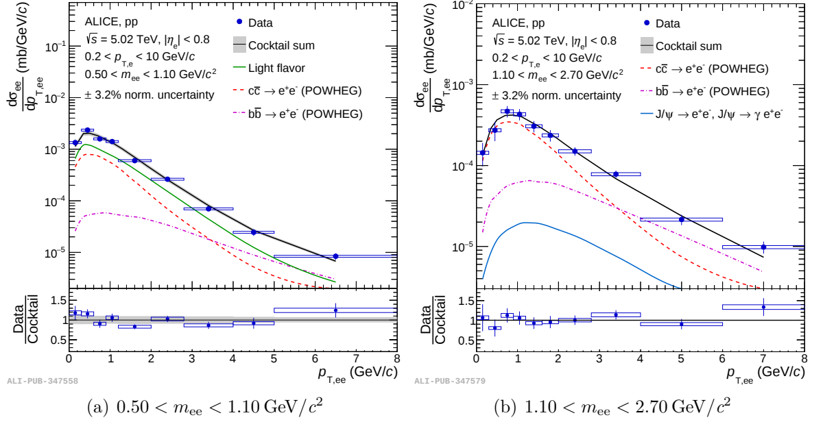
Figure 2.19: The dielectron cross section measured in pp collisions at \sqrt{s_{NN}} = 5.02 TeV as function of p_{T,ee} in two mass intervals [83]. The data are compared to a hadronic cocktail with the heavy-flavour contributions produced with POWHEG and fit to the data in the intermediate mass range ( 1.1 < m_{ee} < 2.7 GeV/c 2 ). The grey band represents the systematic uncertainty of the hadronic cocktail. The lower panel shows the ratio of the data over the hadronic cocktail.
