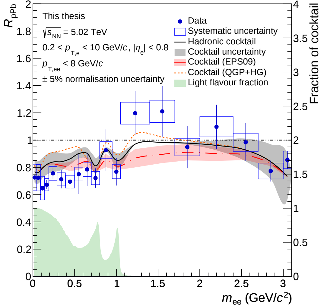
Figure 5.7: The dielectron nuclear modification factor ( R_{pPb} ) as a function of m_{ee} measured at midrapidity at \sqrt{s_{NN}} = 5.02 \text{ TeV} [83]. The hadronic cocktail shown in black represents the baseline expectation with the heavy-flavour contributions generated with POWHEG and the total uncertainty shown in grey. The cocktail (EPS09) (red) incorporates a suppression to the open charm hadron production rate [69], whereas the cocktail (QGP+HG) (orange) includes thermal radiation from the partonic and hadronic phases [63]. The red band represents the uncertainty from the nPDF calculation and the green shaded area is the fraction of light-flavour decays determined from the hadronic p -Pb cocktail.
