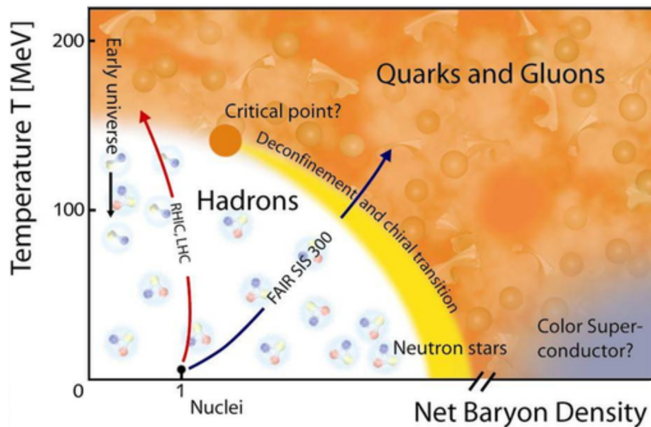
Figure 1.3: Schematic of the QCD phase diagram represented as a function of temperature and net baryon density normalised to nuclear matter density [17].
