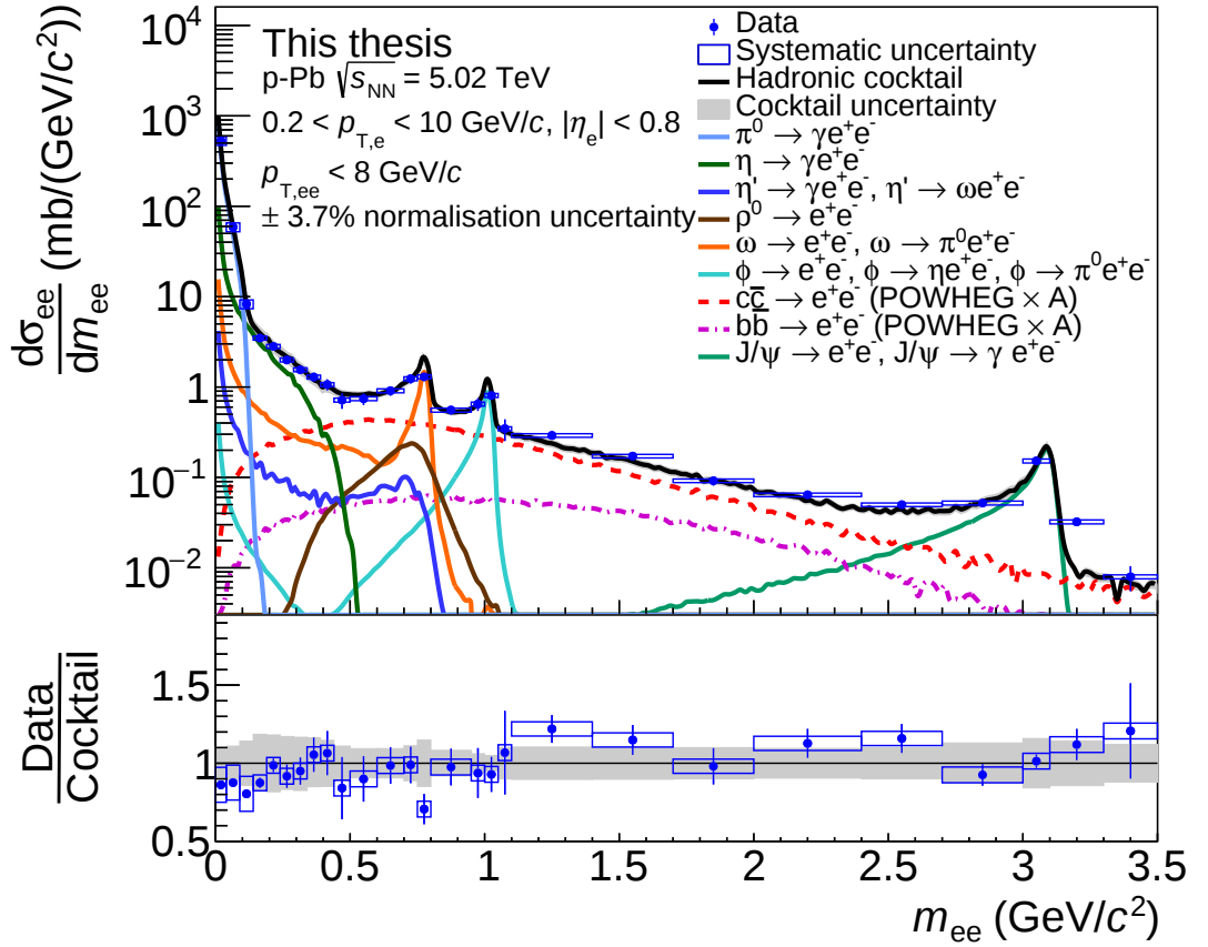
Figure 5.1: The differential dielectron cross section measured in p-Pb collisions at \sqrt{s_{NN}} = 5.02 \text{ TeV} as function of m_{ee} integrated over the range 0 < p_{T,ee} < 8 \text{ GeV}/c . The data are compared to a hadronic cocktail with the heavy-flavour contributions, generated with POWHEG, fit to the cross sections measured in pp collisions [83] and scaled with the atomic mass number of the Pb nucleus ( A = 208 ). The grey band represents the systematic uncertainty of the hadronic cocktail. The lower panel shows the ratio of the data over the hadronic cocktail.
