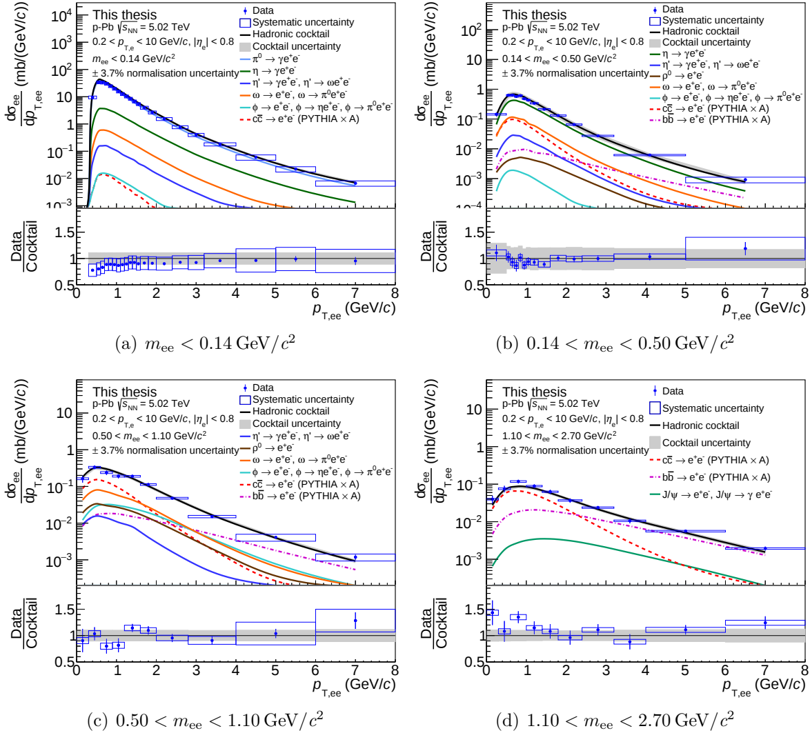
Figure 5.4: The differential dielectron cross section measured in p -Pb collisions at \sqrt{s_{NN}} = 5.02 \text{ TeV} as function of p_{T,ee} in four separate mass intervals. The data are compared to a hadronic cocktail with the heavy-flavour contributions, generated with PYTHIA 6, fit to the cross sections measured in pp collisions [83] and scaled with the atomic mass number of the Pb nucleus ( A = 208 ). The grey band represents the systematic uncertainty of the hadronic cocktail. The lower panel shows the ratio of the data over the hadronic cocktail.
