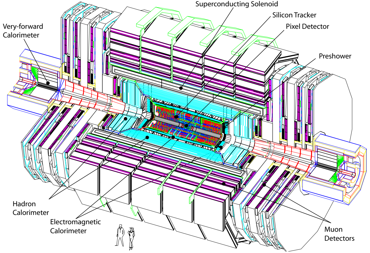
Figure 3.2: Drawing of the CMS detector with its main components [19].
