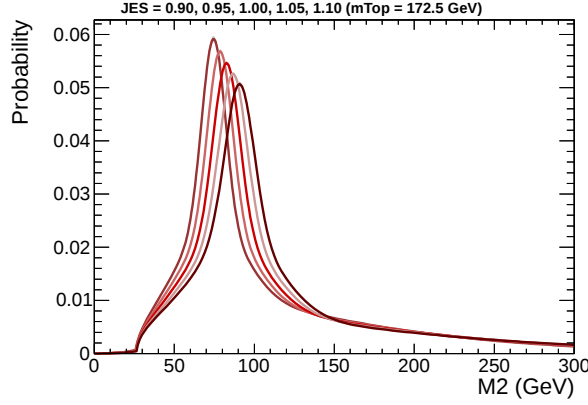
Figure 7.6: Direct comparison of the probability density function P(M2; \text{JES}) at \text{JES} = 0.90, 0.95, 1.00, 1.05, 1.10 .
