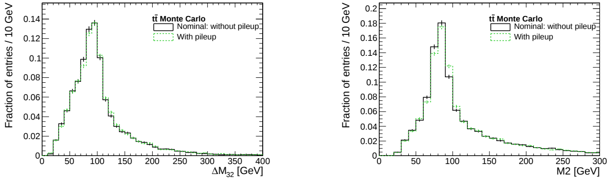
Figure 7.20: Distributions of \Delta M_{32} (left) and M2 (right) in simulated t\bar{t} events with and without pileup.
