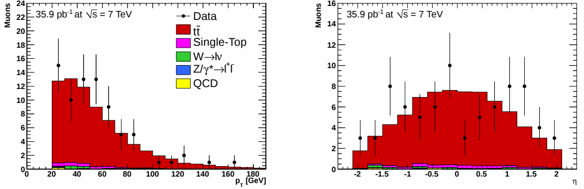
Figure 5.3: Muon transverse momentum (left) and pseudorapidity (right) after the final event selection.
