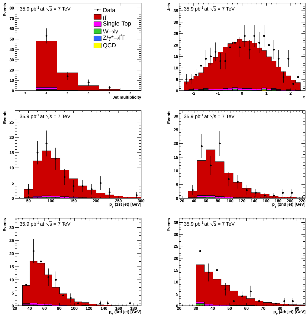
Figure 5.5: Jet multiplicity (first row, left), pseudorapidities (first row, right) and the transverse momenta of the 1st, 2nd, 3rd and 4th leading jet (second row left to third row right) after the final event selection.
