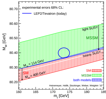
Figure 2.8: Comparison of the measured values of W boson mass, m_W , and top quark mass, m_t , to predictions by the Standard Model (SM) with different Higgs boson masses, m_H , and by the minimal supersymmetric extension (MSSM) with different masses of the supersymmetric particles [12].
