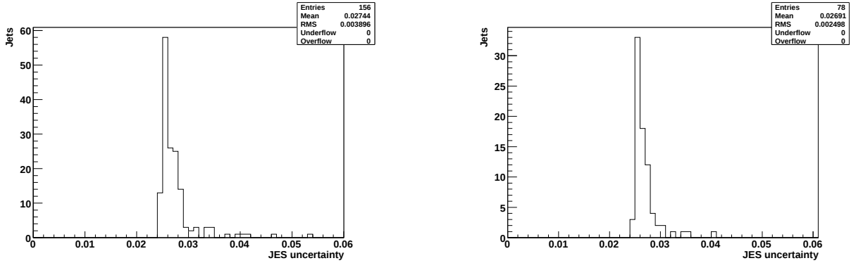
Figure G.1: Uncertainty on the default JES for the 156 light jets (left) and the corresponding 78 b-tagged jets (right) associated to the hadronic decay of a top quark in data.
