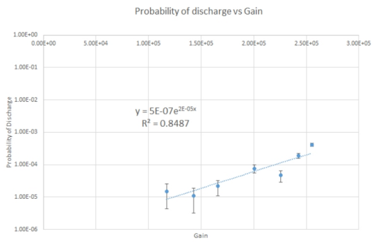
Figure 8: Probability of a Discharge as a function of the gain of the detector
