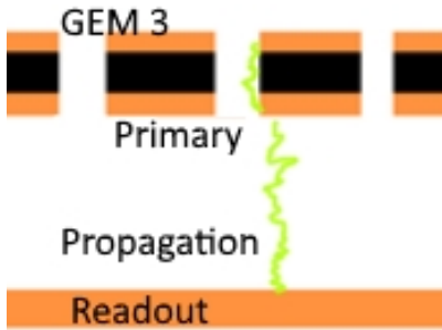
Figure 9: Sketch of a double discharge occurring in the detector showing the first discharge from GEM3 Top to GEM3 Bottom followed by a propagated discharge from GEM3 Bottom to the Readout
