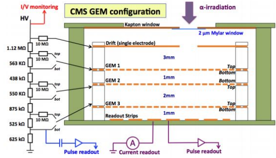
Figure 3: Diagram of the GEM detector showing the spacing and voltage divider circuit to cause the strong electric field. Figure from [1]
