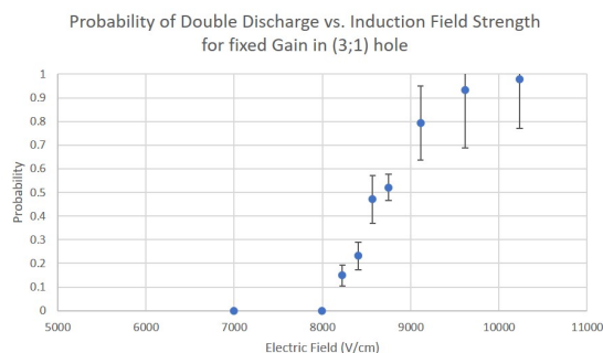
Figure 11: Double discharge propagation probability as a function of electric field strength at source location 3;1 along the edge of the detector
