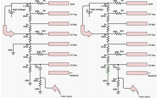
Figure 5: Circuit diagram of the two tests implemented to discover the problematic node. The first test (left) to see whether the issue was caused due to discharging between adjacent nodes or between GEM gaps, the second test (right) to determine if the issue was between a node and ground.
