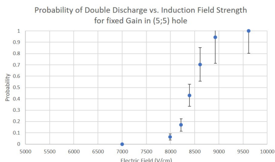
Figure 12: Double discharge propagation probability as a function of electric field strength at source location 5;5 at a corner of the detector
