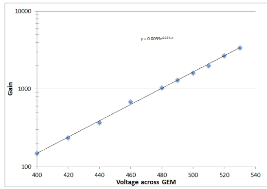
Figure 15: Gain as a function of voltage applied across a single GEM foil
