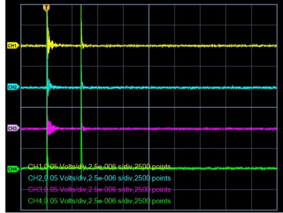
Figure 10: Screen capture of a double discharge viewed on a Tektronix 2024C oscilloscope showing all antenna channels
