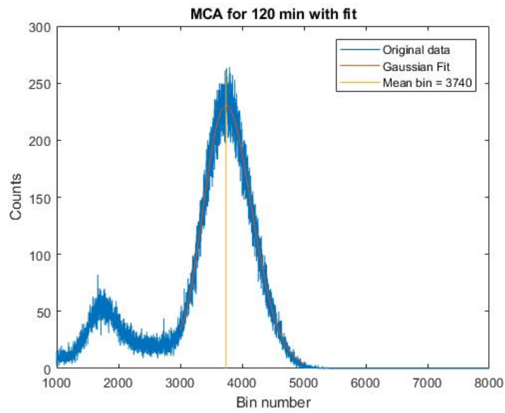
Figure 14: Example of an MCA plot with Gaussian fit applied to the main peak. This plot was taken from the analysis of the effect of charging up time vs. mean bin value. The two peaks correspond to the 5.9 keV ^{55}\text{Fe} X-ray and the \text{Ar} escape peak
