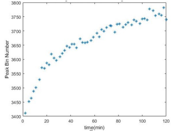
Figure 7: Mean MCA peak number as a function of time the detector has been exposed to the source. The cause for the increase in gain is known to be charge buildup as discussed in [1]
