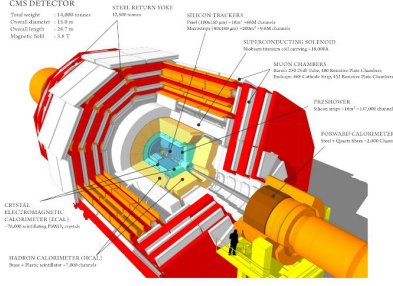
Figure 1: Diagram of the CMS Detector with the main areas labeled. Figure from [1]
