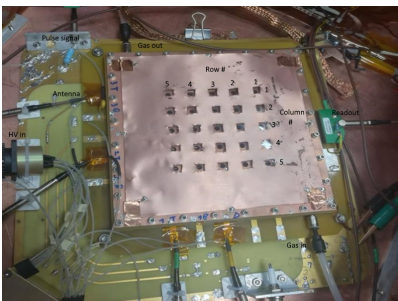
Figure 4: Picture of the 10x10 Prototype detector in the Faraday cage box. Source location numbering convention is labeled. Also pictured at the gas input and output, 4 antennas, readout, and high voltage input. Shown here is the multi-channel high voltage power supply set up
