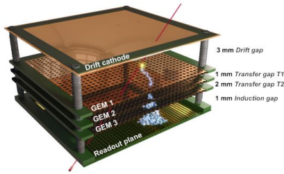
Figure 2: Schematic of the GEM detector showing a mock avalanche effect from an ionizing muon. Figure from [1]
