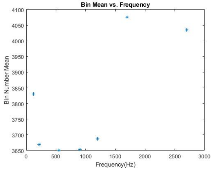
Figure 13: Results of the effect of frequency of the source on the mean bin number measured by MCA
