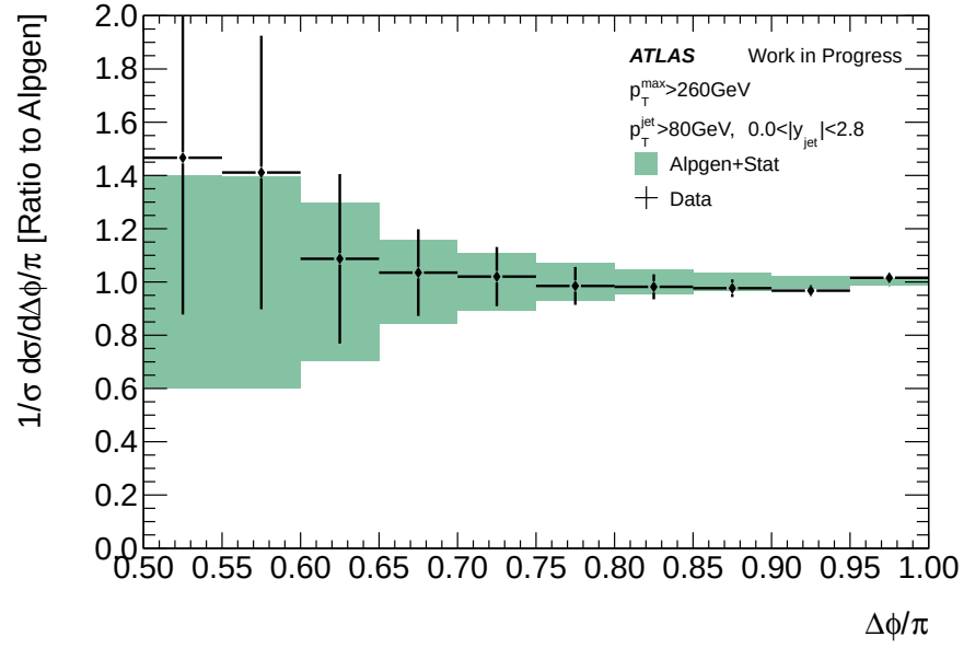
Figure 8.8: The closure test for data unfolded by Alpgen for dphi unfolding for p_T^{\max} bins 110 – 160 GeV, 160 – 210 GeV, 210 – 260 GeV, and > 260 GeV for each trigger selection.
