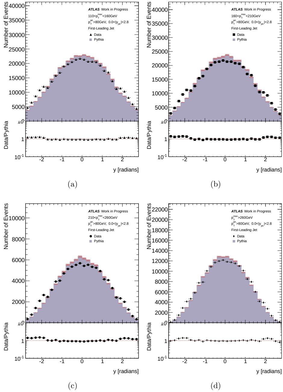
Figure 6.8: The y of the first-leading jet for p_T^{\max} bins 110 – 160 GeV, 160 – 210 GeV, 210 – 260 GeV, and > 260 GeV with statistical errors in hashed area.
