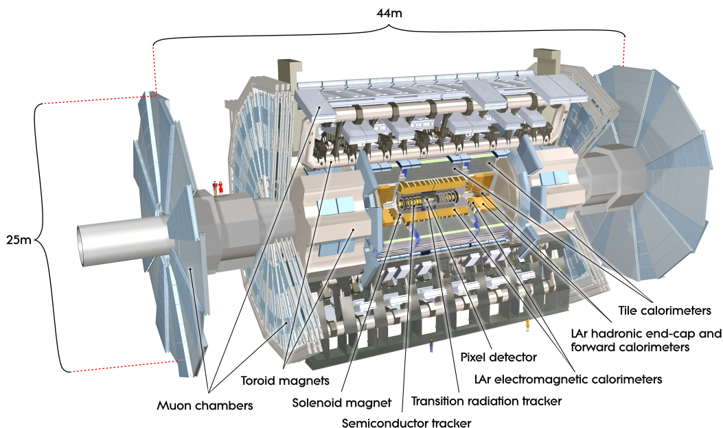
Figure 2.1: The ATLAS detector and its components. People are shown in figure to give scale.
