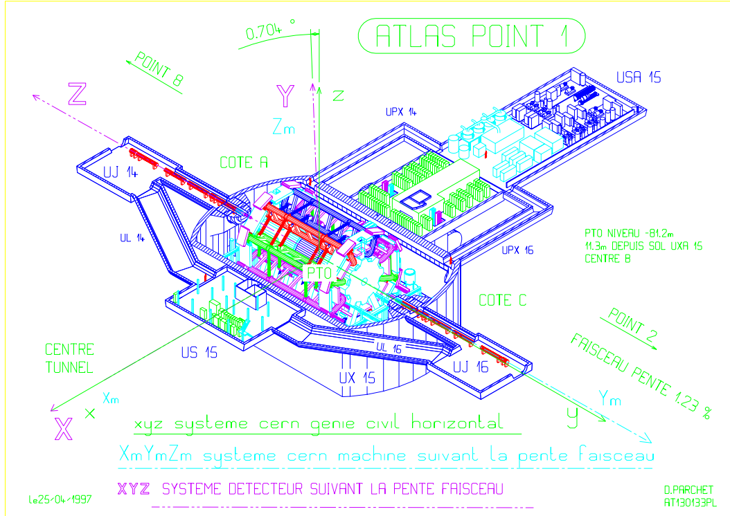
Figure 2.2: The coordinate system for the ATLAS detector.
