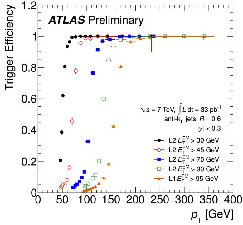
Figure 5.1: Combined L1+L2 jet trigger efficiency as a function of reconstructed jet p_T for anti-kt jets with R = 0.6 in the central region \Delta y < 0.3 shown for different L2 trigger thresholds. The trigger thresholds are at the electromagnetic scale, while the jet p_T is at the calibrated jet scale. The highest trigger chain does not apply a threshold at L2, so its L1 threshold is listed.
