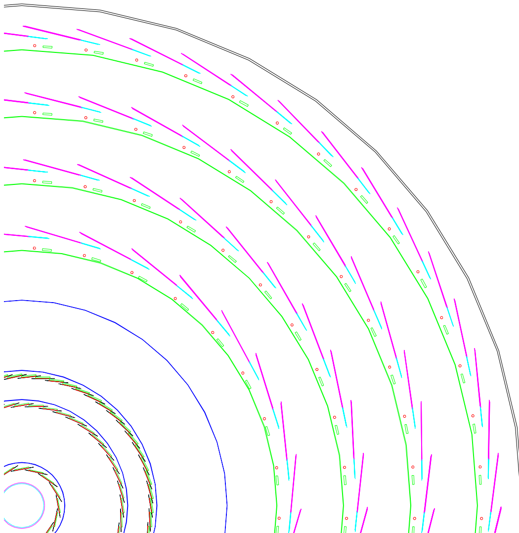
Figure 2.4: Transverse view of a quadrant of the ATLAS Inner Detector (precision layers only). From the center (lower left-hand corner) are: a) the beam pipe, b) three layers of the barrel pixel tracker: ladder support structure (green), silicon crystal (black) with the active regions (red) and support cylinders (dark blue), c) the overall cylindrical stiffener of the barrel pixel detector (dark blue), d) four layers of the SCT tracker: support (green), lumped power cables and cooling (red circles), active silicon (pink) and electronics boards (pale blue), and e) the SCTs insulating layer (black).
