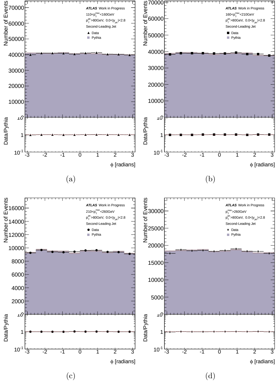
Figure 6.7: The \phi of the second-leading jet for p_T^{\max} bins 110 – 160 GeV, 160 – 210 GeV, 210 – 260 GeV, and > 260 GeV with statistical errors in hashed area.
