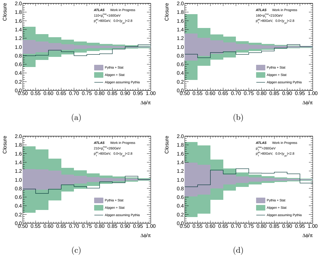
Figure 8.3: The closure test for \Delta\phi unfolding for p_T^{\text{max}} bins 110 - 160 \text{ GeV} , 160 - 210 \text{ GeV} , 210 - 260 \text{ GeV} , and > 260 \text{ GeV} for each trigger selection for Alpgen compared to Pythia.
