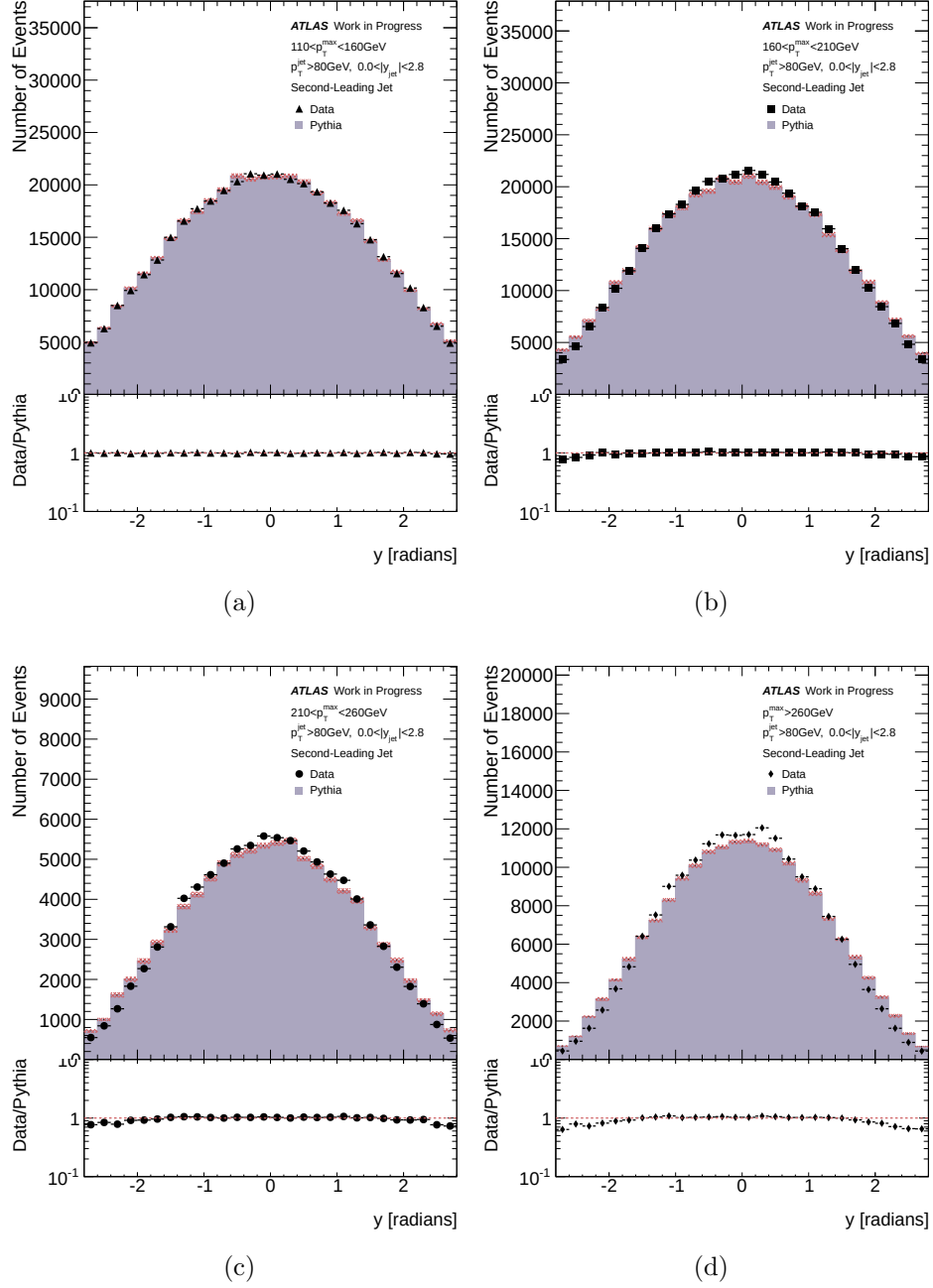
Figure 6.9: The y of the second-leading jet for p_T^{\max} bins 110 – 160 GeV, 160 – 210 GeV, 210 – 260 GeV, and > 260 GeV with statistical errors in hashed area.
