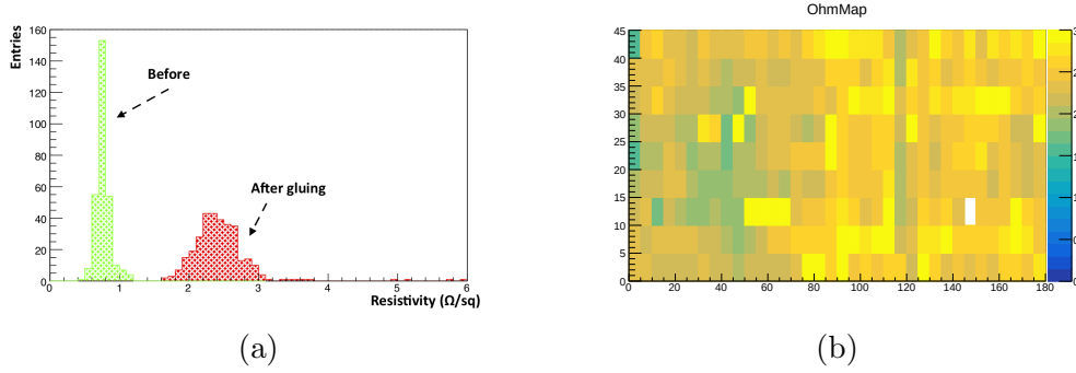
Figure 5.16: Distribution of the resistivity before and after the glueing of the resistive foil (a). Bi-dimensional map of the resistivity (b)
