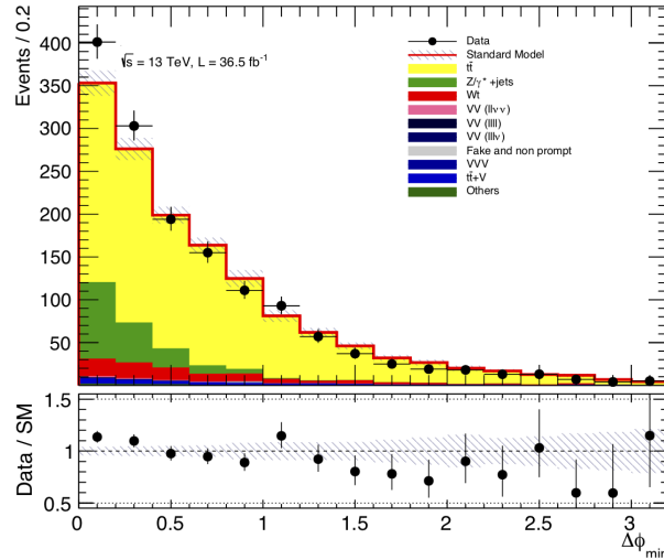
Figure 6.10: \Delta\phi_{min} distribution
