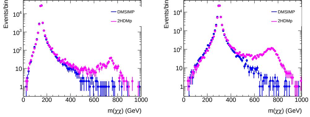
Figure 6.27: Invariant mass of the dark matter pair for both models when m(a)=150 GeV (a) and m(a)=300 GeV are used
