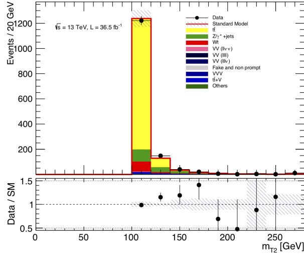
Figure 6.8: Stranverse mass ( m_{T2} ) distribution
