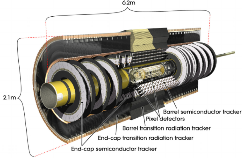
Figure 2.4: The ATLAS inner detector layout.
