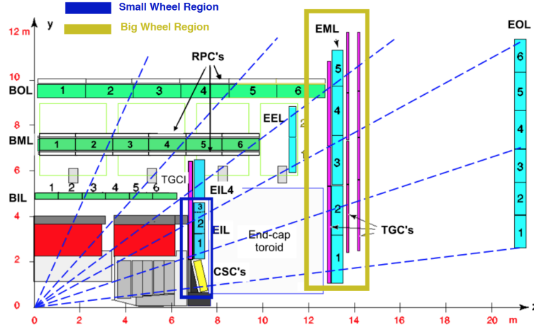
Figure 2.8: Longitudinal view of the muon spectrometer showing the three concentric stations at different distance ( 5, 8, 10 meters) from the interaction point. The innermost wheel, the so called Small Wheel, is outlined
