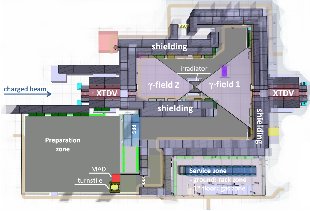
Figure B.2: Layout of the bunker
