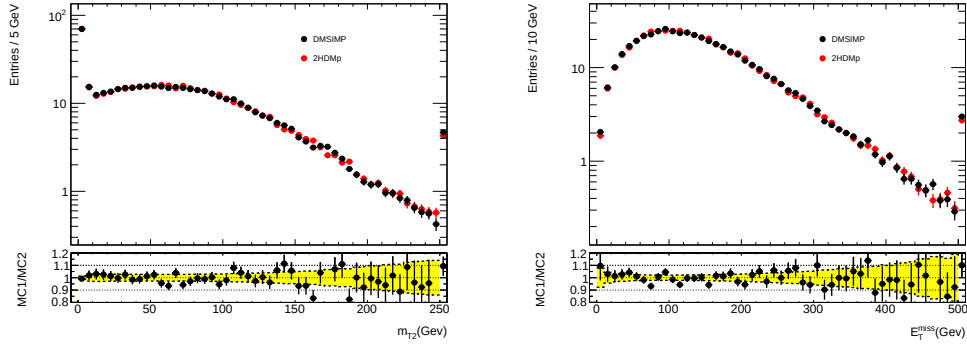
Figure 6.28: Comparison of the distributions of the variables M_{T2} , E_T^{\text{miss}} for the DMSIMP model (black points) and 2HDMa model (red points). The distributions are obtained for m(a) = 150 GeV, and the 2HDMa distributions contain events passing the m(\chi\chi) < 200 GeV requirement.
