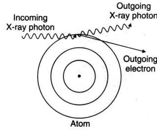
Figure A.5: Scheme of the Compton scattering.
