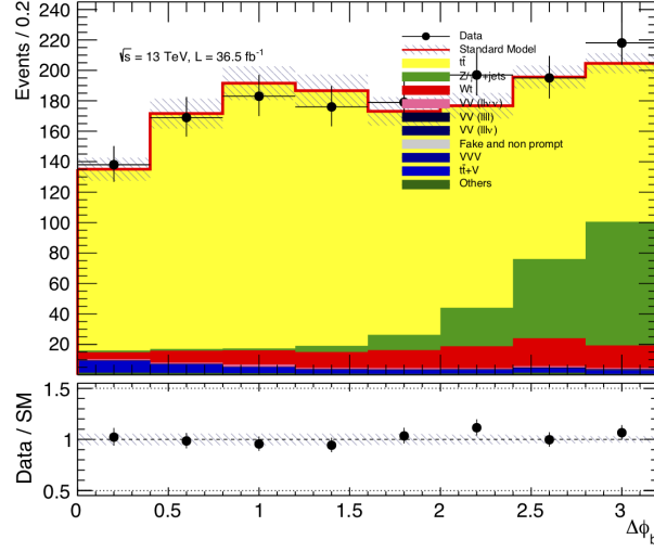
Figure 6.9: \Delta\phi_b distribution
