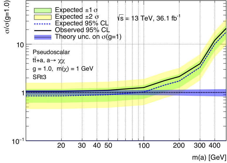
Figure 6.24: Model dependent limit for the pseudoscalar mediator models as a function of the mediator mass and with a fixed DM mass of 1 GeV. All systematic uncertainties and NLO k-factors are included.
