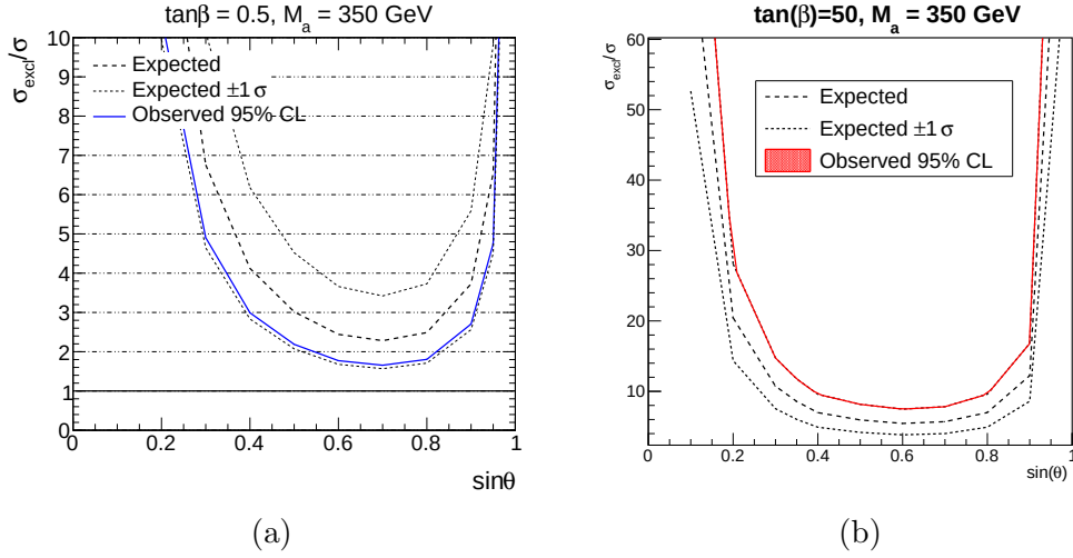
Figure 6.33: Interpretation of the results for the t\bar{t}\chi\bar{\chi} final state (left) and the b\bar{b}\chi\bar{\chi} final state (right) as a function of \sin\theta for M_a = 350 GeV. For the t\bar{t}\chi\bar{\chi} final state the signal region providing the best expected sensitivity is used
