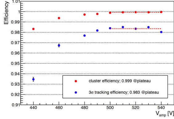
Figure C.8: Cluster efficiency as a function of the amplification field. The red points show the efficiency when clusters are selected in the whole detector: the plateau reaches about the 99.9%. The blue points represent the efficiency obtained by selecting clusters lying closer than 3 times the resolution of the accurate coordinate ( 3\sigma ) from the expected position. In this case, the plateau reaches the 98%.
