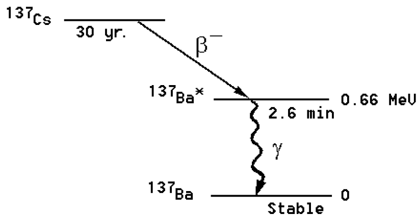
Figure B.1: ^{137}\text{Cs} decay
