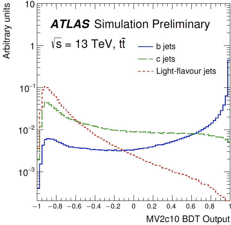
Figure 6.6: BDT MV2c10 output for b-jets, c-jets and light flavour jets
