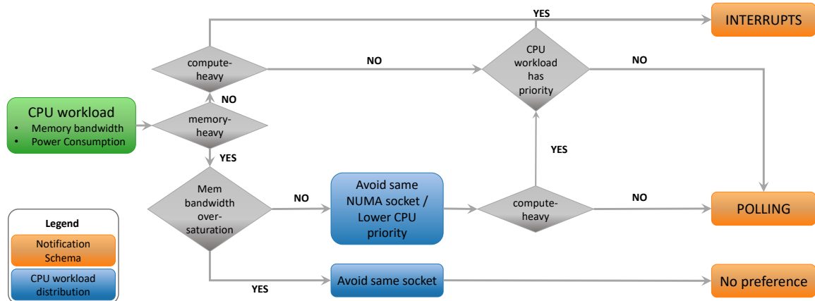
Fig. 5.4 Co-Scheduling Policy
