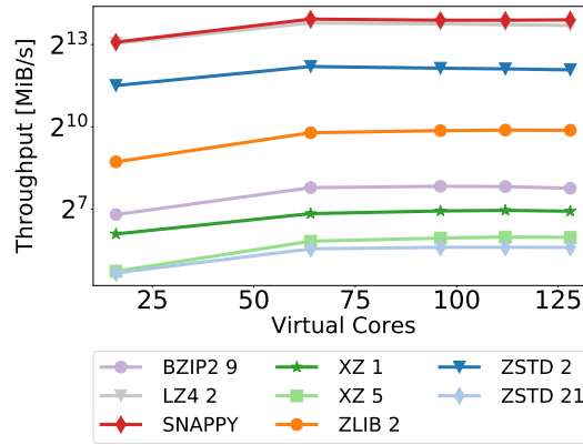
Fig. 4.5 Performance of different compression algorithms for IBM. The performance variance is greatly reduced after SMT4 (= 64 cores).
