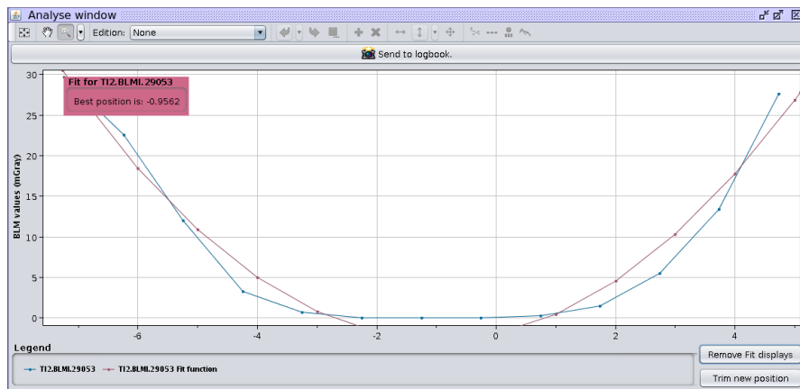
Figure 7.3 – Screen-shot of the operational tool used for the TCDI automatic alignment.
