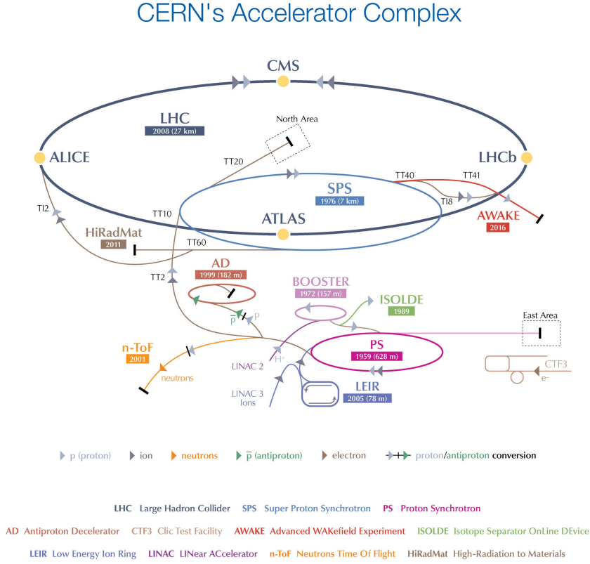
Figure 3.1 – The CERN accelerator complex.
