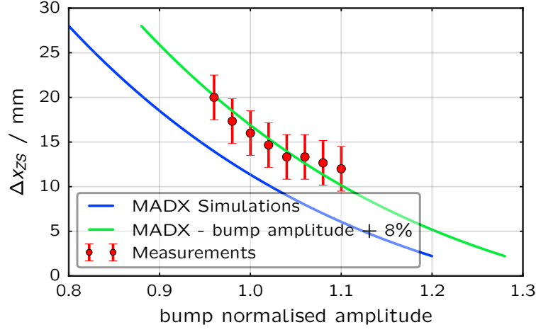
Figure 6.9 – Evolution of the spiral step as a function of the bump amplitude. In blue the spiral step is plotted in case of ideal machine. In red dots the measurements recorded during 2016 slow extraction commissioning are plotted. The case with a bump 8 % larger than theoretically estimated is shown in green.
