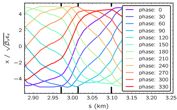
Figure 7.4 – Example of normalised trajectories used for the TCDI validation procedure (TI2 horizontal). The horizontal collimator longitudinal positions are sketched in black.
