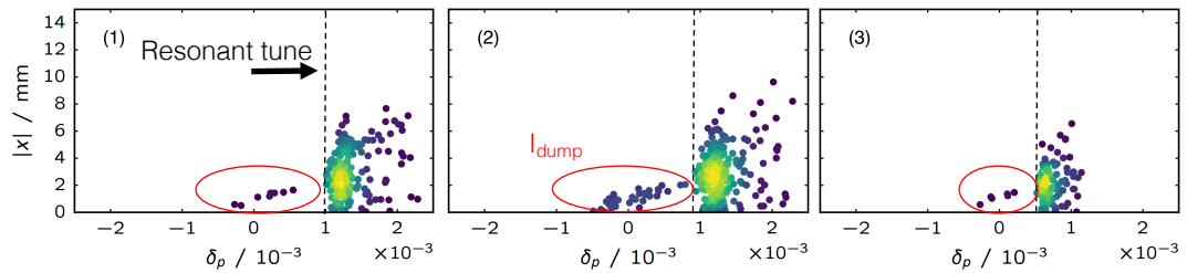
Figure 6.10 – Simulated Steinbach plot, at almost 70 % of the extraction process, for the three case of Table 6.1: 1) SPS FT, 2) SHiP 1 and 3) SHiP 2.
