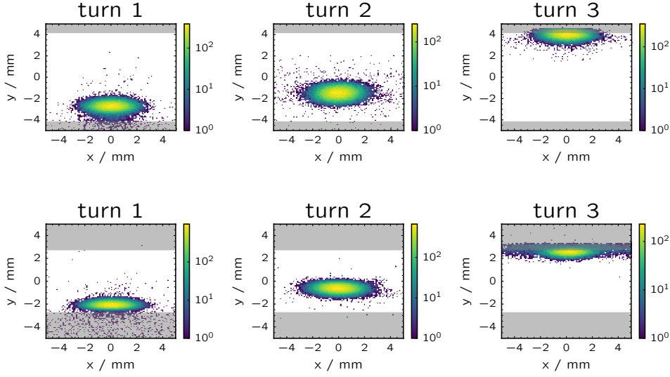
Figure 7.20 – Transverse particle distribution of B1 (top) and B2 (bottom) at the TCLIB in case of MKI flashover for 3 turns.
