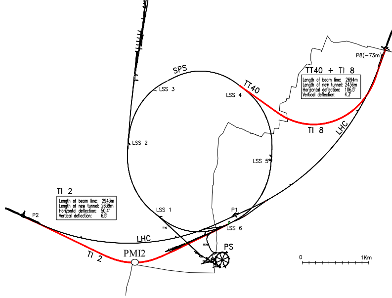
Figure 3.12 – View of the SPS and its TLs to the LHC [16].
