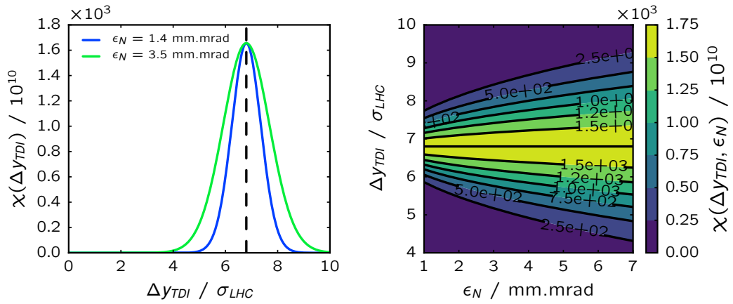
Figure 7.18 – Plots of the analytical relation between intensity of the maximum amplitude surviving the TDI and deflection induced by the MKI for different beam emittances.
