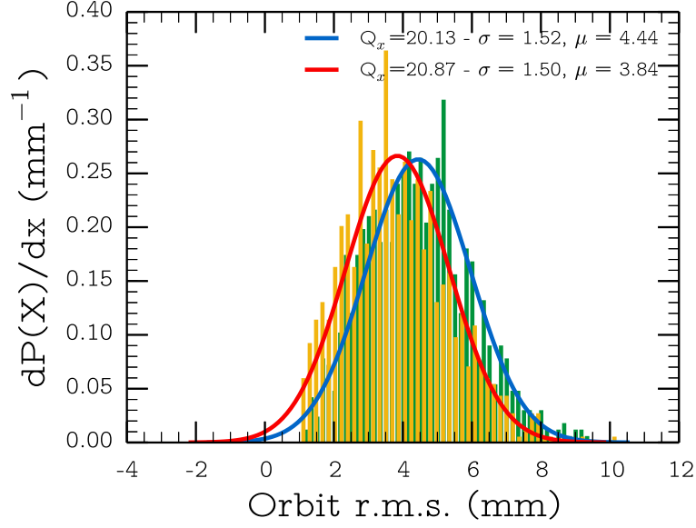
Figure 4.4 – Calculated horizontal r.m.s. orbit distributions obtained misaligning all the quadrupoles in the SPS with MAD-X. Green: \nu_x = 20.13 . Yellow: \nu_x = 20.87 .
