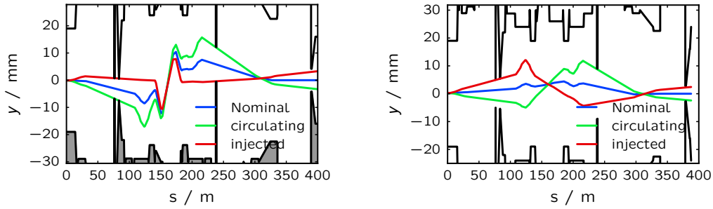
Figure 7.13 – Grazing trajectories of B1 (left) and B2 (right) for k_{MKI} equal to 11% and 9.5% for B1 and B2, respectively. The blue line represent the nominal closed orbit. The green line represents the beam trajectory, in case of failure of the MKI acting on the circulating beam. The red line represents the beam trajectory, in case of failure of the MKI acting on the injected beam.
