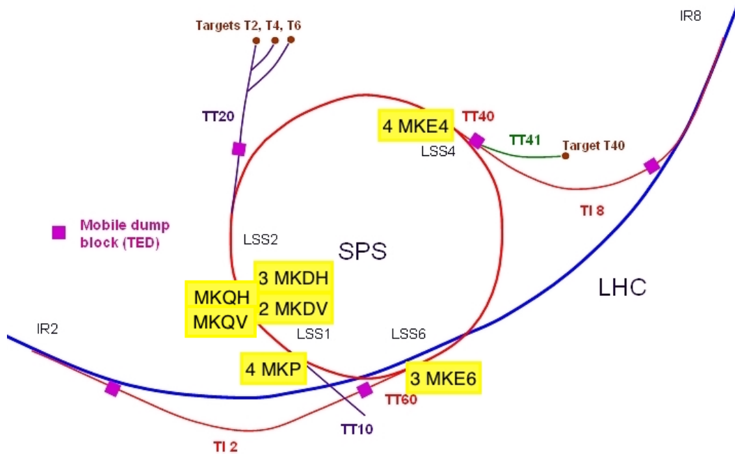
Figure 4.1 – Overview of the all SPS kickers. The MKPs are the injection kickers, the MKQV/H are the tune kickers, the MKDV/H are the dump kickers and the MKEs are the extraction kickers [ Courtesy of M. Barnes ].
