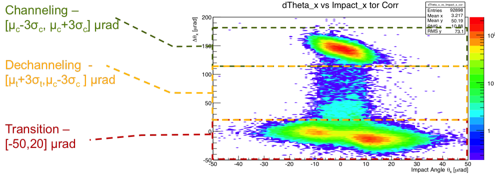
Figure 5.3 – 2D histogram of the deflection angle of the crystal as function of the impacting angle [33].
