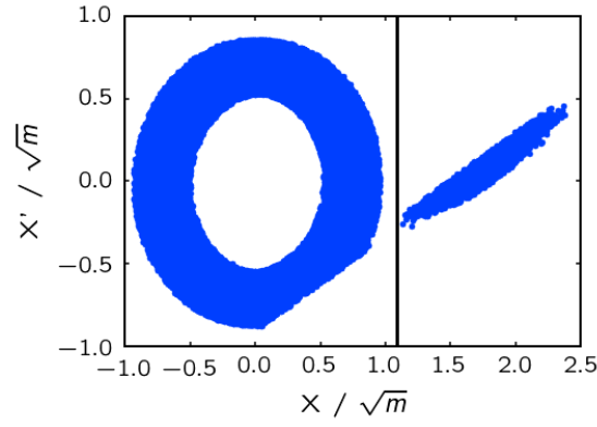
Figure 5.8 – Beam halo at the ZS in LSS2 after deflection at the crystal in LSS5 for an optimal phase advance crystal-ZS.
