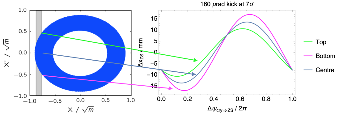
Figure 5.7 – Displacement from the beam centre, at the ZS, for the different parts of the channelled beamlet as a function of the phase advance crystal-ZS. A uniform hollow distribution between 5\sigma and 8\sigma is shown.
