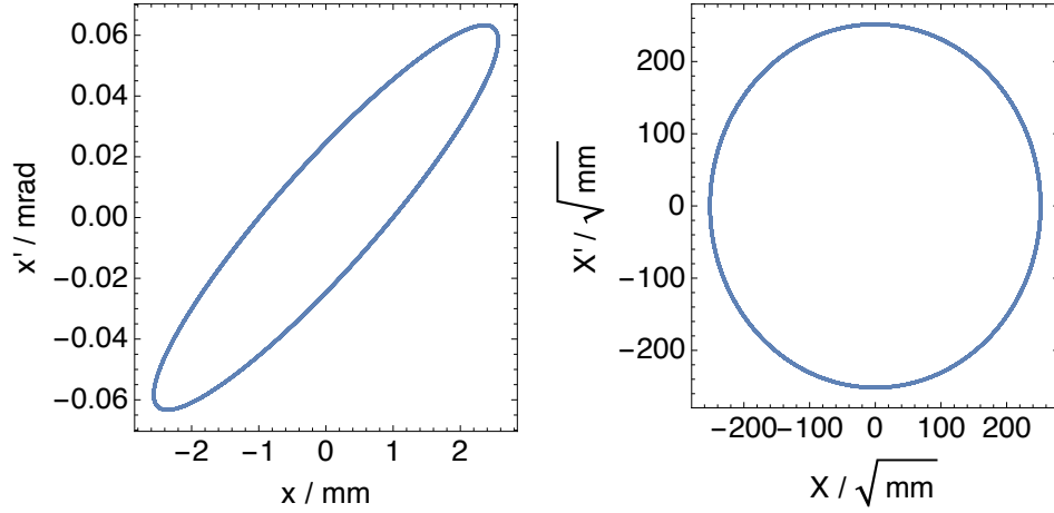
Figure 2.3 – Trace-space (left) compared with normalised phase-space (right).
