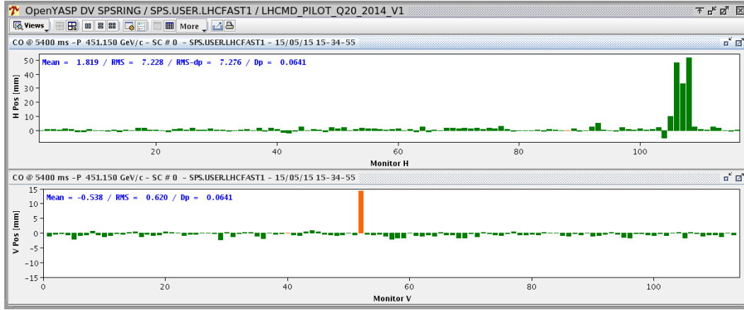
Figure 4.16 – Screen-shot of the SPS steering application showing the closed orbit just before extraction. The CO is shown as difference with respect to the nominal one, in order to evaluate the bump shape and its closure.
