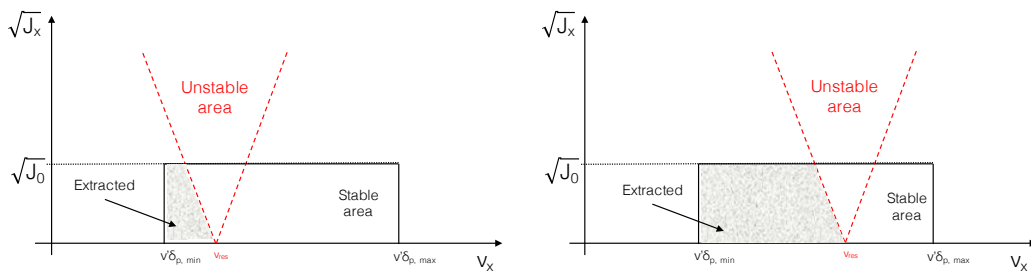
Figure 3.9 – Stainbach diagram of a slow extraction where the machine tune is changed to drive particles unstable.
