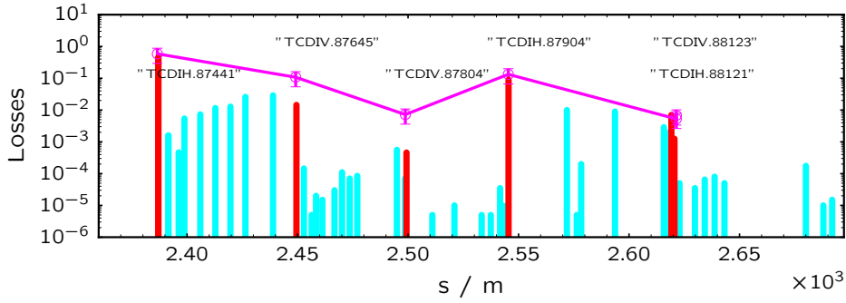
Figure 7.8 – Example of simulated TL loss map. The two different histograms (red and cyan) in the loss map refer to two different kind of losses: the red ones refer to protons that have undergone to an inelastic scattering inside the collimator jaws, the cyan ones refer to protons lost inside the machine elements that are not collimators. In magenta the BLM readings expressed in particle lost.
