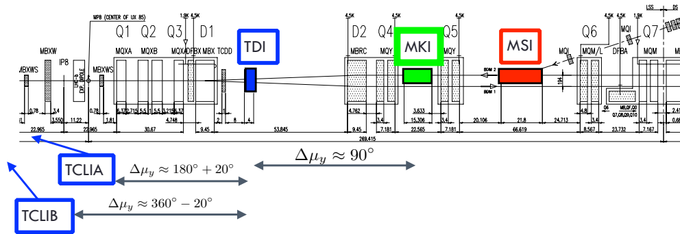
Figure 7.11 – Schematic representation of the LHC injection system [16].
