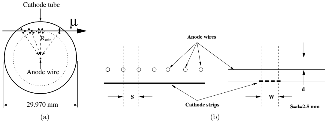
Figure 2.2.9: Precision track position measurement with ATLAS Muon system. Monitored Drift Tube (a) and Cathode-Strip Chambers (b) [56].
