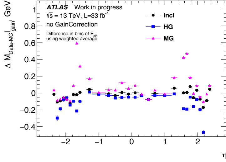
Figure 4.1.7: Difference of invariant mass distribution \Delta m_{ee}^{Data-MC} between Data and MC at \sqrt{s} = 13 TeV, as a function of the pseudorapidity of the electron, for the two gain categories. The Medium gain category is presented with pink points, the High gain category in blue, and the inclusive distributions in black.
