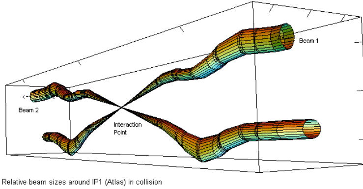
Figure 2.1.3: The beams squeezed down to 64 \mu\text{m} before the interaction point to increase the chances of a collision, providing in average about 23 interactions per bunch crossing.
