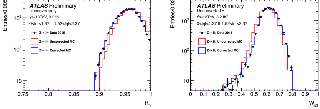
Figure 3.2.3: Two examples of shower-shape variables for unconverted photons: the black points are for the photons from Z \rightarrow l^+l^-\gamma events from data, the red histogram for the photons from Z \rightarrow l^+l^-\gamma event from simulation before applying the shift, and the blue histogram after applying the shift [91].
