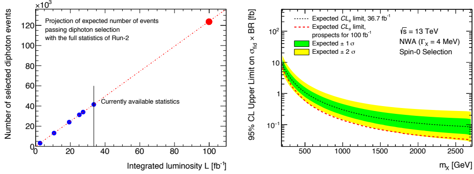
Figure 5.9.3: Left: The scaled number of selected diphoton events as a function of the integrated luminosity. Right: Expected limit on the fiducial production cross-section \sigma_{\text{fid}} as a function of the resonance mass m_X for NWA signal presented in black line for current available statistics, and in red presented projection to 100fb ^{-1} .
