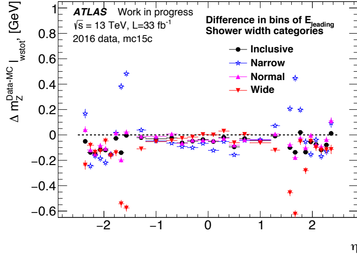
Figure 4.1.11: Difference of invariant mass distribution \Delta m_{ee}^{Data-MC} between Data and MC at \sqrt{s} = 13 TeV, as a function of pseudorapidity of the electron for lateral shower width categories.
