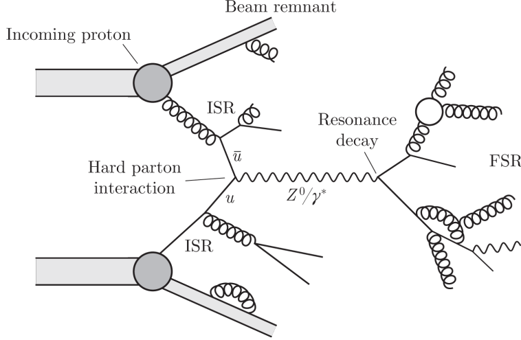
Figure 1.2.1: Schematic representation of a proton-proton hard scattering process [19].
