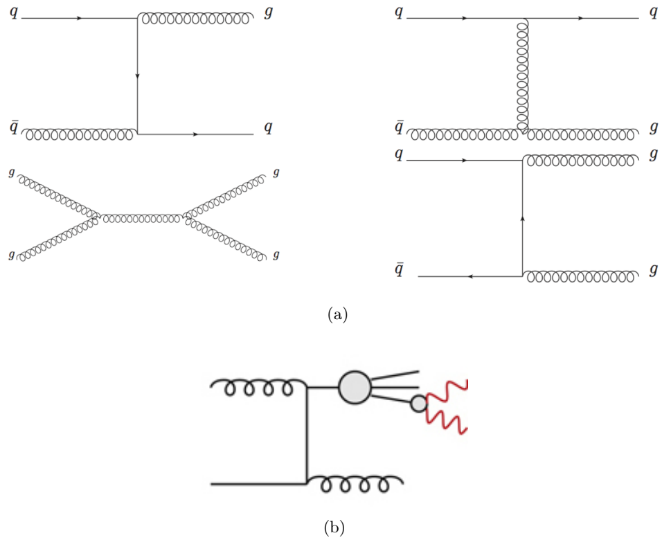
Figure 3.0.2: Feynman diagrams presenting fake photons. a) Diagrams of various processes where quark or gluon initiated jet can be misidentified as a photon, b) photons coming from the decay of the light hadrons.
