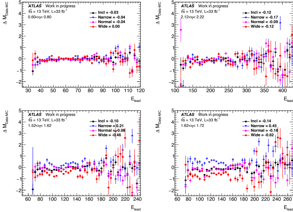
Figure 4.1.10: The difference of invariant mass distribution for Data and MC as a function of energy for categories of the lateral shower width ( \omega_{\text{stot}} ). Top plots presents barrel ( 0.6 < \eta < 0.8 ) and far endcap ( 2.12 < \eta < 2.22 ) bins, the bottom plots correspond to "bad" region.
