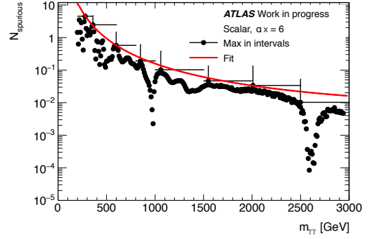
Figure 5.5.2: Result of the spurious signal test for \alpha_X = 6\% . The N_{\text{spurious}} parametrised as a function of diphoton mass, using maximum value in interval over m_{\gamma\gamma} .
