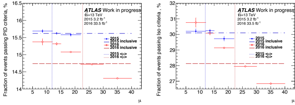
Figure 5.2.3: Distribution of the fraction of events passing the tight photon identification selection cut (left) and for the tight isolation cut (right) as a function of the average number of pile-up events, in blue for 2015 data and in red for 2016 data. The horizontal lines represent the inclusive fractions of selected events and the vertical line represent the average number of pile-up events for each year.
