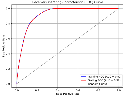
FIG. 2: Receiver Operating Characteristic (ROC) curve. In our case, the value of the Area Under the Curve (AUC) indicates that the ability of the model to distinguish between signal and background is acceptable (above 0.9).
