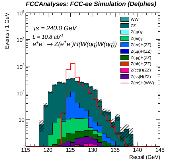
FIG. 7: Recoil mass of the Z(ee) after selections, with background contributions stacked. The solid red line represents the corresponding signal (not stacked with background).
