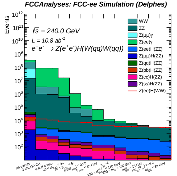
FIG. 5: Cut Flow for the process Z(ee)H, H \rightarrow W^+(qq)W^-(qq) . The filled histograms represent each of the contributing backgrounds (stacked), while the solid red line represents the yield for the signal (not stacked with background).
