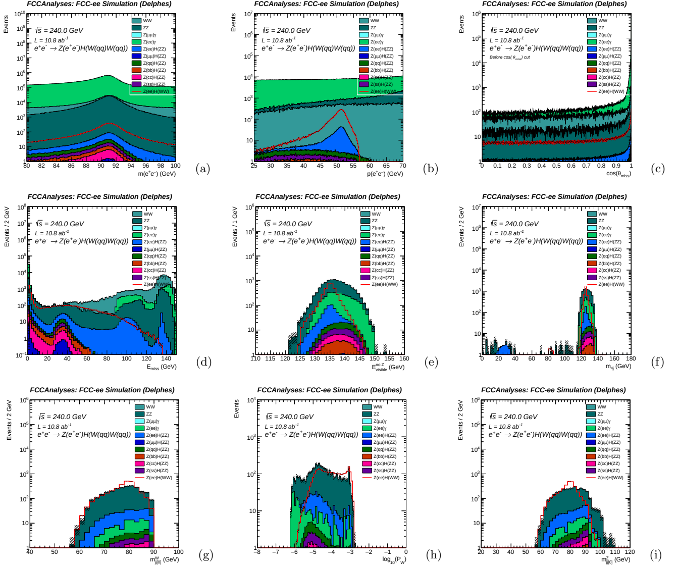
FIG. 9: Distributions for the Z(ee) events prior their respective cuts, where a) is the distribution of m_{ee} , b) p_{ee} , c) |\cos\theta_{miss}| , d) the missing energy ( E_{miss} ), e) the visible energy of the particles excluding the Z muons, f) the four-jet invariant mass, g) the off-shell-W dijet invariant mass, h) the \log_{10}P_W (see Eq. 5) and i) is the invariant mass of the dijet pair chosen around the mass of the Z boson.
