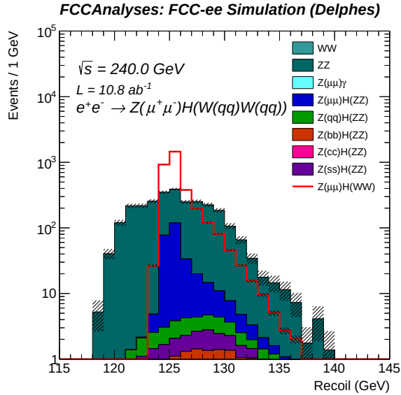
FIG. 6: Recoil mass of the Z(\mu\mu) for this analysis, each with background contributions stacked, while the solid red line represents the yield for the signal (not stacked with background).
