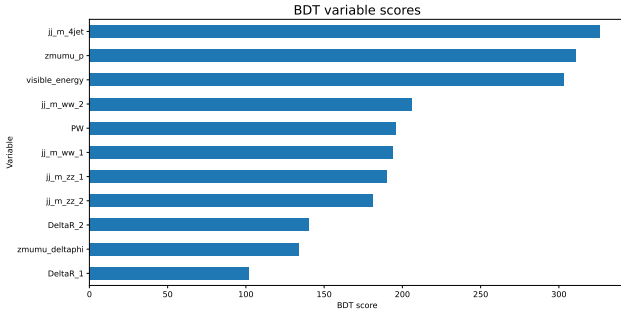
FIG. 1: Scores for each of the features chosen for the classifier in the BDT training. A higher score suggests that the variable is more valuable for classification purposes.
