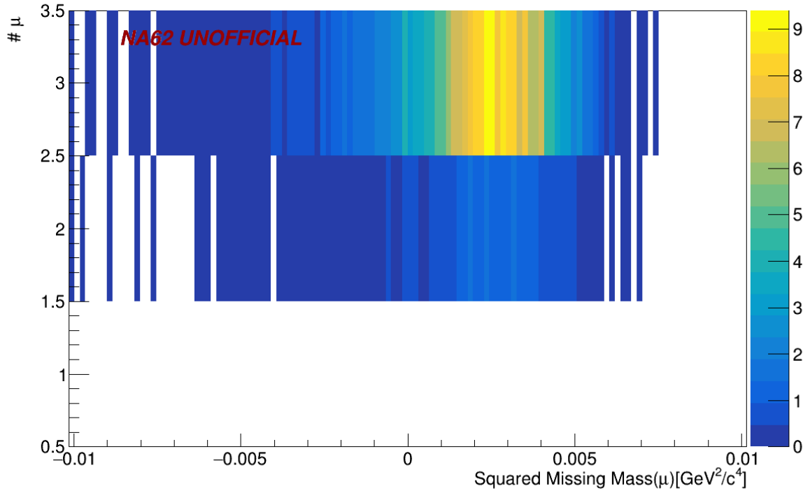
Figure 4.14: Number of muon in final state ( \# \mu ) or number of early decays versus m_{miss}^2(K_{\mu\nu\mu\mu}) for the K_{3\pi} Fast Capped MC sample. Each event contributes to the plot with the weight provided by the MC.
