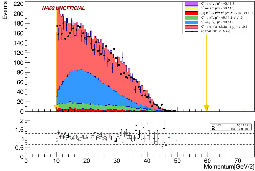
Figure 4.21: Straw tracks momentum for K_{\mu\nu\mu\mu} events before the final m^2_{miss} cut. The arrows mark the momentum cut applied during the Common selection.
