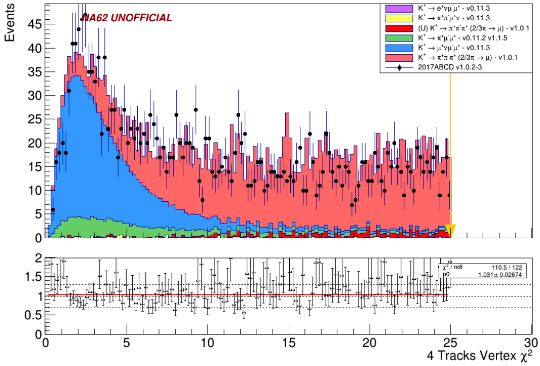
Figure 4.29: Four tracks vertex \chi^2 for K_{\nu\mu\mu} events before the final m_{miss}^2 cut. The arrow indicates the four tracks vertex \chi^2 cut applied during the Common selection.
