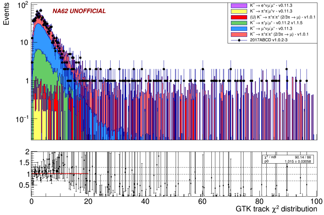
Figure 4.27: GTK track \chi^2 for K_{\mu\nu\mu\mu} events before the final m^2_{miss} cut
