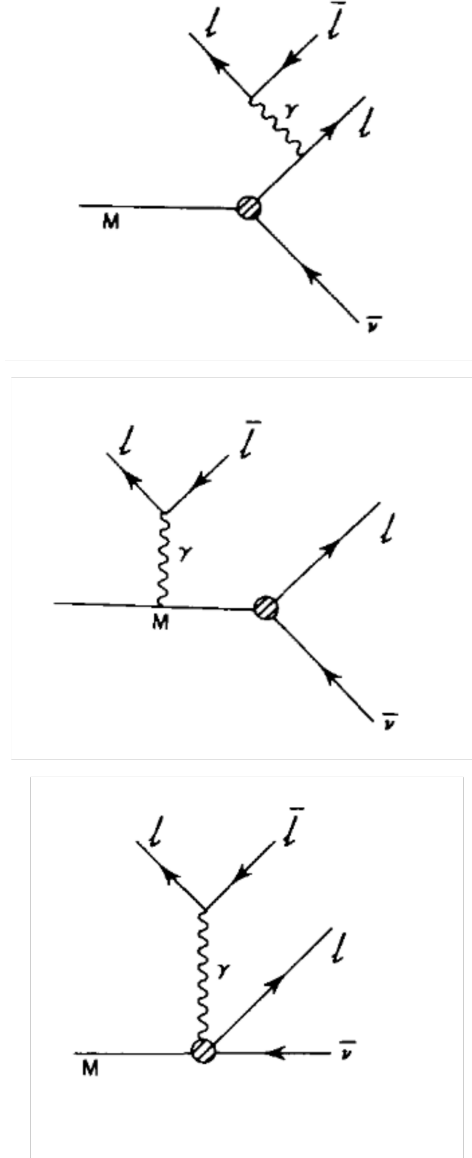
Figure 1.2: Feynmann diagrams for the Inner Bremsstrahlung (IB) and Structure Dependent (SD) contributions to M \rightarrow l \nu l \bar{l} decays[9].
