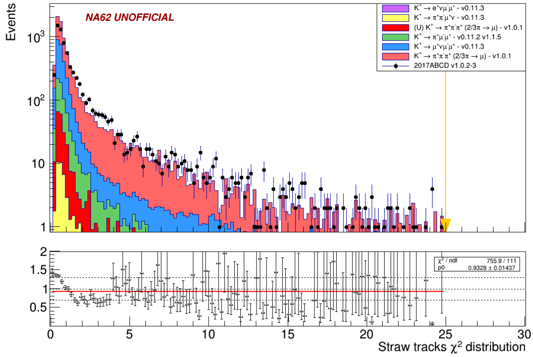
Figure 4.23: Straw tracks \chi^2 for K_{\mu\nu\mu\mu} events before the final m_{miss}^2 cut. The arrow marks the track \chi^2 cut applied during the Common selection.
