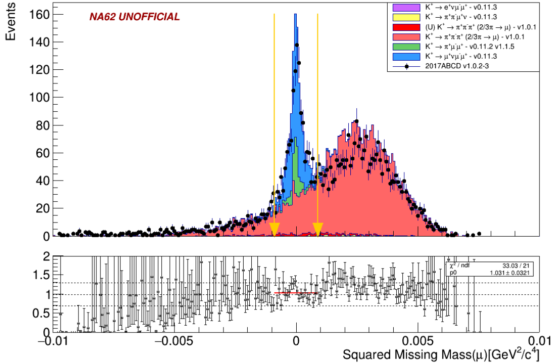
Figure 4.13: The K_{\mu\nu\mu\mu} final plot shows the squared missing mass spectrum for data and MC normalised on K_{\pi\mu\mu} . The two arrows border the standard signal region: [-0.0009, 0.0009] GeV 2 /c 4 . The K_{\mu\nu\mu\mu} MC has been normalised with the theoretical BR value.
