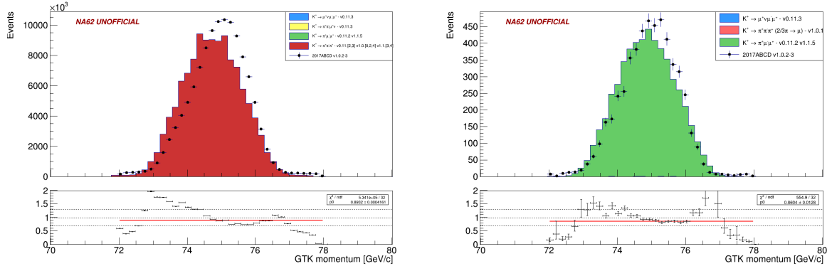
Figure 4.24: GTK tracks momentum for events passing the K_{3\pi} (left) and K_{\pi\mu\mu} (right) event selections.
