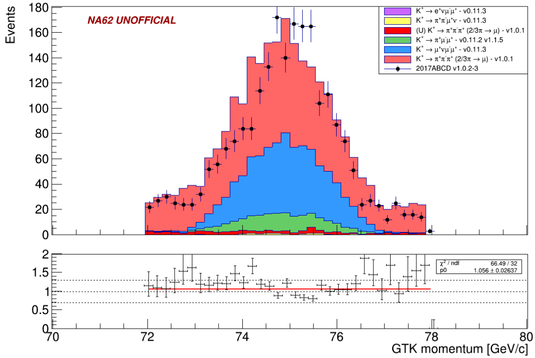
Figure 4.25: GTK track momentum for K_{\mu\nu\mu\mu} events before the final m^2_{miss} cut.
