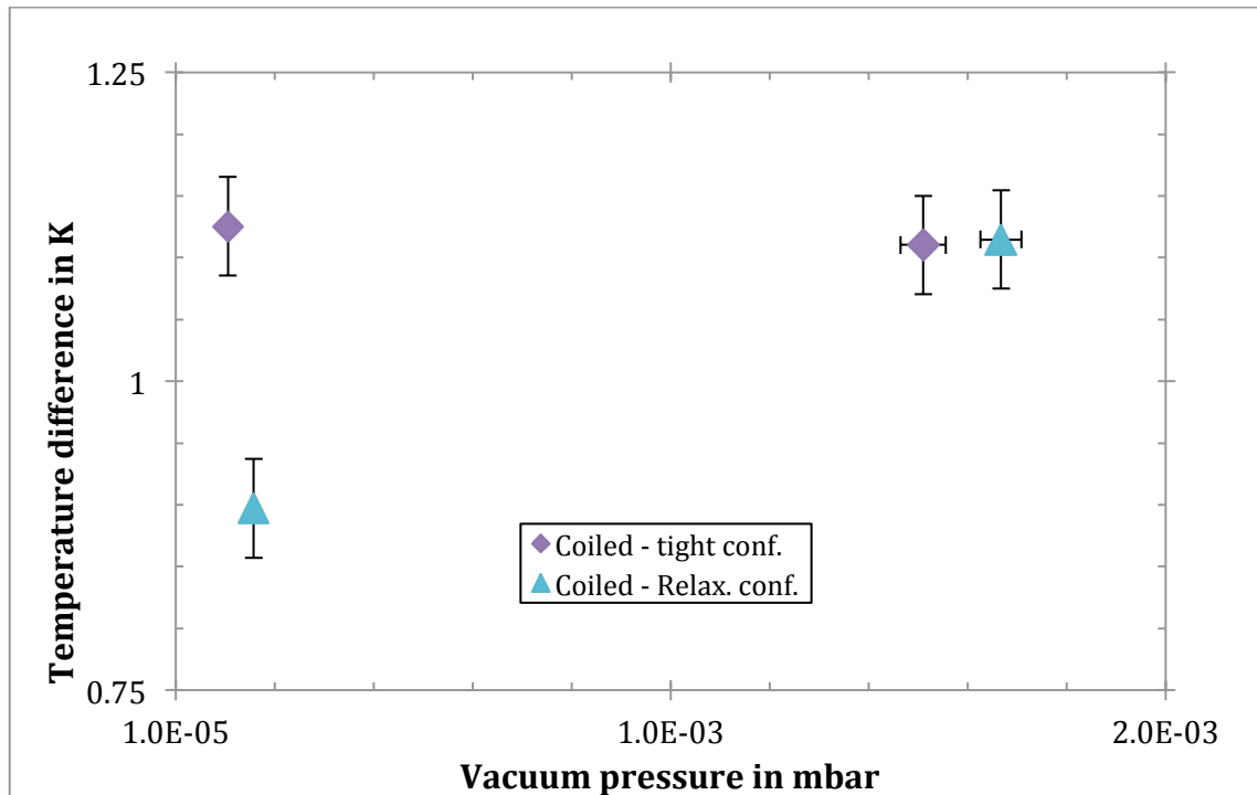
Figure 7-10 Temperature difference between outlet and inlet temperature measured in coiled - tight and coiled - relaxed configuration of the transfer line at different vacuum pressures.
