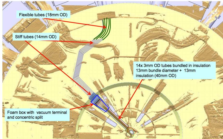
Figure 2-3 Routing of the transfer lines at side A of Inner Detector Endplate. [4]
