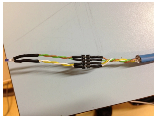
Figure 6-5 PT100 sensor used for the measurement of the surface and the ambient temperatures
