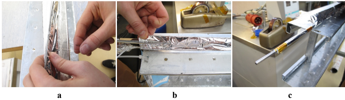
Figure 5-3 Process of the multi-layer insulation installation; a) sewing of the MLI; b) cutting off the excess of the MLI; c) MLI taped with Kapton tape;
