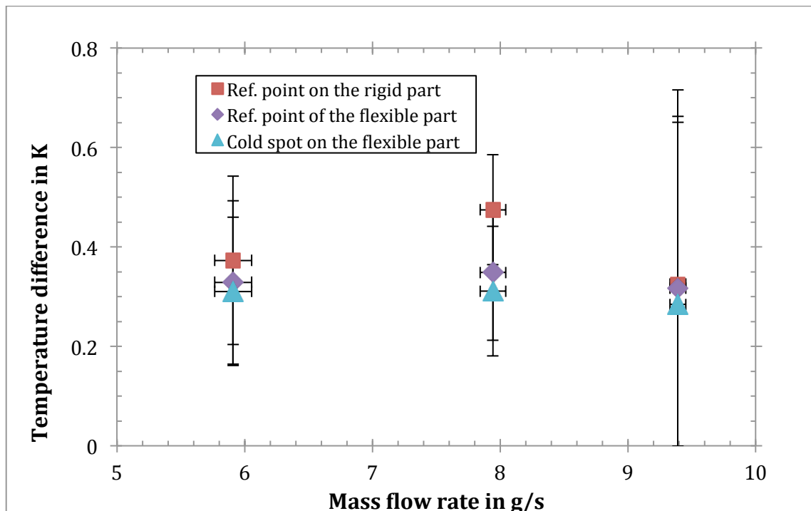
Figure 7-3 Temperature difference between ambient and surface temperature measured on the rigid and flexible part of the transfer line in straight configuration with different mass flow rates with the coolant temperature measured at the inlet = -40^{\circ}\text{C} .
