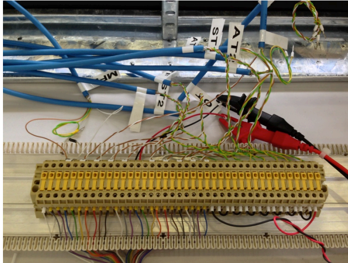
Figure 6-2 Terminals connecting cables from sensors with multimeter.
