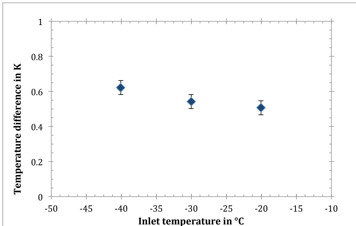
Figure 7-4 Temperature difference between inlet and outlet depending on the temperature of the coolant at the inlet with mass flow rate = 6 g/s.
