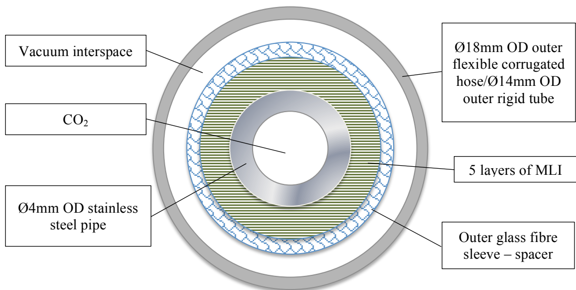
Figure 5-1 Design of the transfer line.
