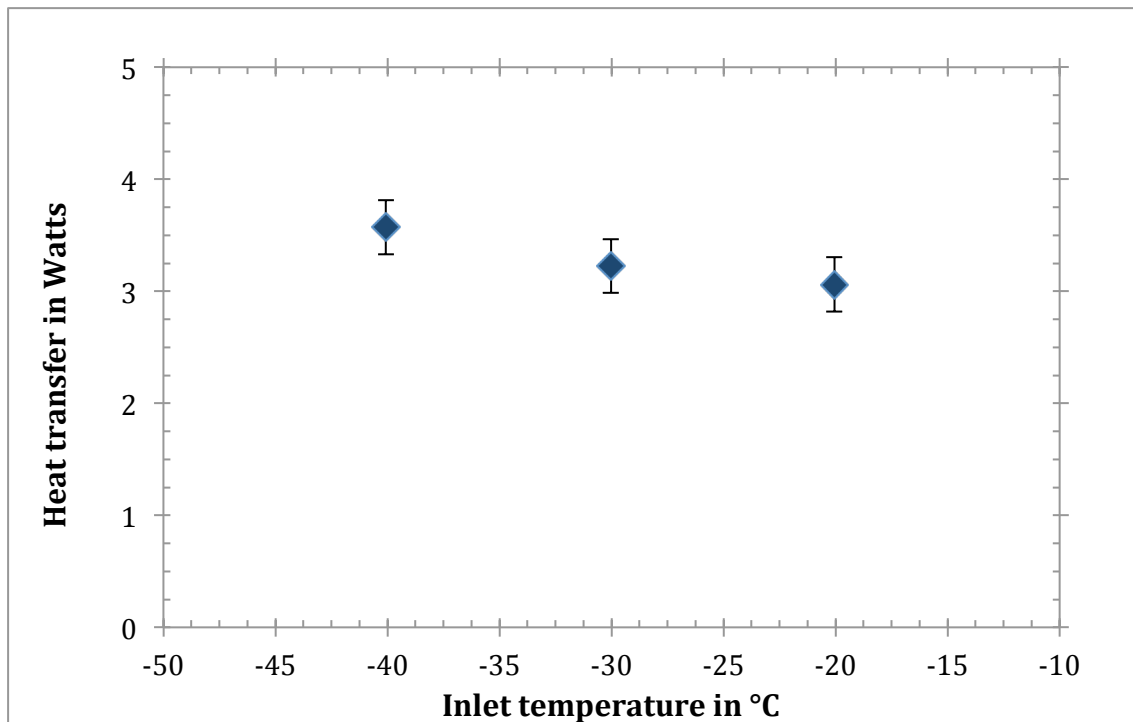
Figure 7-5 Heat transfer depending on the coolant temperature at the inlet of the transfer line during the measurement in straight configuration with mass flow rate = 6 g/s.
