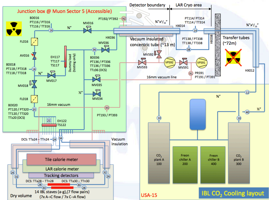
Figure 2-2 P&I of the IBL CO 2 cooling transfer and evaporator system [3].
