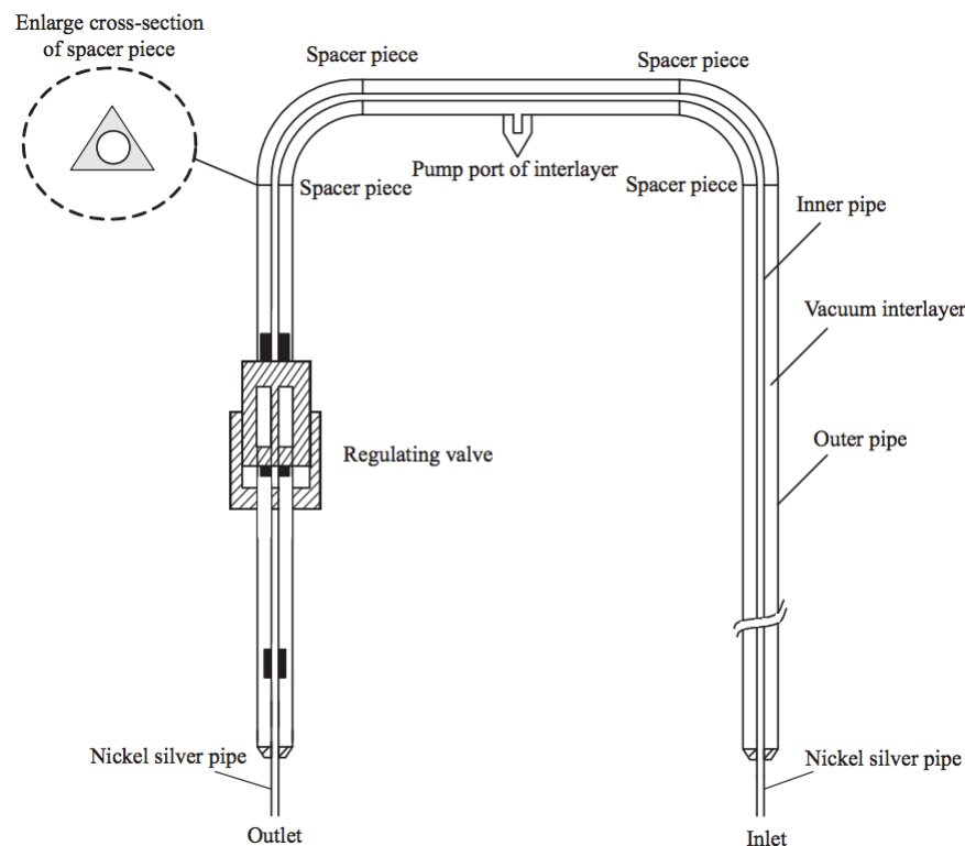
Figure 4-1 Components of a cryogenic transfer line [5].
