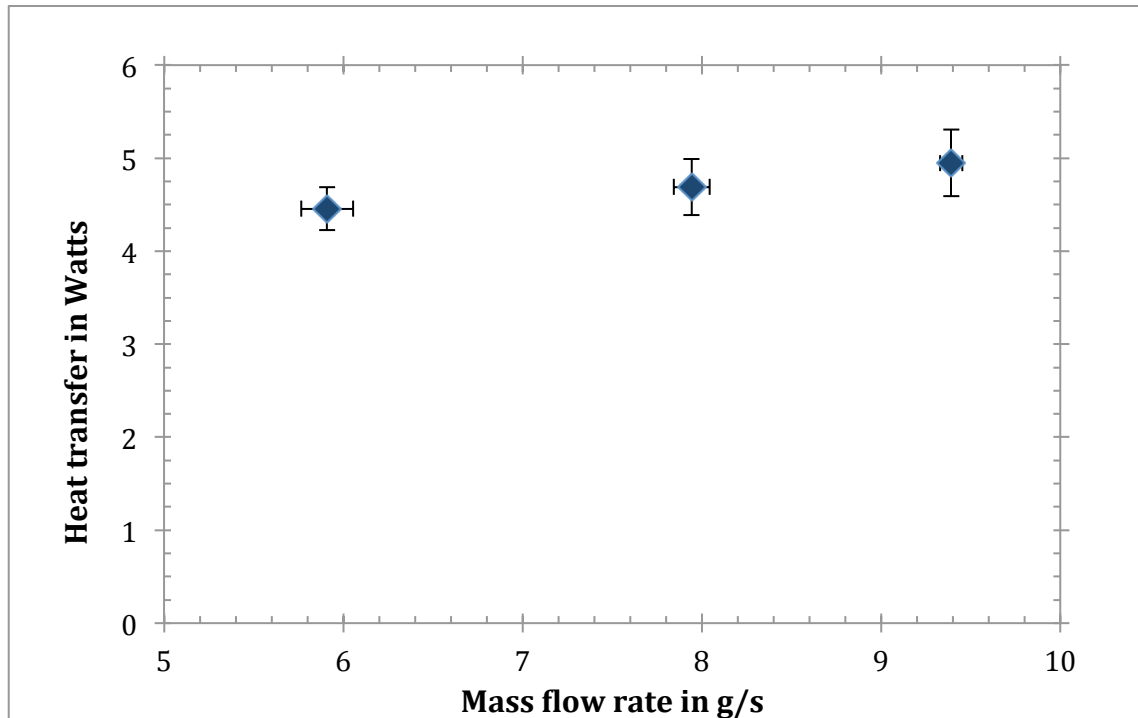
Figure 7-2 Heat transfer depending on mass flow rate during the measurement in straight configuration of the transfer line with the coolant temperature measured at the inlet = -40^{\circ}\text{C} .
