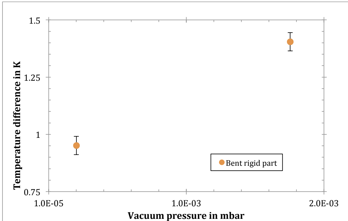
Figure 7-13 Temperature difference between outlet and inlet of the transfer line measured after the bending of the rigid part of the transfer line at different vacuum pressures with the coolant temperature measured at the inlet = -40^{\circ}\text{C} .
