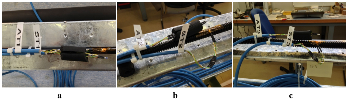
Figure 6-18 Temperature sensors installed on the transfer line used for the ambient and the surface temperature measurements; a) temperature sensors pair no. 1 installed on the reference point of the rigid part of the transfer line; b) temperature sensors pair no. 2 installed on the reference point of the flexible part of the transfer line; c) temperature sensors pair no. 3 installed on the cold spot on the flexible part of the transfer line;
