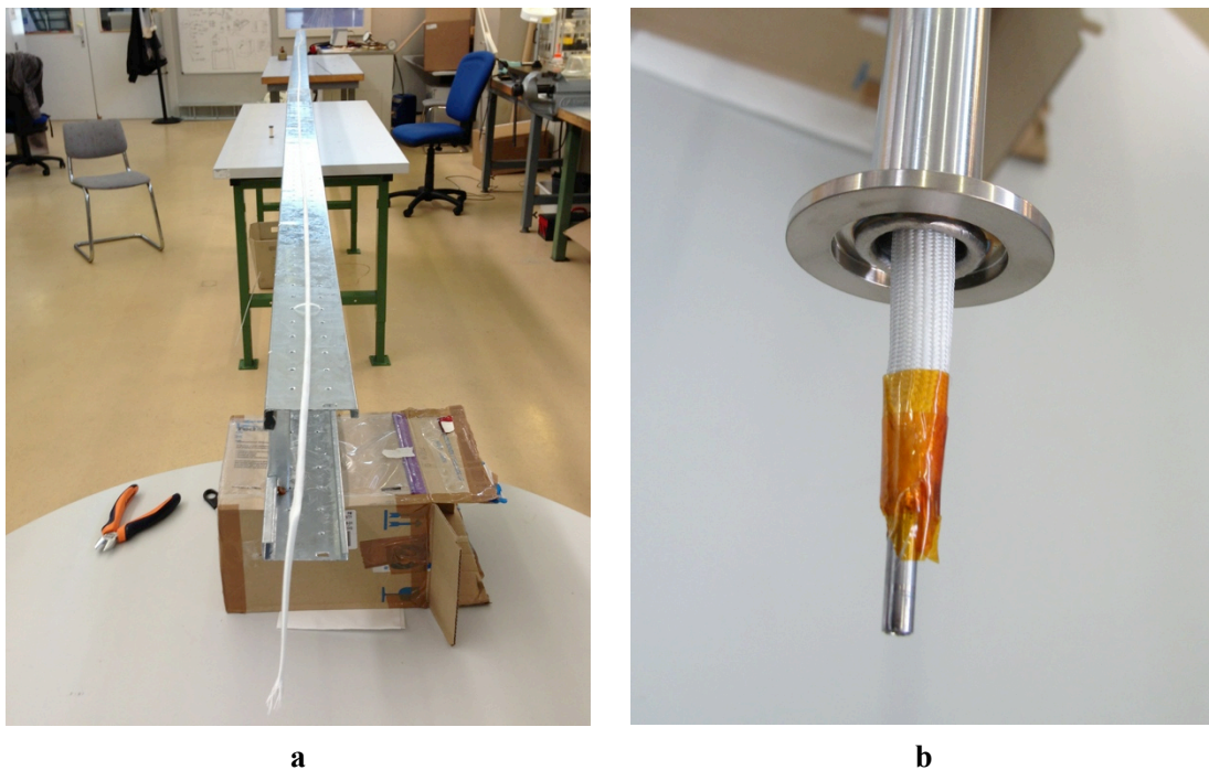
Figure 5-4 Inner tube with MLI and the spacer; a) spacer pulled over the entire length of the inner tube; b) end of the inner tube with MLI and the spacer
