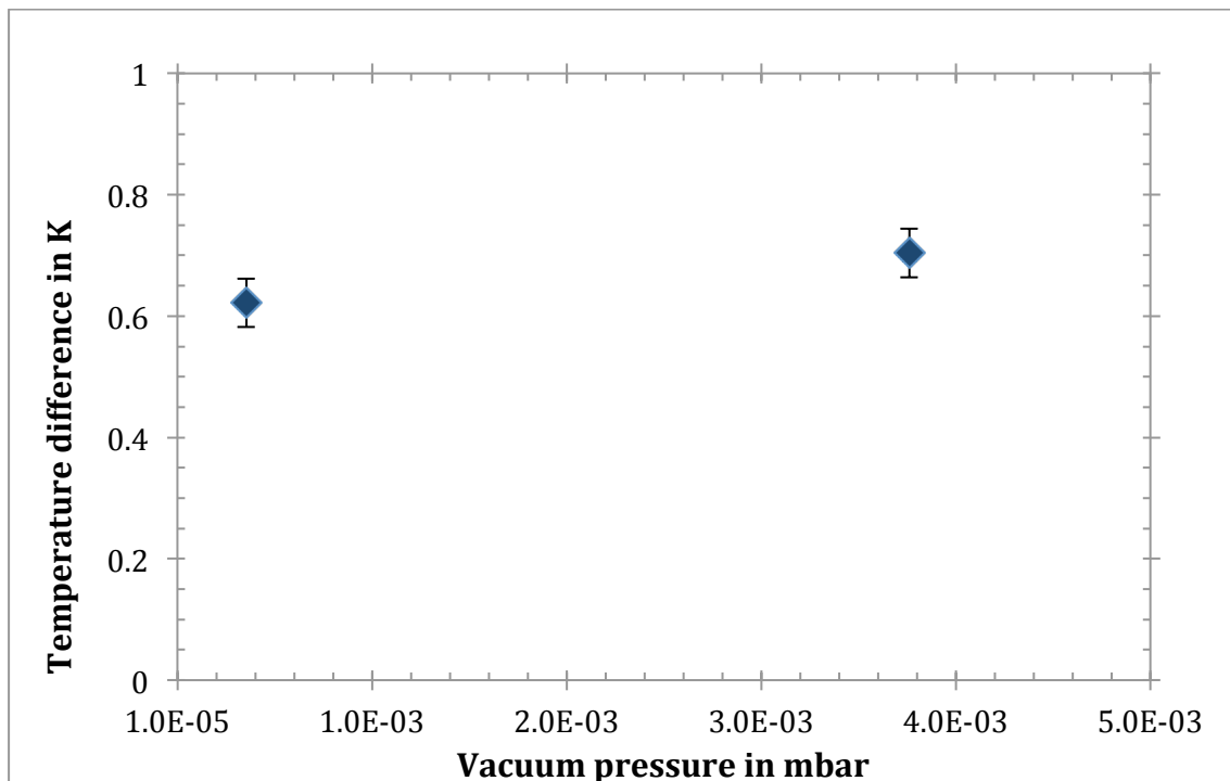
Figure 7-7 Temperature difference between inlet and outlet depending on vacuum pressure during the measurement in straight configuration with the coolant temperature measured at the inlet = -40°C.
