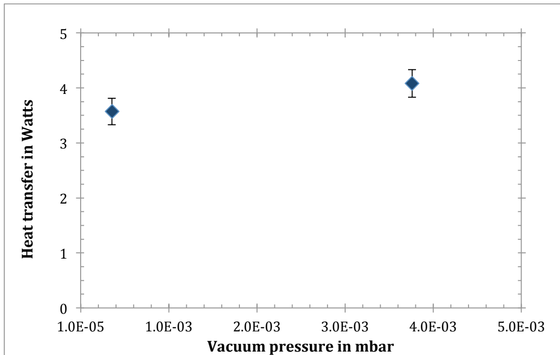
Figure 7-8 Heat transfer depending on vacuum pressure during the measurement in straight configuration with the coolant temperature measured at the inlet = -40°C.
