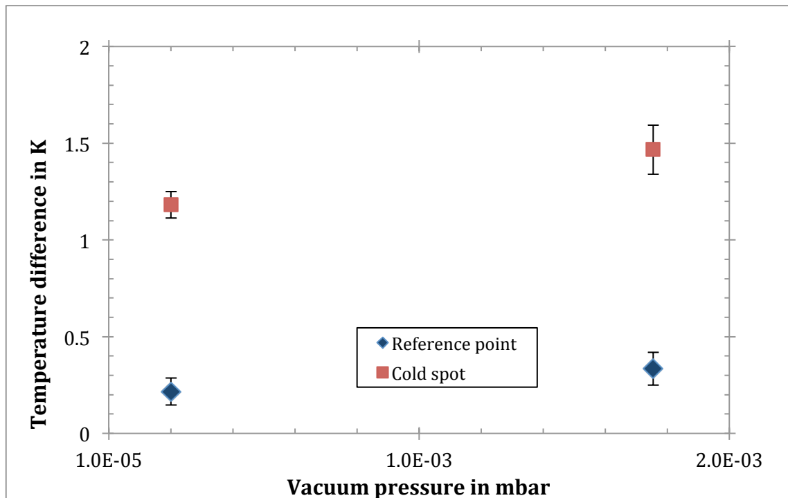
Figure 7-15 Temperature difference between ambient and surface temperature measured on the rigid part of the transfer after bending of it at different vacuum pressures.
