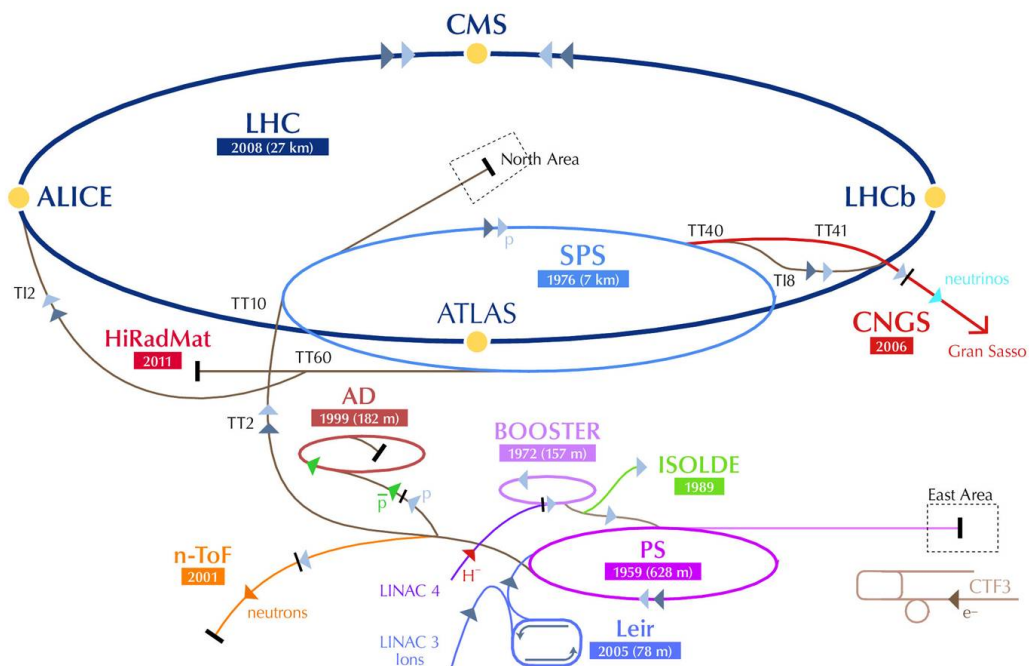
Figure 2-1 Schematic of CERN accelerator complex with four experiments on LHC [1].
