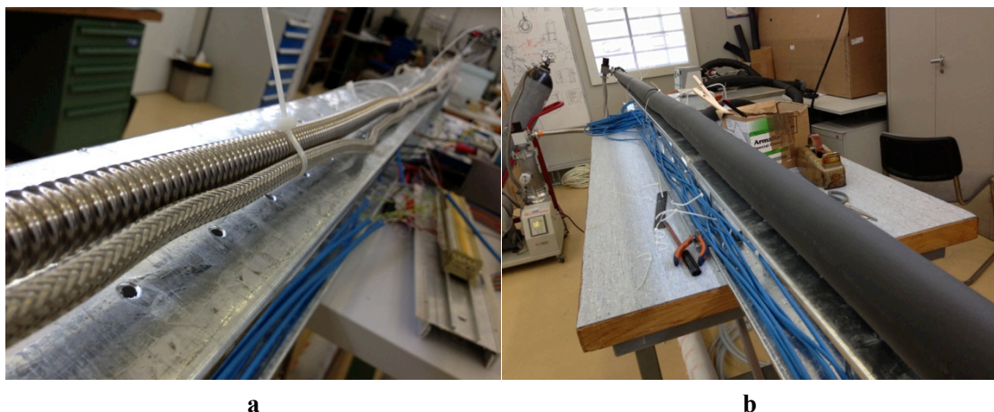
Figure 6-13 Transfer line before the bake-out; a) heating cable attached to the transfer line; b) transfer line before the bake-out insulated with Armaflex;
