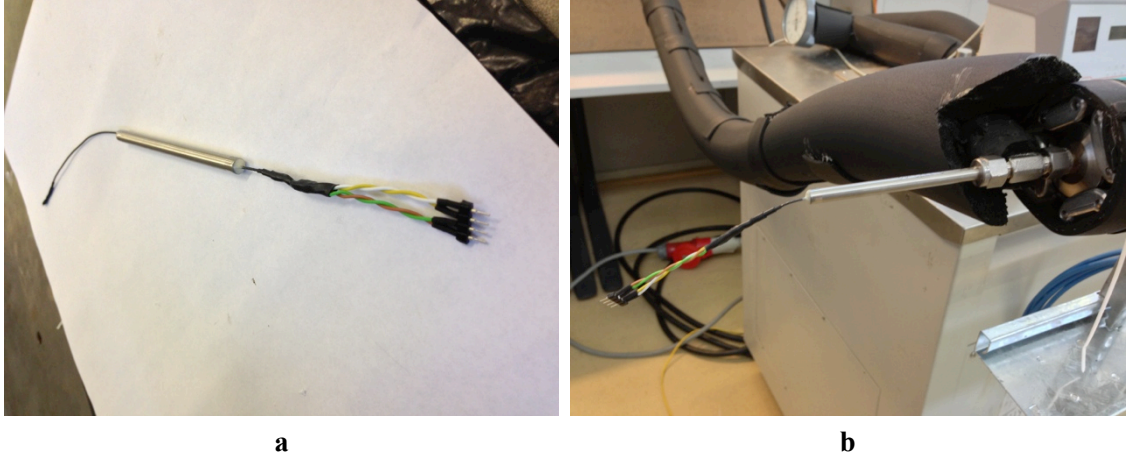
Figure 6-4 PT100 temperature sensor used at the inlet of the transfer line; a) sensor after manufacturing – tip of the sensor is in the top-left corner of the picture; b) sensor installed at the inlet of the transfer line;
