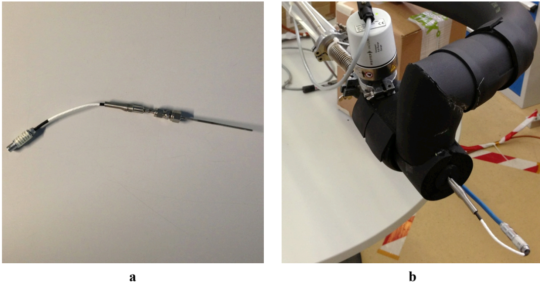
Figure 6-6 PT100 temperature sensor used to measure coolant temperature at the outlet of the transfer line; a) sensor after the measurement with Swagelok components on it; b) temperature inside of the transfer line
