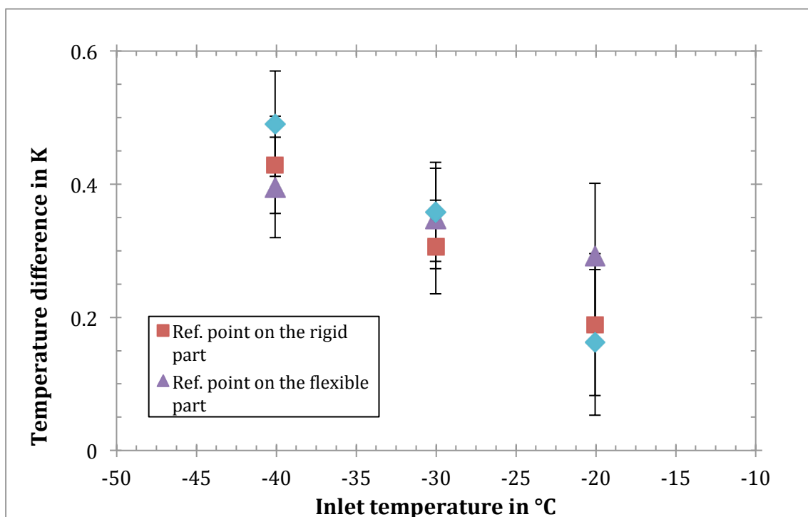
Figure 7-6 Temperature difference between ambient and surface temperatures measured on the rigid and flexible part of the transfer line in straight configuration with different coolant temperatures at the inlet with mass flow rate = 6 g/s.
