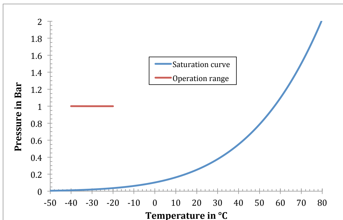
Figure 6-10 Pressure - temperature diagram of C 6 F 14 with saturation curve [16].
