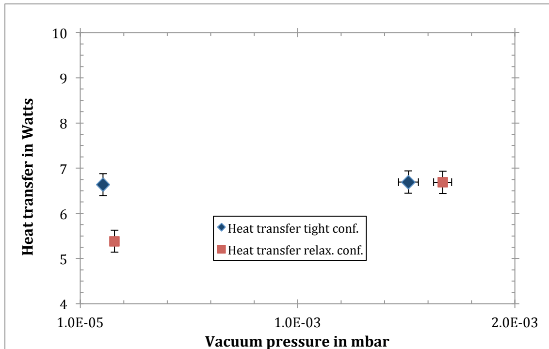
Figure 7-11 Heat transfer during the measurements in coiled - tight and coiled - relaxed configuration of the transfer line at different vacuum pressures with the coolant temperature measured at the inlet = -40°C and mass flow rate = 6g/s.
