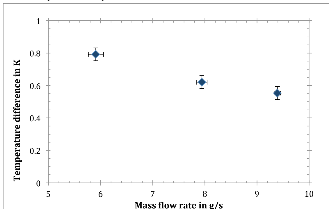
Figure 7-1 Temperature difference between inlet and outlet of the transfer line depending on the mass flow rate in straight configuration with temperature of the coolant measured at the inlet = -40^{\circ}\text{C} .
