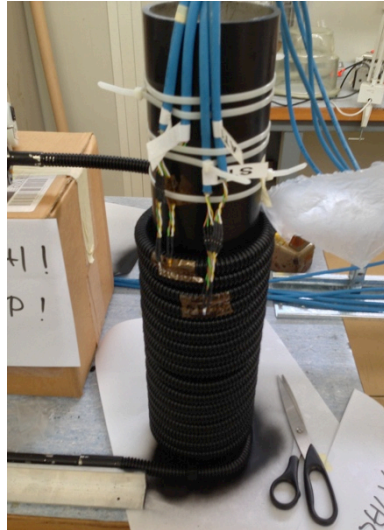
Figure 6-21 Transfer line in coiled – tight/relaxed configuration
