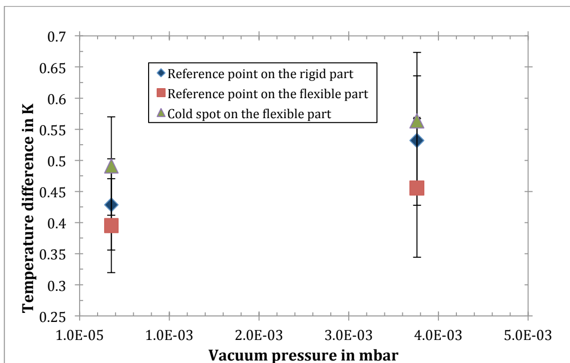
Figure 7-9 Difference between ambient and surface temperature measured on the rigid and flexible part of the transfer line in straight configuration at different vacuum pressures with the coolant temperature measured at the inlet = -40°C.
