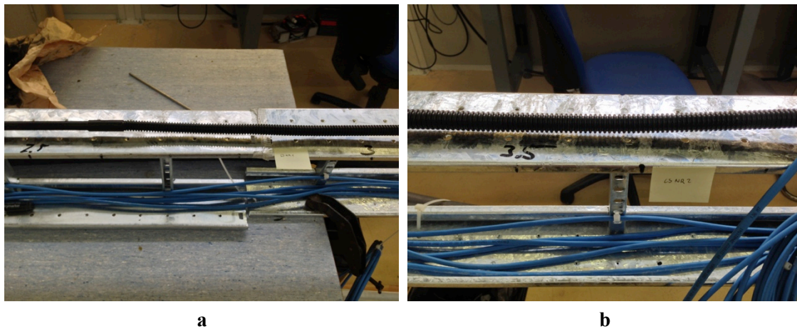
Figure 6-20 Spots where the IR pictures were taken; a) cold spot 1 observed with the IR camera; b) cold spot 2 observed with the IR camera
