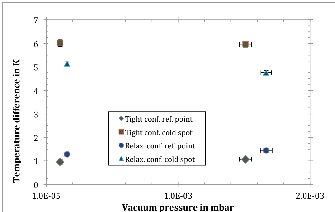
Figure 7-12 Temperature difference between ambient and surface temperature measured on the flexible part of the transfer line in coiled - tight and coiled - relaxed configuration of the transfer line at different vacuum pressures with the coolant temperature measured at the inlet = -40°C and mass flow rate = 6g/s.
