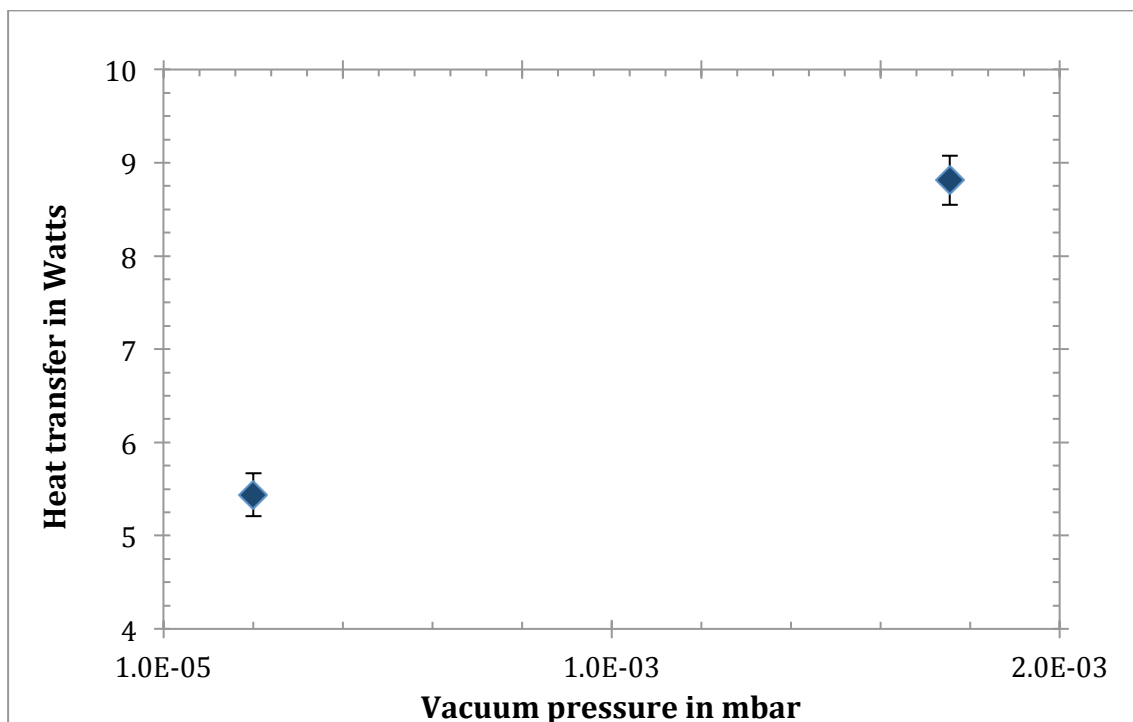
Figure 7-14 Heat transfer depending on vacuum pressure during the measurement after the bending of the rigid part of the transfer line with the coolant temperature measured at the inlet = -40^{\circ}\text{C} .
