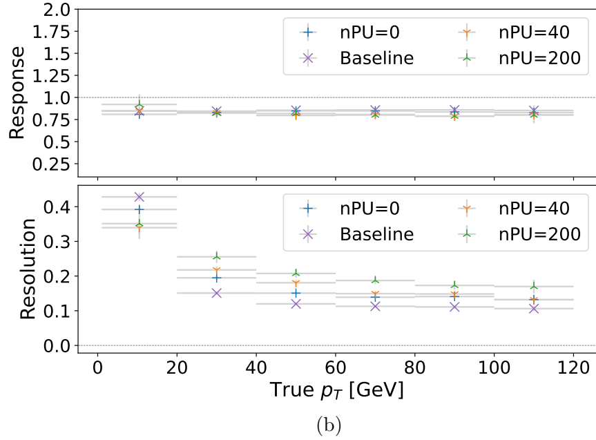
Figure 7.11: The response and the resolution of reconstructed single-particles in different pileup conditions as a function of true p_T . Fig. 7.11a shows the electromagnetic particles and Fig. 7.11b, the hadronic particles.
