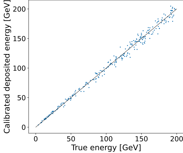
Figure 7.4: A scatter plot showing calibrated deposited energy versus true energy of photons shot between 1.8 < \eta < 2.8 . E_{\text{dep}} = E_{\text{impact}} line is highlighted.
