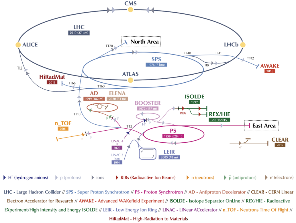
Figure 2.4: The accelerator complex of the LHC. First, hydrogen ions ( \text{H} + \text{e}^- \rightarrow \text{H}^- ) are accelerated at the Linear Accelerator 4 (Arnaudon et al., 2006). They are stripped of their two electrons at the booster to form protons ( \text{H}^- \rightarrow \text{H}^+ + 2\text{e}^- ). These protons ( \text{H}^- ) then make their way through two accelerators, the Proton Synchrotron and the Super Proton Synchrotron, before entering the LHC.
