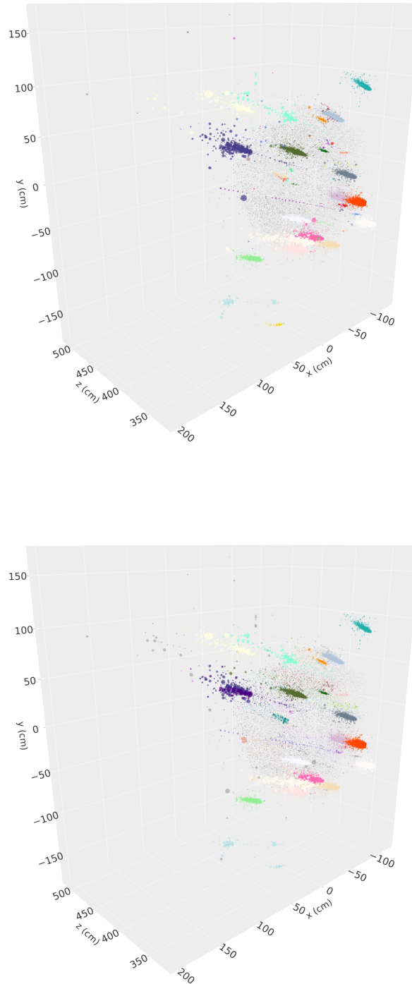
Figure 7.24: An example of event reconstruction in the CMS HGCAL. The top figure shows true showers and the bottom figure shows the predicted showers. The colours are the same if a predicted and a true shower is matched together.
