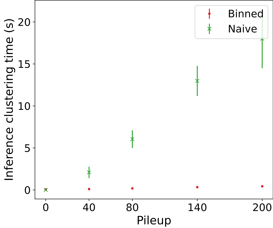
Figure 8.5: Inference clustering time in different pileup conditions. The optimised binned algorithm is compared to the naïve implementation. The error bars highlight the standard deviation instead of the standard error to demonstrate event-by-event variance in inference clustering time.
