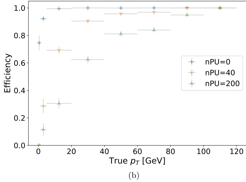
Figure 7.9: Reconstruction efficiency of single particles in different pileup conditions. Fig. 7.9a: efficiency as a function of the true p_T for electromagnetic particles (photons and electrons). Fig. 7.9b: efficiency as a function of the true p_T for hadronic particles (charged pions)
