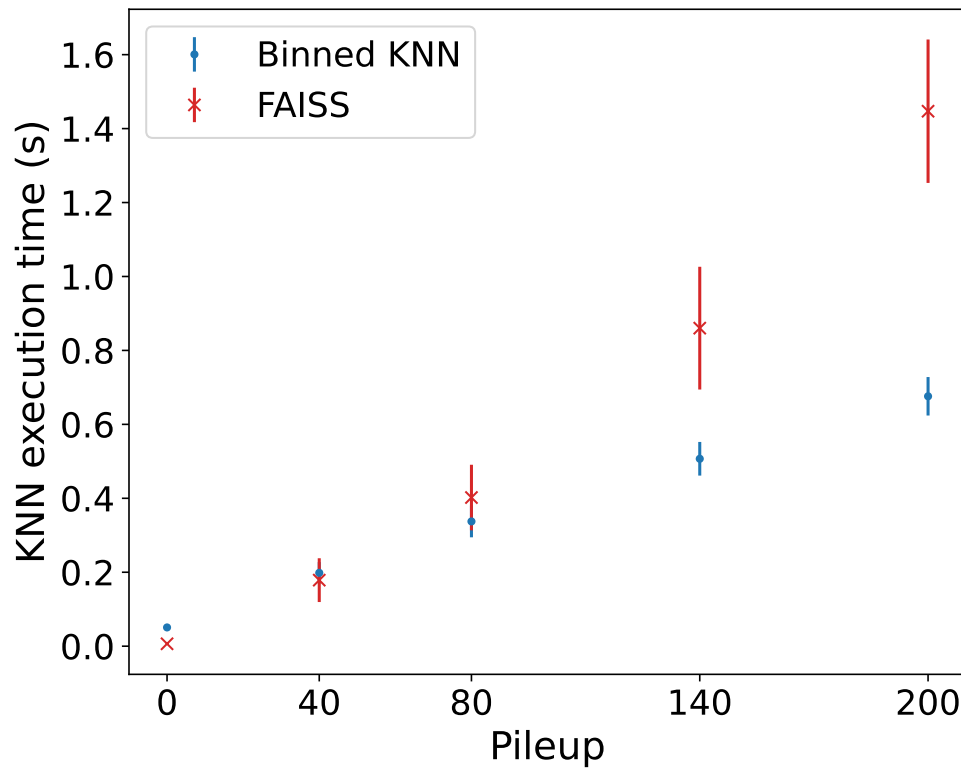
Figure 8.4: Total time taken by the binned KNN algorithm and FAISS (Johnson et al., 2019) to execute all the KNN graph-building operations during execution of the neural network as a function of pileup. The error bars highlight the standard deviation instead of the standard error to demonstrate event-by-event variance in the KNN execution.
