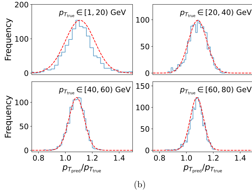
Figure 7.12: Fig. 7.12a: The response and resolution of electromagnetic particles computed as the mean and mean-corrected standard deviation of the Gaussian fit to the p_{T,\text{pred}}/p_{T,\text{true}} distribution in individual p_T bins. Fig. 7.12b: The distribution of p_T response in different p_T ranges corresponding to the first four bins in Fig. 7.12a in 0 pileup environment.
