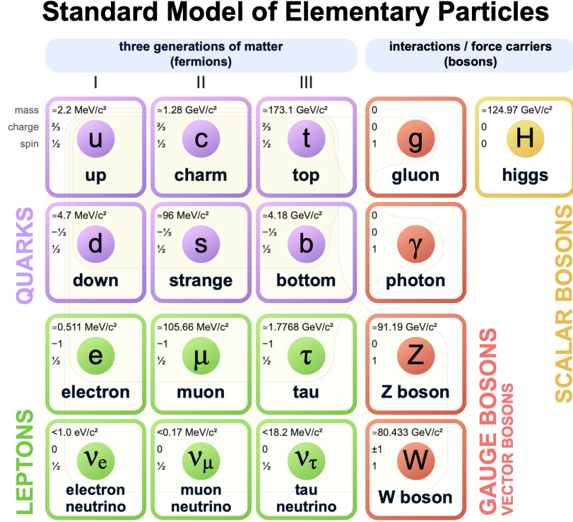
Figure 2.2: The Standard Model particles and their properties (Wikimedia Commons, 2019).
