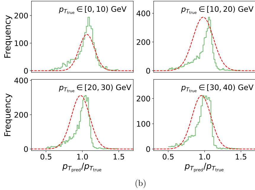
Figure 7.27: Fig. 7.27a shows mean response (top) and resolution (bottom) of the jets clustered on the HGCal data. The resolution is computed as the mean corrected standard deviation, as the data is not Gaussian, as shown in Fig. 7.27b where the fitted Gaussian functions are visualised.
