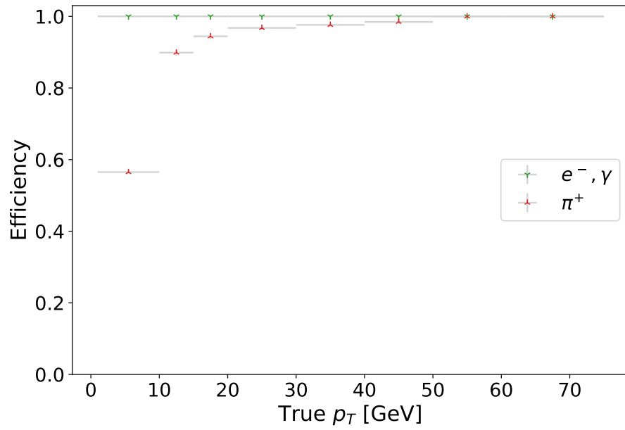
Figure 7.25: Efficiency as a function of predicted p_T with multi-matching allowed in the CMS HGICAL data.
