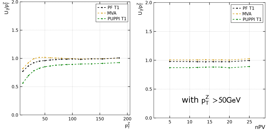
Figure 3.7: The \cancel{E}_T^{\text{MVA}} response is close to unity above p_T^Z > 30 GeV/ c . Thus, it covers an even broader range than the \cancel{E}_T^{\text{PF}} . Above 50 GeV/ c the response is independent on the number of reconstructed primary vertices in all \cancel{E}_T definitions.
