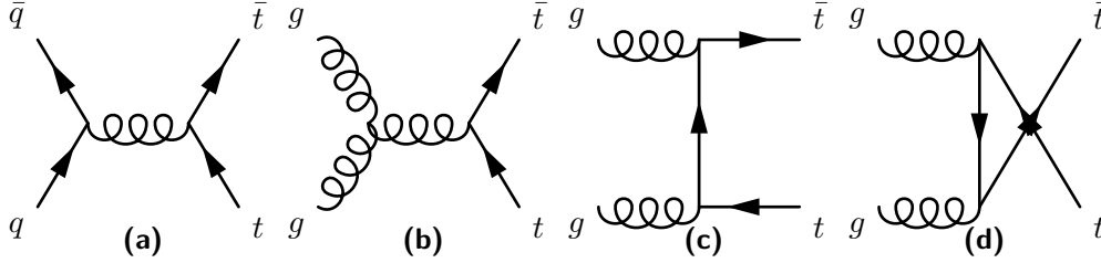
Figure 4.12: Feynman diagrams in leading order that contribute to top quark pair production at the LHC.[74]
