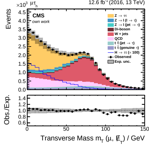
Figure 3.12: m_T^\mu distribution using E_T^{\text{MVA}} in the \mu\tau_h final state of the H \rightarrow \tau\tau analysis. The high- m_T^\mu region is dominated by W + \text{Jets} .
