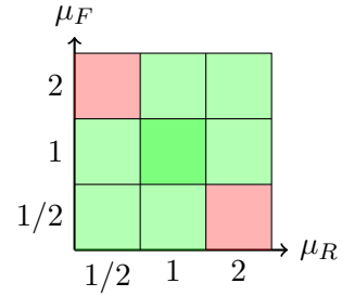
Figure 4.3: QCD scales variation scheme. The red parts are left out. The center is the nominal value, the light green ones are the variations.
