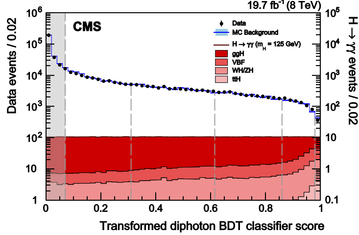
Figure 2.19: Transformed BDT score comparison for simulation and data. The leftmost area in gray is neglected due to its low ( S/(S+B) ) ratio. The dashed lines show the borders between the untagged event classes [47].
