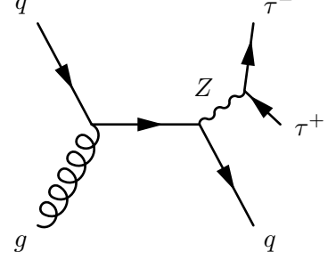
Figure 4.8: Drell-Yan Z production with an additional quark jet in the final state
