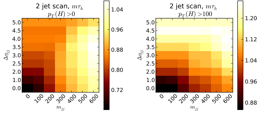
(b) \mu\tau_h with no p_T^H cut (left) and p_T^H > 100 \text{ GeV}/c
