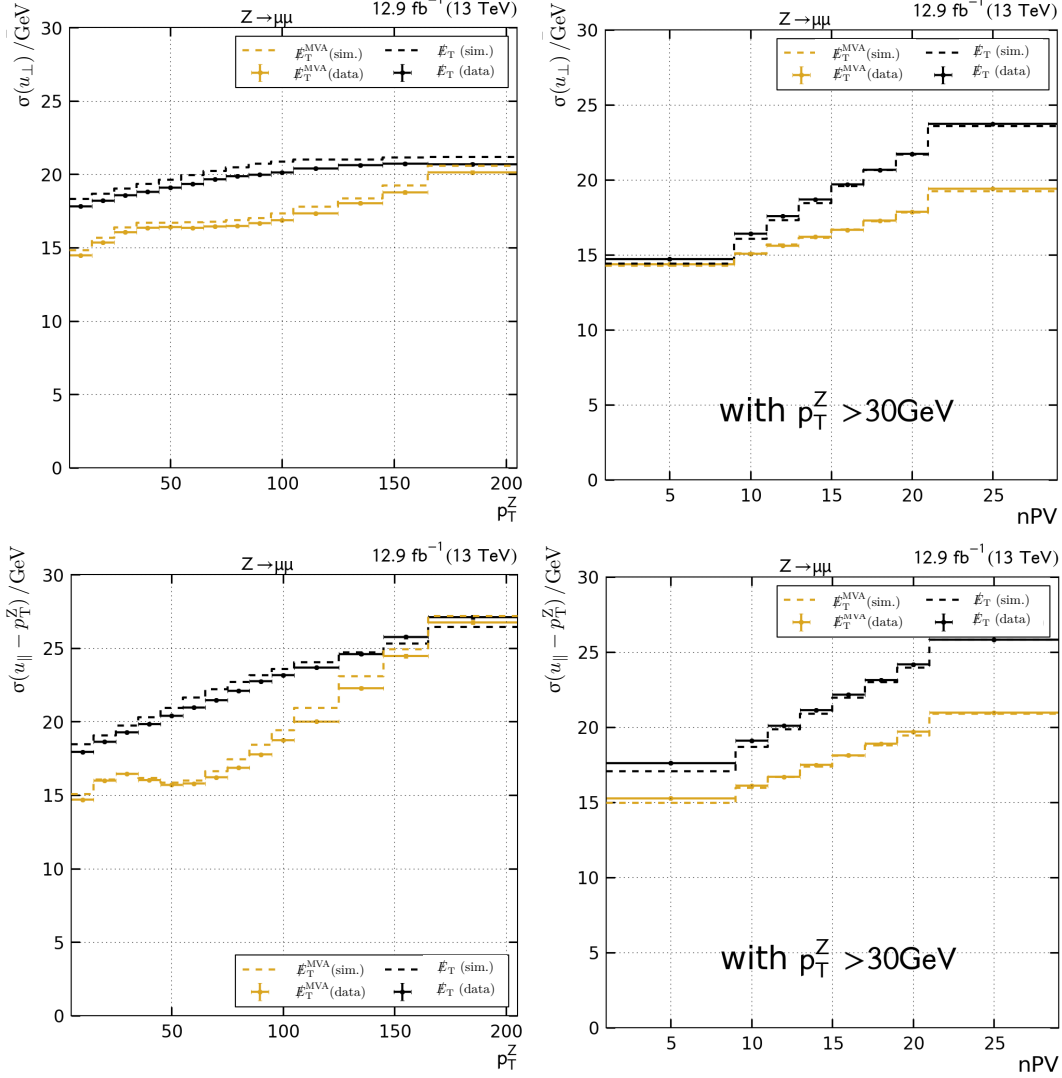
Figure 3.10: Resolution of E_T^{\text{PF}} and E_T^{\text{MVA}} for the 2016 dataset with an integrated luminosity of 12.9 \text{ fb}^{-1} . The multivariate E_T corrects resolution-degrading pile-up effects. These effects become relatively less important with highly boosted Z/\gamma^* bosons. Hence, the resolution gain is highest with boosts around 50 \text{ GeV}/c , where unity response is reached for both E_T definitions and pile-up effects remain important. At a boson p_T above 200 \text{ GeV}/c , both E_T definitions are comparable. The smaller slope in E_T^{\text{MVA}} compared to E_T^{\text{PF}} is also present here in the n_{\text{PV}} distribution on data, showing an increasing advantage of E_T^{\text{MVA}} with rising pile-up.
