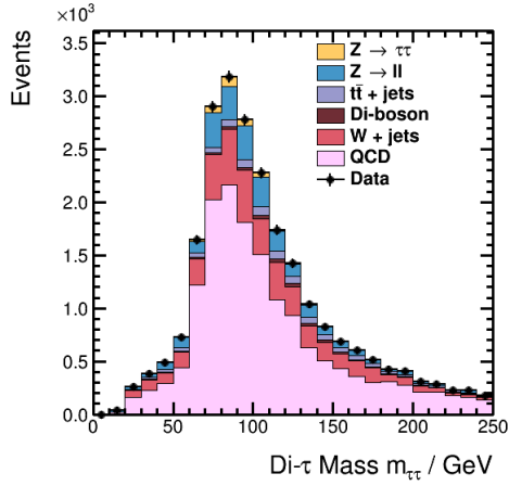
Figure 4.15: QCD background estimation, here in the \mu\tau_h channel. In same-sign di-tau pairs all known backgrounds are subtracted. The remaining events are interpreted as QCD events.
