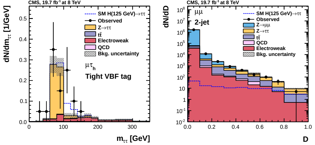
Figure 2.27: Comparison of final discriminating variables. Left: m_{\tau\tau}^{SVFit} in the VBF tight category of the \mu\tau_h channel. 20 events are observed in this category with a signal expectation of 2.4 events. Right: The final discriminating variable D in the H \rightarrow \tau\tau \rightarrow \mu\mu analysis in the VBF category. The prompt Z \rightarrow \mu\mu decays get classified with a low score. The relative signal contribution increases from O(10^{-5}) at low values of D to 9 expected background in 2 expected signal events in the high- D region.
