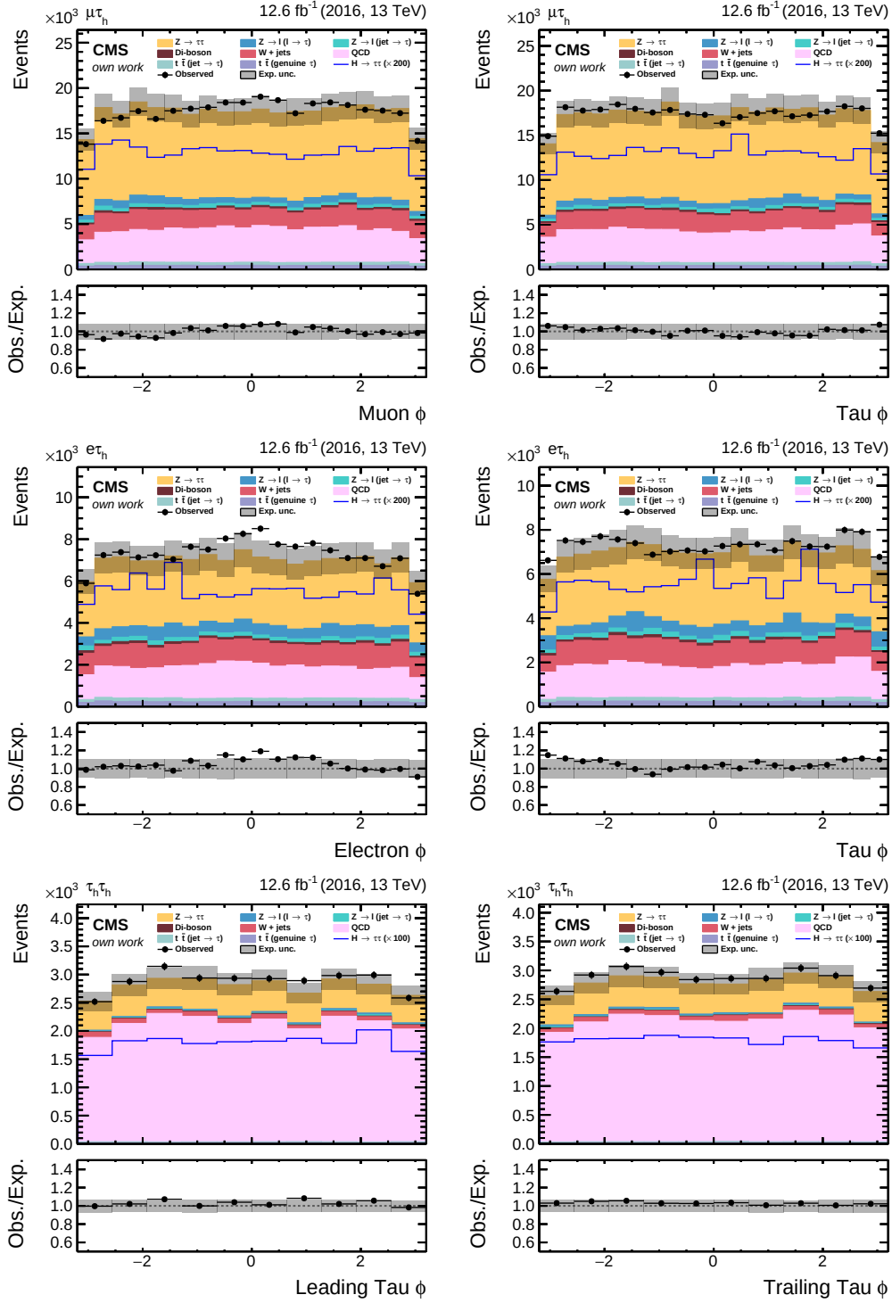
Figure A.5: Di-lepton pair \phi in the \mu\tau_h (first row), e\tau_h (middle row) and \tau\tau_h (bottom row) inclusive channels.
