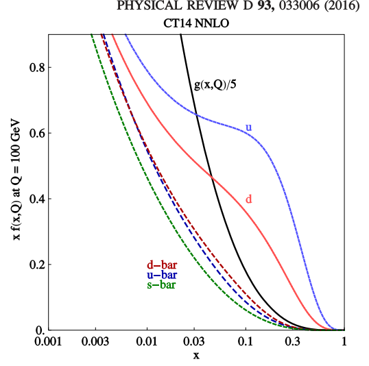
Figure 1.6: Parton distribution function at the scale of Q = 100 \text{ GeV} which is close to the search range of m_H from the global fit to the CT14 NNLO ensemble [12]. The plot shows the probability density functions for observing a valence quark ( u, d ) or anti-quark ( \bar{d}, \bar{u}, \bar{s} = s ) as well as a gluon g (divided by a factor of 5) as a function of x . The PDFs are derived from the CT14 dataset containing the HERA, TEVATRON and LHC Run I measurements.
