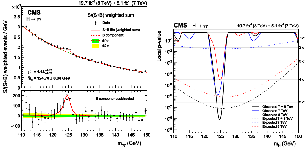
Figure 2.20: Final mass distribution, s/(s+b) weighted (left) showing an excess with a best-fit value of m_H = 124.70 \text{ GeV}/c^2 . right: the local p -value for the 7 and 8 TeV analysis and their combination[47].
