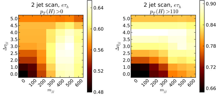
(a) e\tau_h with no p_T^H cut (left) and p_T^H > 110 \text{ GeV}/c
