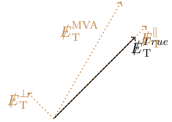
Figure 3.11: Definition of parallel and perpendicular components of the \cancel{E}_T^{\text{True}} .
