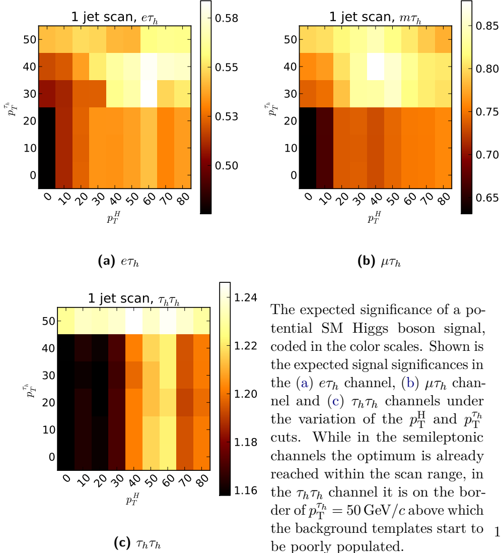
Figure 4.27: Significance scans in the 1-jet categories
