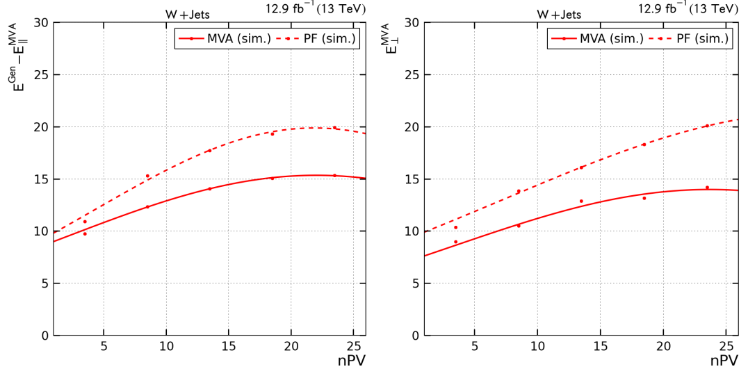
Figure 3.13: Resolution of different E_T definitions, not corrected by their response. An increase of resolution by the n_{\text{PV}} implies a pile-up dependence of the E_T definition. As already seen in the \mu\mu channel, the resolution in E_T^{\text{MVA}} degrades less with more activity in the event compared to the E_T^{\text{PF}} .
