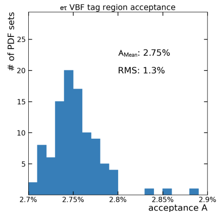
Figure 4.6: An example distribution of acceptances under the variation of PDF sets. Shown is the VBF tagged category in the e\tau_h decay channel.
