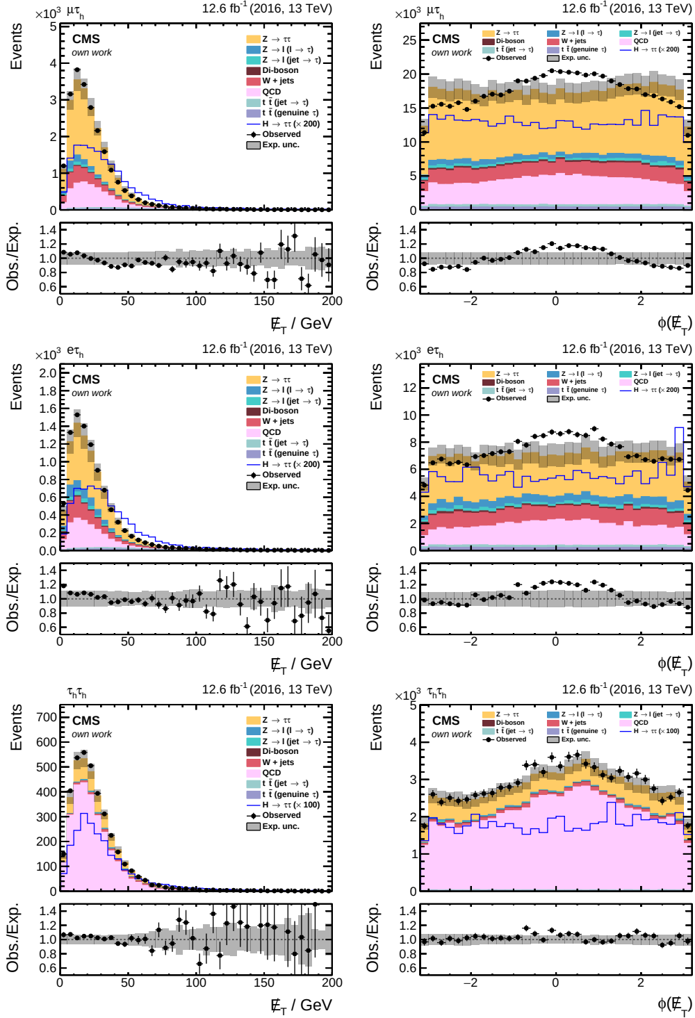
Figure A.11: E_T^{MVA} and \phi_{E_T}^{MVA} in the \mu\tau_h (first row), e\tau_h (middle row) and \tau_h\tau_h (bottom row) inclusive channels.
