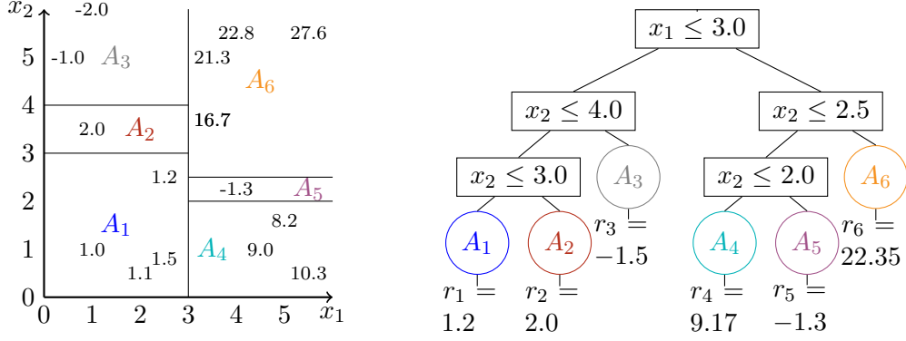
Figure 2.16: An exemplary dataset with 15 two-dimensional input vectors \vec{X} = (x_1, x_2)^T and the 15 target values. The borders of the cut search are marked with lines and the resulting phase-space region are labels with A_m, m \in \{1..6\} . The tree has a depth of three. In a real training, one usually requires a minimal number of events per leaf, which is here left out for simplicity. On the right the corresponding representation in a tree is shown with the regressed value at the end.
