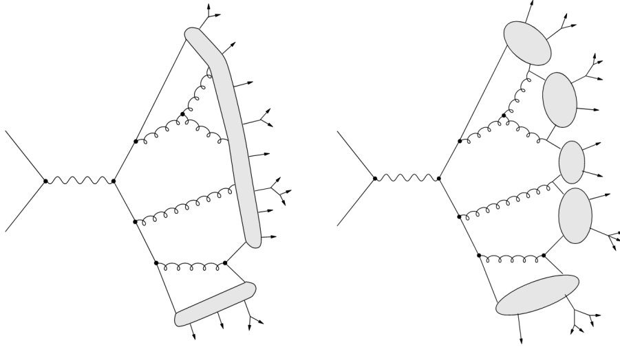
Figure 2.6.: Sketch of string (left) and cluster (right) hadronization model, taken from Ref. [30].
