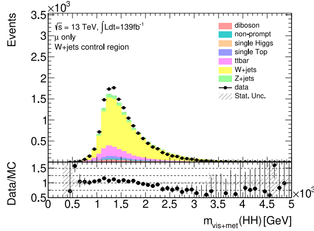
Figure 6.15.: ATLAS data against background including V +jets samples produced with SHERPA 2.2.1 for m_{\text{vis}+\text{met}}(HH) in the W +jets CR.
