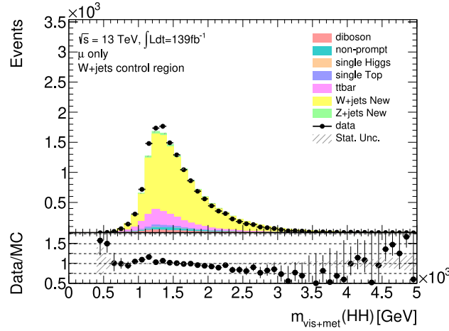
Figure 6.19.: ATLAS data against background for V +jets samples produced with SHERPA 2.2.11 for m_{\text{vis}+\text{met}}(HH) in the W +jets CR.
