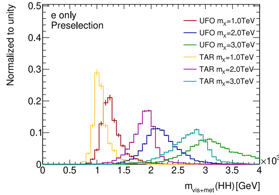
Figure 6.13.: Comparison between TAR and UFO jet objects for HH samples at different mass points m_X in the electron channel for m_{\text{vis}+\text{met}}(HH) .
