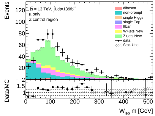
Figure 6.21(b): m(W_{\text{lep}})
