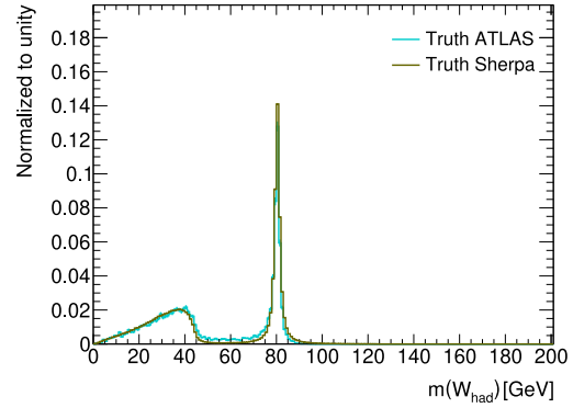
Figure 6.6(b): m(W_{\text{had}})
