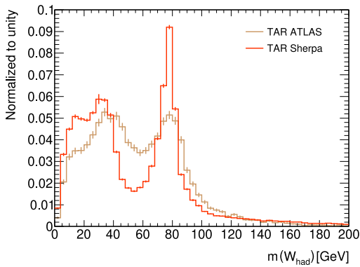
Figure 6.4(a): m(W_{\text{had}})
