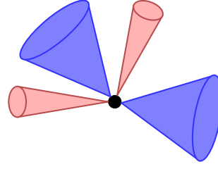
Figure 6.2(b): multijet
