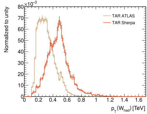
Figure 6.3(b): p_T(W_{\text{had}})
