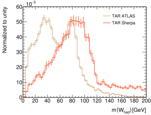
Figure 6.3(a): m(W_{\text{had}})
