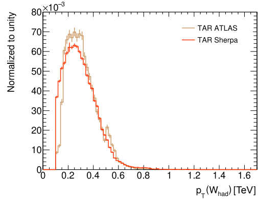
Figure 6.4(b): p_T(W_{\text{had}})
