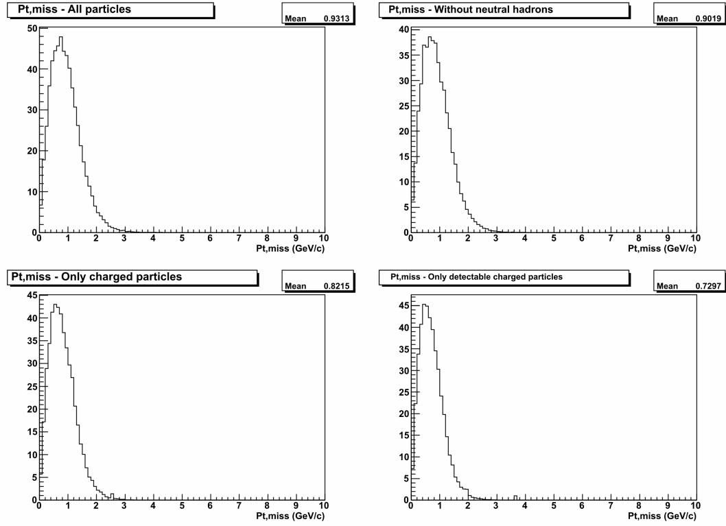
Figure A.9: P_{t,miss} distributions obtained with a non-smeared \nu_\tau CC sample - for details see section 6.3.2 and Figure 6.17
