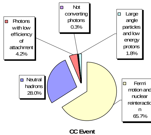
Figure 6.11: Contributions to P_{t,miss} broken up by source: a) Fermi motion and nuclear re-interactions; b) neutral hadrons; c) Photons with low attachment efficiency; d) non-converting photons; e) Particles with a slope larger than 0.5 and protons with energy less than 0.3 GeV/c.
