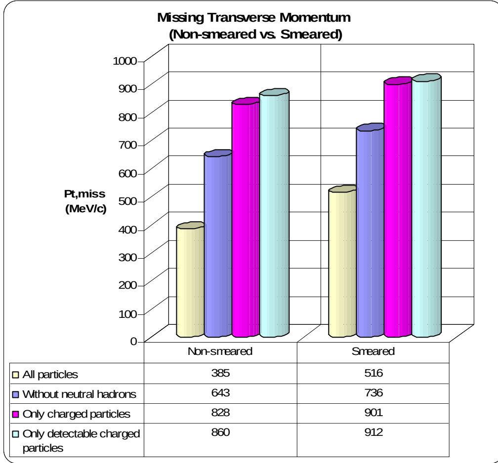
Figure 6.8: Results of P_{t,miss} computed for the non-smeared and smeared samples by considering: a) all particles; b) charged particles and photons; c) just charged particles; d) detectable particles (i.e charged particles with angle less than 0.5 rad and protons with energy larger than 0.3 GeV/c)
