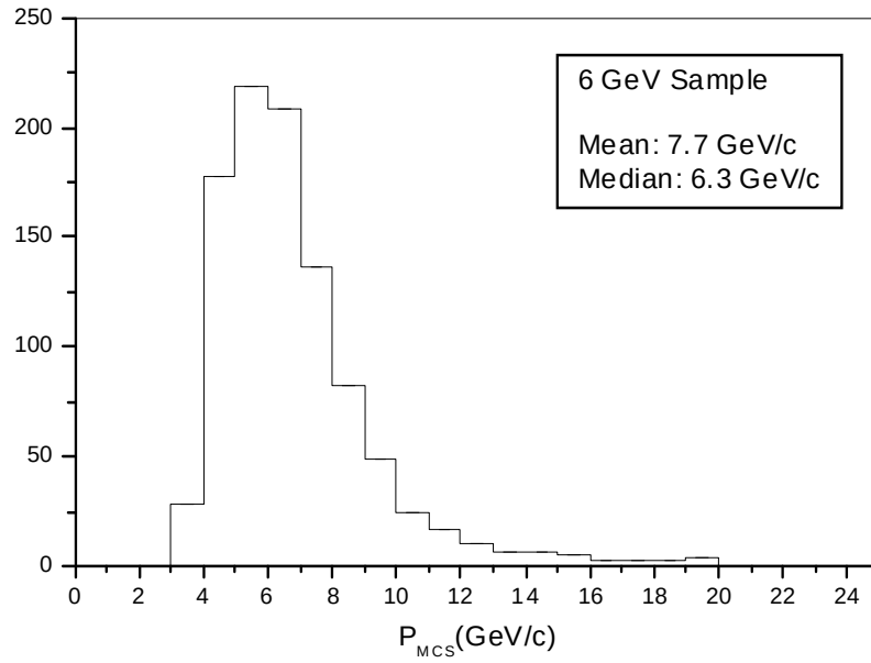
Figure 4.2: The distribution of estimated momenta obtained using a sample of 6 GeV/c simulated data. The distribution shows a long tails for high momentum tracks, which have scattering effect smaller than the measurement error.
