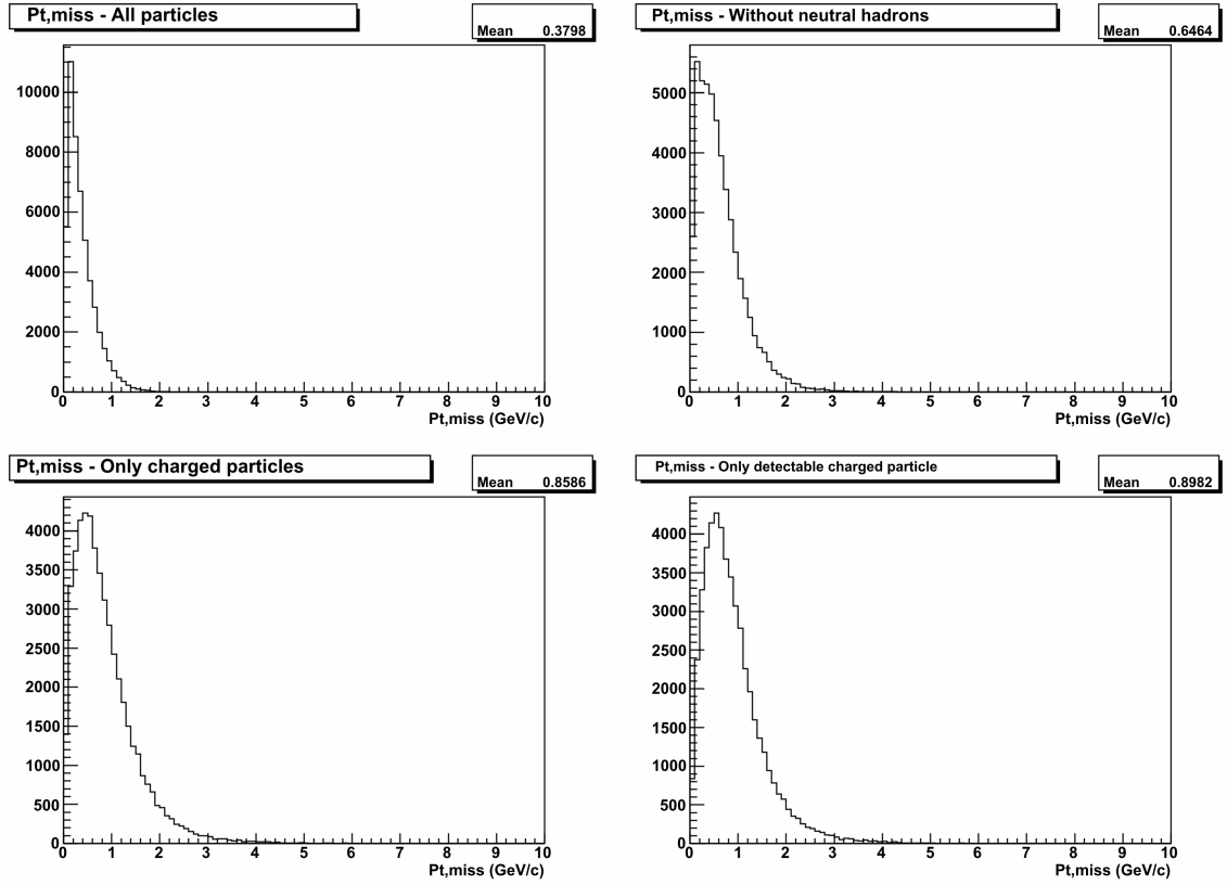
Figure A.5: P_{t,miss} distributions obtained with a non-smeared \nu_\tau CC sample - numbers not shown in previous sections
