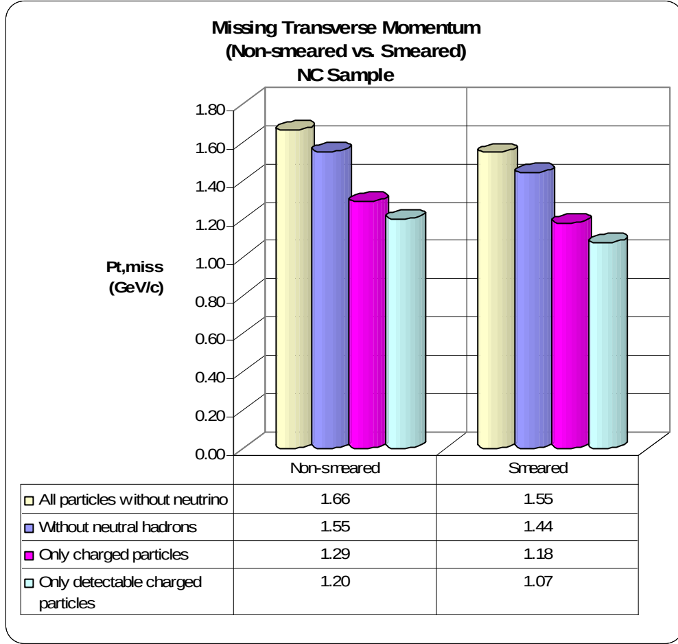
Figure 6.15: Results of P_{t,miss} computed for the non-smeared and smeared samples by considering: a) all particles; b) charged particles and photons; c) just charged particles; d) charged detectable particles (i.e particles with slope below 0.5 and protons with energy larger than 0.3 GeV/c)
