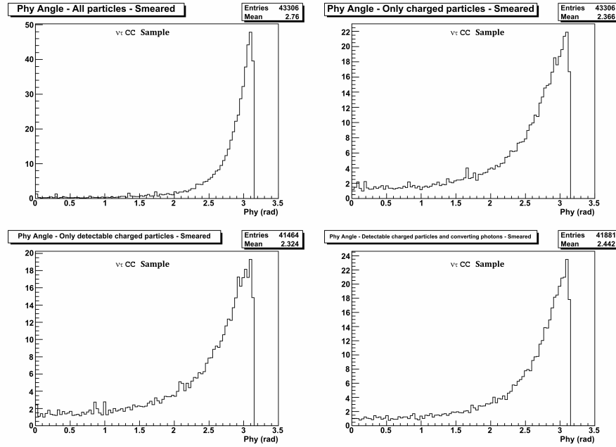
Figure 6.26: The \phi angle distributions obtained for the signal considering different scenarios: (top-left) all particles detected without the neutrino; (top-right) charged particles detected; (bottom-left) charged detectable particles detected; (bottom right) charged detectable particles and converting photons
