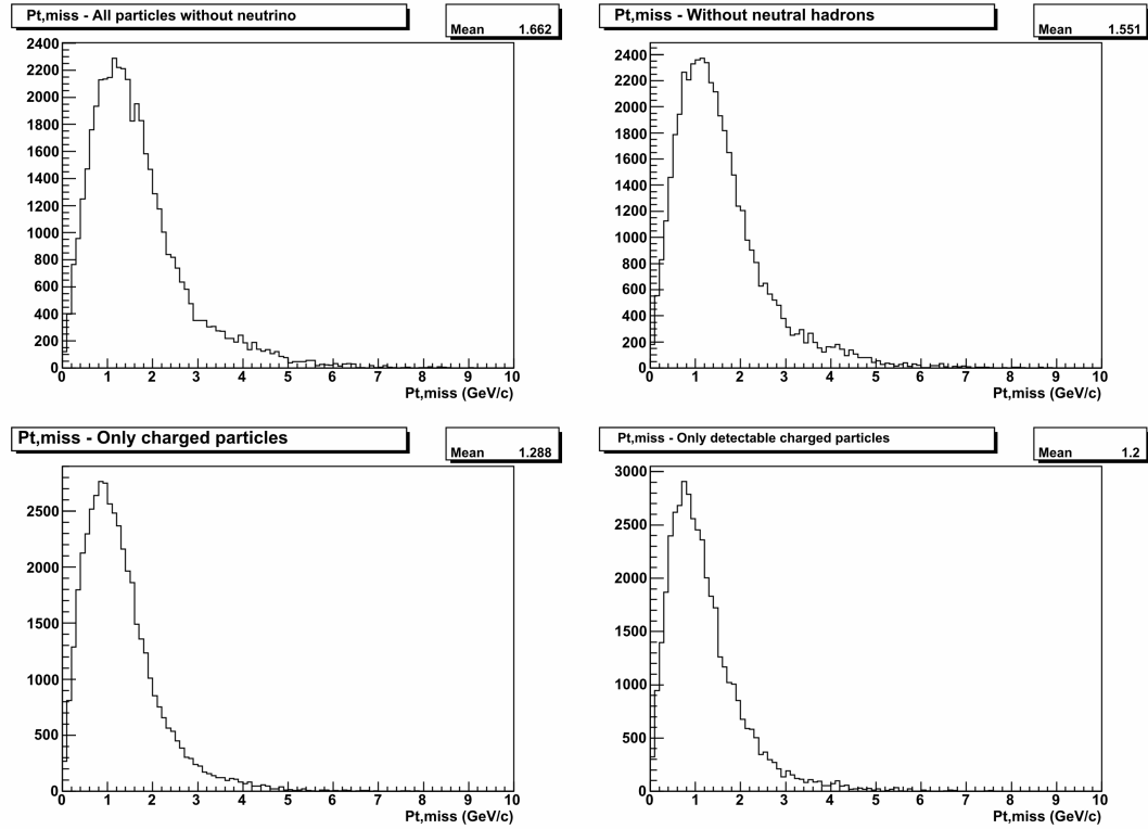
Figure A.7: P_{t,miss} distributions obtained with a non-smeared \nu_\mu NC sample - for details see section 6.3.2 and Figure 6.15 99
