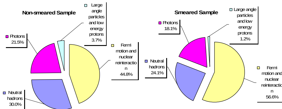
Figure 6.9: Contribution at P_{t,miss} given, for non-smeared and smeared samples, broken up by source: a) Fermi motion and nuclear re-interactions; b) Neutral hadrons, c) Photons; d) Particles with slope beyond 0.5 and protons with energy less than 0.3 GeV/c.
