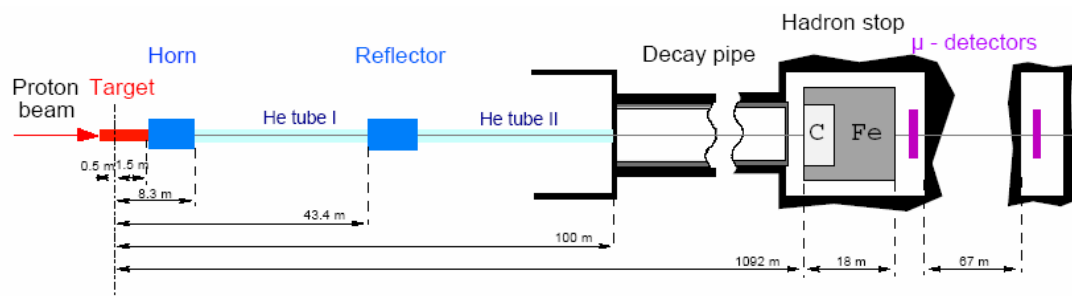
Figure 2.2: Layout of the CNGS beam. The coordinate origin is the focus of the proton beam
