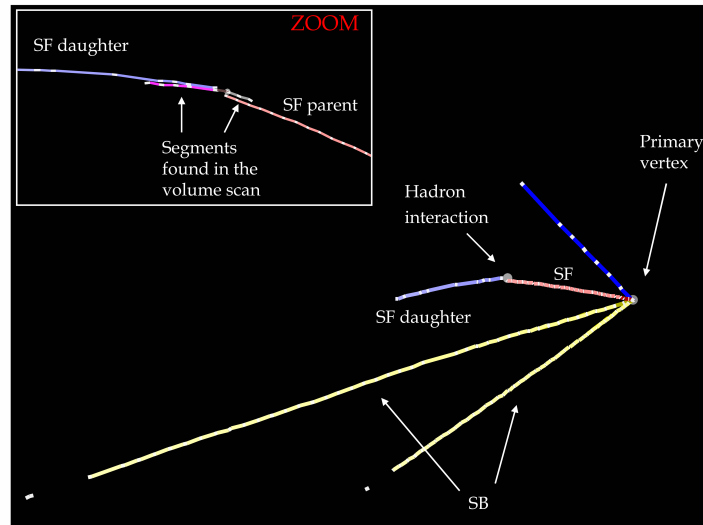
Figure 5.6: An example of an hadron interaction reconstructed in Salerno. The yellow tracks are the SB tracks, the red track is a SF track that stops in the brick and interacts with the lead producing an outgoing hadron (purple). The zoom view enhances the track segments found in the volume scan and in the SF of the parent and the daughter.
