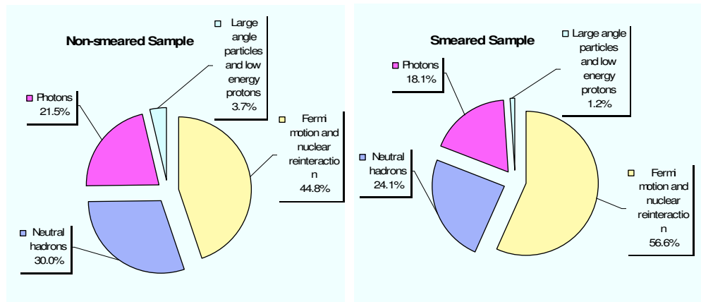
Figure 6.9: Contribution at P_{t,miss} given, for non-smeared and smeared samples, broken up by source: a) Fermi motion and nuclear re-interactions; b) Neutral hadrons, c) Photons; d) Particles with slope beyond 0.5 and protons with energy less than 0.3 GeV/c.
