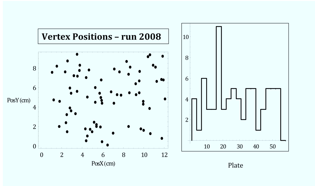
Figure 3.14: Left: The vertex position in the plane X-Y; Right: The longitudinal vertex positions (as number of plate) - Run 2008
