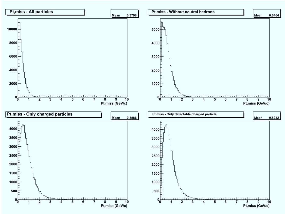
Figure A.5: P_{t,miss} distributions obtained with a non-smeared \nu_\tau CC sample - numbers not shown in previous sections
