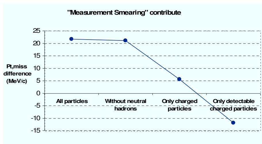
Figure 6.20: Contribution to P_{t,miss} in the \nu_\tau CC sample, given by the “measurement smearing”, as a function of the number of particles removed.
