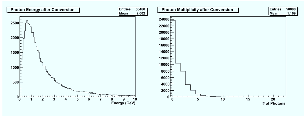
Figure 6.6: Energy (left) and multiplicity (right) distributions of converting photons in an ECC.
