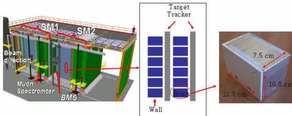
Figure 2.4: Left: schematic drawing of the OPERA detector; Center: sketch of 2 modules; each of them is made of a wall + two Target Tracker planes; Right: real brick picture. CSs sheet are contained in a separate box (white in the image)
