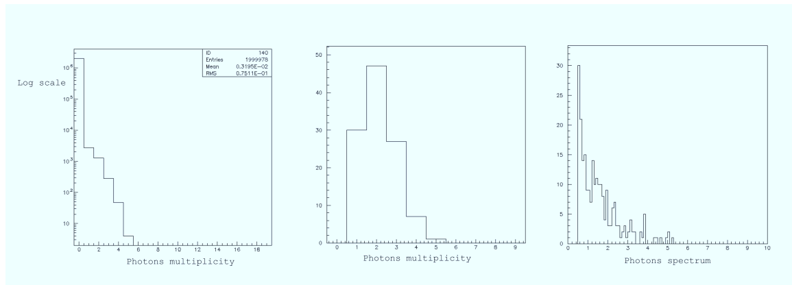
Figure 5.3: Multiplicity of photons produced in the interaction of a beam of 5 GeV pions with 1 mm of lead before (left) and after (center) the kinematical cuts and their energy after the cuts (right) [83]
