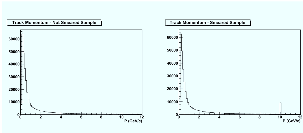
Figure 6.1: The momentum distribution of charged particles attached to primary vertex: comparison between the non-smeared (left) and smeared (right) sample.
