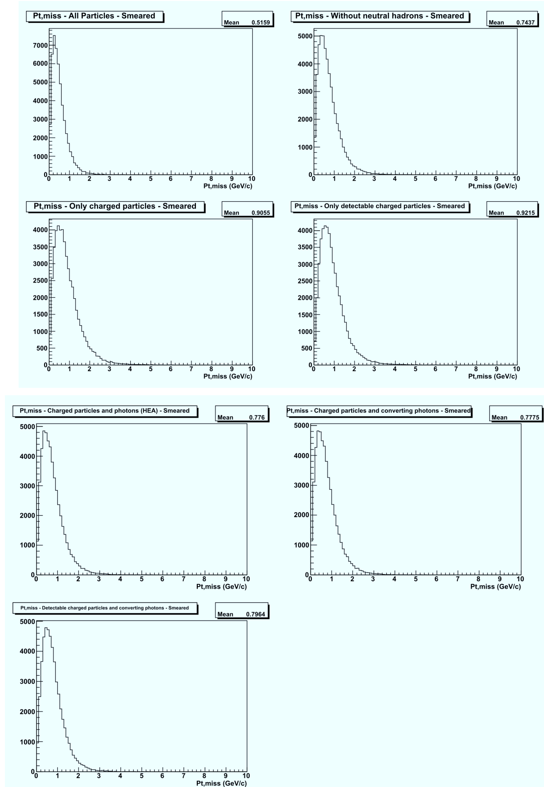
Figure A.4: P_{t,miss} distributions obtained with a smeared \nu_\mu NC sample; the neutrino is treated as a muon particle - for details see section 6.3.2 and Figure 6.12
