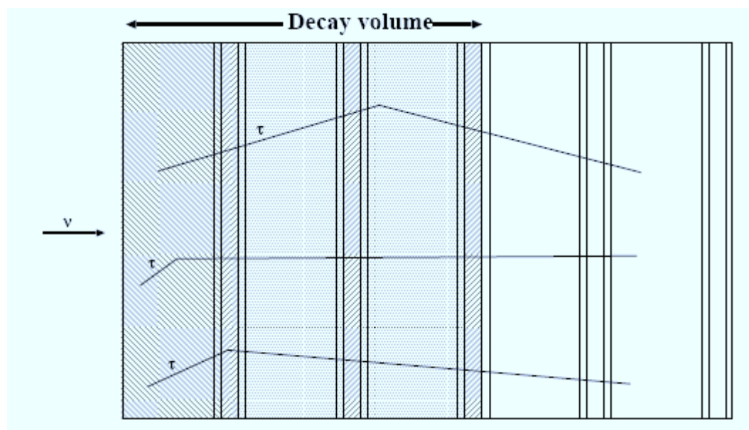
Figure 2.6: Different decay topologies; short decay (left-hatched region); long decays in base (right-hatched region); long decays outside the base (shaded region); very long decays (white region), not shown.
