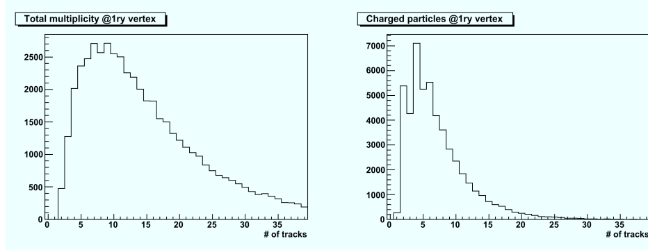
Figure 6.2: The multiplicity distributions of tracks at primary vertex computed by using all charged and neutral hadrons (left) and only charged particles (right).
