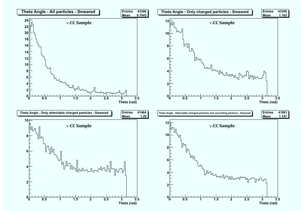
Figure 6.30: The \theta angle distributions obtained for the signal considering different scenarios: (top-left) all particles detected without the neutrino; (top-right) charged particles detected; (bottom-left) charged detectable particles detected; (bottom right) charged detectable particles and converting photons
