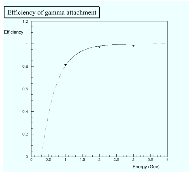
Figure 6.4: Efficiency of gamma attachment as a function of the energy
