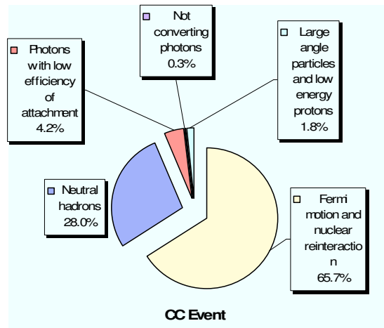
Figure 6.11: Contributions to P_{t,miss} broken up by source: a) Fermi motion and nuclear reinteractions; b) neutral hadrons; c) Photons with low attachment efficiency; d) non-converting photons; e) Particles with a slope larger than 0.5 and protons with energy less than 0.3 GeV/c.
