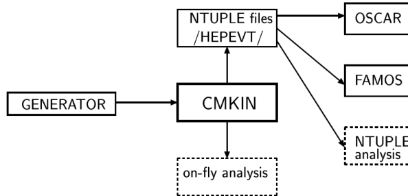
Figure 5.1: Sketch of the interaction of the CMS-specific wrapper program CMKIN with generator programs and detector simulation packages (taken from [PTDR2]).
