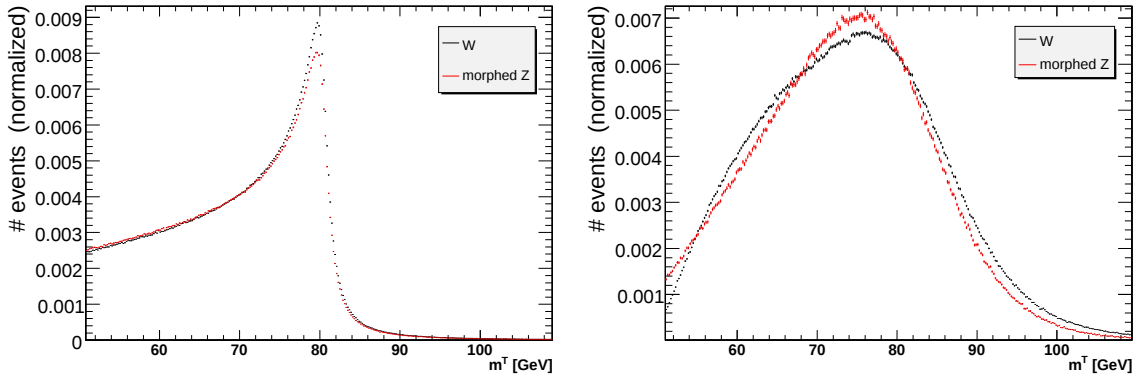
Figure 6.16: The left-hand distributions show the transverse mass of W events generated with Pythia (in black) and corresponding morphed Z bosons events (in red); only the selection cut on the number of muons has been applied. The right-hand distributions show the transverse masses of W events and morphed Z events, simulated with FAMOS and with all selection cuts applied.
