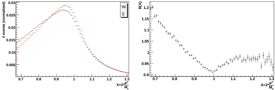
Figure 6.21: Left: the scaled muon momentum distributions for both W and Z boson events after all selection cuts have been applied. Right: the R(X) distribution calculated from the scaled muon momenta.
