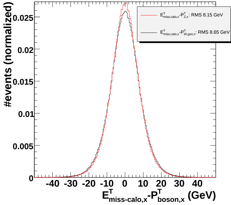
Figure 6.19: Distributions of E_{miss,calor,x}^T - P_{Z,x}^T ( P_Z^T reconstructed from the muons) for Z boson events and E_{miss,calor,x}^T - P_{W,gen,x}^T for W boson events after all selection cuts. The width for Z boson events is 6.1% smaller than the width for W boson events.
