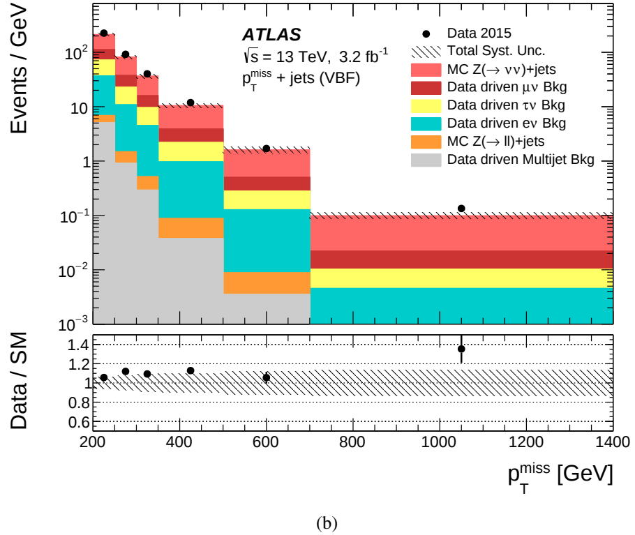
Figure 7.2: The composition of the detector-level combined numerators including all background predictions. These figures show the first two measured distributions for this analysis: p_T^{\text{miss}} for (a) the \geq 1 jet region, and (b) the VBF region. The predictions and data are compared—the ratio panel details this relationship. The statistical uncertainties of the data, and the systematic uncertainties (discussed in Section 7.6.1) are represented by error bars and bands respectively.
