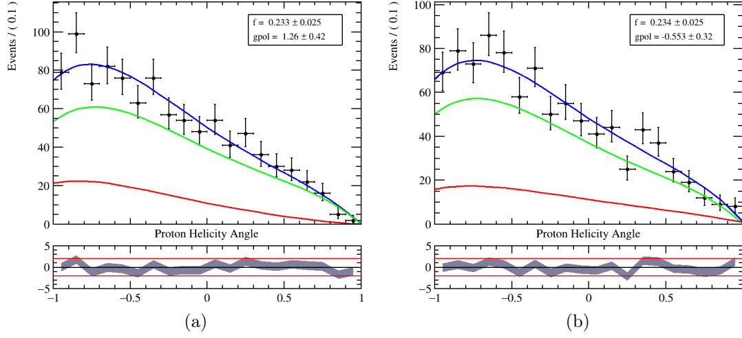
Figure 5.31: Unblinded fit of the cosine of the proton helicity angle distribution for (a) \Lambda_b^0 \rightarrow \Lambda \gamma and (b) \bar{\Lambda}_b^0 \rightarrow \bar{\Lambda} \gamma candidates. The total angular PDF, and the signal and combinatorial background contributions are shown blue, red and green lines, respectively.
