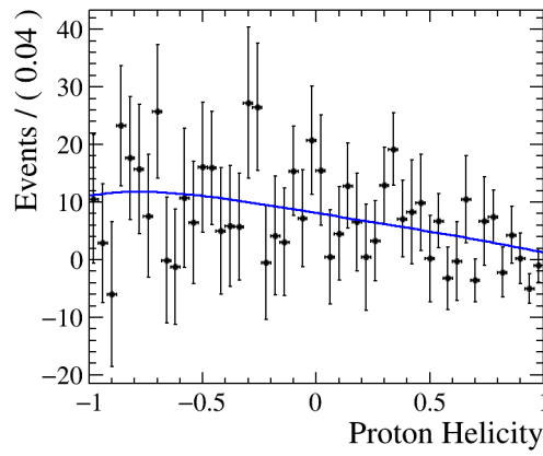
Figure A.24: Weighted unbinned fit to proton helicity distribution from a pseudo-experiment of set N^0 3, the fitted PDF is overlaid.
