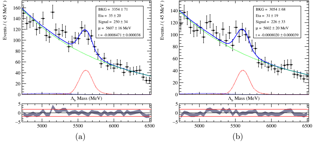
Figure 5.26: Invariant mass distributions of (a) \Lambda_b^0 \rightarrow \Lambda \gamma and (b) \bar{\Lambda}_b^0 \rightarrow \bar{\Lambda} \gamma data candidates after the loose selection (black markers). The result of the invariant mass fit is overlaid. The total PDF is represented by the solid blue curve, while the signal, combinatorial and partially reconstructed \Lambda_b^0 \rightarrow \Lambda \eta background are displayed by the dashed red, green and blue curves, respectively.
