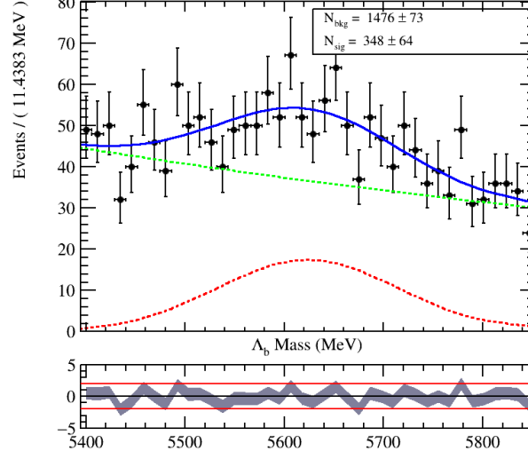
Figure A.23: Invariant mass distribution in the reduced mass region, used to extract per-event s Weights. pseudo-experiment of set N^0 3. The result of the invariant mass fit is overlaid, along the fitted signal and background yields.
