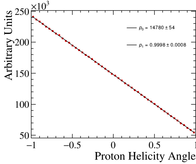
Figure 5.2: Generator-level distribution of \cos \theta_p for signal events with a fit to the photon polarization. Error bars are plotted. The fitted function is W(\theta_p) = p_0 \cdot (1 - \alpha_\Lambda \cdot p_1 \cdot \cos \theta_p) , comparing it to Eq. 5.3, p_1 corresponds to the fitted photon polarization.
