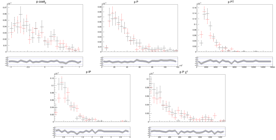
Figure A.4: Proton distributions comparison between Redecay (red) and full simulation (black).
