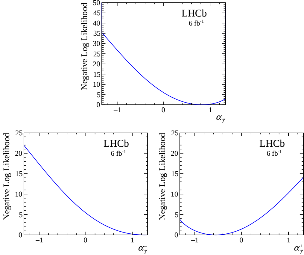
Figure A.34: Profile of the negative log likelihood along the (top) combined, (bottom-left) \Lambda_b^0 \rightarrow \Lambda \gamma and (bottom-right) \bar{\Lambda}_b^0 \rightarrow \bar{\Lambda} \gamma photon polarization values ( \alpha_\gamma , \alpha_\gamma^- and \alpha_\gamma^+ , respectively).
