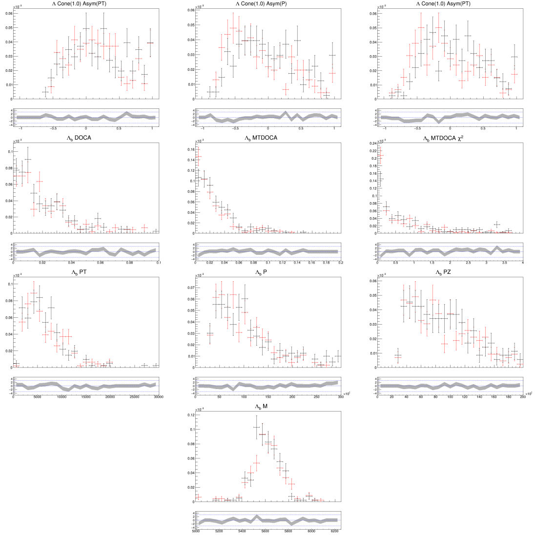
Figure A.1: \Lambda_b^0 baryon distributions comparison between rede cay (red) and full simulation (black).
