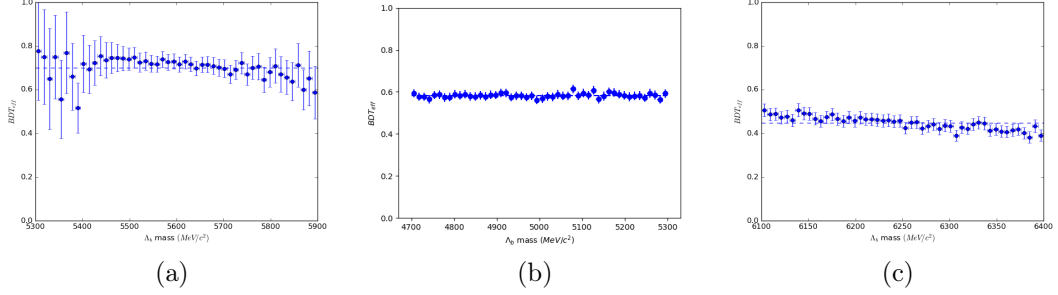
Figure A.19: BDT efficiency per \Lambda_b^0 mass bin on (a) simulation samples and (b, c) LMSB and HMSB data samples of the 2017 period, respectively.
