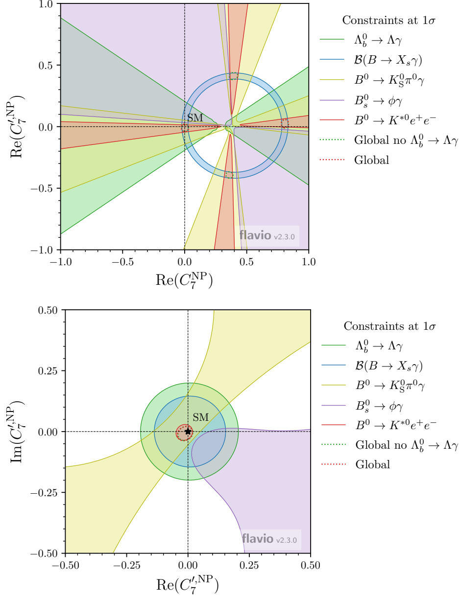
Figure 5.32: Constraints at the 1\sigma level on the new physics contributions to the (top) left- and right-handed Wilson coefficients, C_7^{(\text{eff})} and C_7'^{(\text{eff})} and on the (bottom) real and imaginary parts of C_7'^{(\text{eff})} . In the latter, the C_7^{(\text{eff})} coefficient is fixed to its SM value. The measurements of the inclusive branching fraction, \mathcal{B}(B \rightarrow X_s \gamma) , and the B^0 \rightarrow K_S^0 \pi^0 \gamma mixing-induced CP asymmetry by the Belle and BaBar experiments [50, 75] are shown in blue and yellow, respectively, the B_s^0 \rightarrow \phi \gamma and B^0 \rightarrow K^{*0} e^+ e^- measurements by the LHCb experiment [53, 54] in purple and red, respectively, and the \alpha_\gamma measurement presented in green. The global fit is shown in dashed red (green) lines including (excluding) this measurement.
