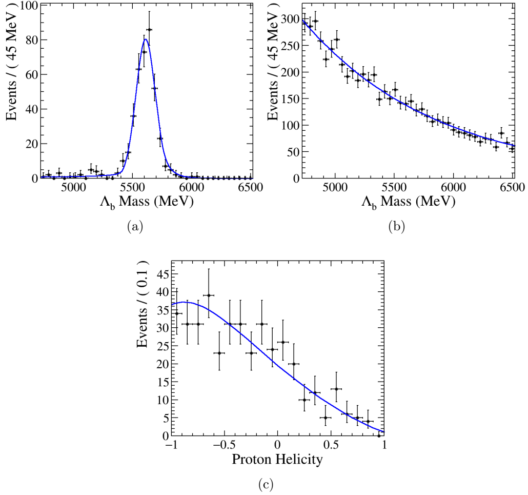
Figure A.22: Generated distributions for the invariant mass of (a) signal and (b) background contributions and for the (c) helicity angle of the signal component. pseudo-experiment of set N o 3, the generation PDF is overlaid.
