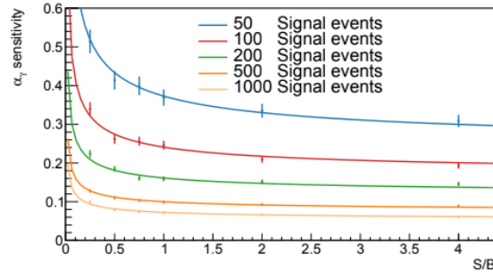
Figure 5.9: Sensitivity to the photon polarization as a function of the signal yield and the signal over background ratio, as extracted from pseudo-experiments (markers) [2]. Collections of pseudo-experiments with the same number of generated signal events are plotted in the same colour. The result of the fit using \sigma_{\alpha_\gamma}^{(1)} from Eq. 5.5 is overlaid.
