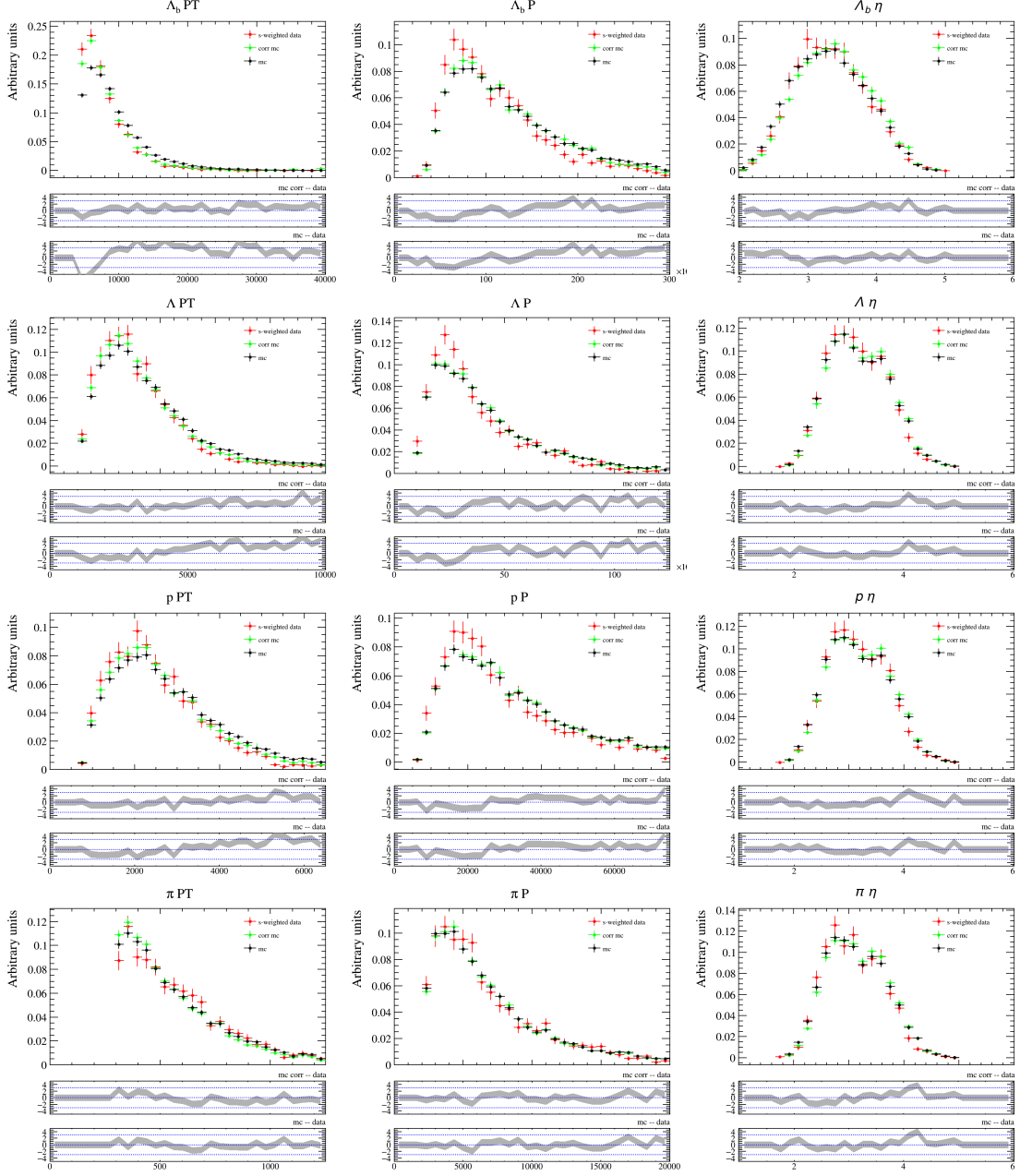
Figure A.8: Distributions of \Lambda , \pi and proton momenta and transverse momenta for sweighted data, simulation and corrected simulation candidates for 2018.
