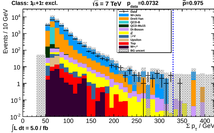
Figure 5.10: The \Sigma p_T distribution of the 1\mu - 1\tau event class. Being a promising candidate for exotic models this final state has to be understood well when searching for new physics. Overall, good agreement between data and Monte Carlo is observed. Dominating contributions are made by the W boson production. No evidence for new physics is observed.
