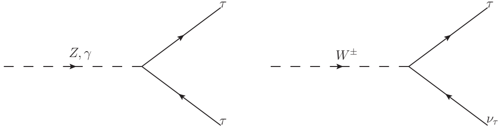
Figure 4.5: Feynman graphs for \tau production. On the left, from the Z or \gamma and on the right from the W^\pm .
