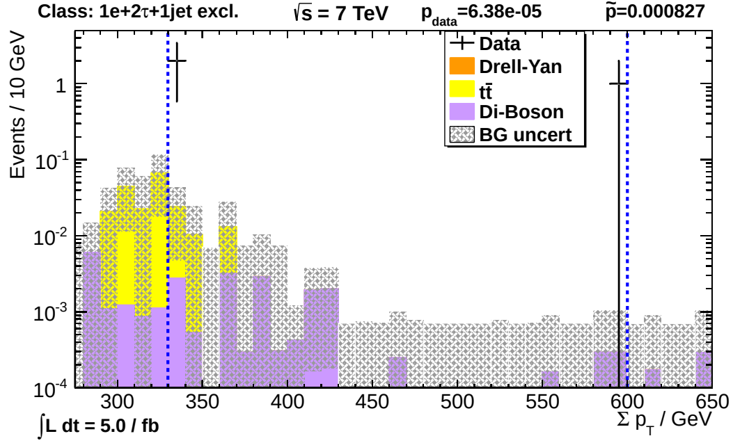
Figure 5.14: The \Sigma p_T distribution of the 1e+2\tau+1\text{jet} event class. The situation observed here is similar to the one observed in section 5.3.5.2. While the expectations is 0.057 \pm 0.035 events, 3 data events are observed.
