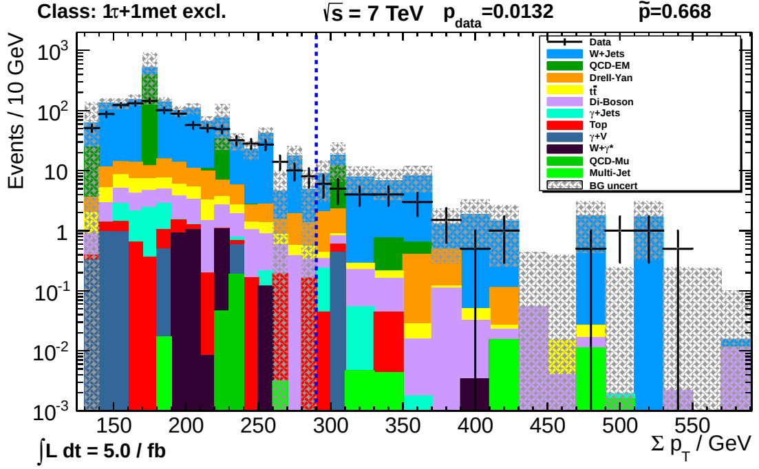
Figure 5.3: The \Sigma p_T distribution of the 1\tau + \text{MET} event class. Dominated by the W \rightarrow \tau \nu_\tau production this event class is the first to profit from the new triggering routine of MUSiC
