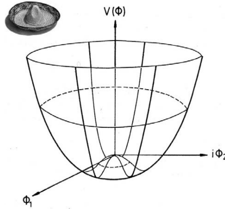
Figure 2.2: A sketch of the Higgs "Mexican Hat" potential as function of \phi_1 and \phi_2 [1]
