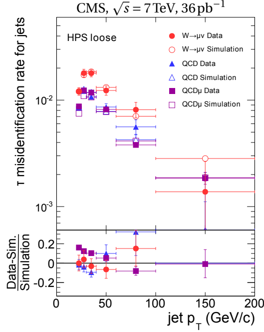
Figure 4.10: Misidentification rate for jets to be identified as \tau_{\text{had}} by the HPS algorithm as function of jet p_T . Starting around 2% at p_T \approx 30 GeV, the fake rate falls down to few times 10^{-3} for higher transverse momenta [41].
