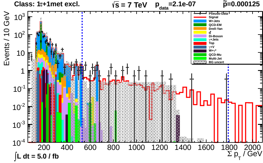
Figure 5.17: The \Sigma p_T distribution of the 1\tau + 1\text{MET} event class of the W' sensitivity study for m_{W'} = 2000 GeV. The last event in the region of interest rests upon a fill up uncertainty of \approx 10^{-4} which is not shown for demonstration purposes. The \tilde{p} indicates a significant deviation from the Monte Carlo prediction resulting in a very broad (over 1000 GeV) region of interest.
