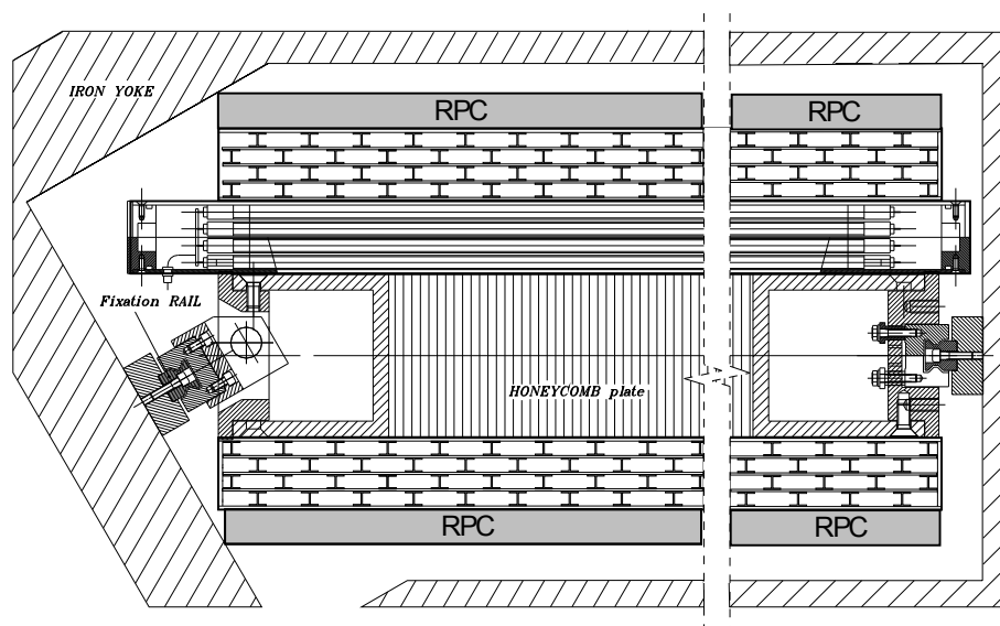
Figure 3.9: A DT chamber installed at CMS. RPCs attached to the DT chambers with plates are not shown [11]
