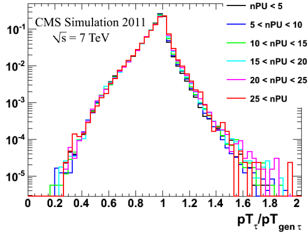
Figure 4.9: Resolution of 1-prong + 1\pi^0 \tau leptons coming from Z \rightarrow \tau^+ \tau^- for different pile-up scenarios – various number of soft interactions. The \tau energy scale is almost not affected by pile-up [44].
