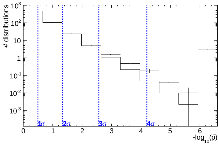
Figure 5.20: The \tilde{p} distribution for the sensitivity study summed up for all distributions \sum p_T , M^T and MET. A clear deviation is visible.
