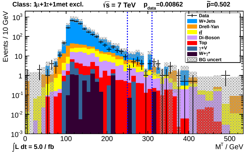
Figure 5.7: The transverse invariant mass distribution of 1\mu+1\tau+1\text{MET} . Unfortunately, the Z peak can not be resolved because of the large W background and the high cuts on the transverse missing energy, the p_T of the \tau and the trigger muon p_T .
