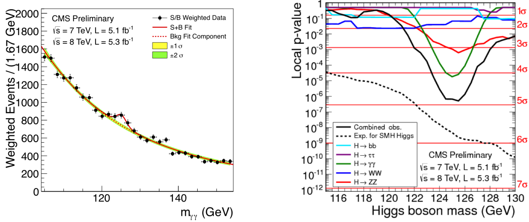
Figure 2.3: On the left: weighted number of observed events as a function of the invariant mass of two photons in the decay channel H \rightarrow \gamma\gamma On the right: the local significance of the combined hypothetical Higgs signal for different decay channels [6]
