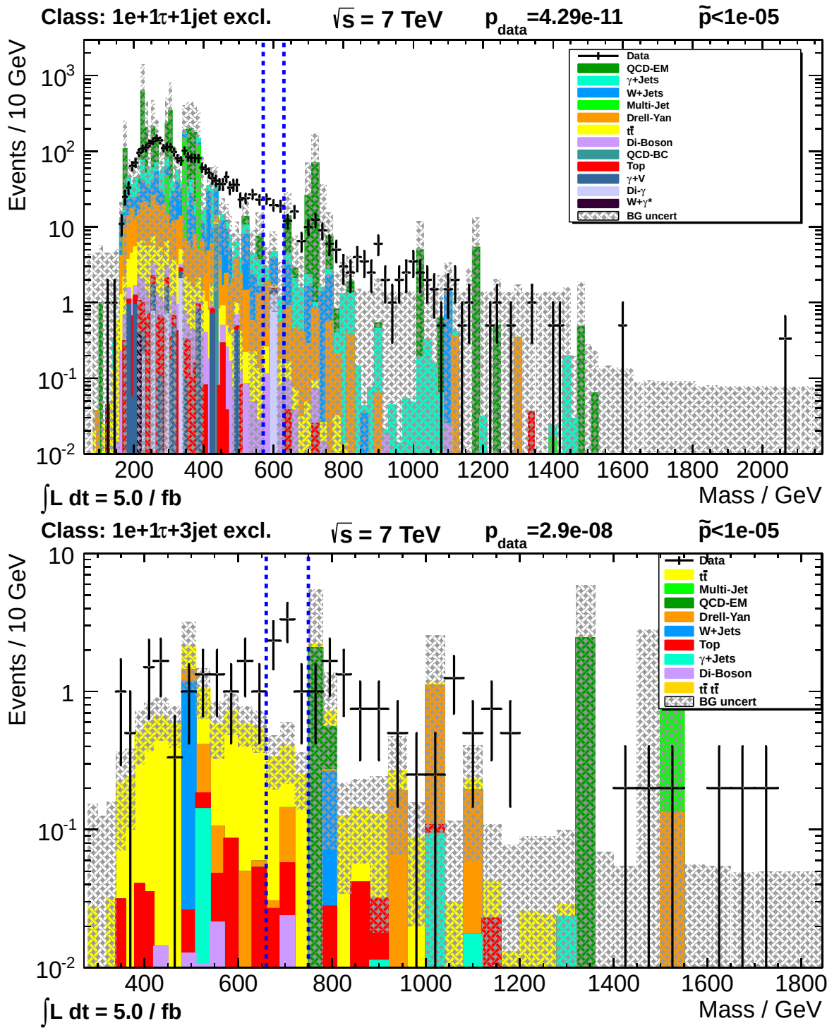
Figure 5.13: The invariant mass distributions of the 1e+1\tau+1\text{jet} (top) and 1e+1\tau+3\text{jet} (bottom) event classes. These event classes possess the highest significance out of all invariant mass distributions.
