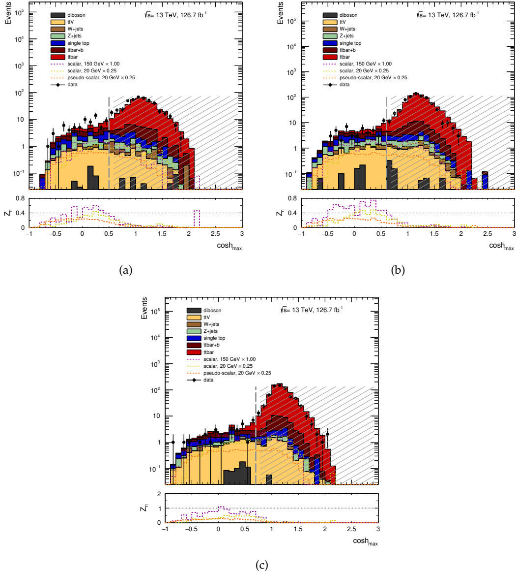
Figure 6.5.1: \cosh_{\max} distributions in (a) the resolved regime, (b) the boosted regime and (c) the highly boosted regime with all SR selections applied except for the \cosh_{\max} cut. The vertical dashed lines represent the selection value of \cosh_{\max} while the hatching lines indicate the direction of the cut. The distributions are shown before the profiling.
