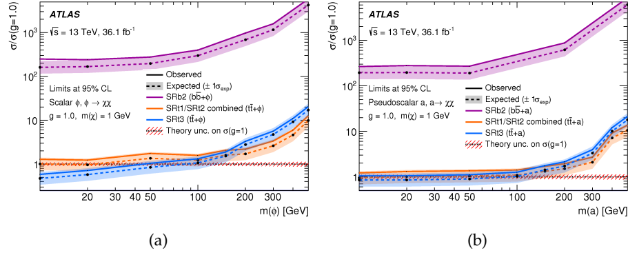
Figure 6.0.1: Observed limit on the signal strength, \mu , for (a) the scalar mediator and (b) the pseudo-scalar mediator simplified models as functions of the mediator mass, m_{\text{med}} , for a fixed DM particle mass, m_\chi = 1 GeV [71], obtained using 36.1 \text{ fb}^{-1} of pp collision data at \sqrt{s} = 13 TeV. The result in fully-hadronic (dileptonic) E_T^{\text{miss}} + t\bar{t} final state is shown as the orange (blue) line, while the result in E_T^{\text{miss}} + b\bar{b} final state is also shown in magenta.
