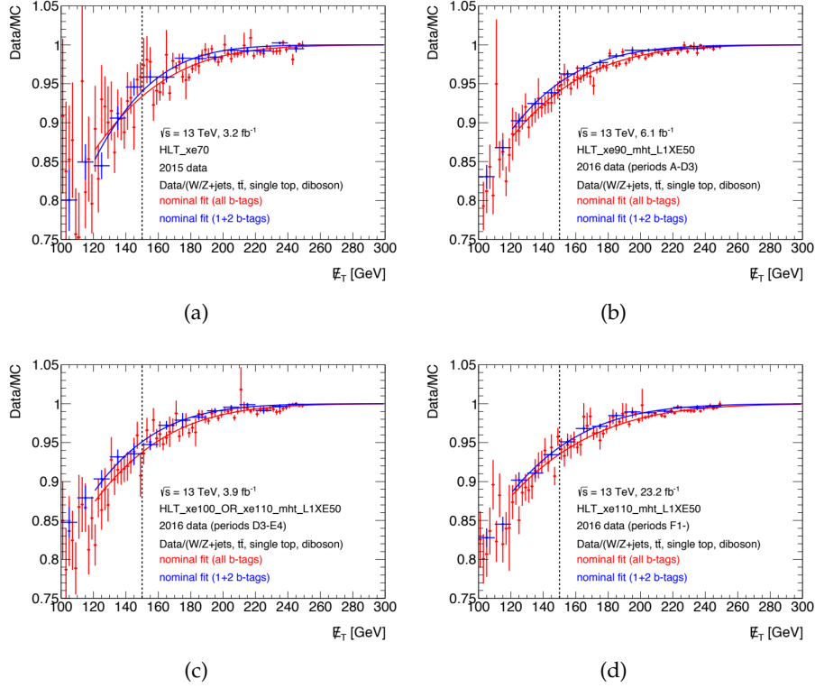
Figure 5.2.2: Comparisons between scale factors derived inclusively in b -tag multiplicity (red) and in events with \geq 1 b -jet (blue), as functions of E_{T,\text{no } \mu}^{\text{miss}} for (a) HLT_xe70, (b) HLT_xe90_mht_L1XE50, (c) HLT_xe100_mht_L1XE50 OR HLT_xe110_mht_L1XE50 and (d) HLT_xe110_mht_L1XE50.
