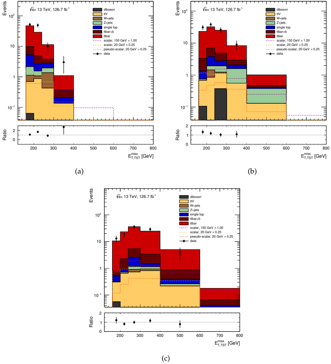
Figure 6.6.10: E_T^{\text{miss}} distributions in the (a) resolved, (b) boosted and (c) highly boosted t\bar{t} enriched validation regions. The distributions are shown before the profiling.
