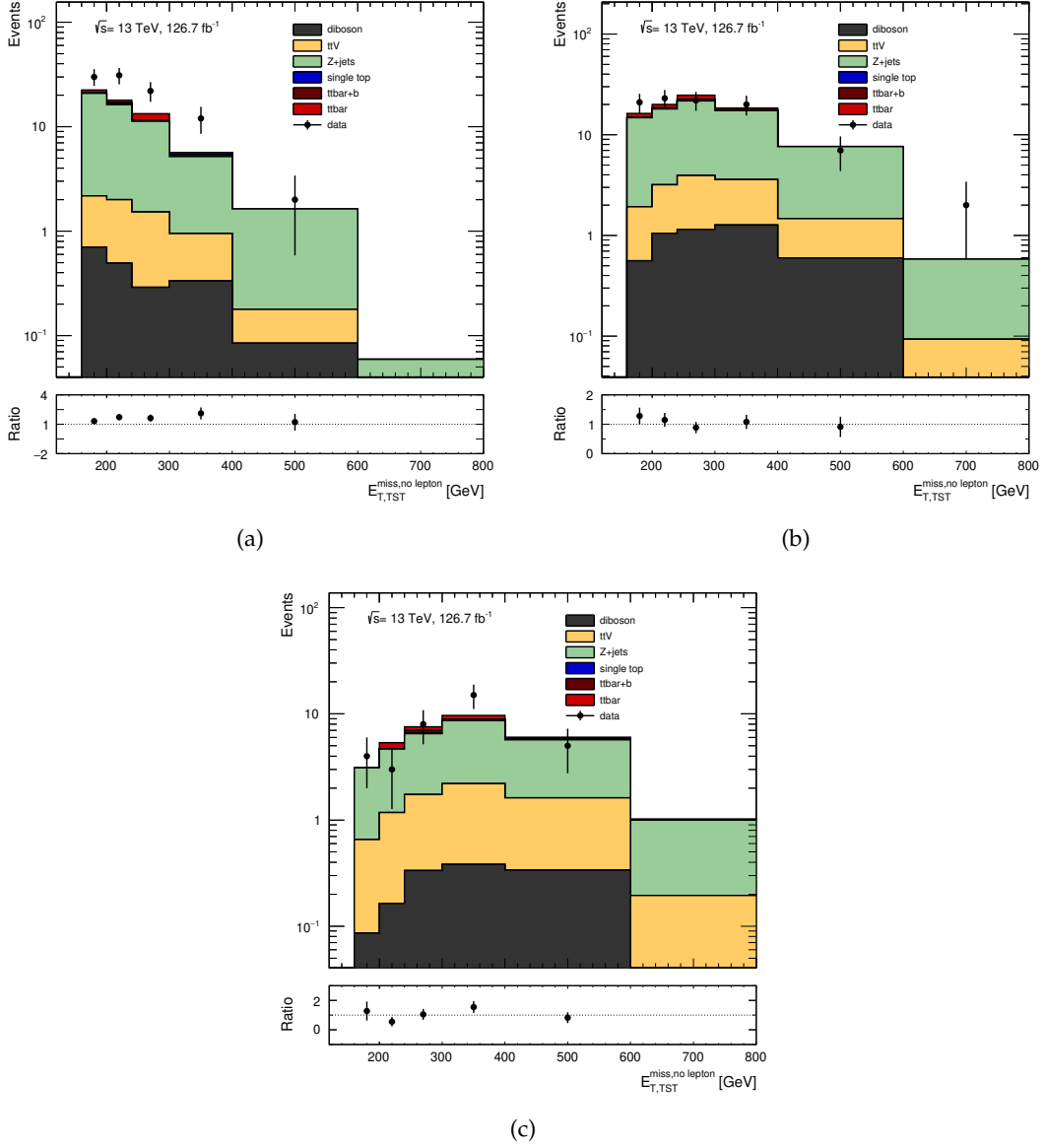
Figure 6.6.6: E_{T, \text{no lepton}}^{\text{miss}} distributions in the (a) resolved, (b) boosted and (c) highly boosted Z+jets enriched control regions. The distributions are shown before the profiling.
