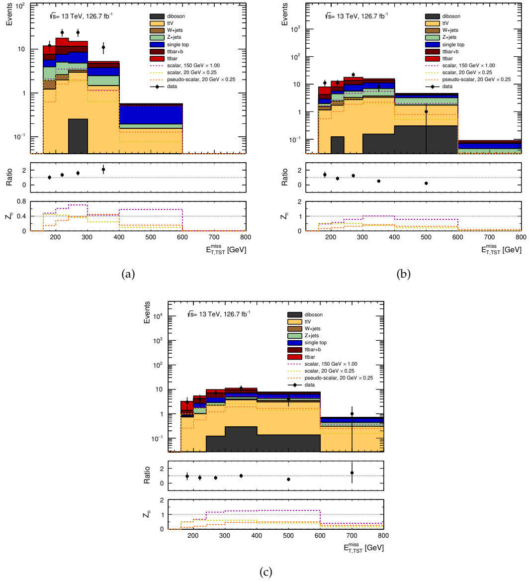
Figure 6.5.3: E_T^{\text{miss}} distributions in the (a) resolved, (b) boosted and (c) highly boosted signal regions. The distributions are shown before the profiling.
