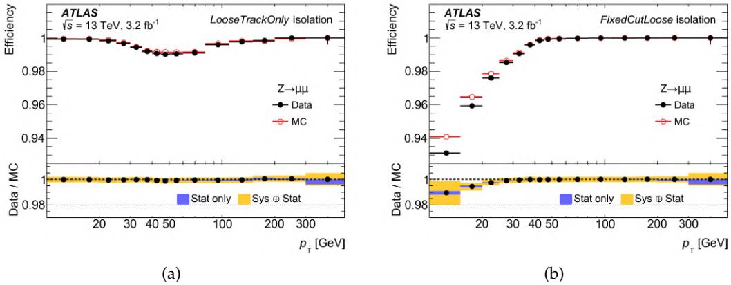
Figure 3.3.6: Muon isolation efficiency evaluated with simulated Z \rightarrow \mu\mu process for (a) LooseTrackOnly and (b) FixedCutLoose as functions of the candidate muon p_T [105]. The empty markers denote predictions given by the Monte Carlo simulation and the full markers denote the data observation.
