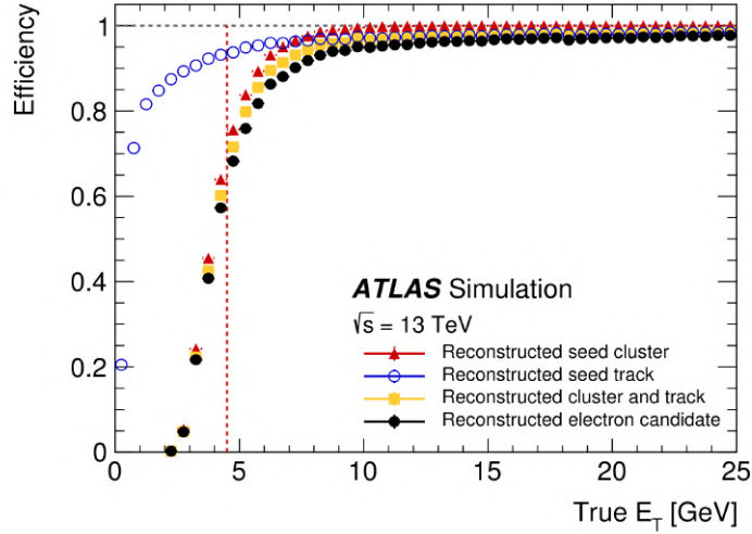
Figure 3.3.2: Reconstruction efficiency for simulated electrons in a single electron sample as a function of the truth-level transverse energy E_T for each step of the electron candidate formation [101]: cluster reconstruction (red triangles), track association (blue empty circles), track refit (yellow squares) and candidate reconstruction (black full circles).
