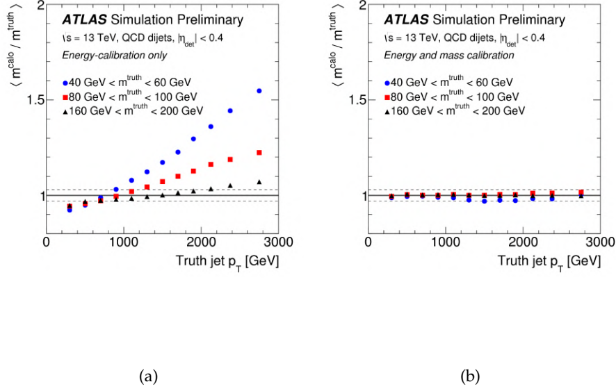
Figure 3.3.16: Average calorimeter-based mass response as functions of p_T^{\text{truth}} for large- R jets in bins of m^{\text{truth}} (a) before and (b) after the JMS calibration [128].
