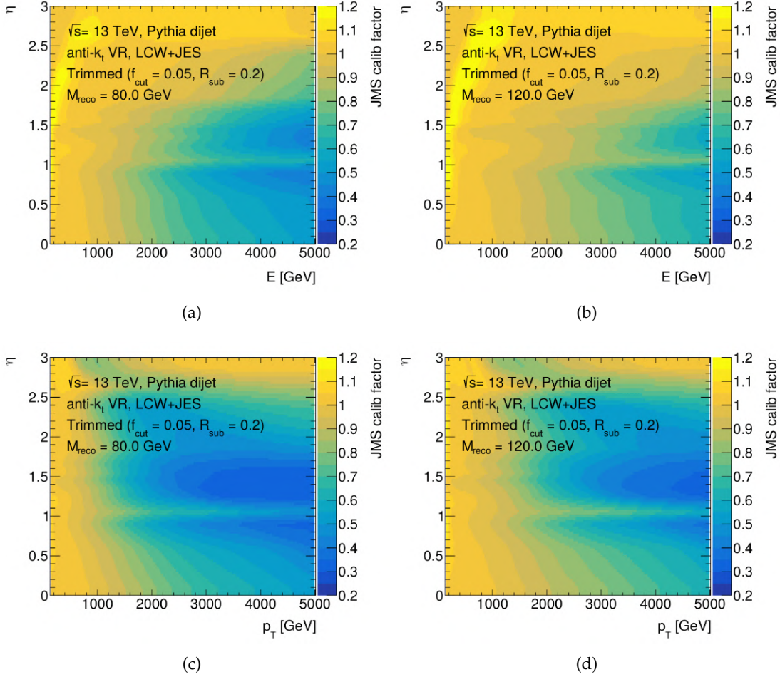
Figure 4.5.1: Calibration maps of the calorimeter-based mass for VR jets with m^{\text{calo}} = 80 GeV (left) and m^{\text{calo}} = 120 GeV (right) as functions of |\eta^{\text{calib}}| and E^{\text{calib}} (top) or p_T^{\text{calib}} (bottom).
