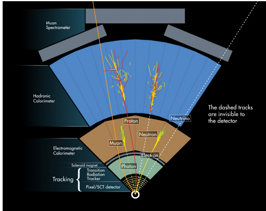
Figure 3.2.2: An illustration of the ATLAS detector in the transverse plane where different types of particles interact with the detector material in different layers [88]. The toroids are not plotted.
