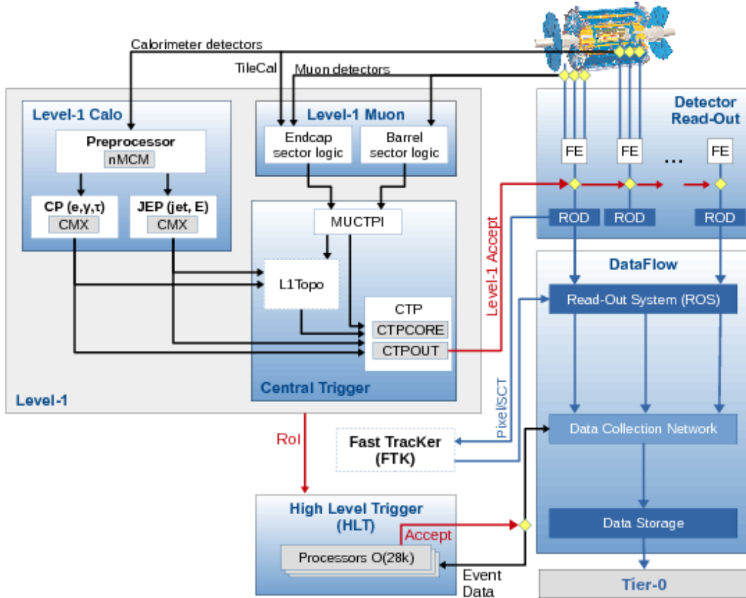
Figure 3.2.9: The ATLAS trigger and data acquisition system (TDAQ) in Run 2 [97]. The hardware-based level-1 (L1) triggers, including L1 Calo, L1 Muon and L1 Topo, and the software-based high-level triggers (HLT) together reduce the event rate from 40 MHz to 1 kHz. The L1 Topo system has been commissioned in 2017, while the FTK is currently being integrated into the ATLAS trigger system, aiming to improve the performance of particle identification at high luminosity.
