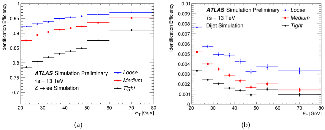
Figure 3.3.3: (a) Electron identification efficiency evaluated with simulated Z \rightarrow ee process and (b) the rate of misidentification where hadrons are identified as electrons evaluated with simulated dijet production for Loose (blue triangles), Medium (red squares) and Tight (black circles) as functions of the candidate electron E_T [103].
