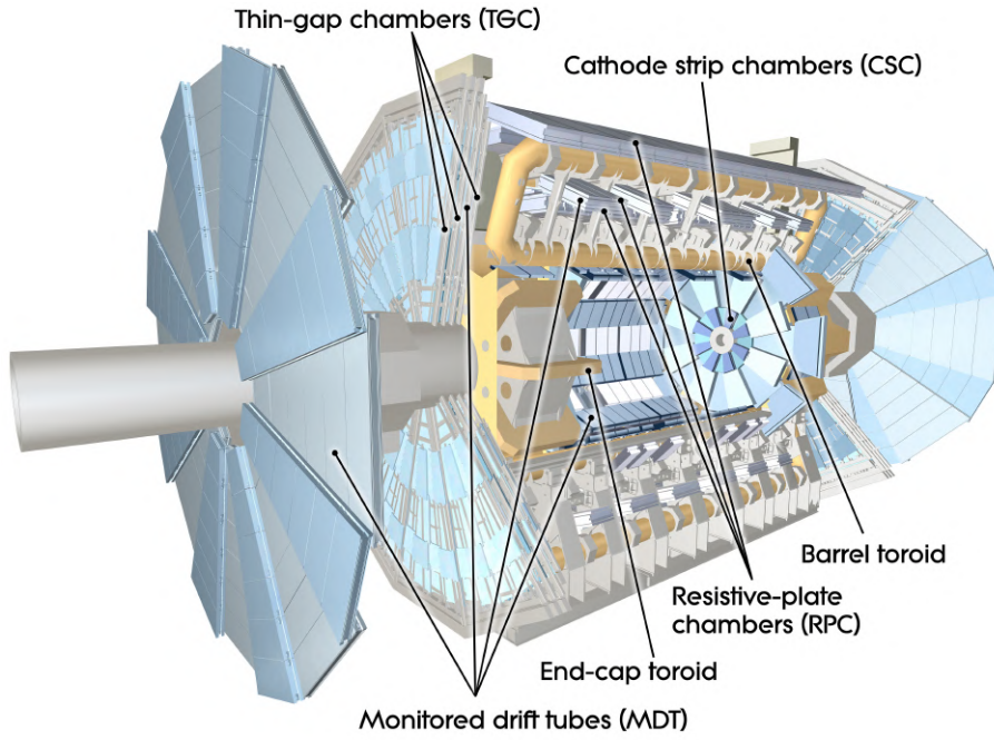
Figure 3.2.8: The general layout of the ATLAS Muon Spectrometer [96].
