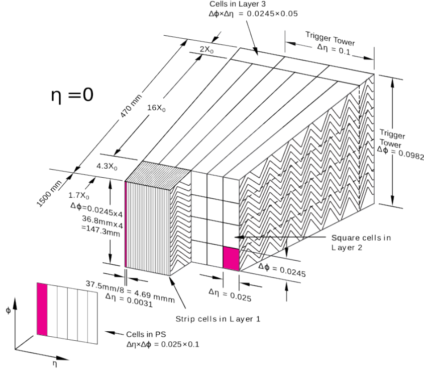
Figure 3.2.6: Sketch of a barrel module in the Electromagnetic Calorimeter at \eta = 0 [87]. The granularities of the cells in three different layers in \eta and \phi are also shown.
