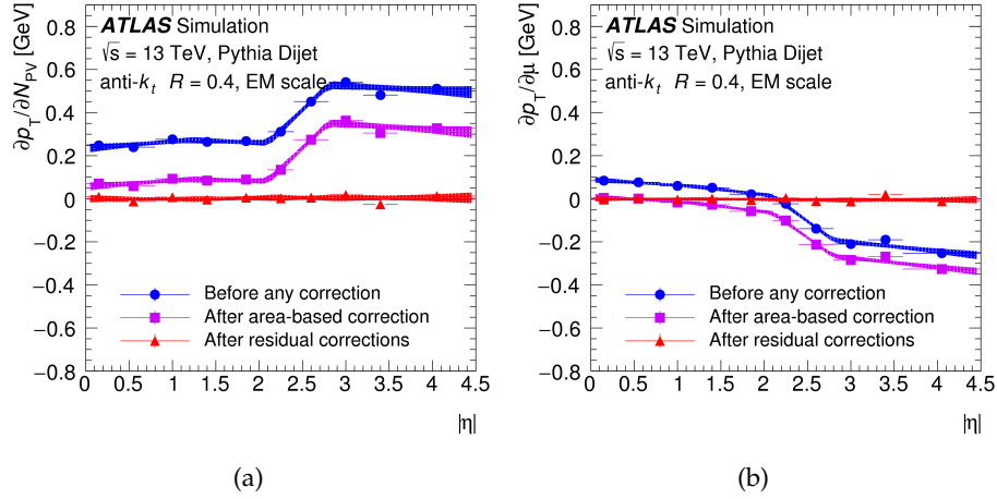
Figure 3.3.8: Dependence of small- R jets on (a) in-time and (b) out-of-time pile-up as functions of |\eta| with p_T^{\text{truth}} = 25 GeV before the pile-up corrections (blue circle), after the jet area-based correction (violet square) and after the residual correction (red triangle) [112].
