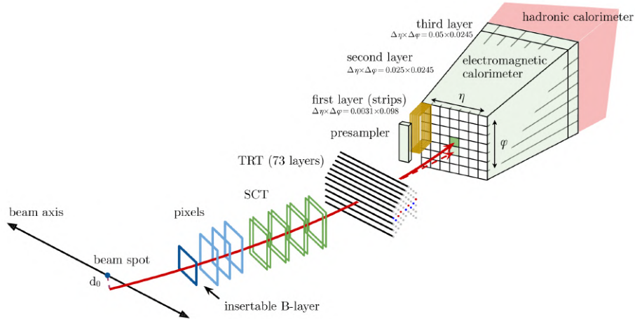
Figure 3.3.1: Illustration of the hypothetical path of an electron traversing the ATLAS detector [101]. The solid red trajectory represents the path of the electron, which first traverses the tracking system and then enters the ECal. The dashed red trajectory represents a secondary photon produced by the interaction between the incident electron and the detector material.
