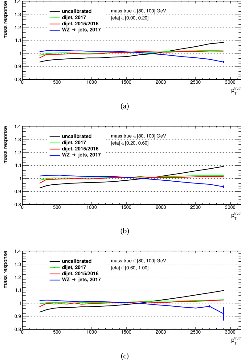
Figure 4.4.3: Average calibrated track-assisted mass response for VR jets with m_{\text{truth}} \in [80, 100] GeV and (a) |\eta| \in [0.0, 0.2] , (b) |\eta| \in [0.2, 0.6] , (c) |\eta| \in [0.6, 1.0] as functions of p_T^{\text{truth}} . The calibration is applied to PYTHIA dijet samples reweighted to match the pile-up condition in 2017 (green), dijet samples reweighted to match the pile-up condition in 2015 and 2016 (red) and W' \rightarrow WZ \rightarrow qqqq samples reweighted to match the pile-up condition in 2017 (blue). The uncalibrated response for PYTHIA dijet samples reweighted to match the pile-up condition in 2017 (black) is also drawn. The error bars shown in the plots correspond to the statistical uncertainty of the fit.
