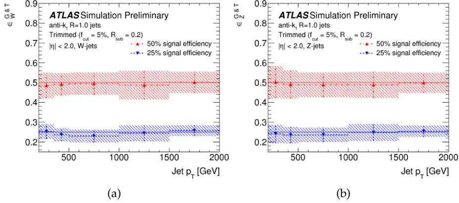
Figure 5.5.2: Signal efficiency versus p_T for large- R jets originating from (a) W bosons and (b) Z bosons with 25% (blue) and 50% (red) fixed-cut working point [160]. The combined systematic and statistical uncertainties are shown in shades.
