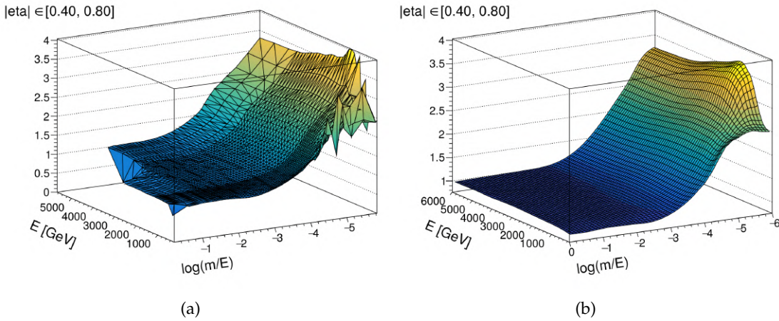
Figure 4.2.1: Average jet mass response \langle R_{\text{reco}} \rangle as functions of E^{\text{truth}} and \log(m^{\text{truth}}/E^{\text{truth}}) for uncalibrated VR jets with |\eta^{\text{truth}}| \in [0.4, 0.8] (a) before and (b) after the two dimensional Gaussian kernel smoothing.
