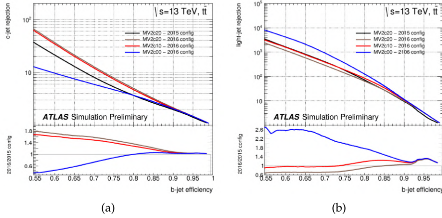
Figure 3.3.11: (a) c -jet and (b) light-flavor jet rejection versus b -tagging efficiency for MV2c10 (red) and MV2c20 (gray for 2016 configuration) [119].
