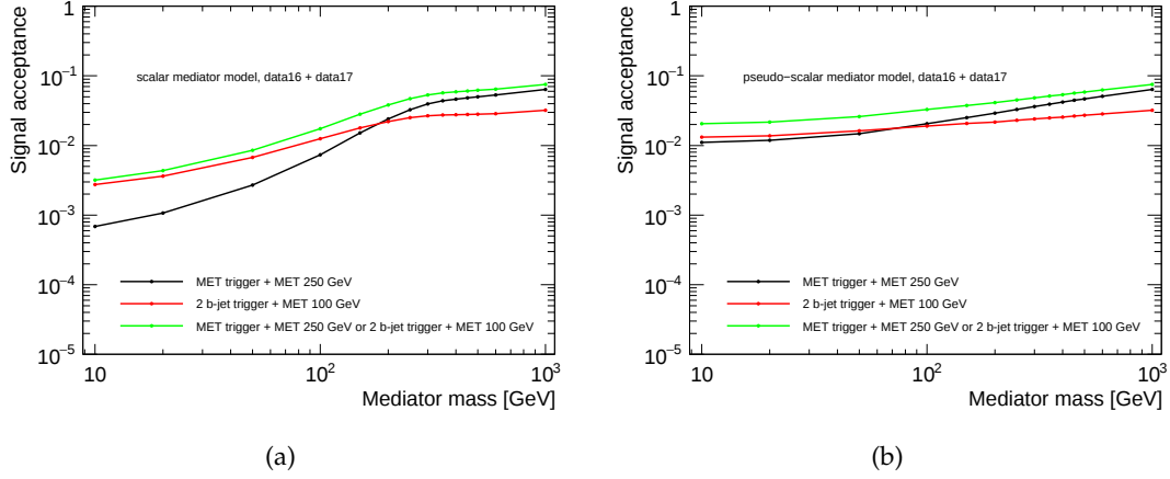
Figure 6.2.1: Signal acceptance after truth-level event selections as functions of m_{\text{med}} with a fixed m_{\chi} of 1 GeV for (a) the scalar mediator models and (b) the pseudo-scalar mediator models. Two medium (tight) b -jets are required in the b -jet trigger based selection to mimic the performance of the 2 b -jet + 2 jet trigger available in 2016 (2017). The combination of the b -jet trigger based selection in 2016 and 2017 is achieved by randomly assigning simulated signal events to either criterion with respect to the integrated luminosity of each year. Hence, any correlation due to double counting the same event in both selections can be avoided.
