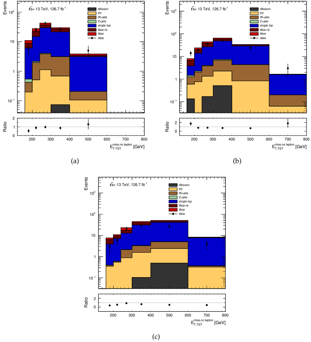
Figure 6.6.3: E_{T, \text{no lepton}}^{\text{miss}} distributions in the (a) resolved, (b) boosted and (c) highly boosted single top enriched control regions. The distributions are shown before the profiling.
