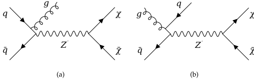
Figure 2.2.7: Feynman diagrams of DM production in association with a quark or a gluon under the description of a vector or axial-vector mediator simplified model.
