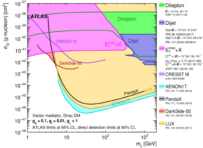
Figure 5.8.8: Exclusion on the spin-independent DM-nucleon scattering cross section as functions of m_\chi inferred from the constraints from the direct detection experiments at 90% CL and from the ATLAS limits at 95% CL [175]. Note that the comparison is valid solely in the context of the vector mediator simplified model with the couplings of the mediator to the SM and DM particles fixed to g_q = 0.1 , g_l = 0.01 and g_\chi = 1 .
