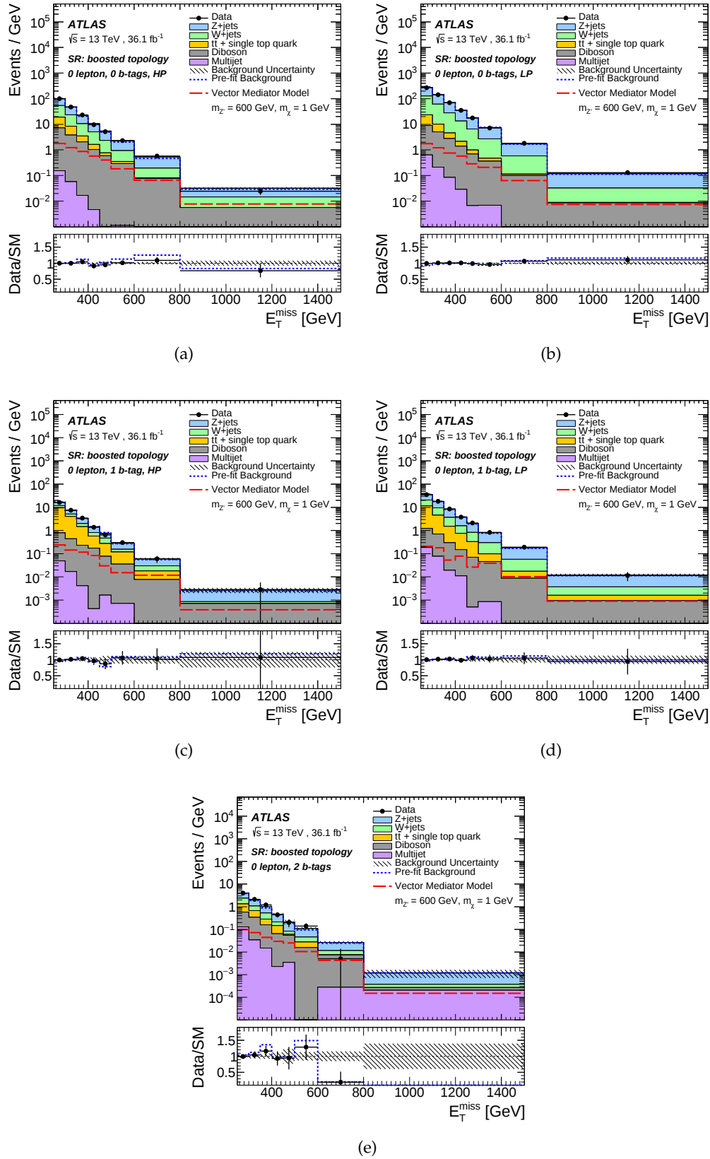
Figure 5.8.3: E_T^{\text{miss}} distributions after the combined profile likelihood fit in the boosted signal regions: (a) 0 b -tag high purity signal region, (b) 0 b -tag low purity signal region, (c) 1 b -tag high purity signal region, (d) 1 b -tag low purity signal region and (e) 2 b -tag high purity signal region [1].
