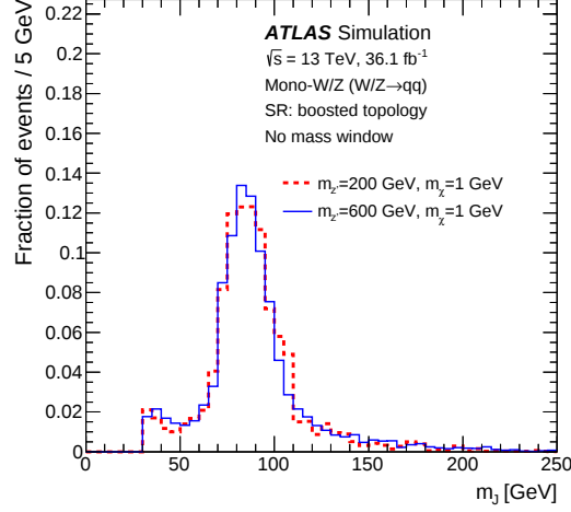
Figure 5.5.1: Expected invariant mass distributions of the leading large- R jet, normalized to unit area, for the vector mediator simplified model with m_{\text{med}} = 200 GeV (dashed red) and 600 GeV (solid blue) in the boosted regime [1].
