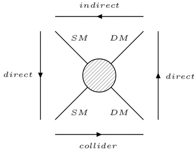
Figure 2.2.6: A simple illustration of the physical processes probed by the three types of DM searches. From top to bottom (bottom to top) is the scattering between the SM and DM particles (direct detection search). From right to left is the SM production via DM self-annihilation (indirect detection search). From left to right is the DM pair production at high energy colliders (collider search).
