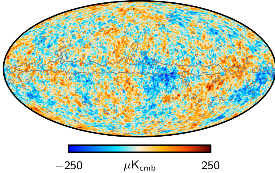
Figure 2.2.4: Commander CMB temperature map derived from the Planck 2015, nine-year WMAP and 408 MHz Haslam observations [30] et al.
