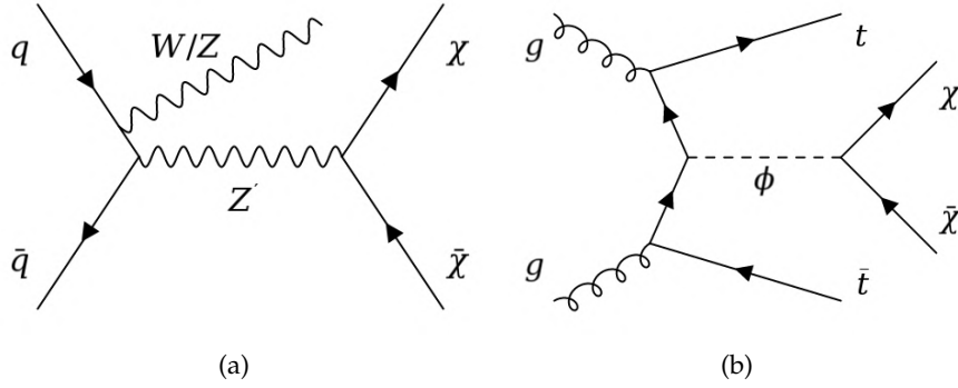
Figure 2.2.9: (a) Feynman diagram of DM production in association with a W or Z boson under the description of vector or axial-vector mediator simplified model. (b) Feynman diagram of DM production in association with a pair of top quarks under the description of scalar or pseudo-scalar mediator simplified model.
