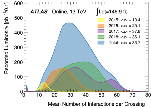
Figure 3.1.3: Luminosity weighted distribution of the mean number of interactions per crossing recorded by ATLAS for pp collisions at 13 TeV center-of-mass energy from 2015 to 2018 [86].
