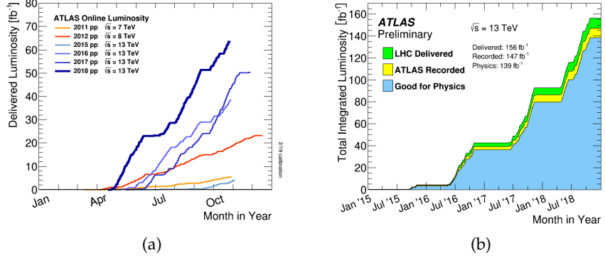
Figure 3.1.2: (a) Integrated luminosity versus time delivered to ATLAS during stable beams for high energy pp collisions in 2011 - 2018 and (b) integrated luminosity versus time delivered to ATLAS (green), recorded by ATLAS (yellow), and certified to be good quality data (blue) during stable beams for pp collisions at 13 TeV center-of-mass energy from 2015 to 2018 [86].
