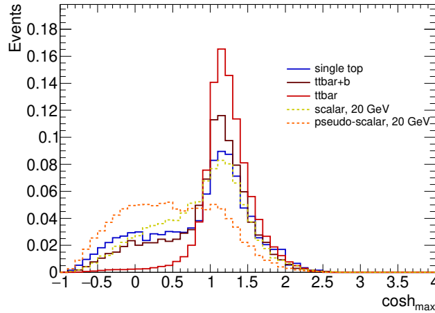
Figure 6.3.1: \cosh_{\max} distribution for t\bar{t} (solid red), t\bar{t} + b (solid brown) and single top (solid blue) backgrounds, normalized to unit area. The scalar mediator (dashed yellow) and the pseudo-scalar mediator (dashed orange) models are plotted alongside. The broad peak visible for the scalar model comes from the semi-leptonically decaying signal events with the lepton being either lost or misidentified as a jet. This is not a part of the phase space expected to be constrained by the E_T^{\text{miss}} + t\bar{t} (fully-hadronic) search.
