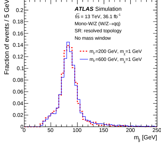
Figure 5.5.3: Expected invariant mass distributions of the leading two central jets, normalized to unit area, for the vector mediator simplified models with m_{\text{med}} = 200 GeV (dashed red) and 600 GeV (solid blue) in the resolved regime [1].
