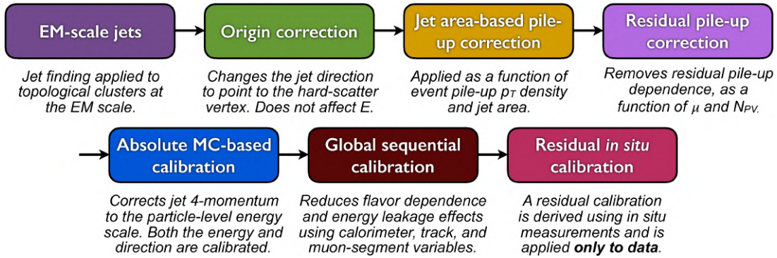
Figure 3.3.7: Overview of the sequential calibration scheme for small- R jets [112]. All corrections are applied to the four-momentum of the jet as scale factors, except for the origin correction which recalculates the jet direction in order to point to the hard-scatter PV while keeping the jet energy unchanged.
