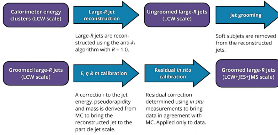
Figure 3.3.14: Overview of the reconstruction, grooming and calibration for large- R jets [125]. The calorimeter energy clusters from which jets are reconstructed have already been adjusted to point towards the hard-scatter PV.
