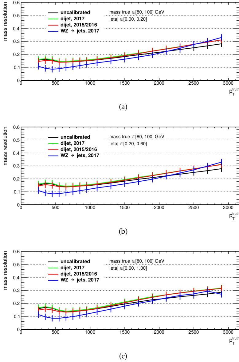
Figure 4.4.2: Average calibrated calorimeter-based mass resolution for VR jets with m_{\text{truth}} \in [80, 100] GeV and (a) |\eta| \in [0.0, 0.2] , (b) |\eta| \in [0.2, 0.6] , (c) |\eta| \in [0.6, 1.0] as functions of p_T^{\text{truth}} . The calibration is applied to PYTHIA dijet samples reweighted to match the pile-up condition in 2017 (green), dijet samples reweighted to match the pile-up condition in 2015 and 2016 (red) and W' \rightarrow WZ \rightarrow qqqq samples reweighted to match the pile-up condition in 2017 (blue). The uncalibrated resolution for PYTHIA dijet samples reweighted to match the pile-up condition in 2017 (black) is also drawn. The error bars shown in the plots correspond to the statistical uncertainty of the fit.
