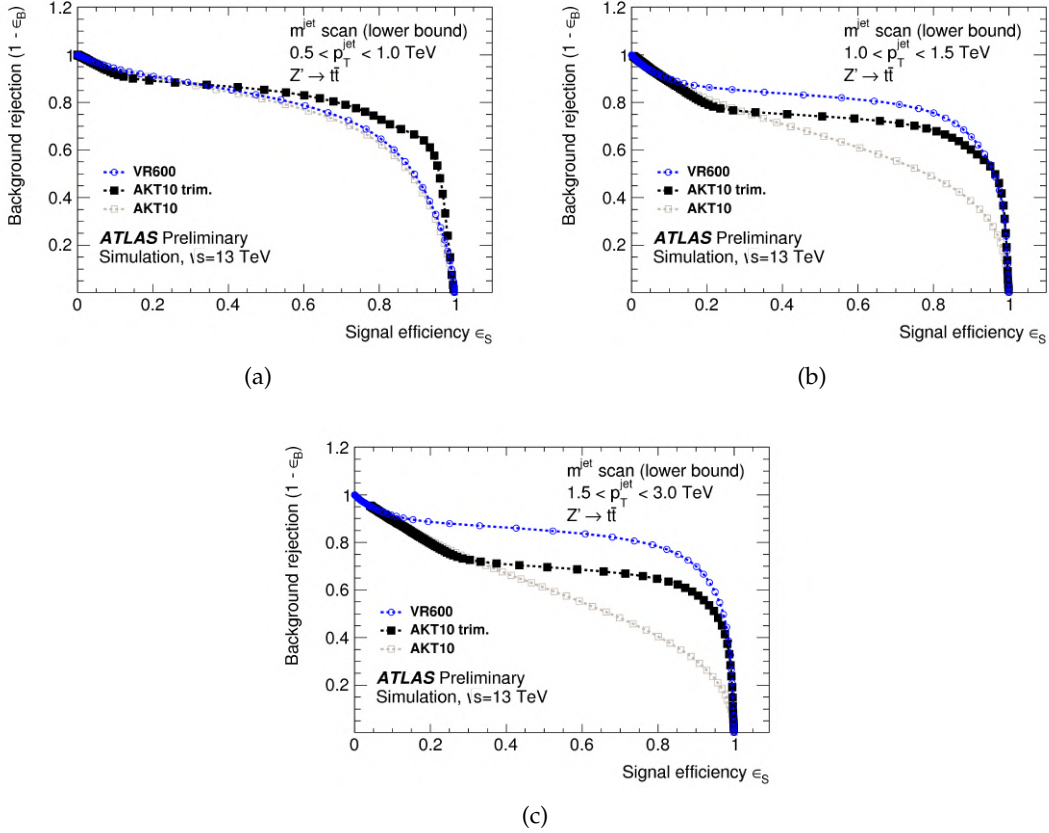
Figure 4.1.1: Background rejection versus signal efficiency evaluated with simulated Z' signal and dijet background [141]. The performances are shown for ungroomed VR jets (blue circles), trimmed large- R jets (black full squares) and ungroomed large- R jets (gray empty squares) in events with (a) 0.5 \text{ TeV} < p_T^{\text{jet}} < 1.0 \text{ TeV} , (b) 1.0 \text{ TeV} < p_T^{\text{jet}} < 1.5 \text{ TeV} and (c) 1.5 \text{ TeV} < p_T^{\text{jet}} < 3.0 \text{ TeV} . The curves are obtained by varying the value of a hypothetical lower bound on the jet mass.
