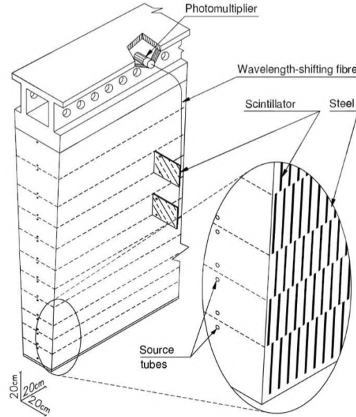
Figure 3.2.7: Sketch of a barrel module in the Tile Calorimeter [87], showing the major components of the optical read-out, including the tiles, the fibers and the PMTs.
