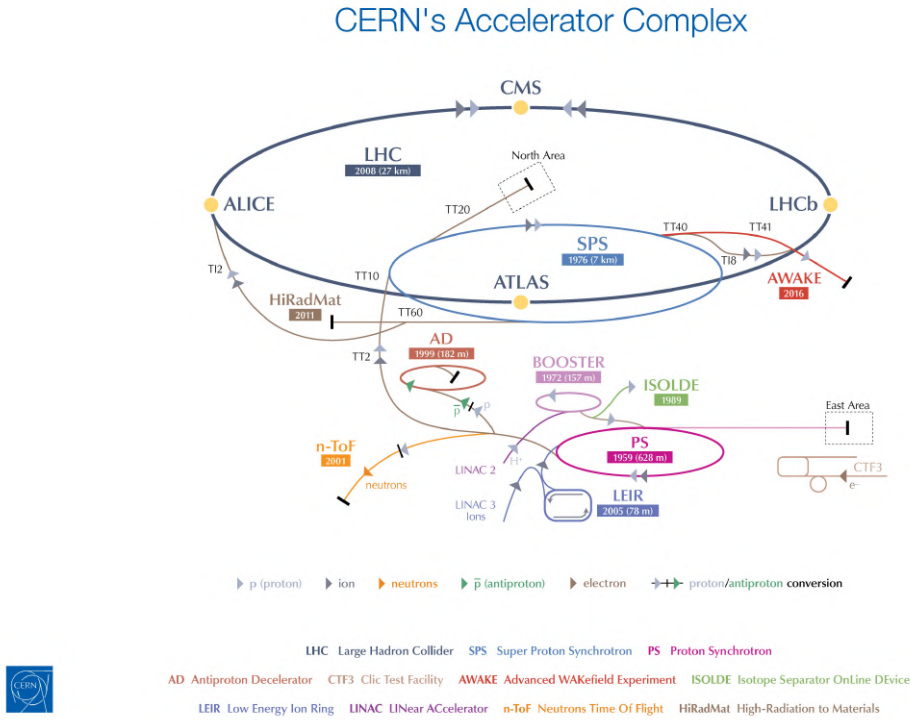
Figure 3.1.1: Illustration of the LHC accelerator complex. The beam acceleration starts at LINAC 2 and then through the Proton Synchrotron Booster (BOOSTER), the Proton Synchrotron (PS), the Super Proton Synchrotron (SPS) and finally the LHC [84]. The beams cross at four interaction points located along the LHC ring where the four major experiments take place, while the other three smaller experiments are not shown in the plot.
