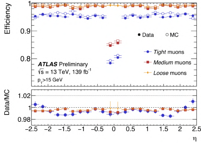
Figure 3.3.5: Muon identification efficiency evaluated with simulated Z \rightarrow \mu\mu process for Loose (orange diamonds), Medium (red squares) and Tight (blue circles) as functions of the candidate muon \eta [104]. The empty markers denote predictions given by the Monte Carlo simulation and the full markers denote the data observation.
