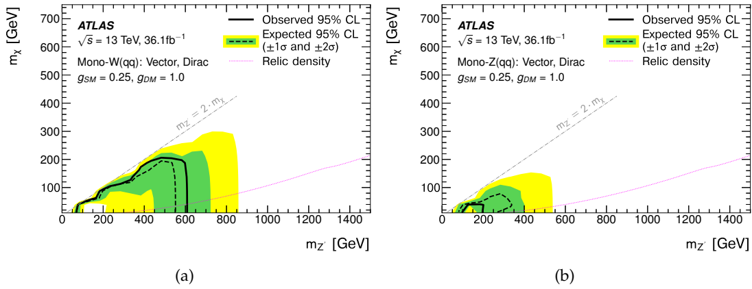
Figure 5.8.5: Exclusion limits on the Dark Matter production in association with (a) a W boson and (b) a Z boson for the vector mediator simplified model in the m_\chi - m_{\text{med}} plane [1]. The couplings of the mediator to the SM and DM particles are fixed to g_q = 0.25 and g_\chi = 1 , following the recommendations of the dark matter forum [147]. The solid (dashed) black curve shows the median of the observed (expected) exclusion limit, while the filled green (yellow) band denotes the \pm 1\sigma ( \pm 2\sigma ) uncertainties on the expected result. The dotted magenta line represents the mass points for which the expected DM relic density is consistent with the WMAP [173] and Planck [29] measurements ( \Omega_{\text{DM}} h^2 = 0.1186 \pm 0.0020 ), computed with MadDM [174]. The region on the right of the curve corresponds to higher predicted relic abundance.
