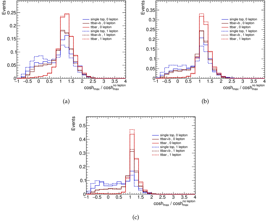
Figure 6.6.4: Shape of \cosh_{\max} in 0 lepton final state (solid lines) and \cosh_{\max}^{\text{no lepton}} in 1 lepton final state (dashed lines), normalized to unit area, for t\bar{t} (red), t\bar{t} + b (brown) and single top (blue) processes after the baseline selection and the anti-QCD requirements applied in (a) the resolved regime, (b) the boosted regime and (c) the highly boosted regime.
