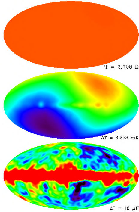
Figure 2.2.3: Four-year DMR sky maps [36] measured at the 53 GHz band and smoothed to an effective angular resolution of 10 degrees. The top map is plotted on a scale from 0 - 4 K, showing the near-uniformity of the CMB temperature. The middle map is plotted on a scale intended to enhance the contrast due to the dipole anisotropy. The bottom map is the CMB distribution after subtracting the dipole component.
