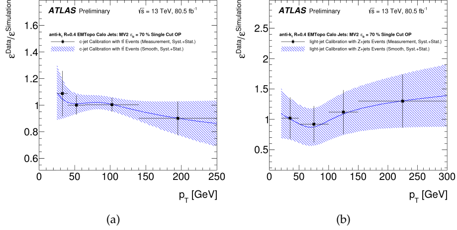
Figure 3.3.13: (a) Corrections on c -jet mistag rate of MV2 algorithm for small- R jets with a 70% fixed-cut working point evaluated with simulated t\bar{t} events using a likelihood fit [121]. (b) Corrections on light-flavor jet mistag rate of MV2 algorithm for small- R jets with a 70% fixed-cut working point evaluated with simulated Z +jets events using a negative-tag method [122]. The plots are taken from Ref. [123].
