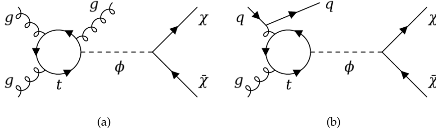
Figure 2.2.8: Feynman diagrams of DM production in association with a quark or a gluon under the description of a scalar or pseudo-scalar mediator simplified model.
