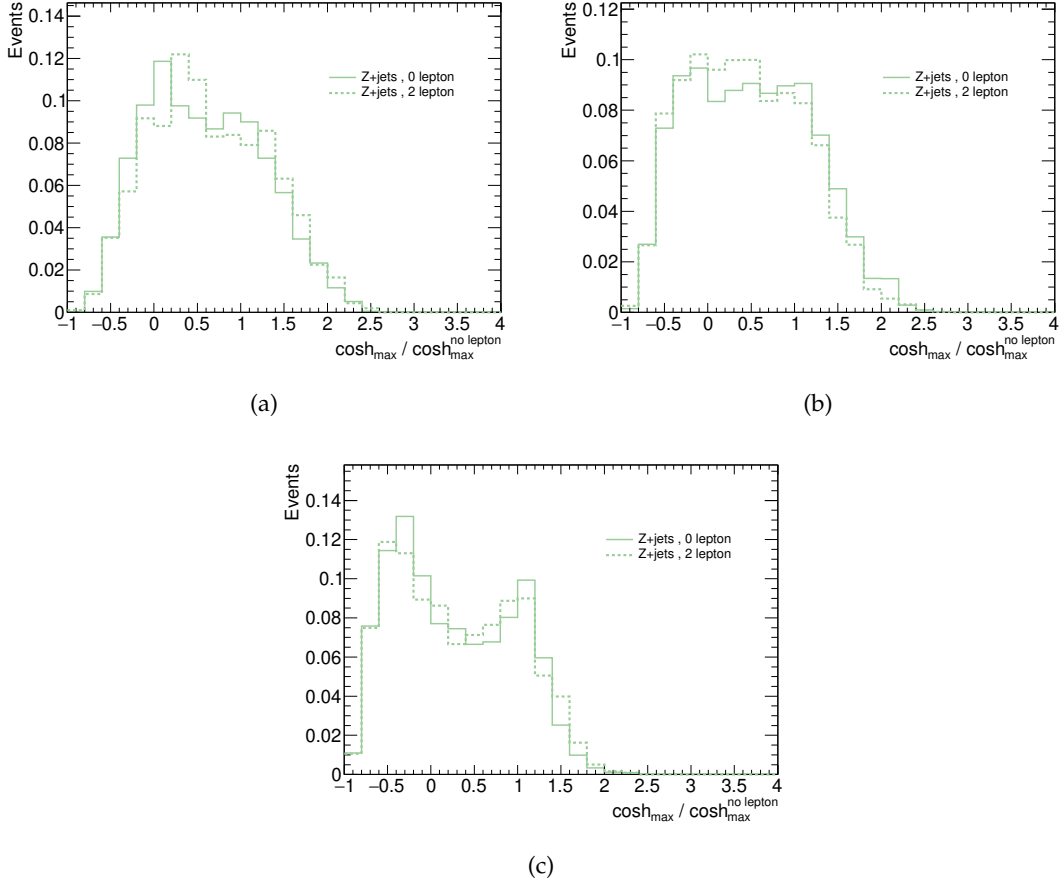
Figure 6.6.8: Shape of \cosh_{\max} in 0 lepton final state (solid lines) and \cosh_{\max}^{\text{no lepton}} in 2 lepton final state (dashed lines), normalized to unit area, for Z+jets process after the baseline selection and the anti-QCD requirements applied in (a) the resolved regime, (b) the boosted regime and (c) the highly boosted regime.
