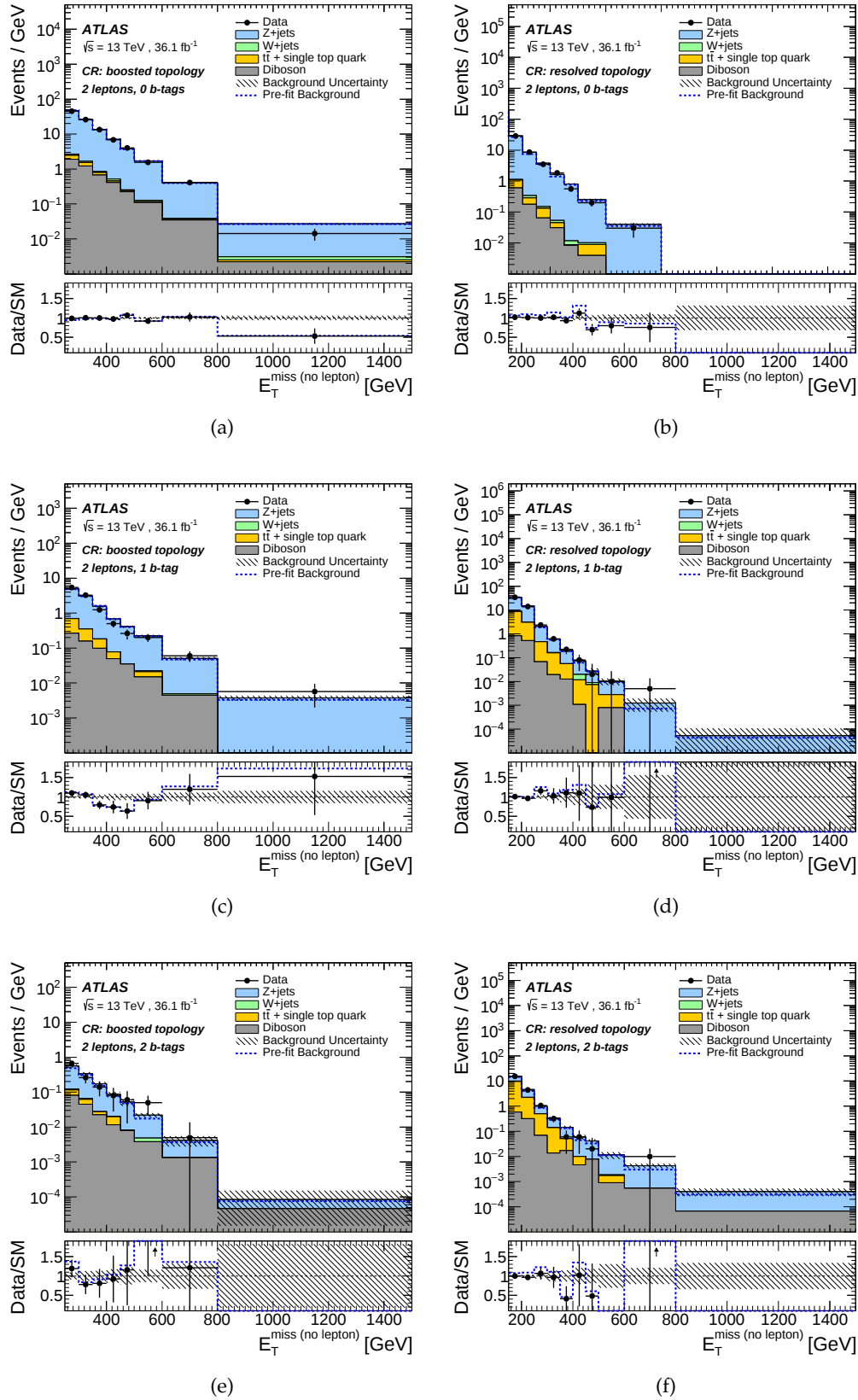
Figure 5.8.2: E_T^{\text{miss}} distributions after the combined profile likelihood fit in the boosted (left) and the resolved (right) 2 lepton control regions with 0 b-tag (top), 1 b-tag (middle) and 2 b-tag (bottom) [1].
