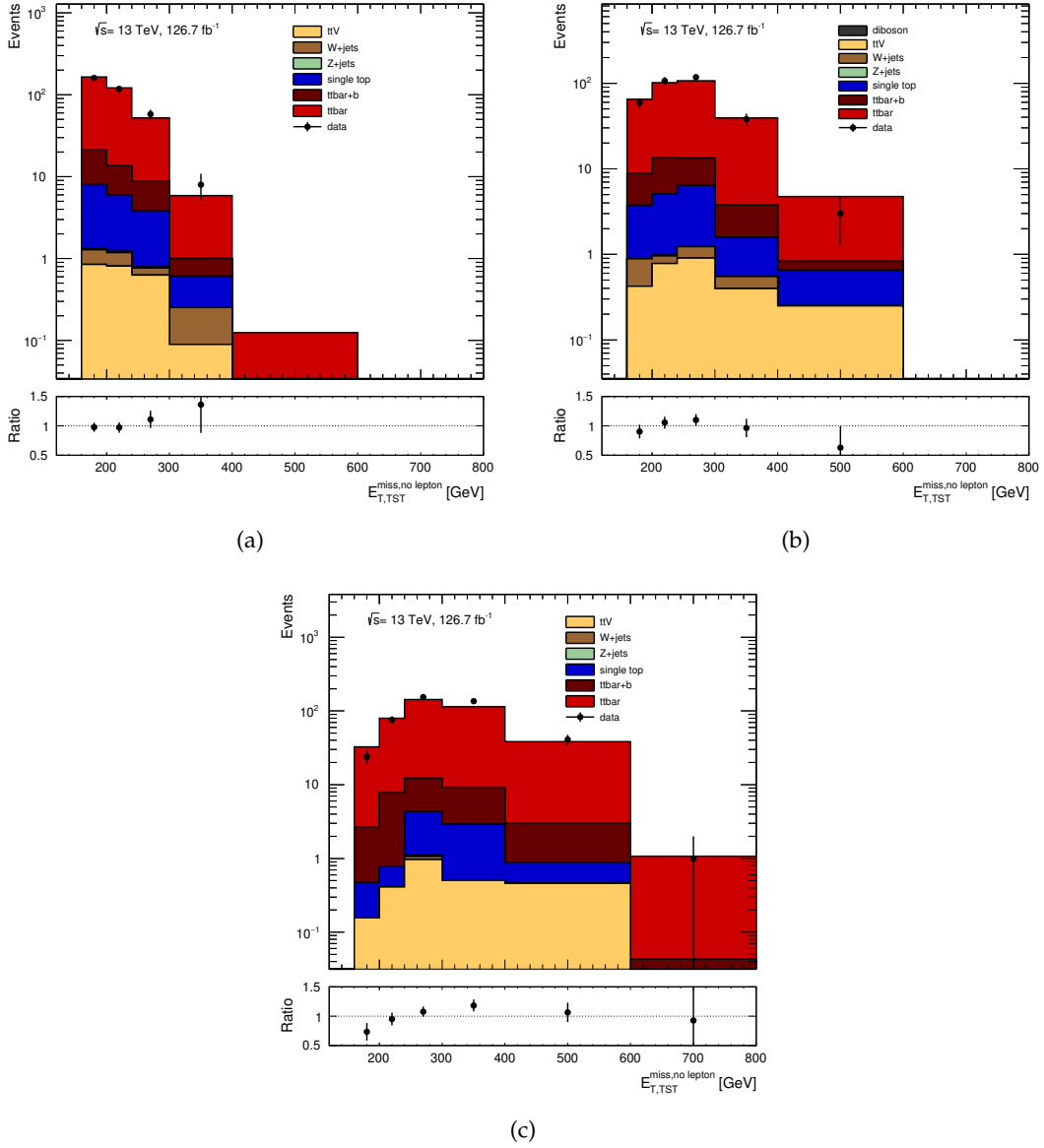
Figure 6.6.1: E_{T, \text{no lepton}}^{\text{miss}} distributions in the (a) resolved, (b) boosted and (c) highly boosted t\bar{t} enriched control regions. The distributions are shown before the profiling.
