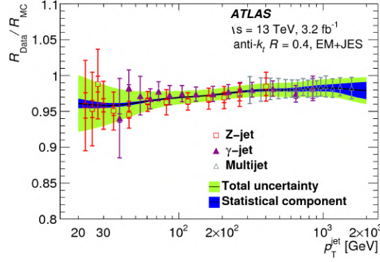
Figure 3.3.10: Ratio of the EM+JES jet response between data and MC simulation as functions of jet p_T for Z+jet, \gamma +jet, and multijet in-situ calibrations [112]. The final correction (black) and its statistical (dark blue) and total (light green) uncertainty are also shown.
