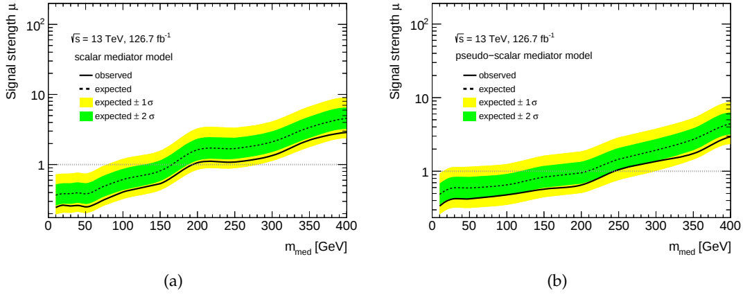
Figure 6.8.3: Exclusion limits on the Dark Matter production in association with fully-hadronic t\bar{t} for (a) the scalar mediator simplified model and (b) the pseudo-scalar mediator simplified model as functions of the mediator mass m_{\text{med}} for a fixed DM mass m_\chi = 1 GeV. The couplings of the mediator to the SM and DM particles are fixed to g = g_\chi = g_q = 1 , following the recommendations of the dark matter forum [147]. The solid (dashed) black curve shows the median of the observed (expected) exclusion limit, while the filled green (yellow) band denotes the \pm 1\sigma ( \pm 2\sigma ) uncertainties on the expected result.
