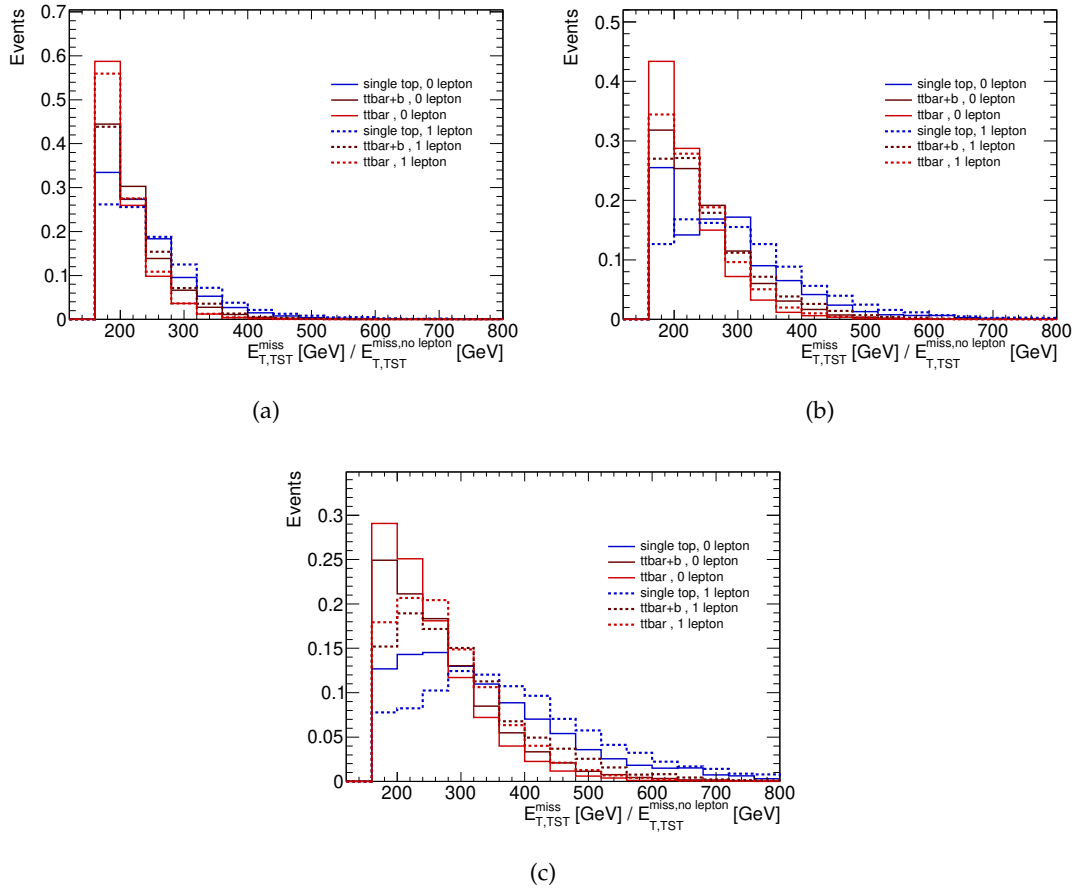
Figure 6.6.5: Shape of E_T^{\text{miss}} in 0 lepton final state (solid lines) and E_T^{\text{miss}} in 1 lepton final state (dashed lines), normalized to unit area, for t\bar{t} (red), t\bar{t} + b (brown) and single top (blue) processes after the baseline selection, the anti-QCD requirements and the leptonic top reconstruction cut applied in (a) the resolved regime, (b) the boosted regime and (c) the highly boosted regime.
