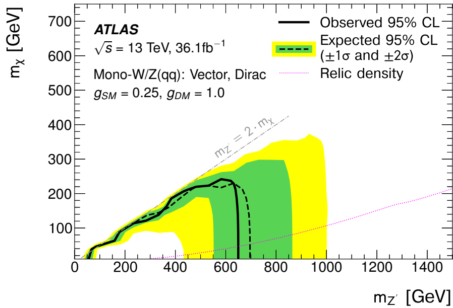
Figure 5.8.6: Exclusion limits on the Dark Matter production in association with a W/Z boson for the vector mediator simplified model in the m_{\chi} - m_{\text{med}} plane [1]. The couplings of the mediator to the SM and DM particles are fixed to g_q = 0.25 and g_{\chi} = 1 , following the recommendations of the dark matter forum [147]. The solid (dashed) black curve shows the median of the observed (expected) exclusion limit, while the filled green (yellow) band denotes the \pm 1\sigma ( \pm 2\sigma ) uncertainties on the expected result. The dotted magenta line represents the mass points for which the expected DM relic density is consistent with the WMAP [173] and Planck [29] measurements ( \Omega_{\text{DM}} h^2 = 0.1186 \pm 0.0020 ), computed with MadDM [174]. The region on the right of the curve corresponds to higher predicted relic abundance.
