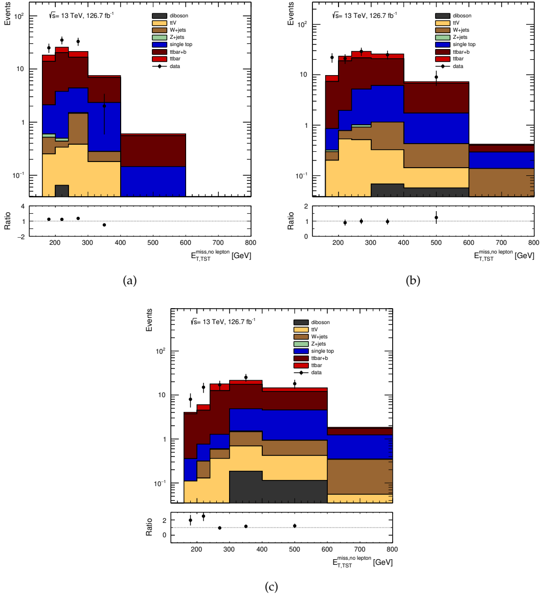
Figure 6.6.2: E_{T, \text{no lepton}}^{\text{miss}} distributions in the (a) resolved, (b) boosted and (c) highly boosted t\bar{t} + b enriched control regions. The distributions are shown before the profiling.
