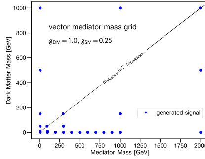
Figure 5.1.1: Grid of generated signal model samples with different configurations for mediator mass m_{\text{med}} and DM mass m_\chi .
