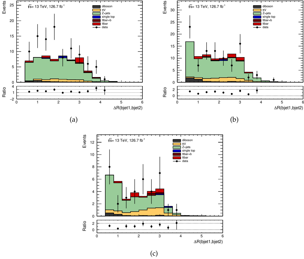
Figure 6.6.7: \Delta R(b_1, b_2) distributions in the (a) resolved, (b) boosted and (c) highly boosted Z+jets enriched control regions. The distributions are shown before the profiling.
