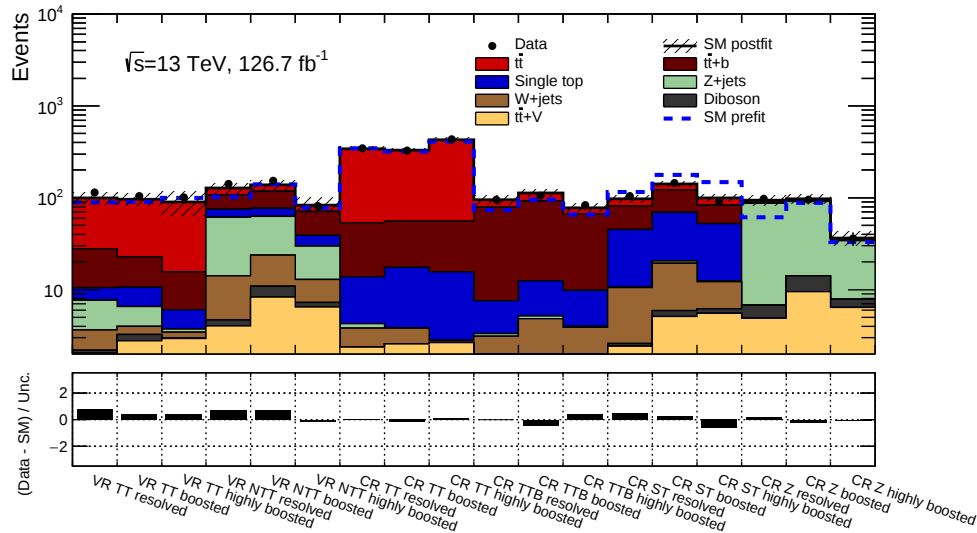
Figure 6.8.1: Event yield in all validation regions and control regions after the ‘background-only’ fit. The stacked histograms show the SM prediction and the hatched uncertainty band around the SM prediction corresponds to the total MC uncertainty, which consists of the MC statistical uncertainty, experimental systematic uncertainties and theoretical systematic uncertainties. The dotted blue line denotes the MC prediction before the background-only fit. The lower band shows the deviation between observation and prediction with respect to the total uncertainty, which consists of the total MC uncertainty and the data statistical uncertainty.
