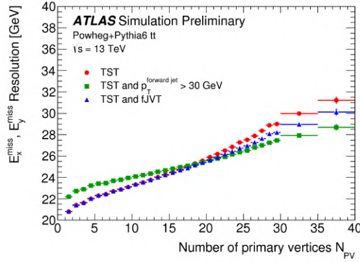
Figure 3.3.19: E_T^{\text{miss}} resolution as functions of the number of primary vertices ( N_{\text{PV}} ) evaluated with simulated semi-leptonically decaying t\bar{t} events [136]. Three E_T^{\text{miss}} definitions are shown, differing only in the forward jet selection. Red circles denote E_T^{\text{miss}} reconstructed with the Loose working point, where the input forward jets are required to have p_T > 20 GeV. Green squares denote E_T^{\text{miss}} reconstructed with the Tight working point, where the p_T selection for forward jets is tightened to 30 GeV. Blue triangles denote E_T^{\text{miss}} reconstructed with the Loose working point with additional fJVT requirements.
