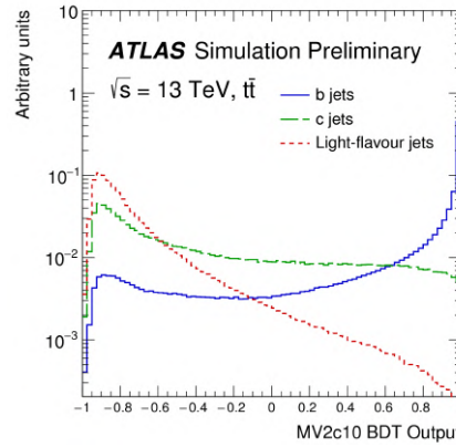
Figure 3.3.12: MV2c10 score for b -jet (solid blue), c -jets (dashed green) and light-flavor jets (dotted red) evaluated with simulated t\bar{t} events [119].
