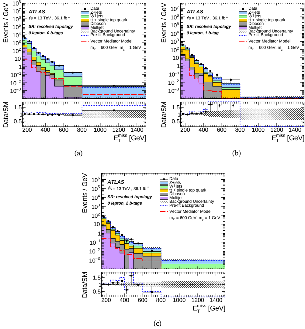
Figure 5.8.4: E_T^{\text{miss}} distributions after the combined profile likelihood fit in the resolved signal regions: (a) 0 b -tag high purity signal region, (b) 1 b -tag high purity signal region and (c) 2 b -tag high purity signal region [1].
