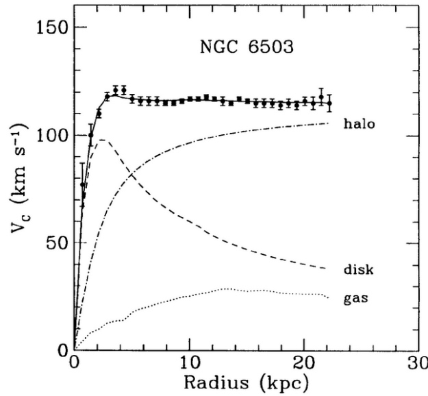
Figure 2.2.1: Rotation curve of the galaxy NGC6503 with a three-parameter dark halo fit (solid curve) to the observed data [27]. The dashed curve shows the rotation curve for visible matter. The dotted curve shows the rotation curve for gas component. The dash-dot curve shows the rotation curve for the dark halo. The parameters of the fit include the mass-to-light ratio of the disk ( M/L ), the halo core radius ( r_c ) and the halo asymptotic circular velocity ( V_h ).
