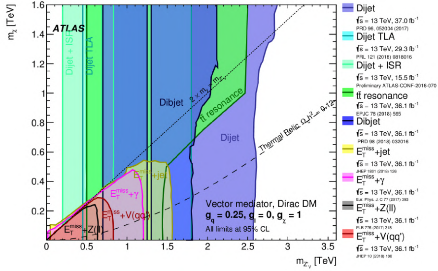
Figure 5.8.7: Exclusion in the m_\chi - m_{\text{med}} plane at 95% CL by the dijet, dileptonic t\bar{t} resonance searches and the E_T^{\text{miss}} + X searches for the vector mediator simplified model [175]. The couplings of the mediator to the SM and DM particles are fixed to g_q = 0.25 , g_l = 0 and g_\chi = 1 . The dashed line represents the mass points for which the expected DM relic density is consistent with the WMAP [173] and Planck [29] measurements ( \Omega_{\text{DM}} h^2 = 0.1186 \pm 0.0020 ), computed with MadDM [174]. The region on the right of the curve corresponds to higher predicted relic abundance.
