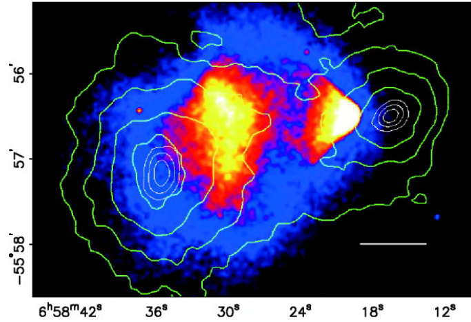
Figure 2.2.2: Illustration of bullet cluster 1E 0657-558 measured by the Chandra X-ray Observatory [28]. The green contours mark the different levels of reconstructed cluster surface mass density \kappa based on weak gravitational lensing effect. The white contours show the errors on the positions of the \kappa peaks and correspond to 68.3%, 95.5%, and 99.7% confidence levels. The colored area indicates the mass density of X-ray plasma clouds from the two colliding clusters. Significant deviations between the \kappa peaks and the mass peaks of plasma clouds can be observed.
