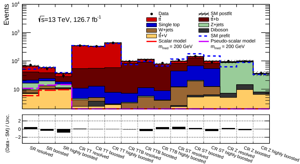
Figure 6.8.2: Event yield in all signal regions and control regions after the combined profile likelihood fit. The stacked histograms show the SM prediction and the hatched uncertainty band around the SM prediction corresponds to the total MC uncertainty, which consists of the MC statistical uncertainty, experimental systematic uncertainties and theoretical systematic uncertainties. The dotted blue line denotes the MC prediction before the combined fit. The dashed lines represent the expected contribution of the scalar mediator simplified model with m_{\text{med}} = 200 GeV (violet) and the pseudo-scalar mediator simplified model with m_{\text{med}} = 200 GeV (red) assuming g = 1 . The lower band shows the deviation between observation and prediction with respect to the total uncertainty, which consists of the total MC uncertainty and the data statistical uncertainty.
