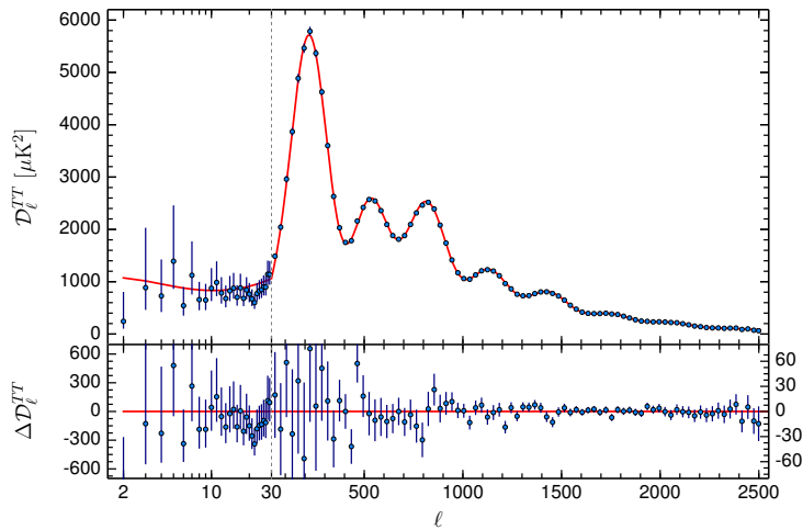
Figure 2.2.5: Planck 2015 CMB spectrum with the base \Lambda CDM fit to data (red line) [30]. D_l^{TT} = l(l+1)C_l^{TT}/(2\pi) is shown for better visualization. The horizontal scale changes from logarithmic to linear at the ‘hybridization’ scale, l = 29 .
