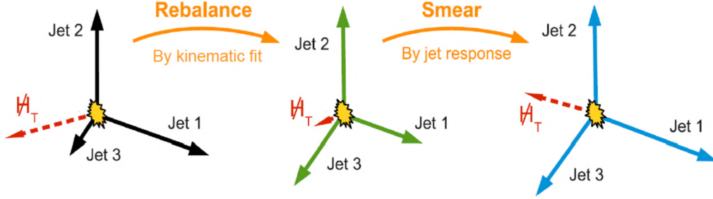
Figure 6.6.12: Schematic illustration of the ‘Rebalance and Smear’ method used to provide the multijet background estimation.
