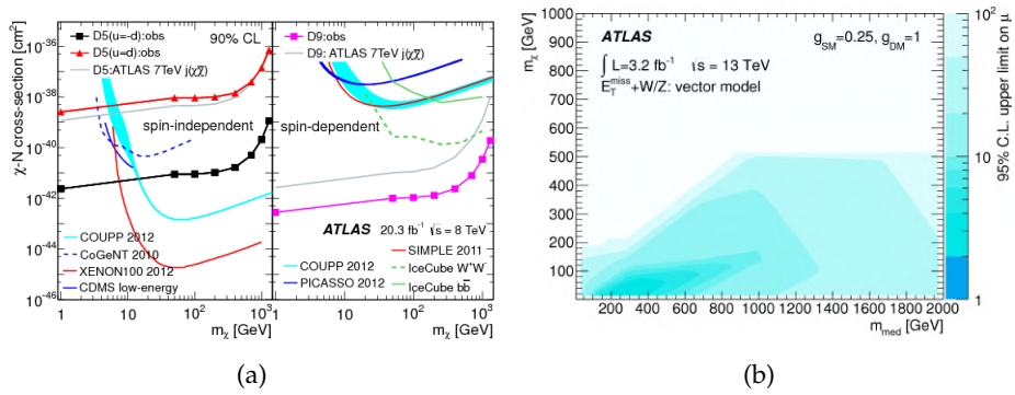
Figure 5.0.1: (a) Observed limit on the DM-nucleon scattering cross section of the spin-independent effective field theory as a function of the DM mass m_\chi [145], obtained using 20.3 \text{ fb}^{-1} of pp collision data at \sqrt{s} = 8 TeV. (b) Observed limit on the signal strength, \mu , for the vector mediator simplified model in the plane of the DM particle mass, m_\chi , and the mediator mass, m_{\text{med}} [146], obtained using 3.2 \text{ fb}^{-1} of pp collision data at \sqrt{s} = 13 TeV.
