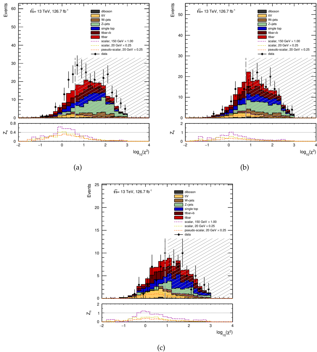
Figure 6.5.2: \log_{10}(\chi^2_{t\bar{t}, \text{had}}) distributions in (a) the resolved regime, (b) the boosted regime and (c) the highly boosted regime with all SR selections applied except for the \chi^2_{t\bar{t}, \text{had}} cut. The vertical dashed lines represent the selection value of \chi^2_{t\bar{t}, \text{had}} while the hatching lines indicate the direction of the cut. The distributions are shown before the profiling.
