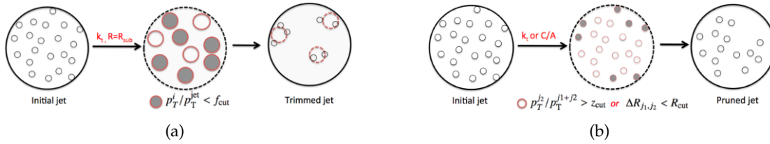
Figure 3.3.15: Illustration of two jet grooming algorithms [127]. (a) Diagram depicting the trimming procedure, the standard ATLAS jet grooming algorithm for large- R jet which removes reclustered subjets with p_T below a certain threshold. (b) Diagram depicting the pruning procedure, an alternative method to build groomed large- R jets by introducing additional requirements on \Delta R_{ij} , p_{Ti} and p_{Tj} during the jet clustering process in order to veto wide-angle and soft pseudojets.
