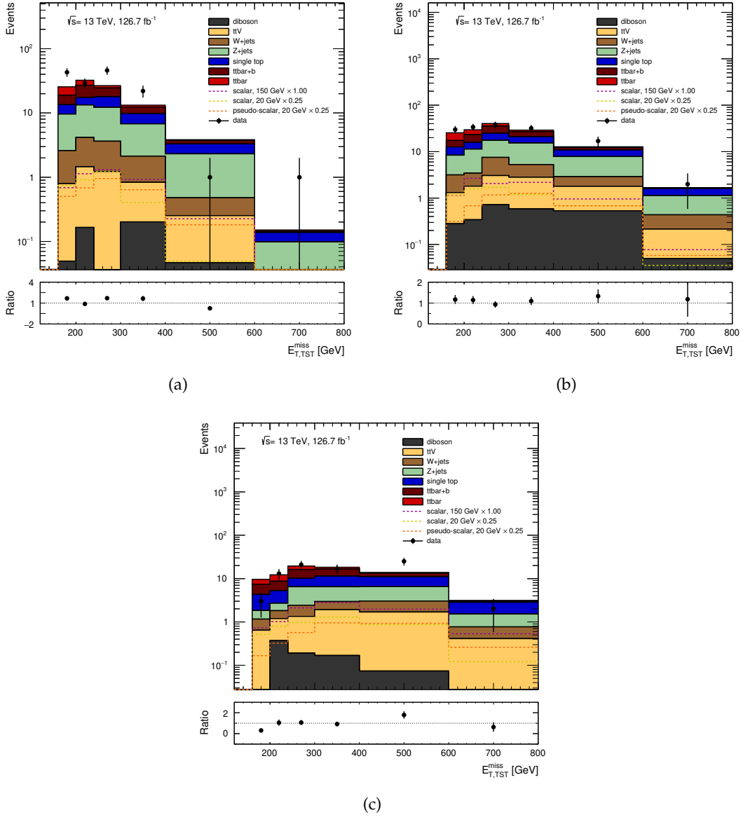
Figure 6.6.11: E_T^{\text{miss}} distributions in the (a) resolved, (b) boosted and (c) highly boosted t\bar{t} suppressed validation regions. The distributions are shown before the profiling.
