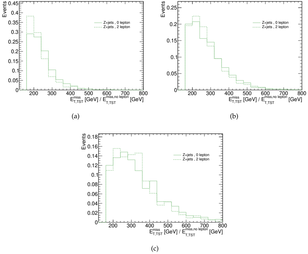
Figure 6.6.9: Shape of E_T^{\text{miss}} in 0 lepton final state (solid lines) and E_T^{\text{miss, no lepton}} in 2 lepton final state (dashed lines), normalized to unit area, for Z+jets process after the baseline selection, the anti-QCD requirements and the leptonic top reconstruction cut (only in SRs) applied in (a) the resolved regime, (b) the boosted regime and (c) the highly boosted regime.
