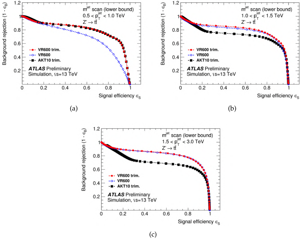
Figure 4.1.2: Background rejection versus signal efficiency evaluated with simulated Z' signal and dijet background [141]. The performances are shown for trimmed VR jets (red full circles), ungroomed VR jets (blue empty circles) and trimmed large- R jets (black squares) in events with (a) 0.5 \text{ TeV} < p_T^{\text{jet}} < 1.0 \text{ TeV} , (b) 1.0 \text{ TeV} < p_T^{\text{jet}} < 1.5 \text{ TeV} and (c) 1.5 \text{ TeV} < p_T^{\text{jet}} < 3.0 \text{ TeV} . The curves are obtained by varying the value of a hypothetical lower bound on the jet mass.
