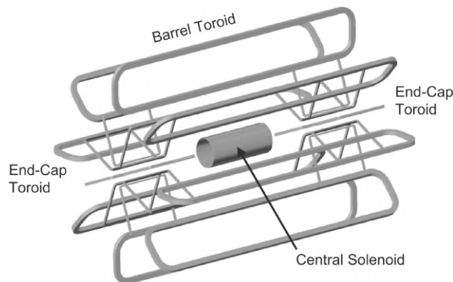
Figure 3.2.3: An illustration of the layout of the ATLAS magnet system [89].
