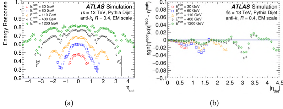
Figure 3.3.9: (a) Average energy response and (b) signed difference between reconstructed and truth \eta as functions of \eta_{\text{det}} for small- R jets with p_T^{\text{truth}} = 30, 60, 110, 400, 1200 GeV before the MC-based calibration [112].
