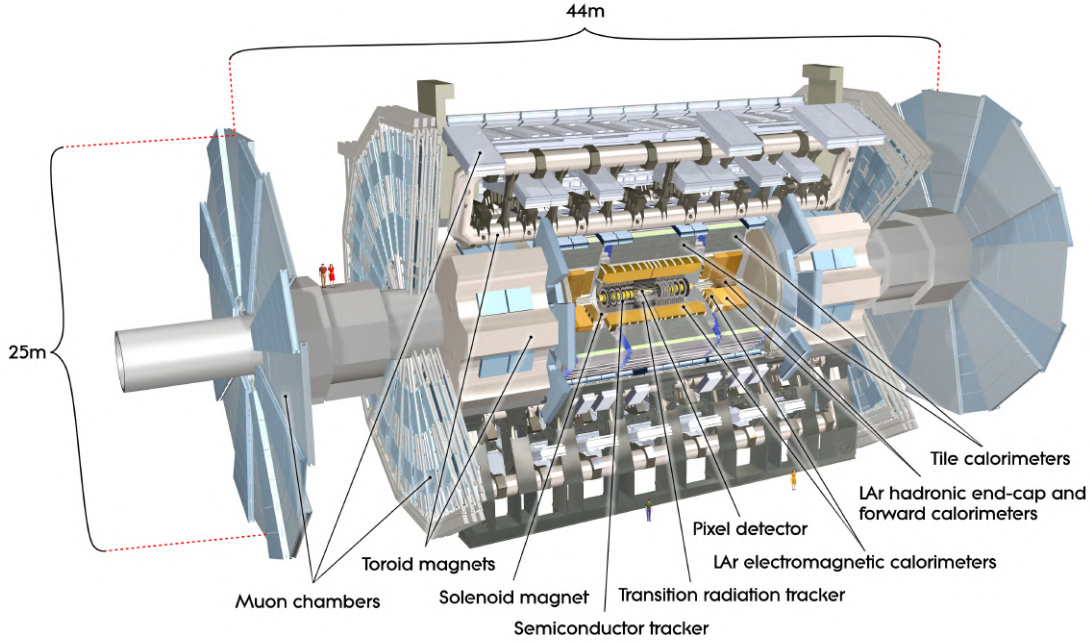
Figure 3.2.1: An illustration of the whole ATLAS detector [87] which consists of four major components, namely the Inner Detector (tracking system), the Calorimeter (calorimeter system), the Muon Spectrometer (muon system) and the magnet system.
