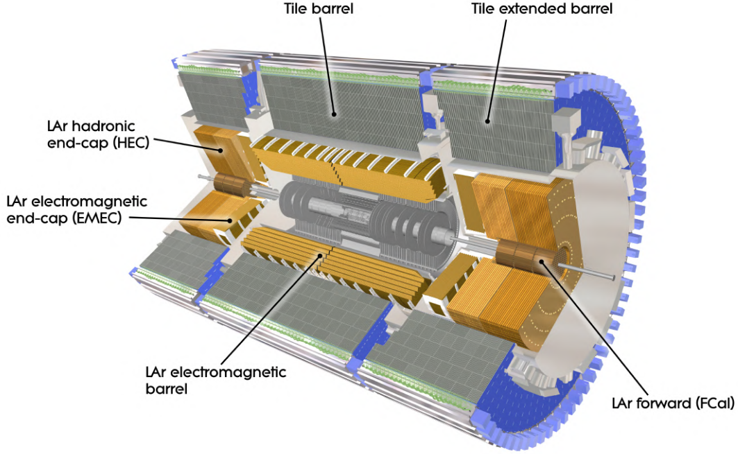
Figure 3.2.5: The general layout of the ATLAS calorimeter system [93].
