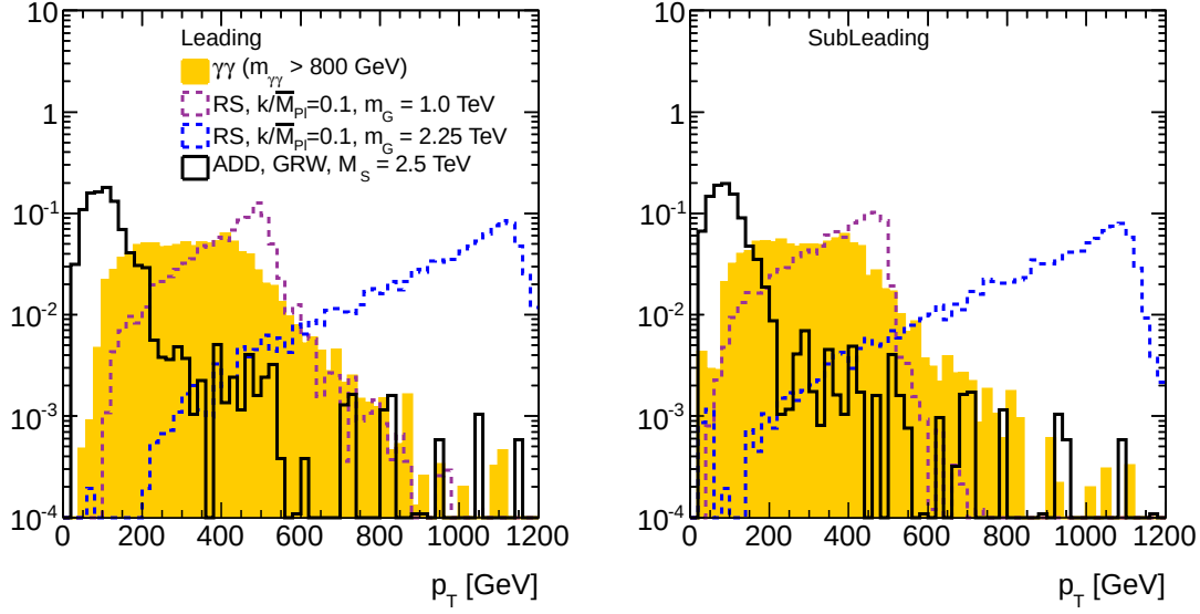
(a) p_T
