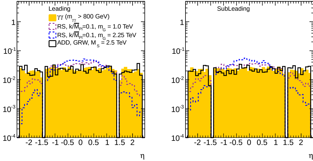
(b) \eta
