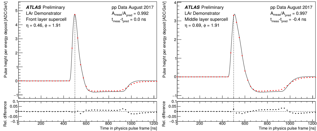
Figure 5.16.: Normalised and averaged pulse shapes for two super cells in (left) front and (right) middle layer. The measured samples of the pulses in proton-proton collision data from August 2017 are shown in red. The predicted pulses in black are estimated using the response transformation method on the OF coefficients. The estimates of A_{\text{meas}} and t_{\text{meas}} use five samples around the peak sample (dashed line) [10].
