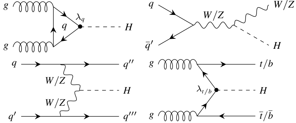
Figure 1.3.: Leading order Feynman diagrams for Higgs boson production in (top left) gluon-gluon fusion, (top right) associated production with a vector boson, (bottom left) vector boson fusion and (bottom right) associated production with pair of top- or bottom-quarks. The quark Yukawa coupling, entering in the gluon-gluon fusion is marked with \lambda_q . The t\bar{t}H ( b\bar{b}H ) production gives direct access to the top (bottom) Yukawa coupling \lambda_{t(b)} .
