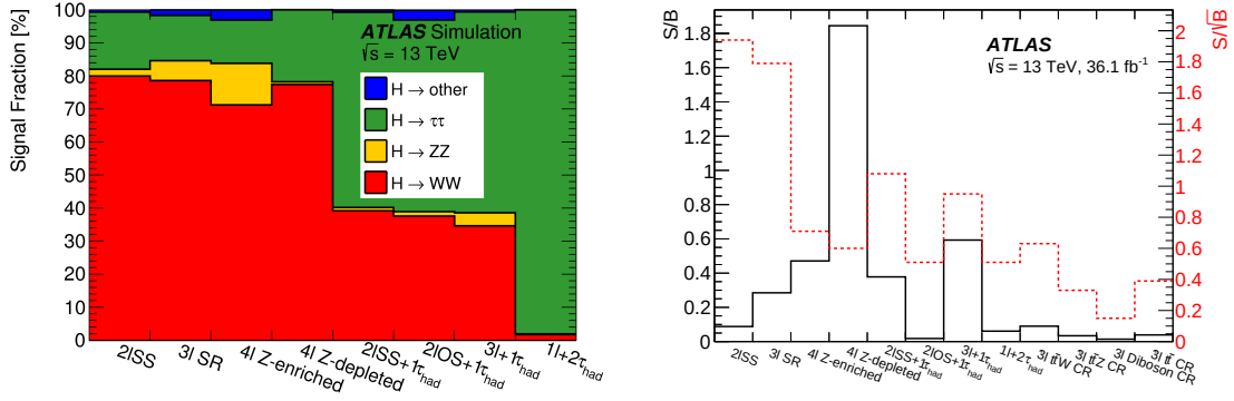
Figure 3.19.: (Left) Fraction of Higgs boson decays in the t\bar{t}H signal in the signal regions and (right) S/B and S/\sqrt{B} for all signal and control regions with signal S and total background B . All values are estimated from SM pre-fit expectation [4].
