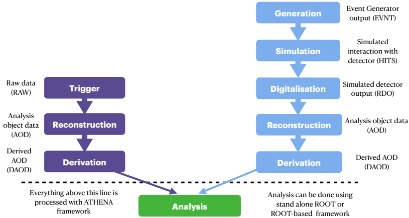
FIGURE 4.4: Schematic of the simulation and reconstruction procedure for data and MC events in ATLAS experiment by ATHENA framework.
