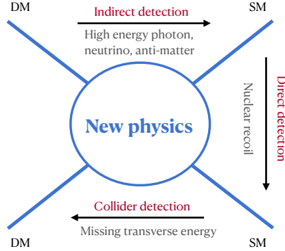
FIGURE 2.3: Schematic diagram to show the relation among the direct detection, indirect detection and collider detection of DM. The arrows indicate the direction of reaction.
