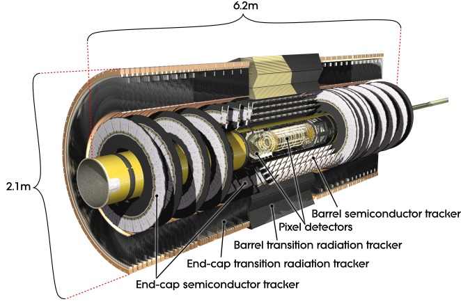
FIGURE 3.7: The ATLAS Inner Detector [186].
