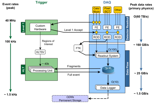
FIGURE 3.10: The ATLAS DAQ System in LHC Run 2. Events passing the L1 hardware trigger (top left) are passed to the HLT (bottom left) via the farm supervisor node (HLT SV), now including assembly of Regions of Interest. Simultaneously to this, event data from the detector front-end electronics systems are sent to the ROS via optical links from the Readout Drivers (RODs) in response to a L1 trigger accept signal. These data are then buffered in the ROS and made available for sampling by algorithms running in the HLT. Once the HLT accepts an event it is sent to permanent storage via the Data Logger [195].
