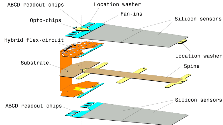
Figure 30: An expanded view of the geometry of the SCT double layers in the barrel region [19].
