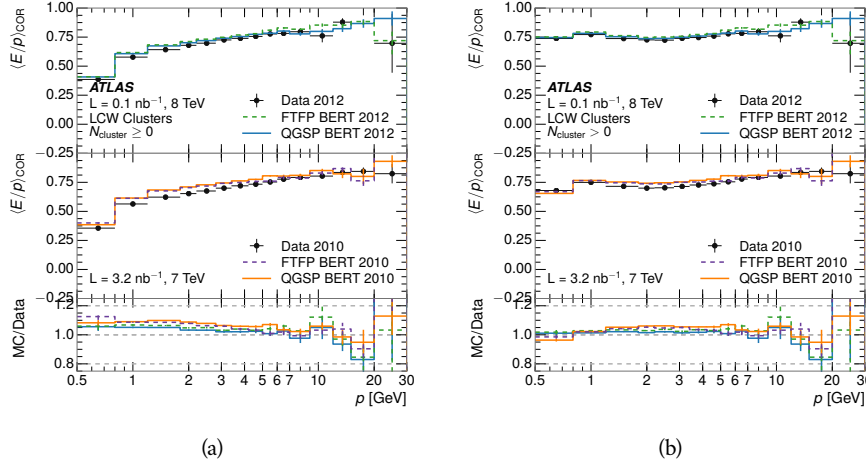
Figure 55: \langle E/p \rangle_{\text{COR}} calculated using LCW-calibrated topological clusters as a function of track momentum for tracks with (a) zero or more associated topological clusters or (b) one or more associated topological clusters.
