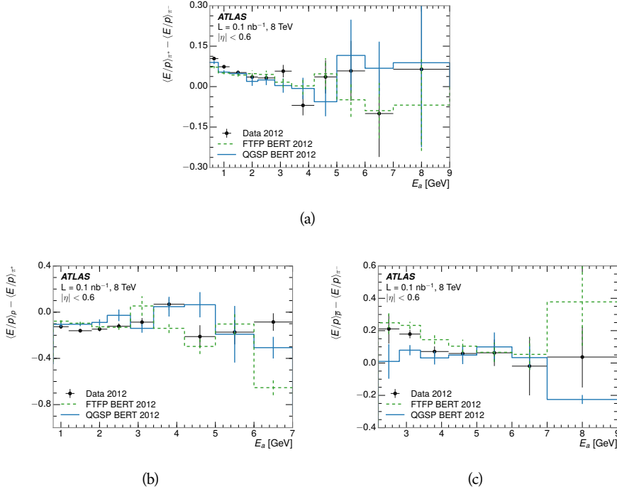
Figure 64: The difference in \langle E/p \rangle between (a) \pi^+ and \pi^- (b) p and \pi^+ , and (c) \bar{p} and \pi^- .
