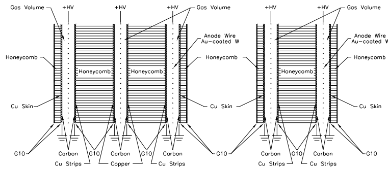
Figure 41: A schematic of the TGC doublet and triplet layers [19].
