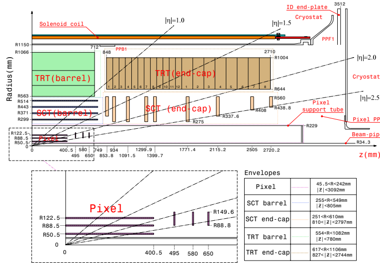
Figure 23: A quarter section of the ATLAS inner detector which shows the layout of each of the subdetectors in detail. The lower panel shows an enlarged view of the pixel detector. Example trajectories for a particle with \eta = 1.0, 1.5, 2.0, 2.5 are shown. The IBL, which was added after the original detector commissioning, is not shown [19].
