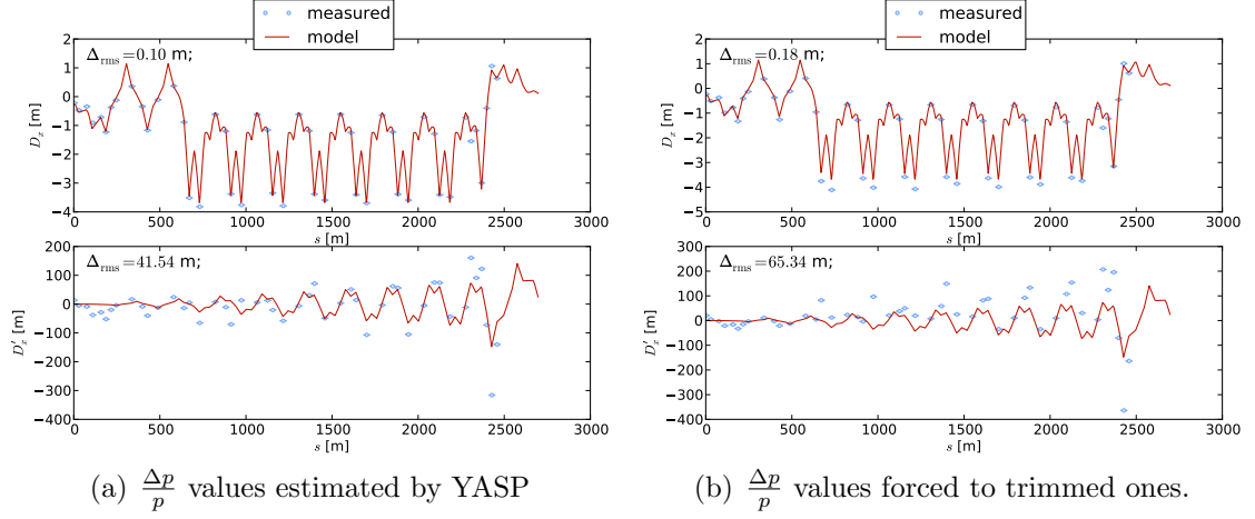
Figure 8.24.: Horizontal dispersion in TI8 calculated from linear fits to position data.
