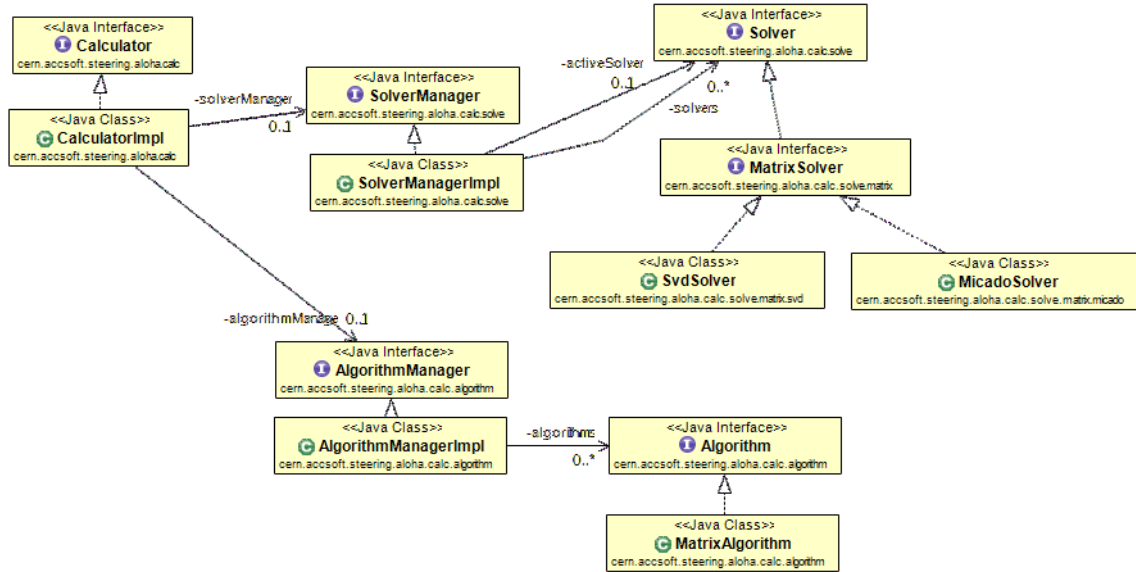
Figure 7.2.: Class diagram of classes involved in the fitting procedure in Aloha.
