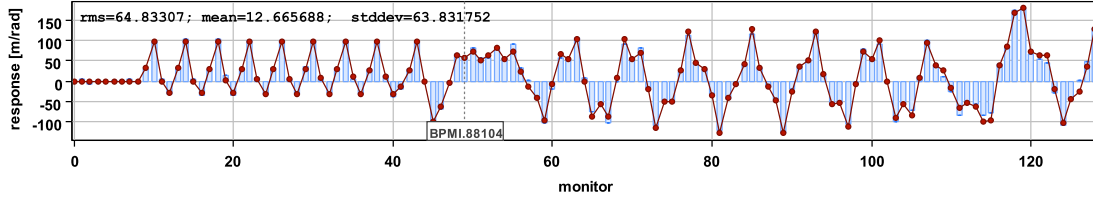
(a) Horizontal response for horizontal corrector MCI AH.80804.
