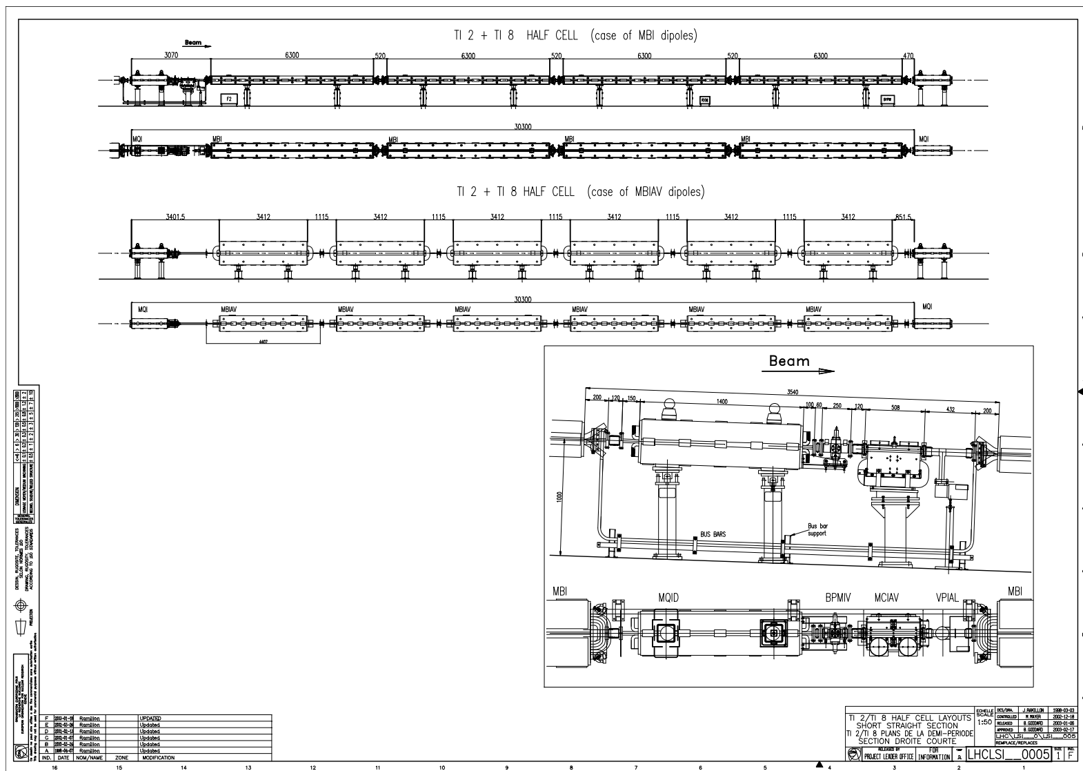
Figure A.1.: Half-cell layout of TI8 and TI2.
