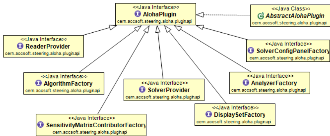
Figure 7.9.: Class diagram of Aloha plugin API.
