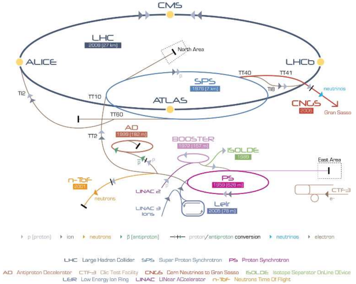
Figure 2.2.: The CERN accelerator complex.
