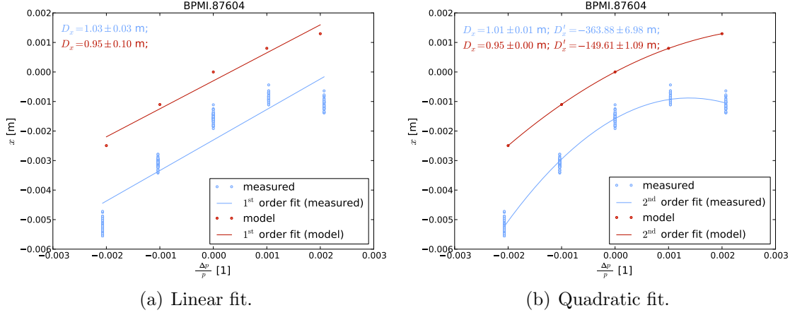
Figure 8.22.: Model and measured positions for an example BPM (BPMI.87604) in the TI8 transfer line with \frac{\Delta p}{p} values forced to trimmed ones.
