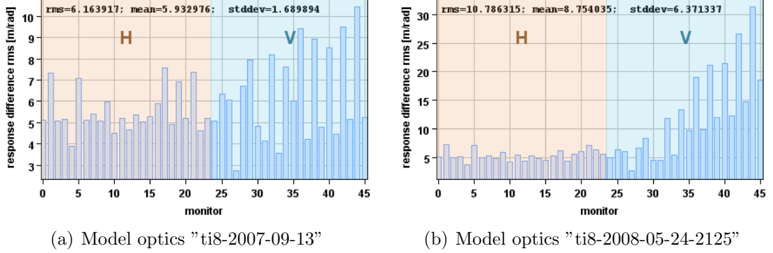
Figure 8.5.: RMS differences per monitor between measurement and model; Same measurement, different model settings. Note the different vertical scales: The maximum difference for optics "ti8-2007-09-13" is about \frac{1}{3} of the maximum for optics "ti8-2008-05-24-2125".
