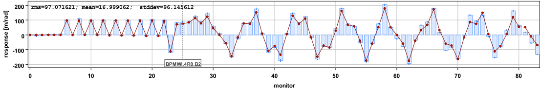
(a) Horizontal response for horizontal corrector.
