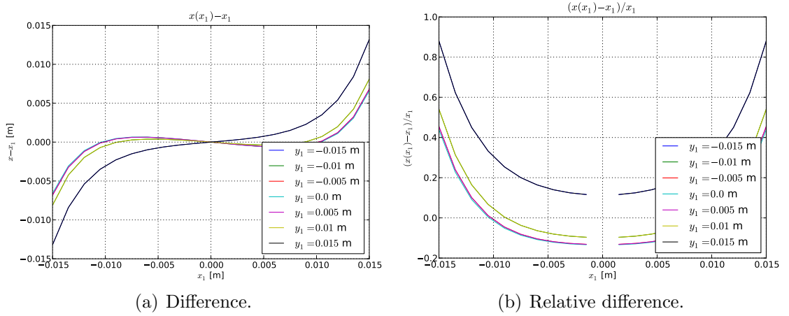
Figure 8.27.: Differences between corrected and uncorrected positions.
