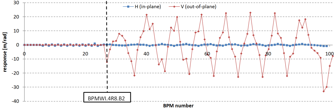
Figure 4.4.: Difference between analytically and numerically calculated response. The marker 'BPMWI.4R8.B2' indicates the first BPM in the LHC.
