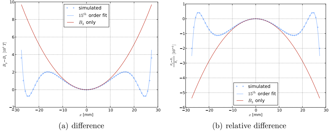
Figure 8.37.: Differences between simulated and nominal vertical field in TI8 MBIs.
