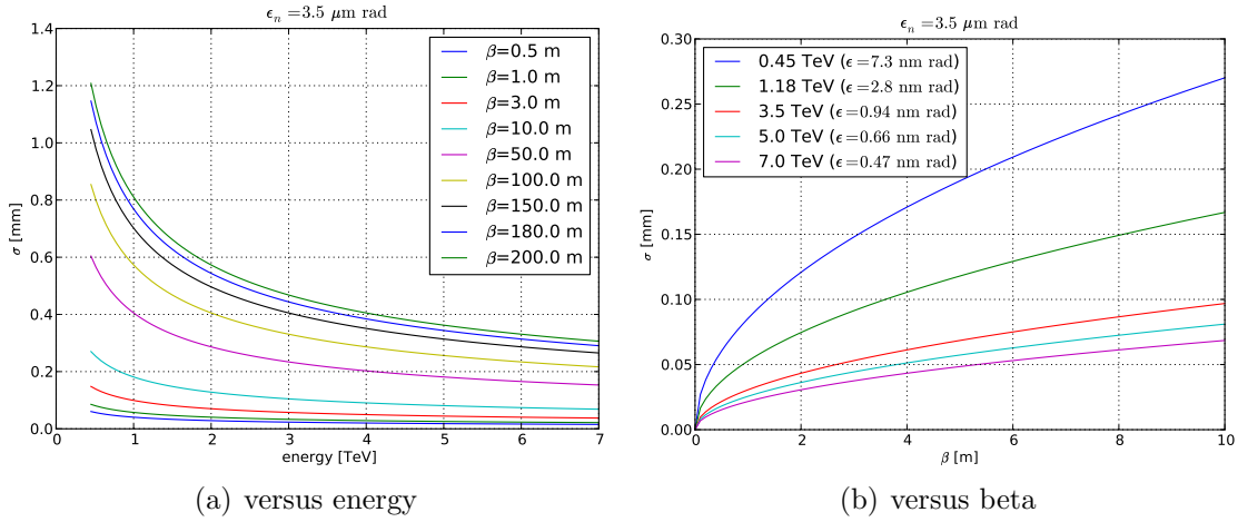
Figure 3.2.: LHC Beam size dependence on beam energy and beta-value.
