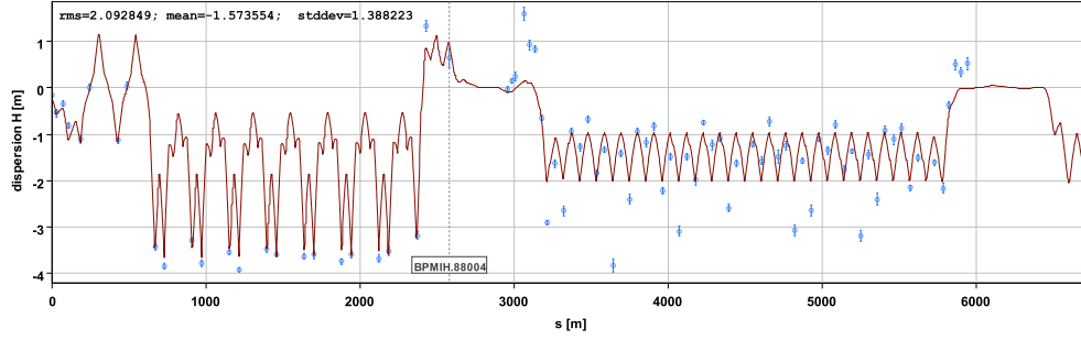
(a) Measured dispersion compared with calculated.
