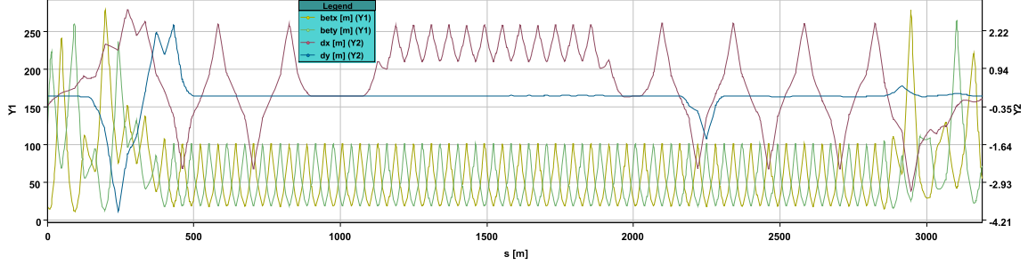
Figure 5.4.: Optics functions of the TI2 transfer line.
