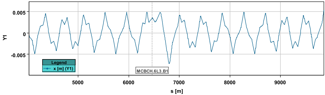
Figure 4.1.: Effect of a corrector-kick (horizontal corrector MCBCH.6L3.B1) on the orbit in a ring. The orbit without the kick would be zero at all s-positions.
