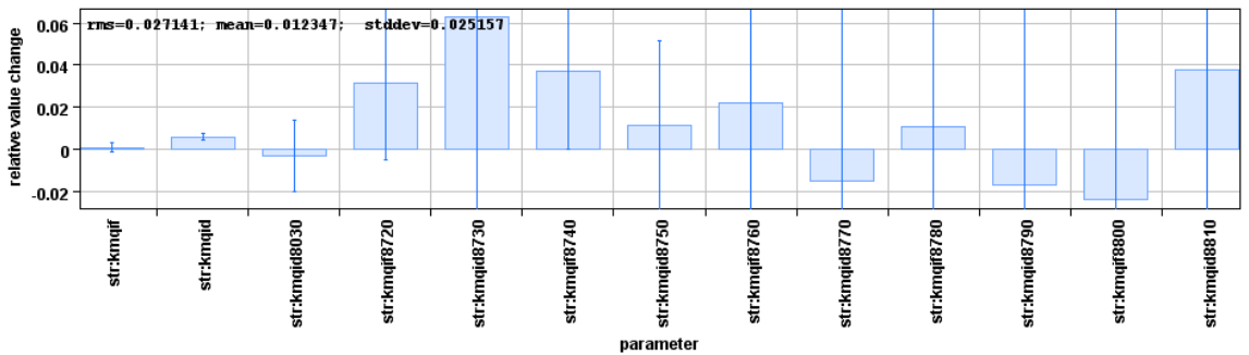
Figure 8.18.: Relative parameter changes after SVD fit using all individually powered quadrupoles in TI8 downstream of MCIAH.80204.
