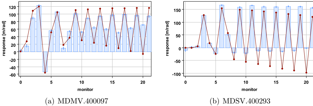
Figure 8.4.: Vertical responses for 2 correctors with reduced kqid.80500 in machine, compared with model using the same settings as in the machine ("ti8-2008-05-24-2125").
