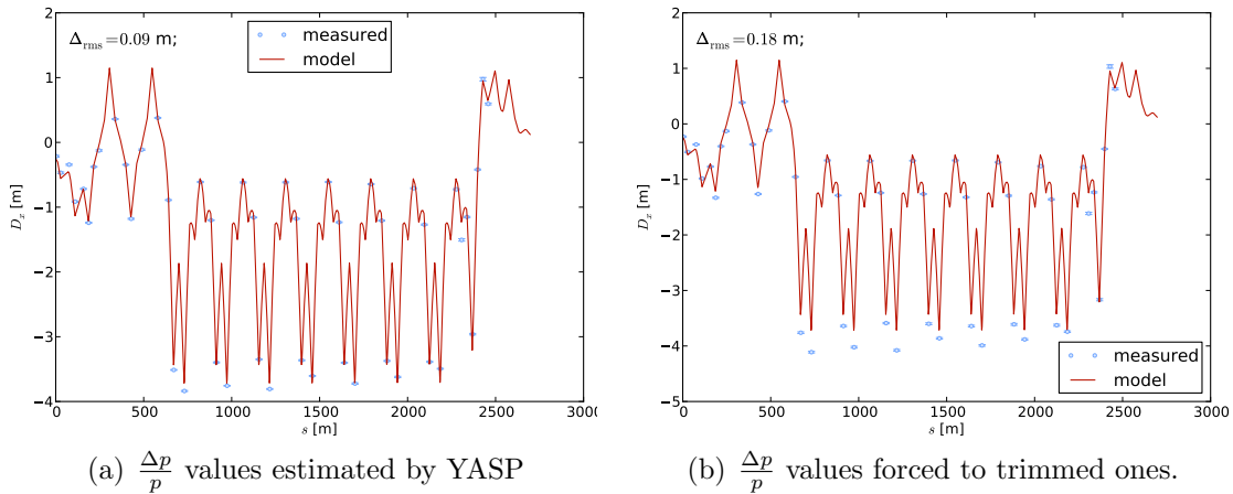
Figure 8.23.: Horizontal dispersion in TI8 calculated from linear fits to position data.
