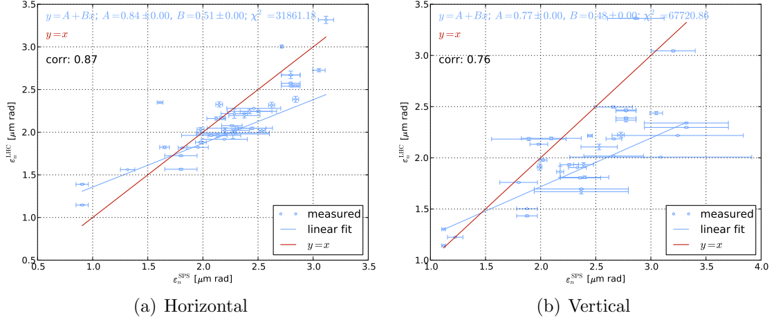
Figure 8.45.: Emittance transfer from SPS to LHC beam 1.
