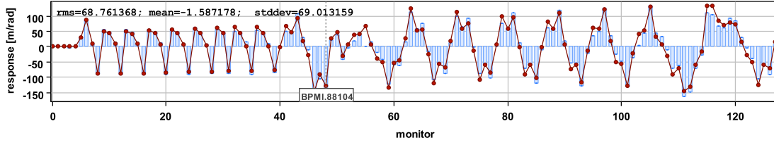
(b) Vertical response for vertical corrector MCI AV.80104.
