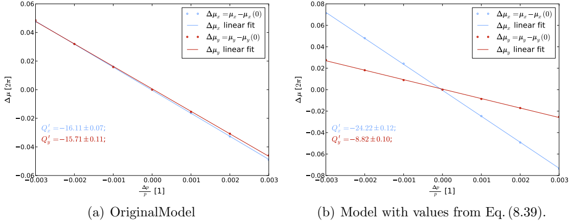
Figure 8.35.: Comparison of natural chromaticity for TI2 (Note: The scales of the vertical axes are different in the two plots.).
