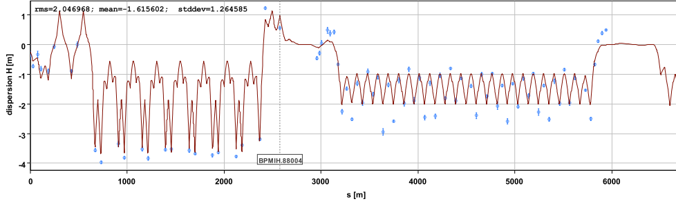
(a) Measured dispersion compared with calculated.
