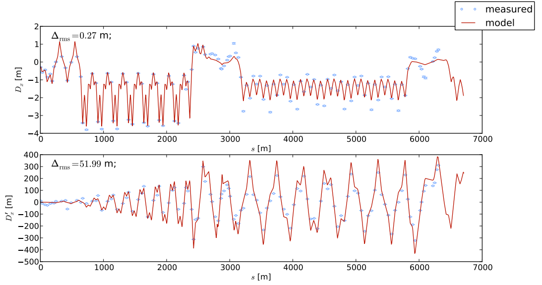
Figure 8.43.: Original horizontal dispersion in TI8 and LHC sector 78.
