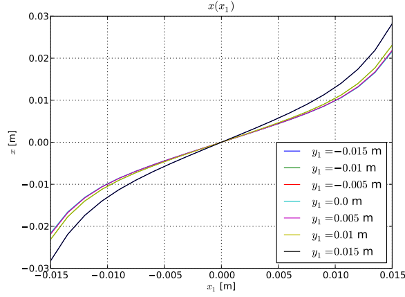
Figure 8.26.: Dependence of real beam position x on uncorrected position x_1 .
