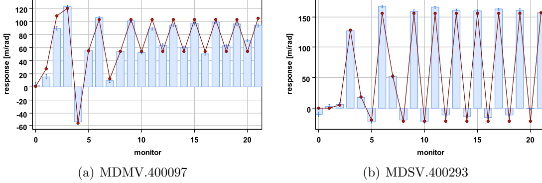
Figure 8.3.: Vertical responses for 2 correctors with reduced kqid.80500 in machine, compared with model using original 2007 optics ("ti8-2007-09-13").
