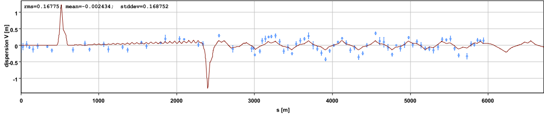
(b) Vertical dispersion.
