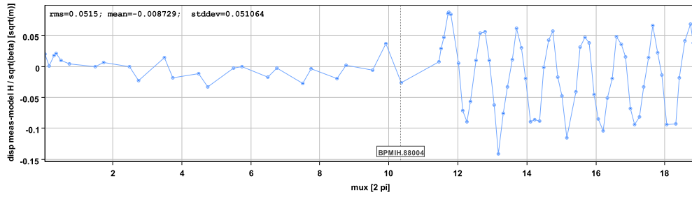
(b) Normalized dispersion difference between measurement and model.
