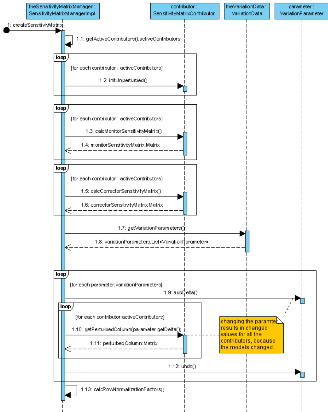
Figure 7.6.: Creation of the Sensitivity matrix.
