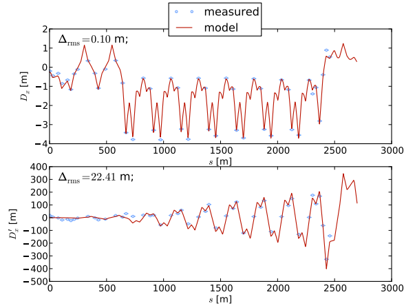
Figure 8.29.: Horizontal dispersion in TI8. BPM data calibrated, model with values from Eq. (8.22).
