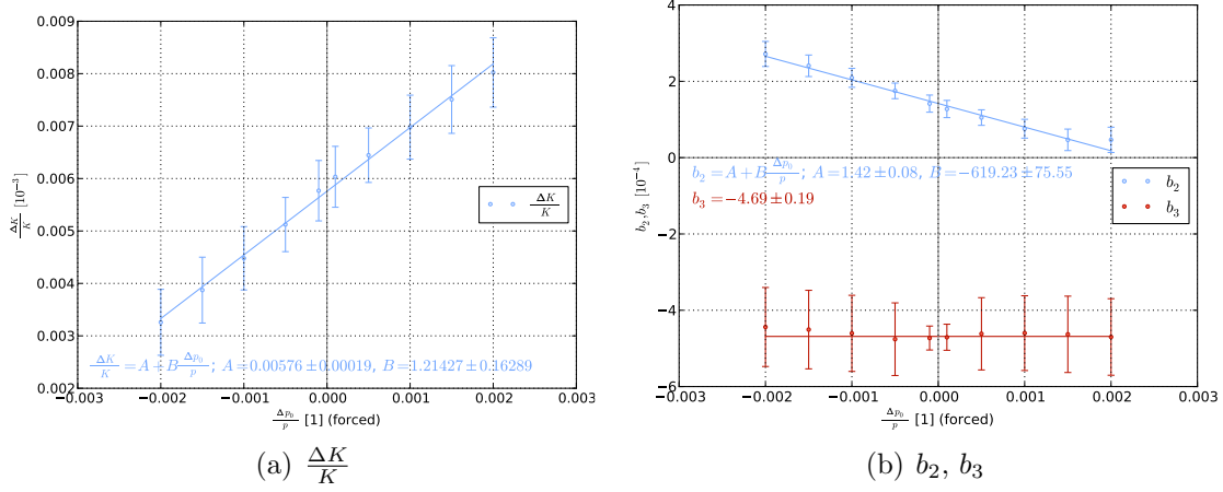
Figure 8.38.: Dependence of fit parameters on forced values of \frac{\Delta p_0}{p} for TI8.
