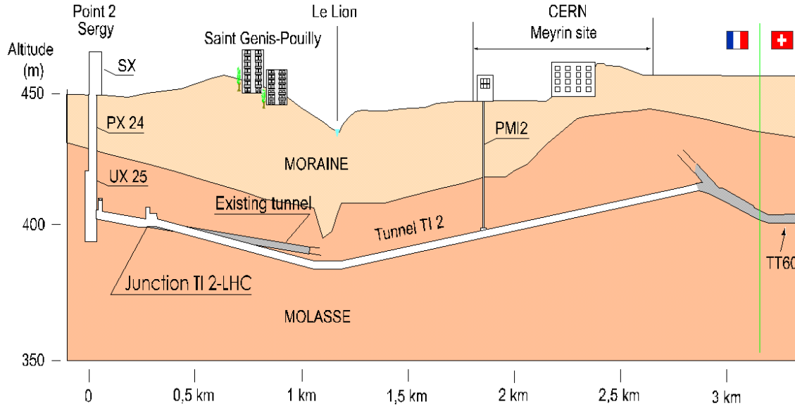
Figure 5.2.: Vertical profile of TI2 (taken from [UAC + 05]).
