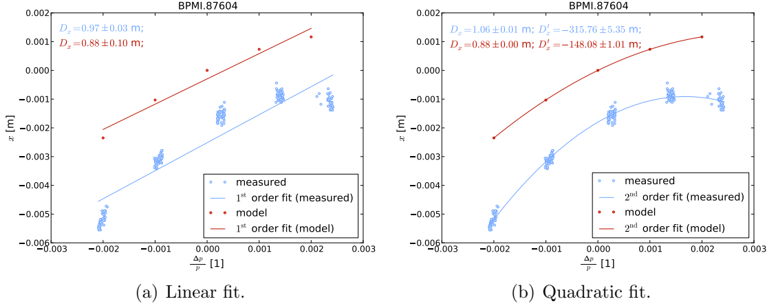
Figure 8.21.: Model and measured positions for an example BPM (BPML.87604) in the TI8 transfer line.
