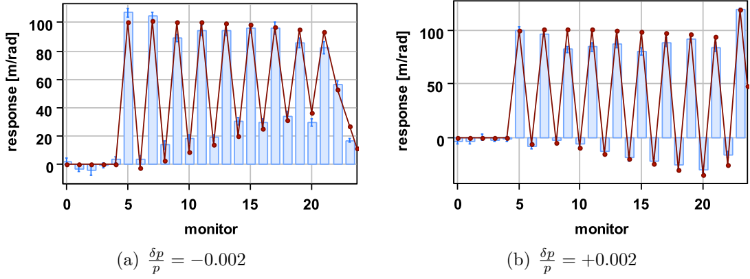
Figure 8.32.: Horizontal response for the same corrector as in Fig. 8.30 with the values of Eq. (8.22) applied to the model. Bars represent the measured data, dots the updated model.
