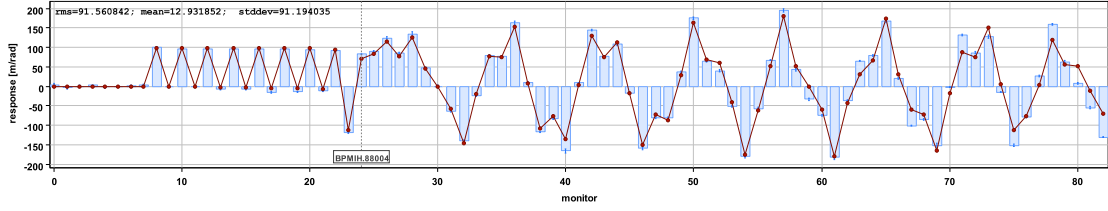
(b) Optics "ti8-2008-08-24-0327" in model (kqif.87600 reduced by 9% also in model).
