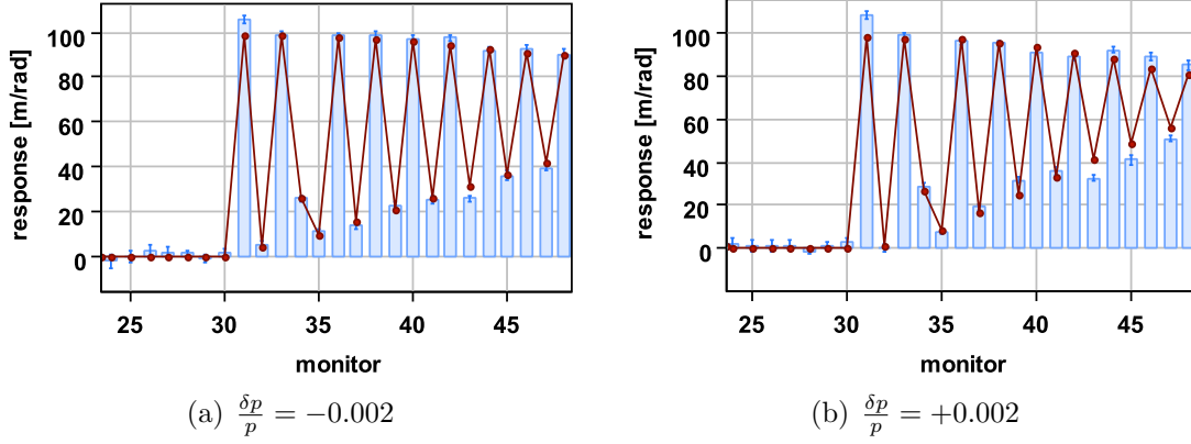
Figure 8.33.: Vertical response for the same corrector as in Fig. 8.31 with the values of Eq. (8.22) applied to the model. Bars represent the measured data, dots the updated model.
