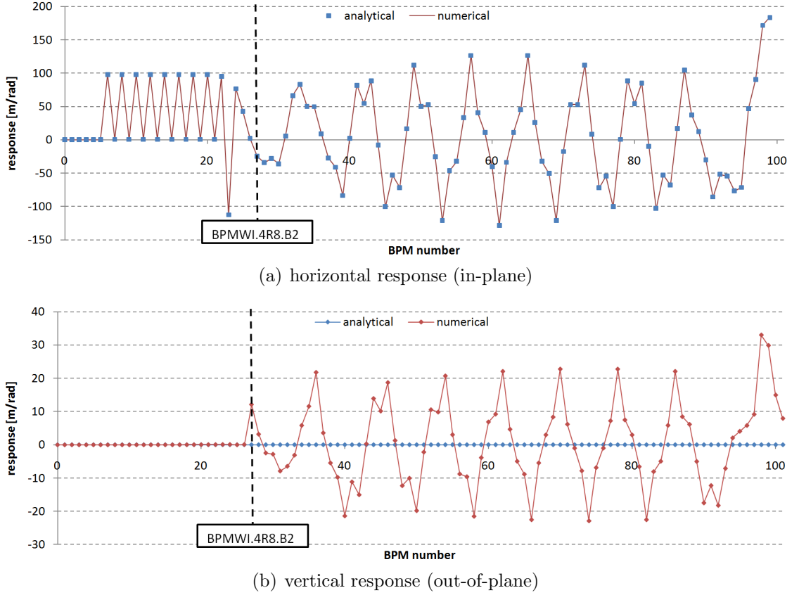
Figure 4.3.: Comparison of response for one horizontal corrector in TI8+LHC sector 78, calculated from Eq. (4.6) ('analytical') and numerically using MadX (Note the different scales of the vertical axes: The peak of the vertical response is about 20% of peak of the horizontal response). The marker 'BPMWI.4R8.B2' indicates the first BPM in the LHC.
