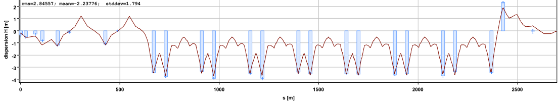
(a) Measured dispersion (blue bars) compared with model dispersion (red lines).
