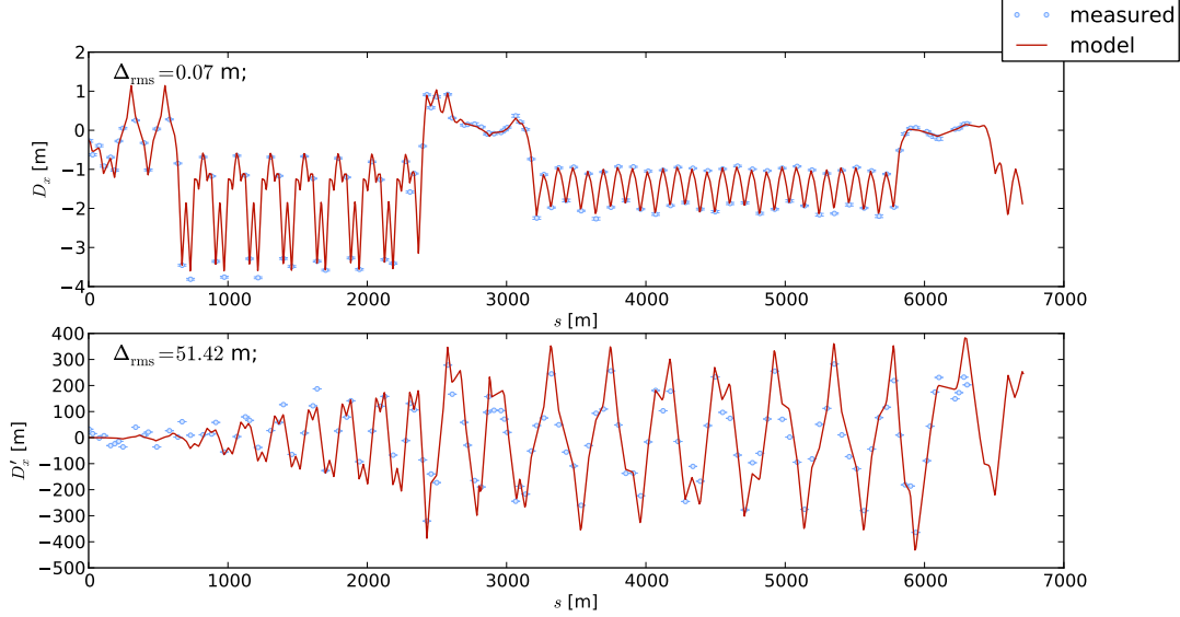
Figure 8.44.: Horizontal dispersion in TI8 and LHC sector 78 after applied correction as given in Table 8.8.
