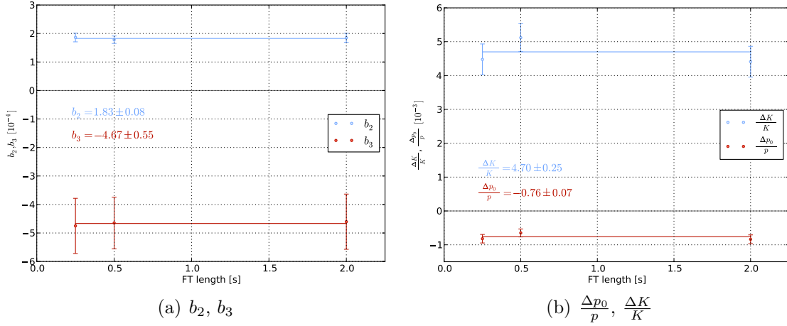
Figure 8.36.: Dependence of fit results on flat top length.
