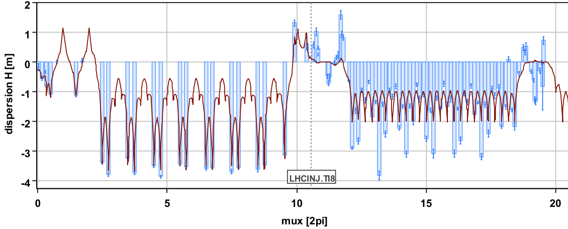
Figure 5.10.: Horizontal dispersion of TI 8 and LHC sector 78. Bars represent the measured dispersion and the line represents the dispersion calculated from the nominal model. The marker 'LHCINJ.TI8' indicates the junction between the transfer line and the LHC.
