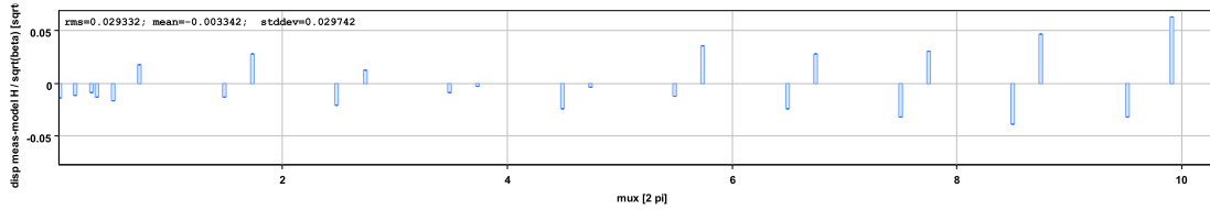
(b) Dispersion difference between measurement and model, normalized by \sqrt{\beta_x} .
