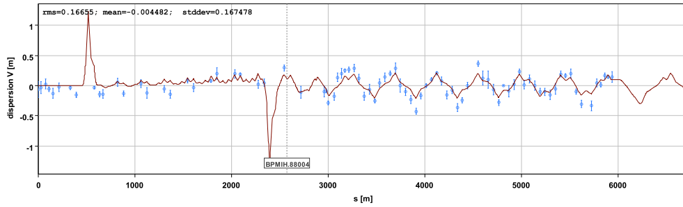
(b) Optics "ti8-2008-08-24-0327" in model (kqif.87600 reduced by 9% also in model).
