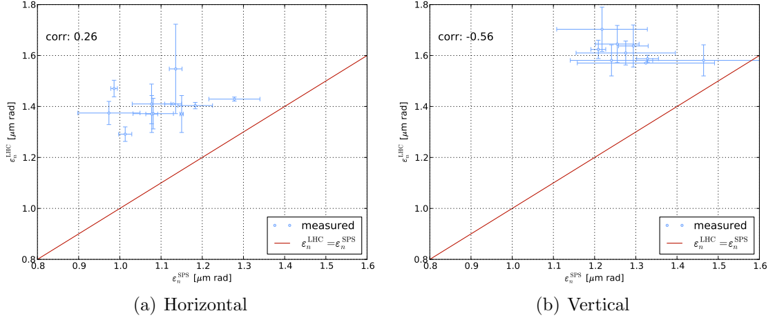
Figure 8.48.: Emittance transfer from SPS to LHC beam 2.
