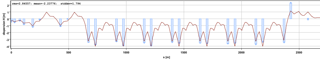
(a) Measured dispersion (blue bars) compared with model dispersion (red line).
