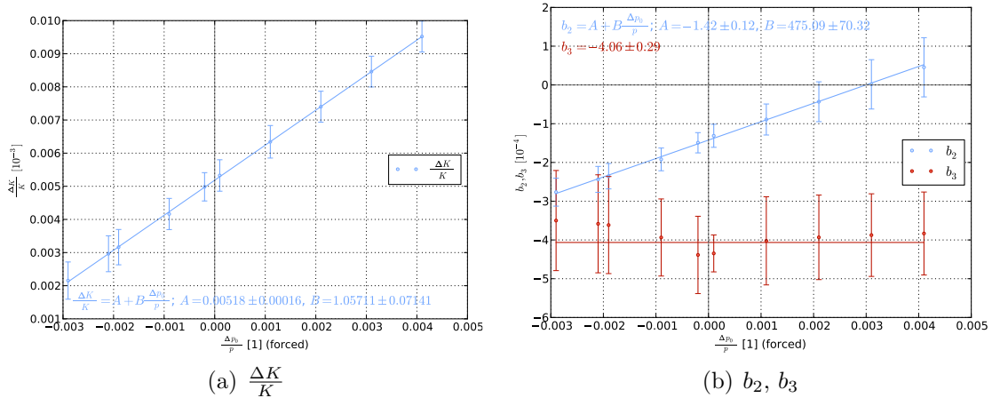
Figure 8.39.: Dependence of fit parameters on forced values of \frac{\Delta p_0}{p} for TI2.
