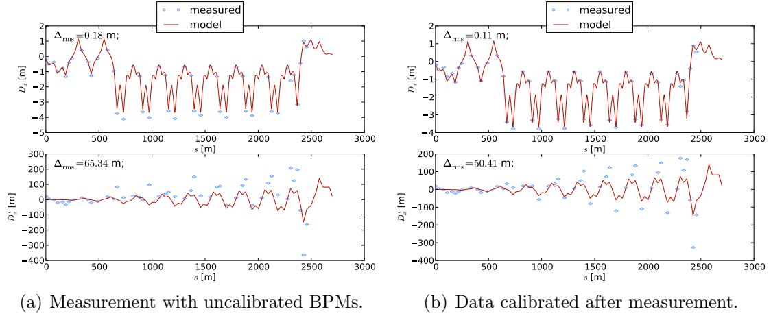
Figure 8.28.: Influence of BPM calibration on horizontal dispersion in TI8.
