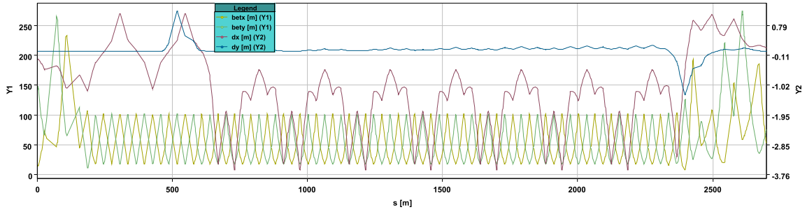
Figure 5.5.: Optics functions of the TI8 transfer line.
