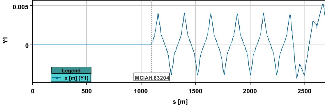
Figure 4.2.: Effect of a corrector-kick (horizontal corrector MCIAH.83204) on the trajectory in a transfer line. The trajectory without the kick would be zero at all s -positions.
