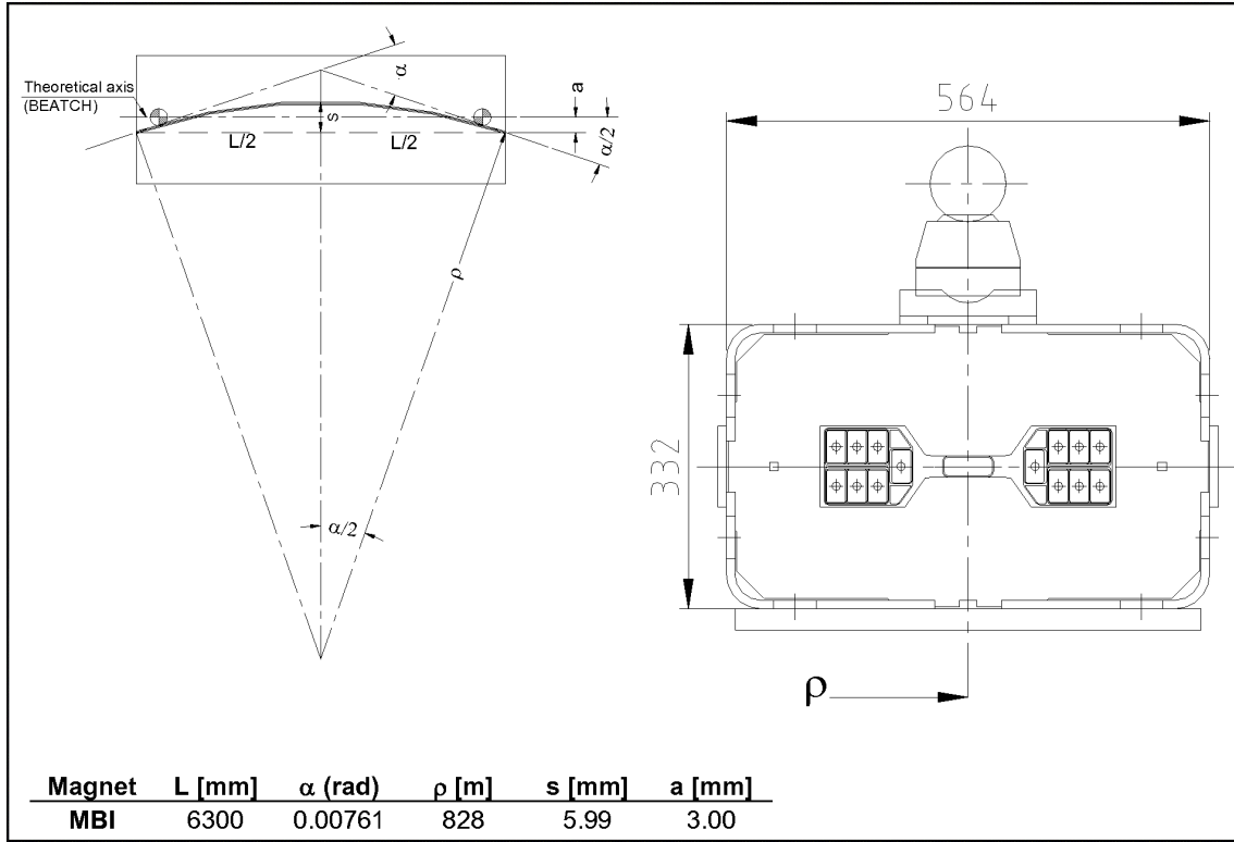
Figure 8.40.: Sketch of beam sagitta within an MBI magnet. (Taken from [WWDB03]).
