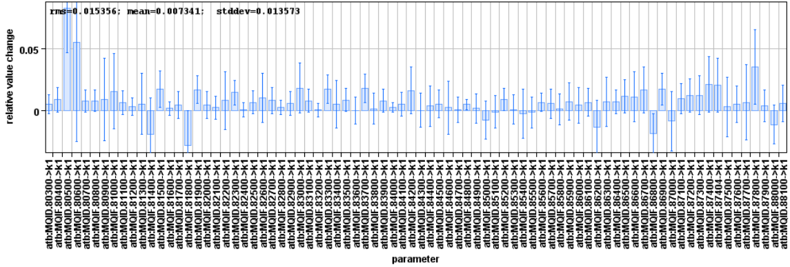
Figure 8.17.: Relative parameter changes for first fit iteration using all quadrupole strengths in TI8 as free parameters.
