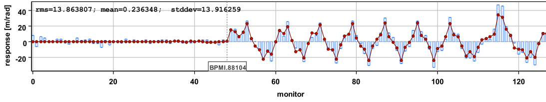
(a) Vertical response for horizontal corrector MCI AH.80804.
