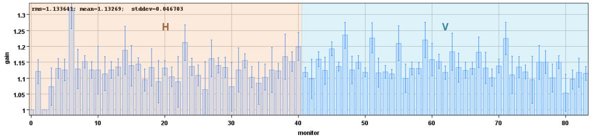
Figure 8.25.: BPM gains for TI8, resulting from a fit using BPM gains and main quadrupole strengths as free parameters.
