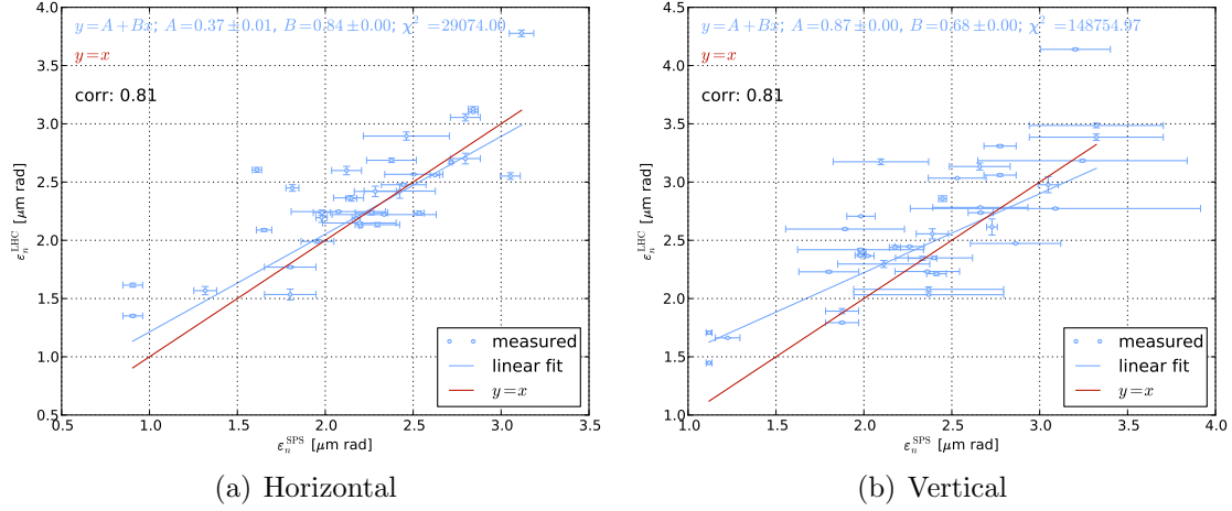
Figure 8.46.: Emittance transfer from SPS to LHC beam 2.
