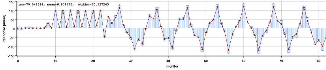
(b) Vertical orbit response of corrector MCI AV.81504.
