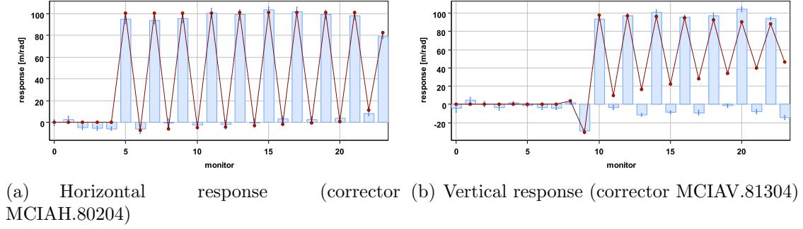
Figure 5.9.: Example responses to demonstrate phase error in vertical plane of TI8. Each blue bars represents a measured trajectory response at one BPM. Red dots represent the respective values, calculated from the nominal model.
