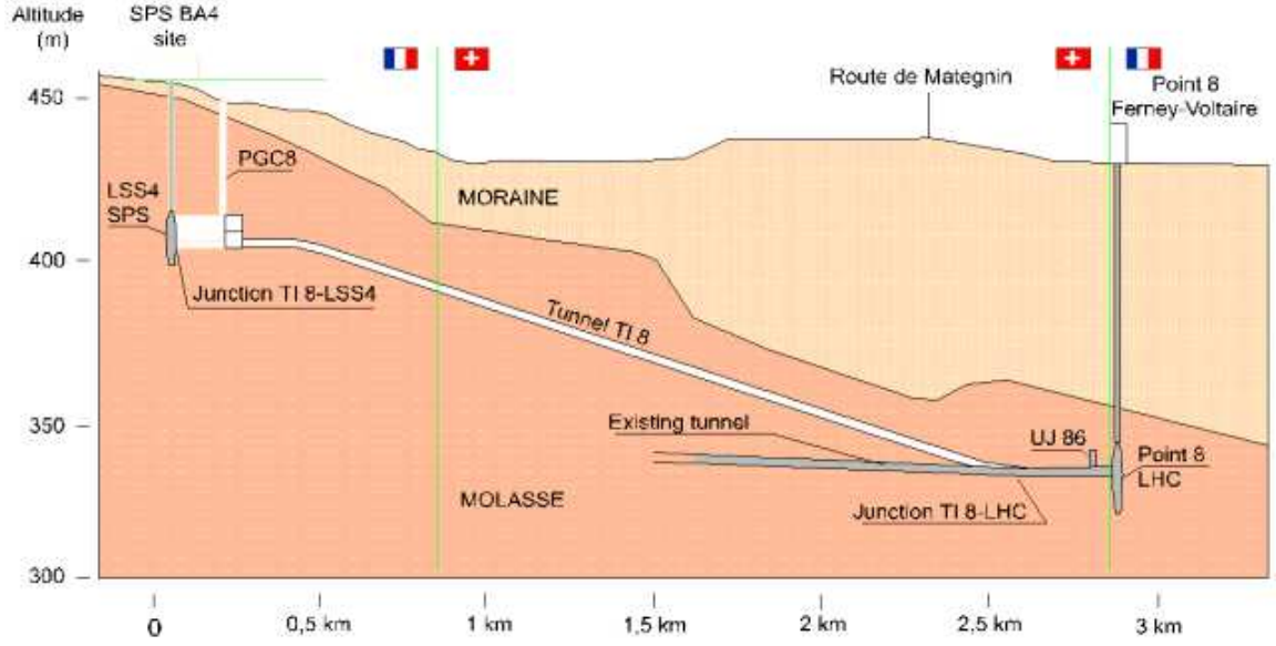
Figure 5.3.: Vertical profile of TI8 (taken from [UAA + 08]).
