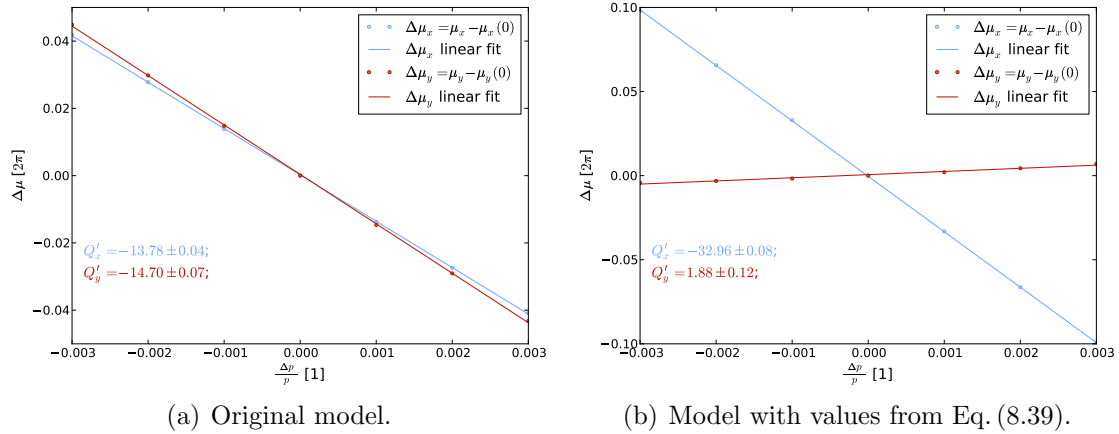
Figure 8.34.: Comparison of natural chromaticity for TI8 (Note: The scales of the vertical axes are different in the two plots.).
