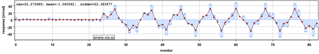
(b) Vertical response for horizontal corrector.
