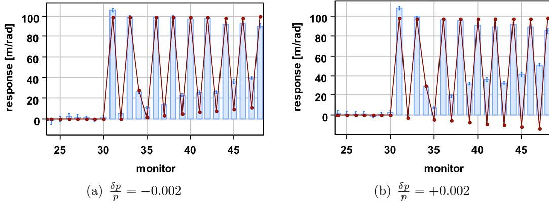
Figure 8.31.: Vertical response for one vertical corrector. Bars represent the measured data, dots the nominal model. Almost no difference in the measured data is visible, while there should be a dependence on \frac{\delta p}{p} according to the model.
