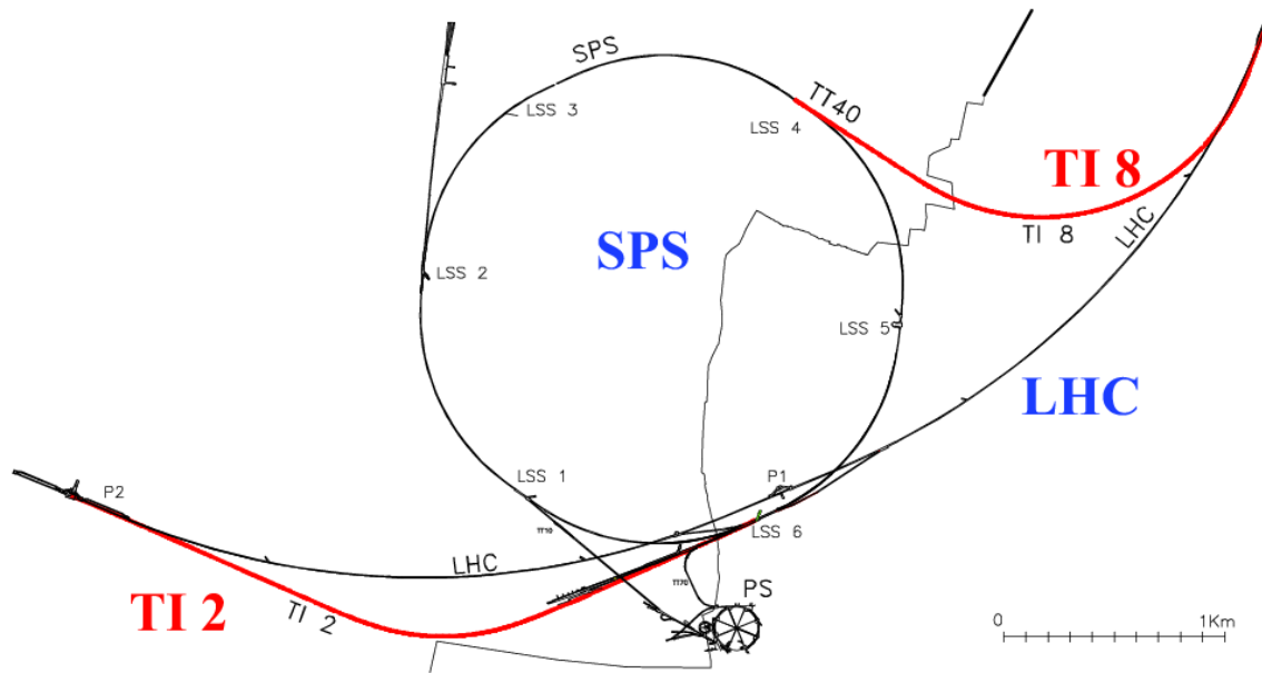
Figure 5.1.: Overall layout of the SPS to LHC transfer lines TI2 and TI8 (taken from [UAC + 05]).
