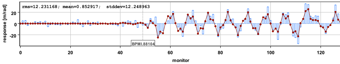
(b) Horizontal response for vertical corrector MCI AV.80104.
