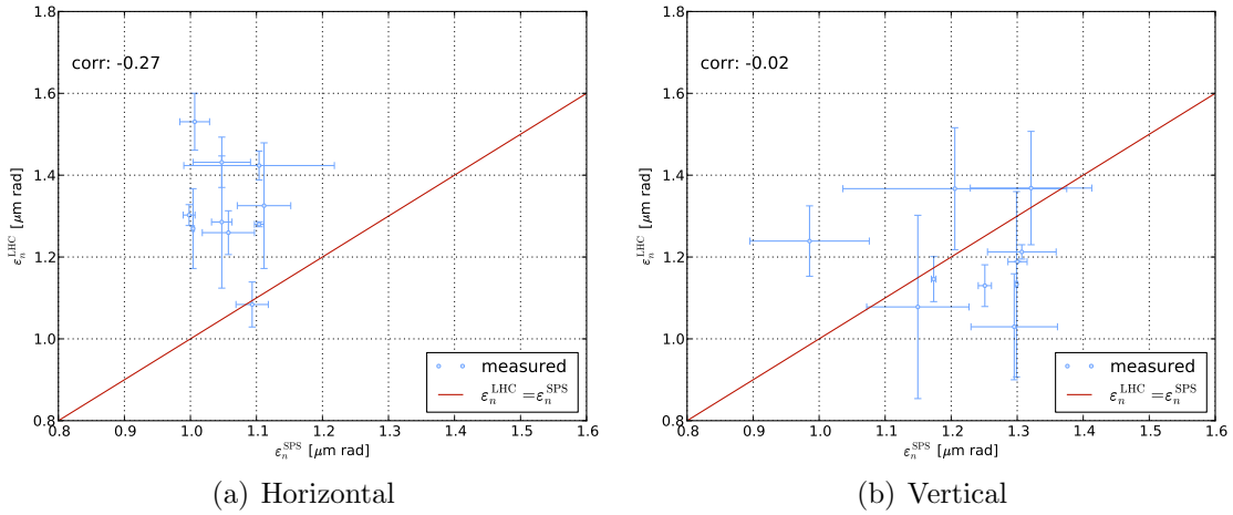
Figure 8.47.: Emittance transfer from SPS to LHC beam 1.
