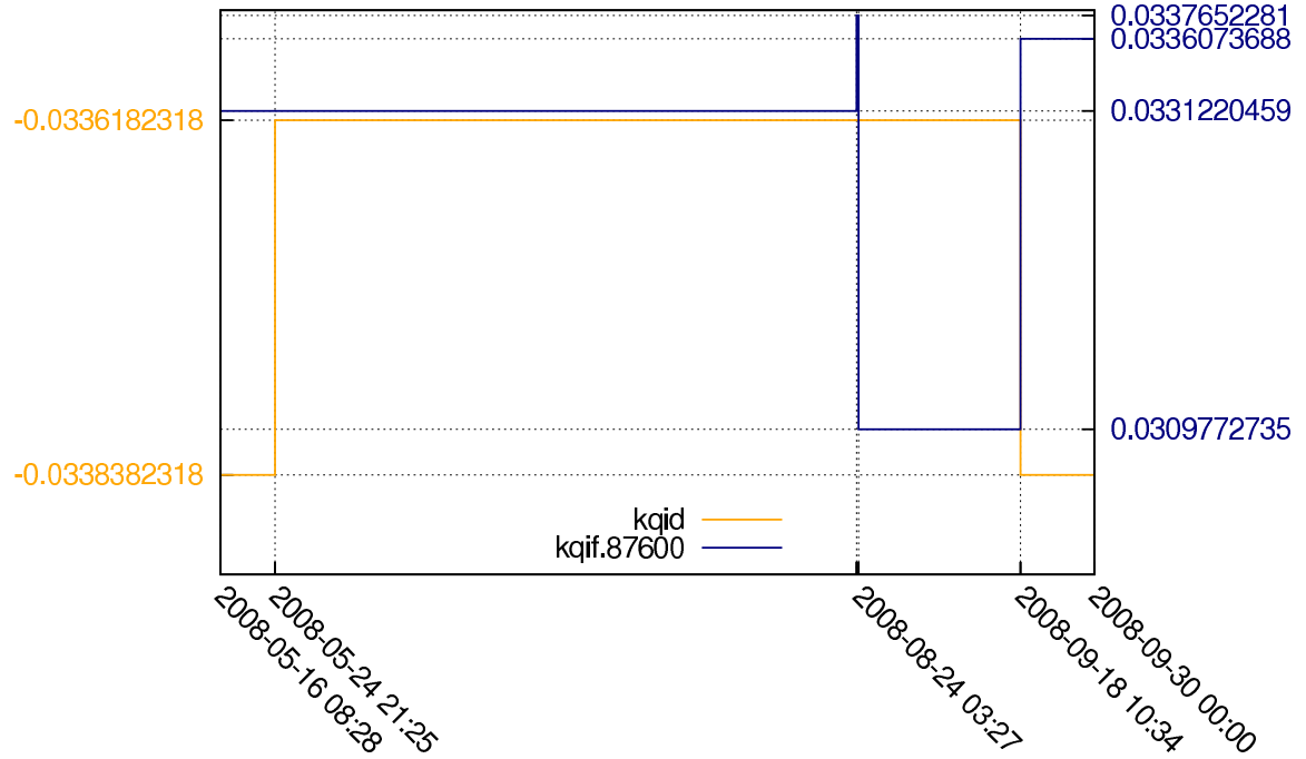
Figure 8.1.: Effect of optics changes of the TI8 transfer line during summer 2008 on two characteristic strength parameters.
