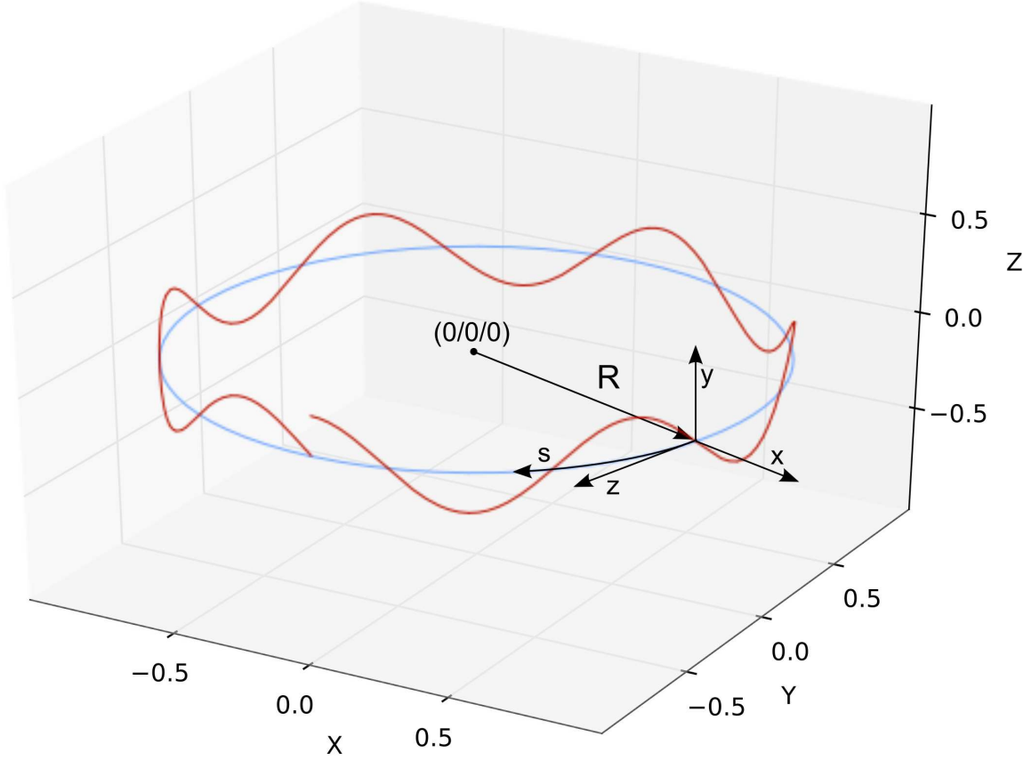
Figure 3.1.: Co-rotating coordinate system.
