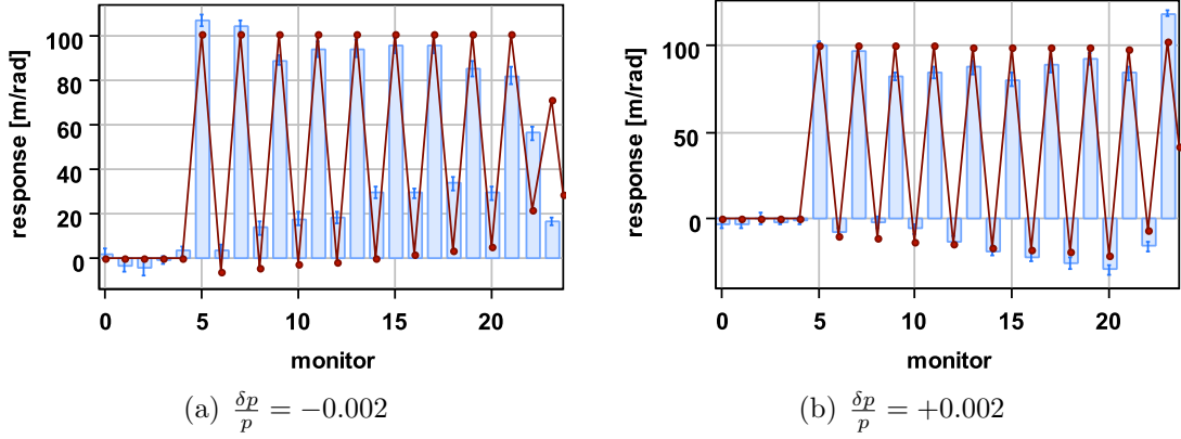
Figure 8.30.: Horizontal response for one horizontal corrector. Bars represent the measured data, dots the nominal model. A clear dependence on \frac{\delta p}{p} is visible, which is only partly reproduced by the model.
