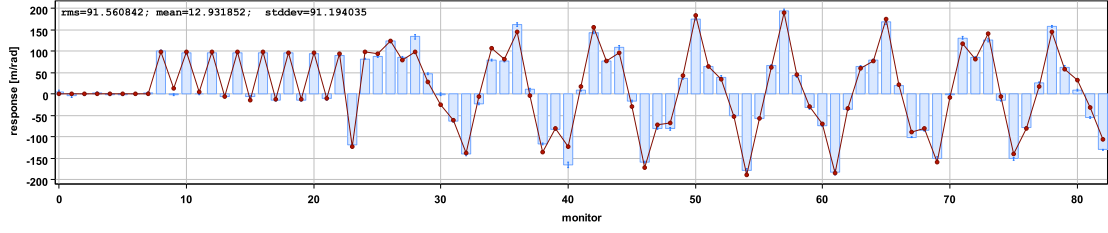
(a) Horizontal orbit response of corrector MCI AH.81604.
