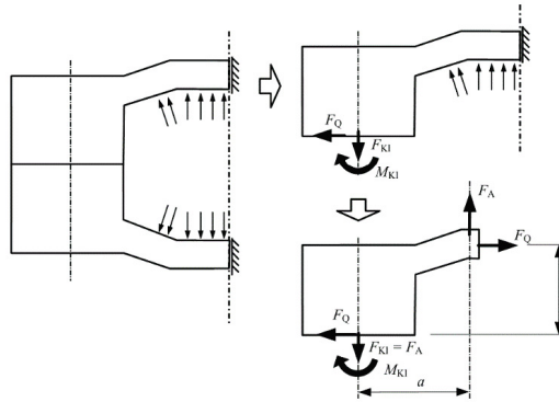
Figure 4. Model for determining s_{sym} for an eccentrically clamped joint from an imaginary concentrically clamped joint
