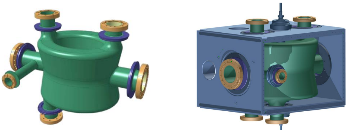
Figure 16: DQW Crab Cavity, bare (left) and in He-vessel (right) ©CERN
