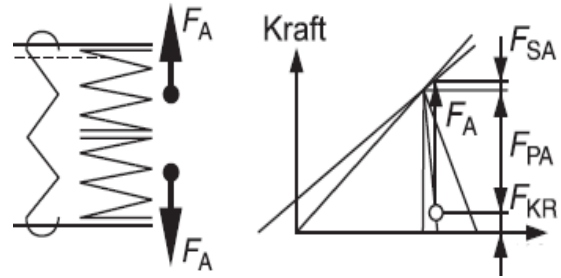
Figure 5: Distortion triangle for n < 1
