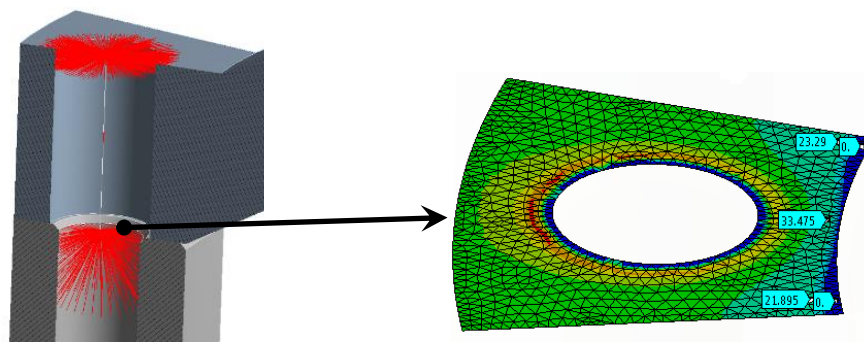
Figure 12: Effect of rigid MPCs on mesh stiffness and the resulting pressure distribution with Class II model
