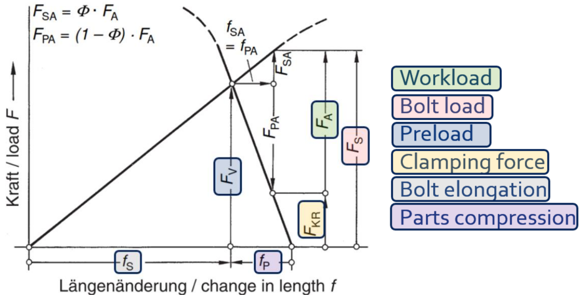
Figure 6: Joint diagram with associated quantities [Pt.1 - Figure 22]
