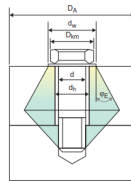
Tapped Thread Joint (TTJ)
