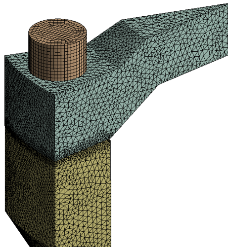
Figure 3: Meshed model
