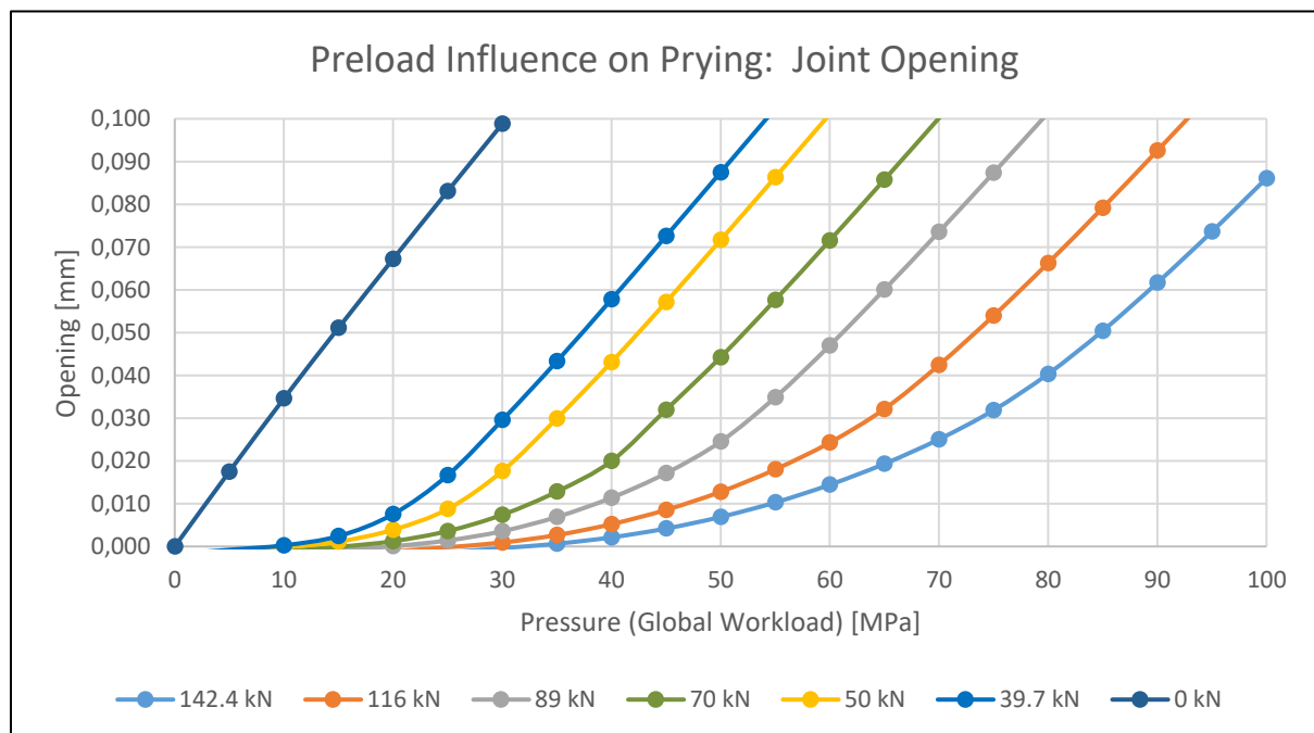
Figure 34: Joint opening for various preload levels
