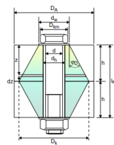
Through Bolted Joint (TBJ)
