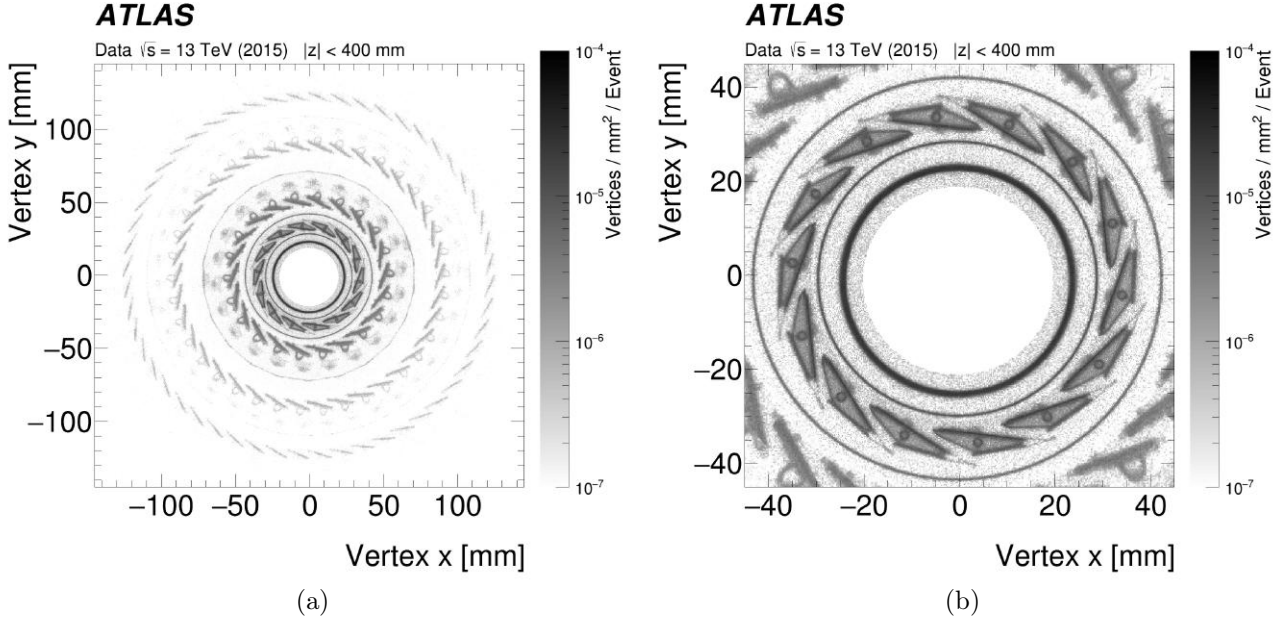
Figure 2.13: Distribution of hadronic-interaction vertex candidates for |\eta| < 2.4 and |z| < 400 mm in collision events: (a) x-y view of the pixel detector; (b) x-y view zooming into the beam pipe and IBL region [57].
