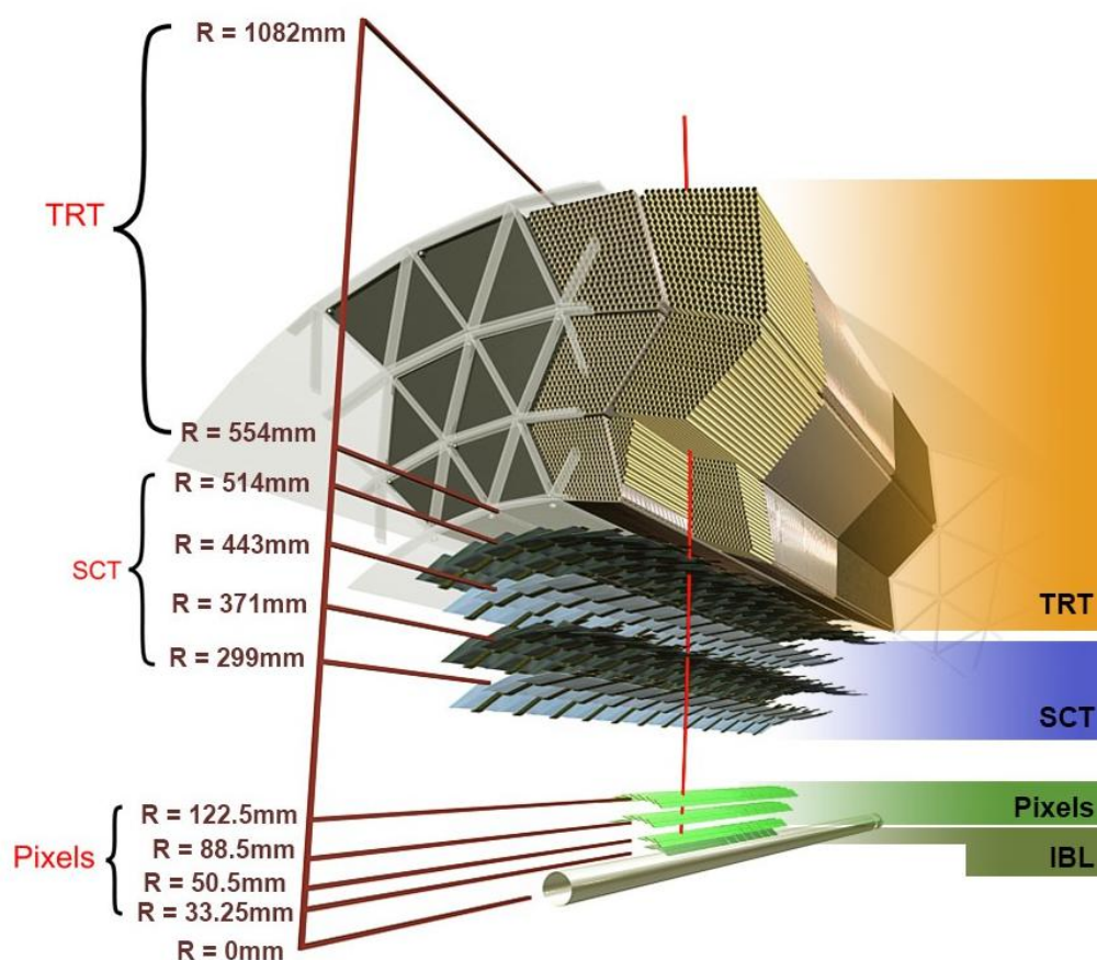
Figure 2.6: Schematic views of the ATLAS Inner Detector and its three sub-detectors.
