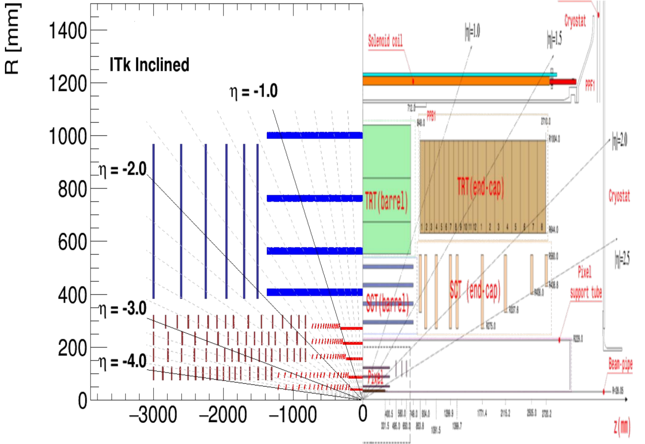
Figure 7.1: Distribution of ITk layers and disks (negative z values) compared to the current ATLAS ID (positive z values). The tracking volume is shown using the same scale.
