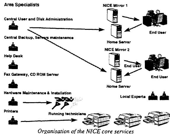
Organisation of the NICE core services
