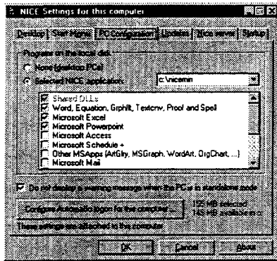
Mirroring the programs disk locally
