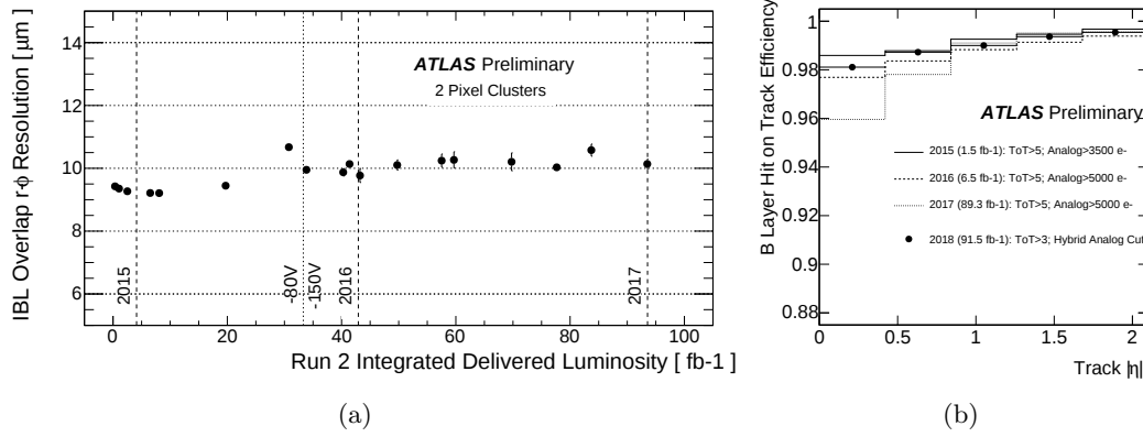
Figure 3.2.: Azimuthal r\phi position resolution versus integrated luminosity (a). It corresponds to the residual r\phi position of the cluster with respect to the reconstructed track crossing the overlap regions in the IBL. The hit efficiency for B-layer against \eta (b) is measured by associating a detected cluster to a reconstructed track. Inefficiencies come from outliers, that are clusters too far from the track, or missing clusters [60].
