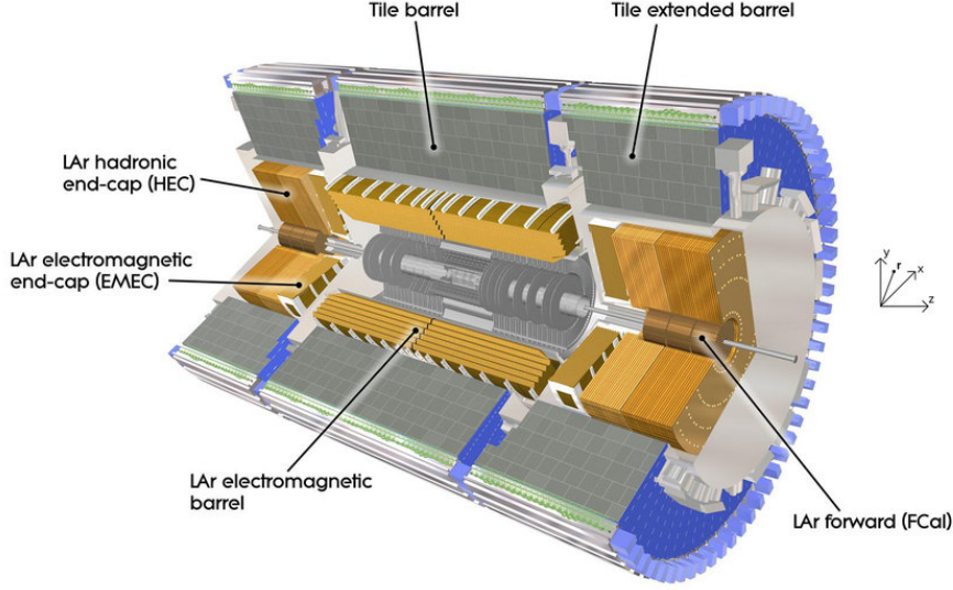
Figure 2.3.: Layout of the ATLAS Calorimetry system © CERN.
