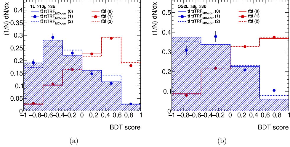
Figure 5.6.: Separation plots for single lepton (a) and opposite-sign dilepton (b) channel. The t\bar{t} estimation is given by t\bar{t} TRF method, described in Section 7.1.
