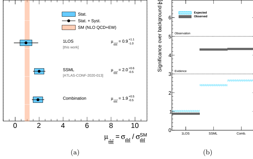
Figure 8.7.: Comparison of the measured signal strength in the individual channels and in the combination (a). Comparison of the significance of the tt\bar{t}\bar{t} signal over the background-only hypothesis in the individual channels and in their combination (b).
