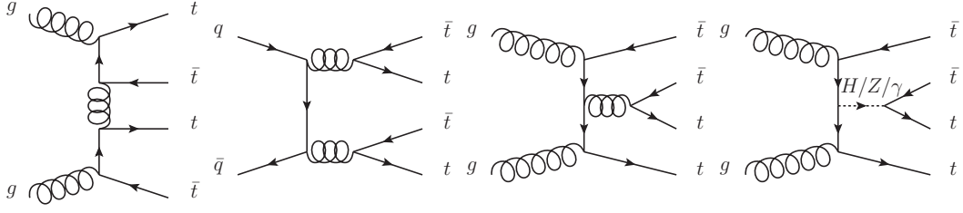
Figure 1.5.: Examples of Leading Order (LO) QCD diagrams contributing to t\bar{t}t\bar{t} production at hadron colliders.
