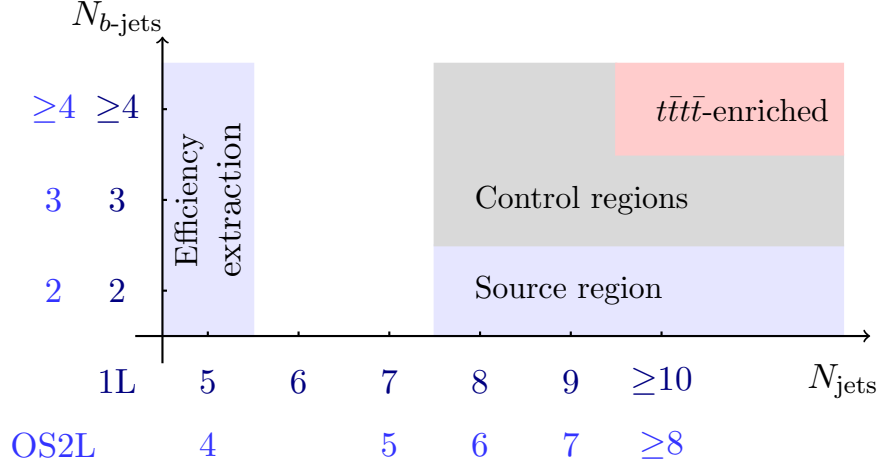
Figure 7.3.: Regions definition for t\bar{t} TRF method derivation and application.
