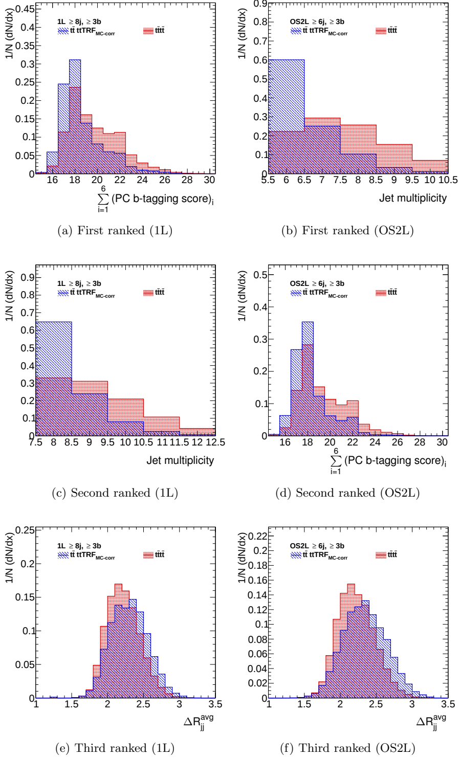
Figure 5.5.: Comparison of the distributions for t\bar{t} and t\bar{t}t\bar{t} for the most important variables in the BDT training in single lepton (1L, left column) and opposite-sign dilepton (OS2L, right column) channels. The variables are displayed from top to bottom in order of importance. The distributions for t\bar{t} are obtained with the t\bar{t} TRF method, described in Section 7.1.
