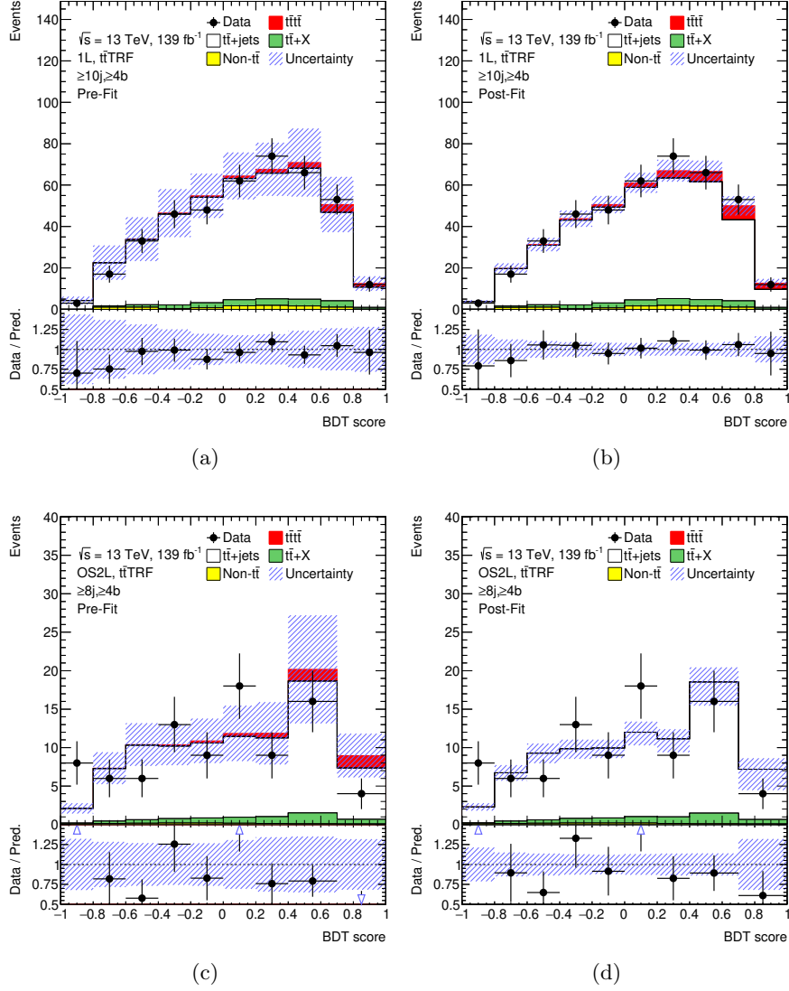
Figure 8.1.: Pre-fit and post-fit distributions of the BDT score for the most sensitive regions in the single-lepton (a,b) and opposite-sign dilepton channel (c,d). Since the the fit in the opposite-sign dilepton channel yield a negative value for the signal strength of the t\bar{t}t\bar{t} process, the t\bar{t}t\bar{t} is not displayed in (d).
