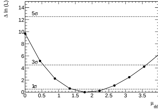
Figure 8.6.: Scan of the likelihood values as a function of the t\bar{t}t\bar{t} signal strength. The lines are in correspondence of the values of the likelihood at \mu_{t\bar{t}t\bar{t}} = 0 at which different values of the signal significances are reached in terms of standard deviations ( \sigma ).
