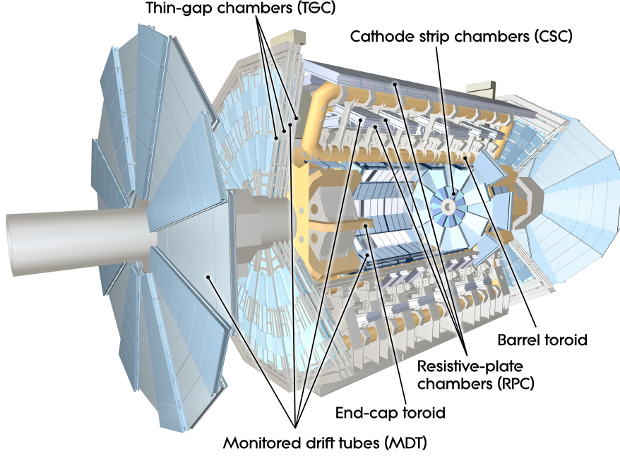
Figure 2.4.: Layout of the ATLAS Muon Detector © CERN.
