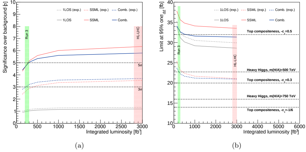
Figure 9.1.: Significance of the t\bar{t}t\bar{t} signal over the background in terms of number of standard deviations ( \sigma ) as a function of the integrated luminosity (a). Limits on the t\bar{t}t\bar{t} production cross-section ( \sigma_{t\bar{t}t\bar{t}} ) at 95% CL as a function of the integrated luminosity. Five predictions for the t\bar{t}t\bar{t} cross-section are shown from two BSM scenarios for different values of the respective parameters (b). The green and pink bands indicate the expected integrated luminosity of Run 3 and HL-LHC, respectively.
