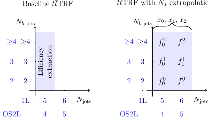
Figure 7.11.: Change of the efficiency extraction regions of the baseline t\bar{t} TRF (described so far, in the left scheme) for the t\bar{t} TRF with the jet multiplicity dependence estimation ( N_j extrapolation, in the right scheme). Here, f_x^y stands for fraction of the events with x more jets than in the extraction region and y radiated b -jets. In terms for b -jet and jet multiplicity they correspond to the events in (5+x)j(2+y)b for the single lepton and in (4+x)j(2+y)b for the opposite-sign dilepton channel. Those values are used to extract the parameters x_0 , x_1 and x_2 .
