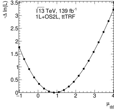
Figure 8.4.: Likelihood value as a function of the signal strength \mu_{t\bar{t}\bar{t}} for the combination of the single lepton and opposite-sign dilepton channels.
