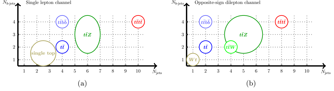
Figure 5.1.: Summary of signatures for t\bar{t}t\bar{t} and main background processes at LO in terms of jets and b -jets multiplicity for the single lepton (a) and opposite-sign dilepton (b) channels.
