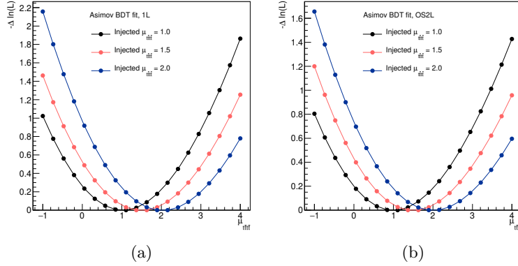
Figure B.3.: Likelihood scans for different injected signal strength \mu_{t\bar{t}t\bar{t}} for the signal lepton (a) and opposite-sign dilepton (b) channels.
