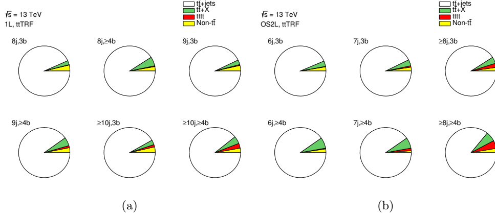
Figure 5.3.: Background composition in the 1LOS channel: six regions at increasing number of jets and b -jets for both single lepton (a) and opposite-sign dilepton (b) channels. Regions are labelled as XjYb , indicating a region that requires for X jets and Y b -jets. The label t\bar{t}+X stands mostly for t\bar{t}+Z/W/H , while Non-t\bar{t} events include all the processes without a top quark pair in the final state (single-top production, W/Z +jets, diboson). The estimation of the t\bar{t} +jets background here is obtained with the t\bar{t} TRF method, described in Section 7.1.
