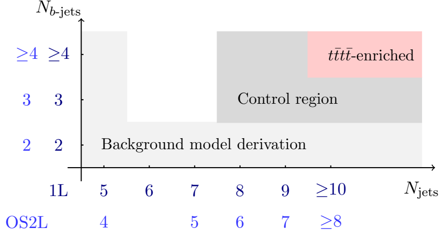
Figure 5.2.: Region categorisation in the 1LOS channel.
