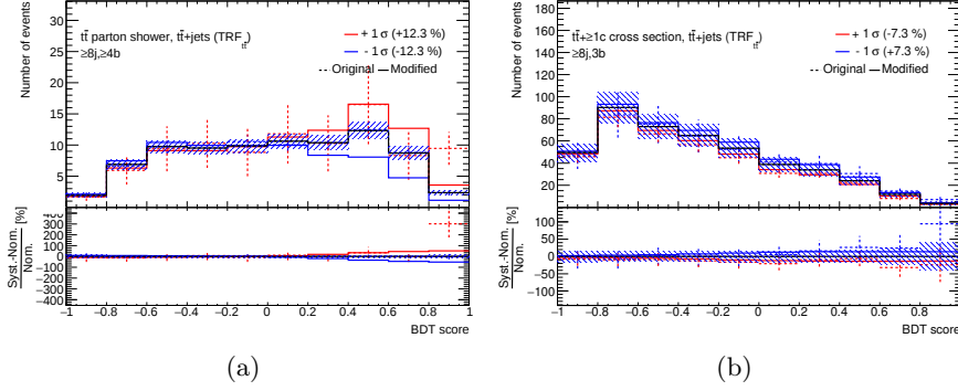
Figure A.2.: Pre-fit uncertainties associated to t\bar{t} parton shower and hadronisation modelling in OS2L \geq 8j \geq 4b region (a) and t\bar{t}+c -jets normalisation (b) in 1L \geq 8j3b region. Red points refer to the original variation, with associated statistical error. The red solid line is obtained by smoothing the uncertainty consistently with the statistics of the variation. The blue solid line is obtained by symmetrising the red one. Red and blue solid lines give the uncertainty on the prediction.
