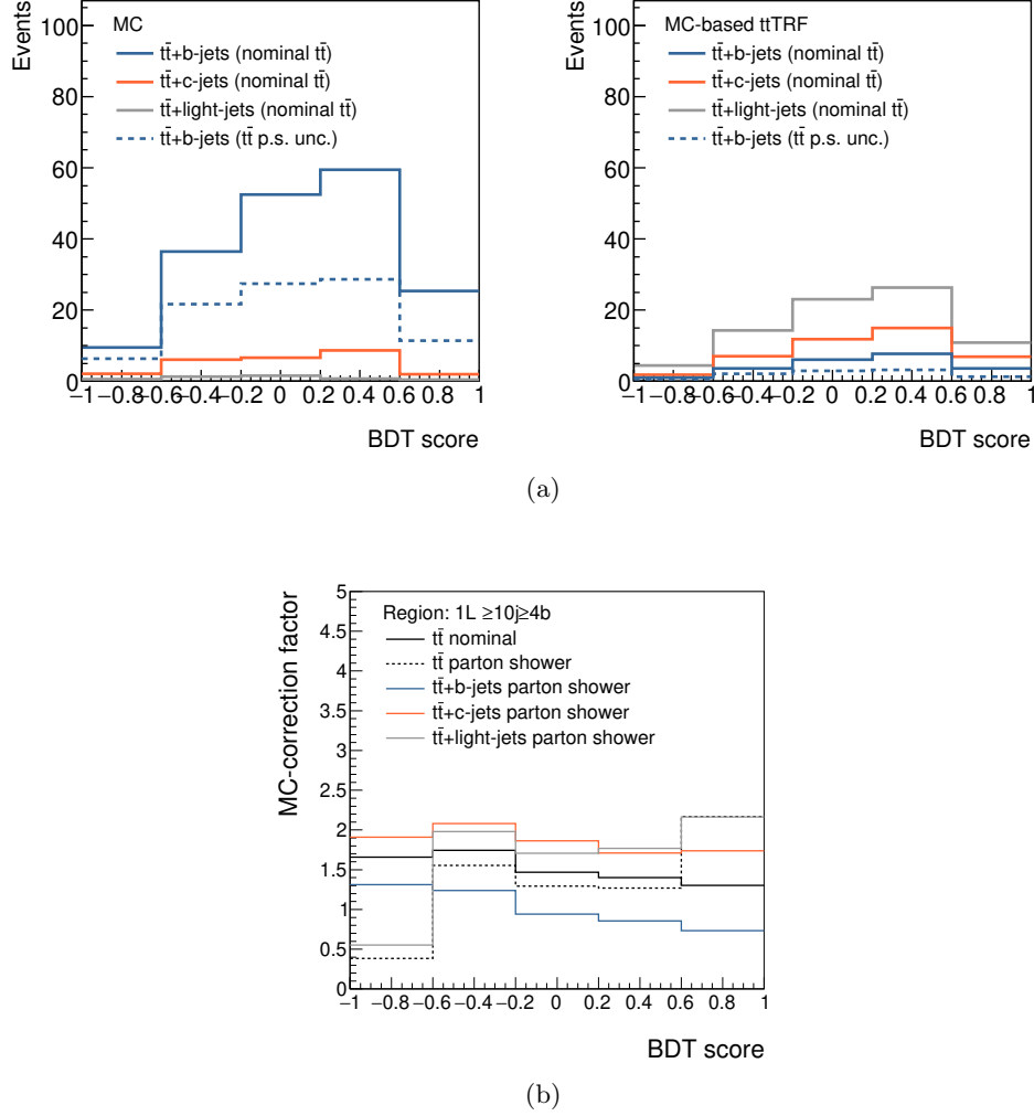
Figure 7.16.: Distributions of the BDT score for the components used for the evaluation of the uncertainty associated to the choice of the parton shower and hadronisation algorithm on the t\bar{t}+b -jets prediction with the t\bar{t} TRF method (a). The yields of the different flavour components of the t\bar{t} radiation in the MC prediction and in the MC-based t\bar{t} TRF prediction are shown on the left and right, respectively. The figures refer to the \geq 10j \geq 4b region in single lepton (1L) channel. Comparison of the corresponding MC correction factors for “flavour-splitted” and inclusive variations with the nominal one (b).
