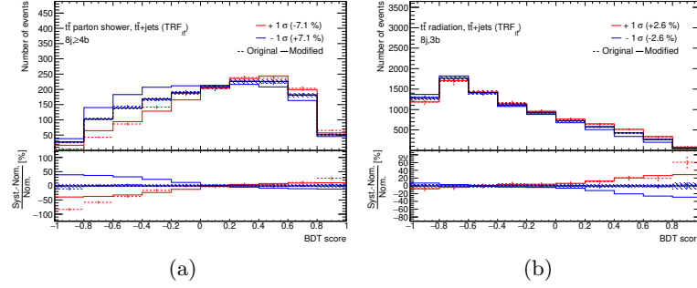
Figure 7.20.: Pre-fit uncertainties associated to t\bar{t} parton shower and hadronisation modelling in 1L 8j \geq 4b region (a) and hdamp choice (b) in 1L 8j3b region as a function of the BDT score. Red points refer to the original variation, with associated statistical error. The red solid line is obtained by smoothing the uncertainty consistently with the statistical uncertainty of the variation. The blue solid line is obtained by symmetrising the red one. Red and blue solid lines give the uncertainty on the prediction.
