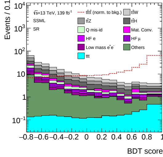
Figure 5.8.: Shape comparison of the BDT score in SSML channel events in the signal region between signal and total background. The event categories are defined in Table 5.5. The t\bar{t}t\bar{t} contribution is normalised to the total background yield.
