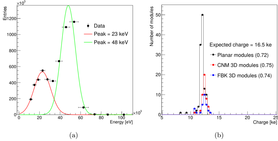
Figure 3.5.: Typical measured spectrum from ^{241}\text{Am} in production stage data (a). Summary of the photopeak energy for all the analysed modules is shown in (b). In parenthesis the fraction of average observed charge with respect to the expected 16.5ke for the different module types (planar and 3D from CNM and FBK factories).
