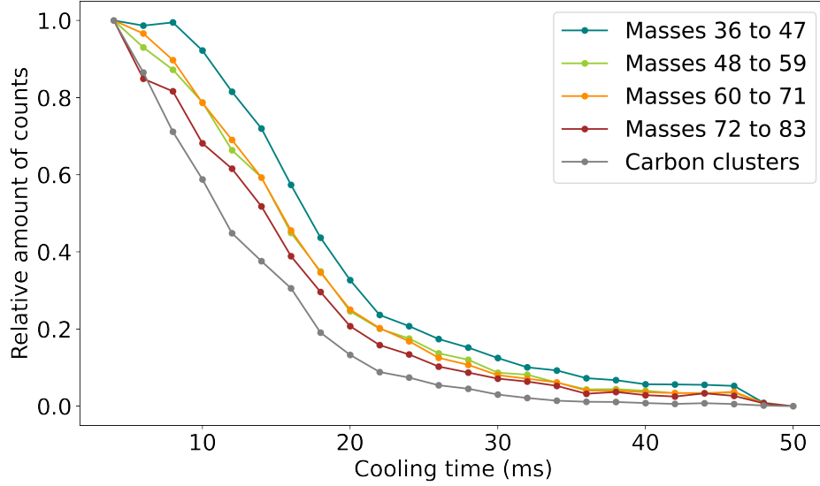
Figure 10: Sum of counts over the eleven hydrocarbon peaks corresponding to each carbon cluster, relative to the first measurement, against the cooling time in the main buncher. The relative amount of counts for the carbon clusters from Figure 9 is shown in grey as comparison.
