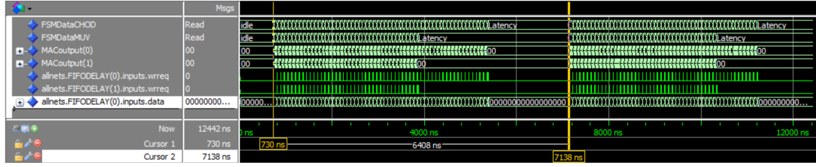
Figure 3.8. Simulation of a MTP extraction. All the primitives are passed to FIFODELAY(i), which is the main component of the Delay Generator. The figure shows a packet frame of 6.4 \mu s.
