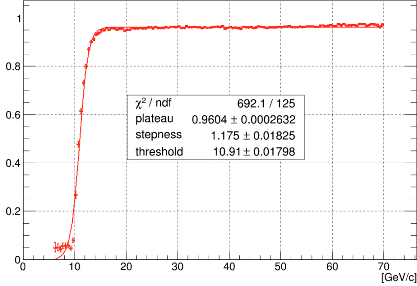
Figure 5.3. Efficiency of RICH primitive generation as measured from a K_{\mu 2} sample.
