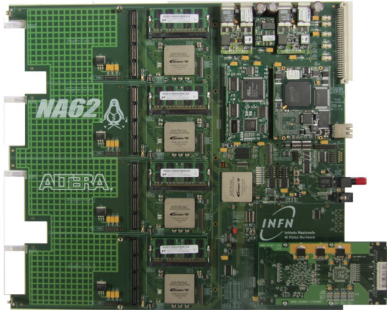
Figure 2.14. TEL62 read-out board.
