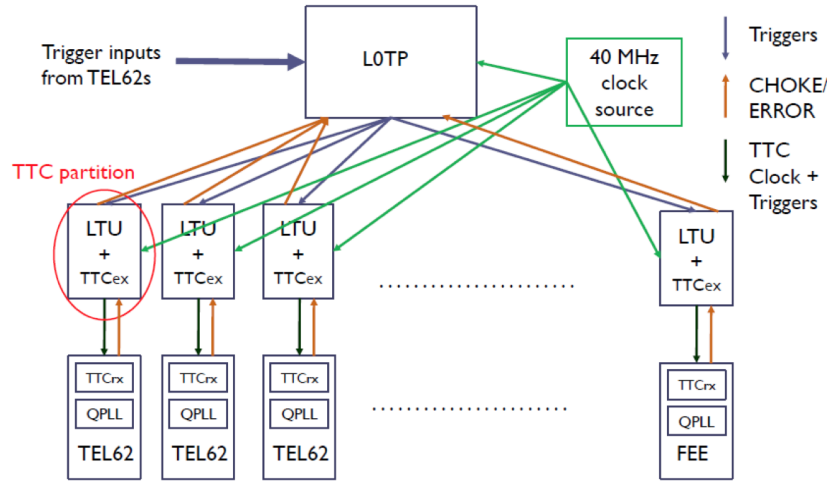
Figure 2.13. Schematic view of the Timing, Trigger Control.
