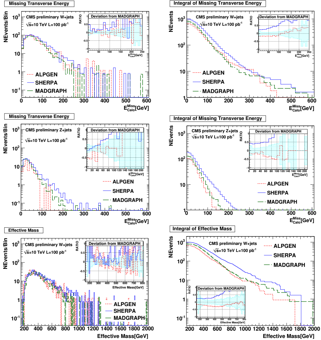
Figure 6.25: Differential (left) and integral (right) E_{Calo}^{Miss} and effective mass M_{eff} = E_{Calo}^{Miss} + \sum_{i=5}^n P_T^{j_i} distribution for W+jets and Z+jets (middle) production simulated with Alpgen, Sherpa and Madgraph after applying the single muon selection step. Ratio: relative differences of Alpgen and Sherpa with respect to Madgraph.
