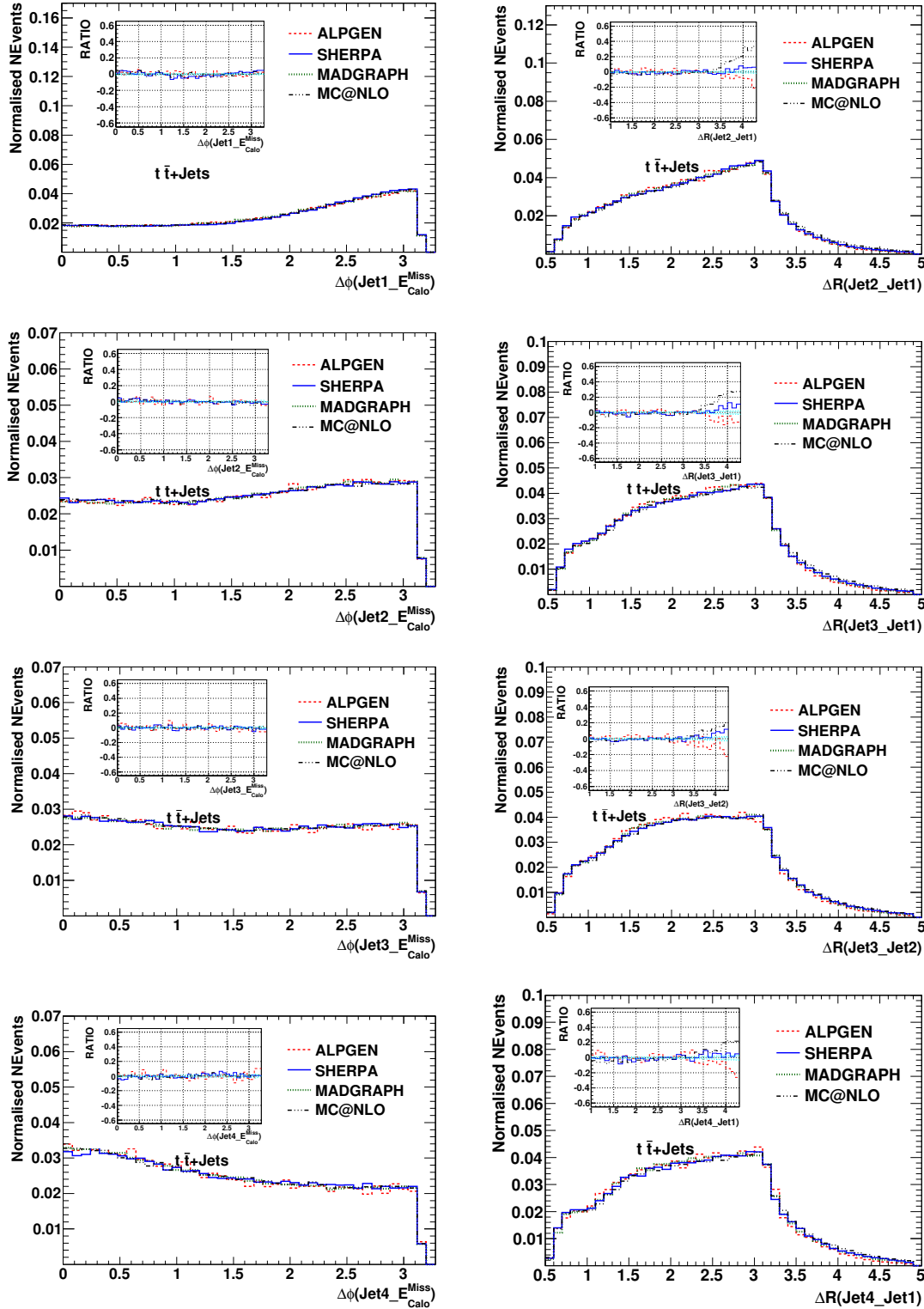
Figure 5.36: Left: Azimuthal angle ( \Delta\phi ) between leading jets and calorimeter missing transverse energy for inclusive t\bar{t} + \text{jets} . Right: \Delta R separation between leading jets. Ratio: relative differences of Alpgen, Sherpa and MC@NLO with respect to Madgraph.
