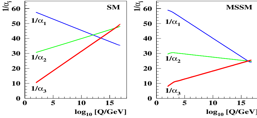
Figure 2.3: Unification of the coupling constants in the SM (Left) and Minimal Supersymmetric SM (Right) [46].
