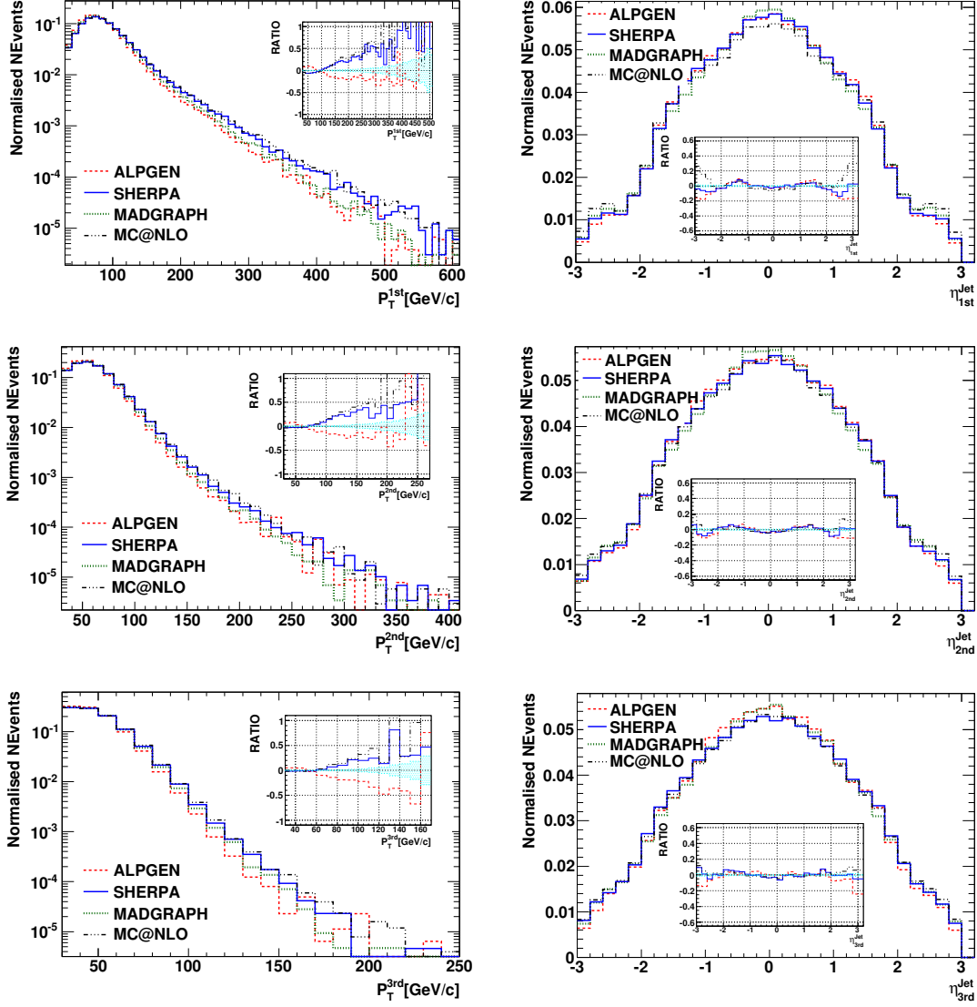
Figure 5.29: P_T (left) and \eta (right) distribution of the three leading jets for the inclusive Alpgen, Sherpa and Madgraph t\bar{t} +jets production at detector level. Ratio: relative differences of Alpgen and Sherpa with respect to Madgraph.
