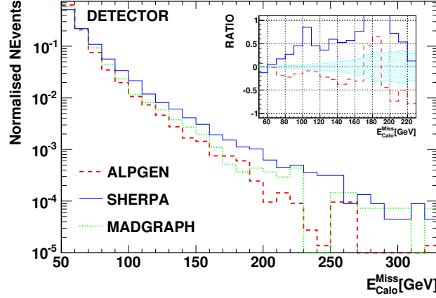
Figure 5.6: Detector level E_{Calo}^{Miss} > 50 GeV distribution for the inclusive Z(l\bar{l}) +jets ( l = e, \mu, \tau ) production simulated with Alpgen, Sherpa and Madgraph. Ratio: relative differences of Alpgen and Sherpa with respect to Madgraph.
