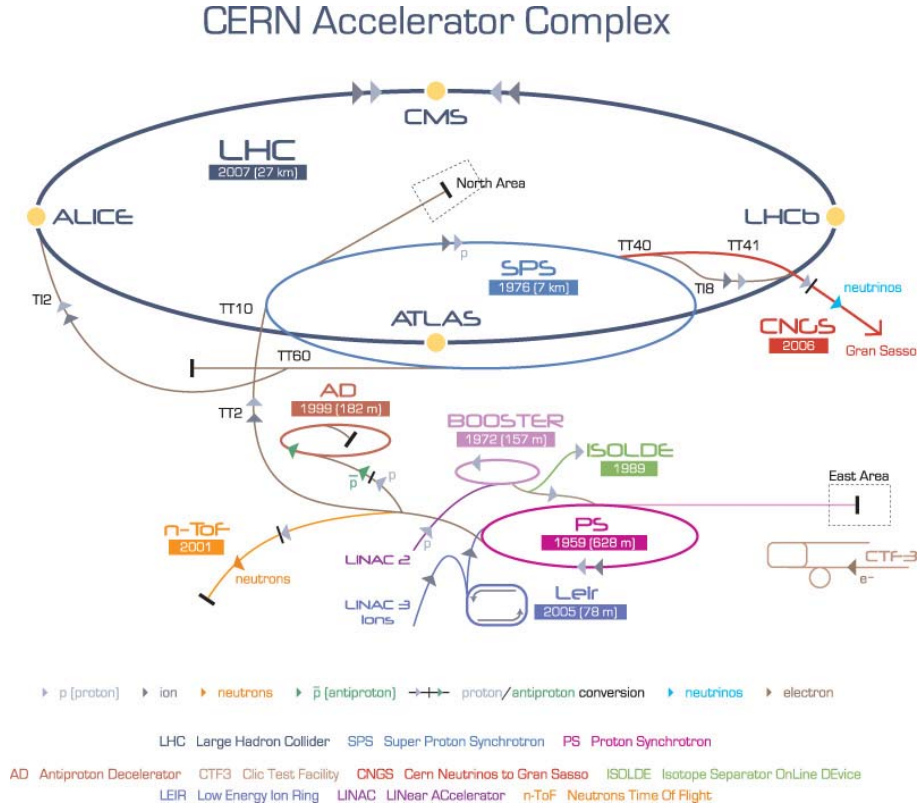
Figure 3.2: Schematic layout of the LHC accelerator complex. The four main experiments are LHCb, which explores b-physics in proton-proton collisions, ALICE, which investigates heavy-ion physics in lead-lead collisions, and the two general purpose experiments ATLAS and CMS [55].
