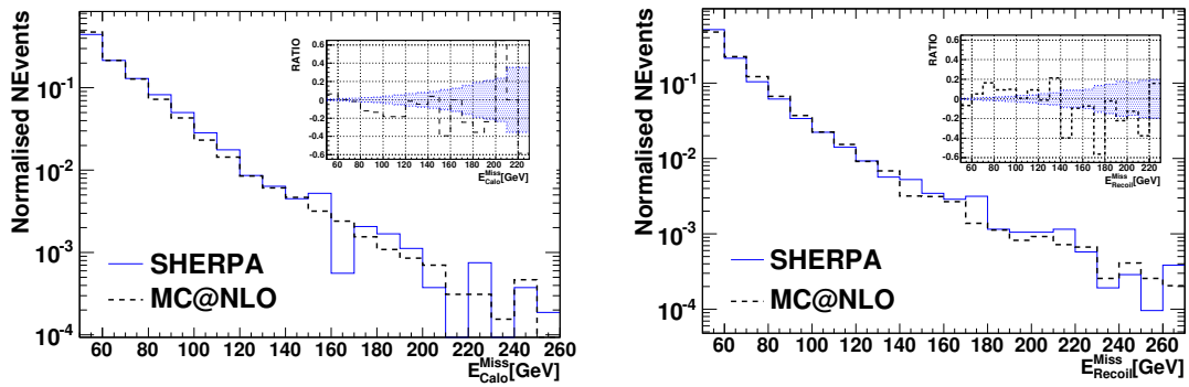
Figure 5.4: Detector level E_{Calo}^{Miss} > 50 GeV (left) and E_{Recoil}^{Miss} > 50 GeV (right) distributions for the exclusive Z(\mu\bar{\mu}) +1jet samples simulated with MC@NLO and Sherpa. Ratio: relative difference of MC@NLO with respect to Sherpa. The (blue) shaded area represents the statistical uncertainty.
