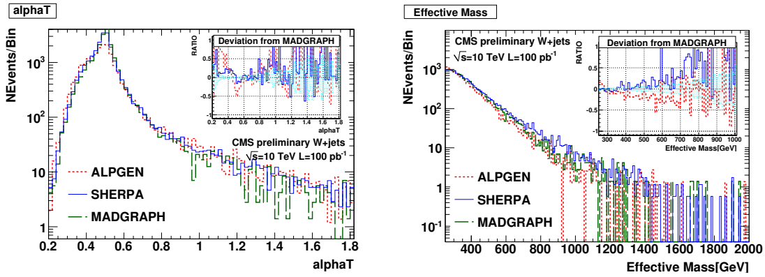
Figure 6.14: \alpha_T (left) and effective mass M_{eff} = E_{Calo}^{Miss} + \sum_{i=5}^n P_T^{j_i} (right) distribution for W+jets production simulated with Alpgen, Sherpa and Madgraph after applying the lepton-veto selection step. Ratio: relative differences of Alpgen and Sherpa with respect to Madgraph.
