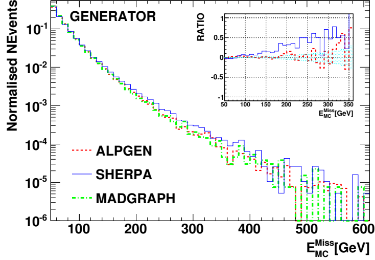
Figure 5.14: Generator level E_{MC}^{Miss} > 50 GeV distribution for the inclusive W(l\nu) +jets ( l = e, \mu, \tau ) production simulated with Alpgen, Sherpa and Madgraph. Ratio: relative differences of Alpgen and Sherpa with respect to Madgraph.
