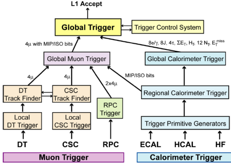
Figure 3.9: Design of the CMS L1-Trigger [63].
