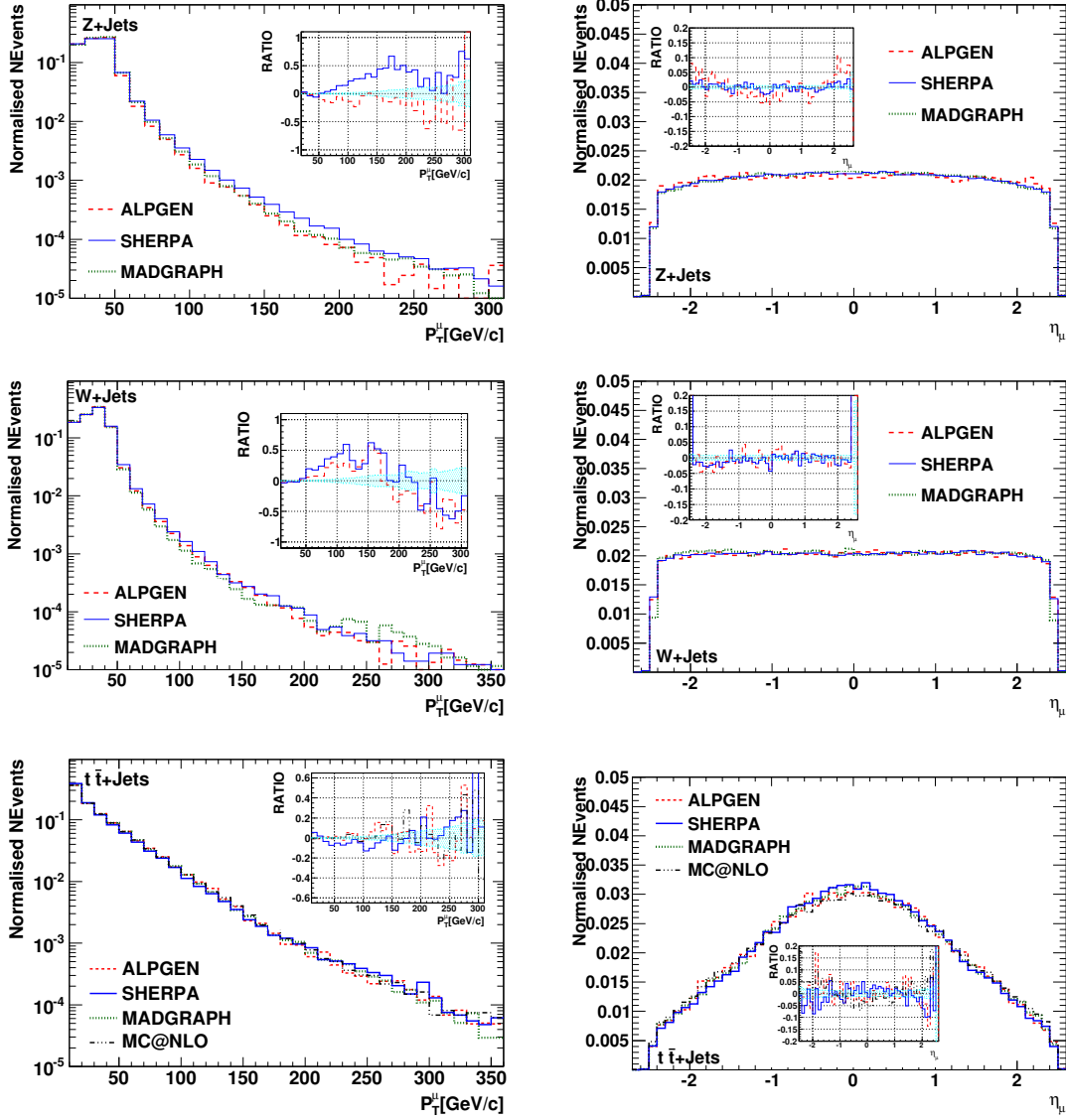
Figure 5.42: Left: detector level P_T distribution of muons for the Z(l\bar{l}) +jets, W(l\nu) +jets ( l = e, \mu, \tau ) and t\bar{t} +jets production simulated with Alpgen, Madgraph, MC@NLO and Sherpa. Right: detector level \eta distribution of muons for Z(l\bar{l}) +jets, W(l\nu) +jets and t\bar{t} +jets calculated with Alpgen, Madgraph and Sherpa. Ratio: relative difference of Alpgen, Sherpa and MC@NLO with respect to Madgraph.
