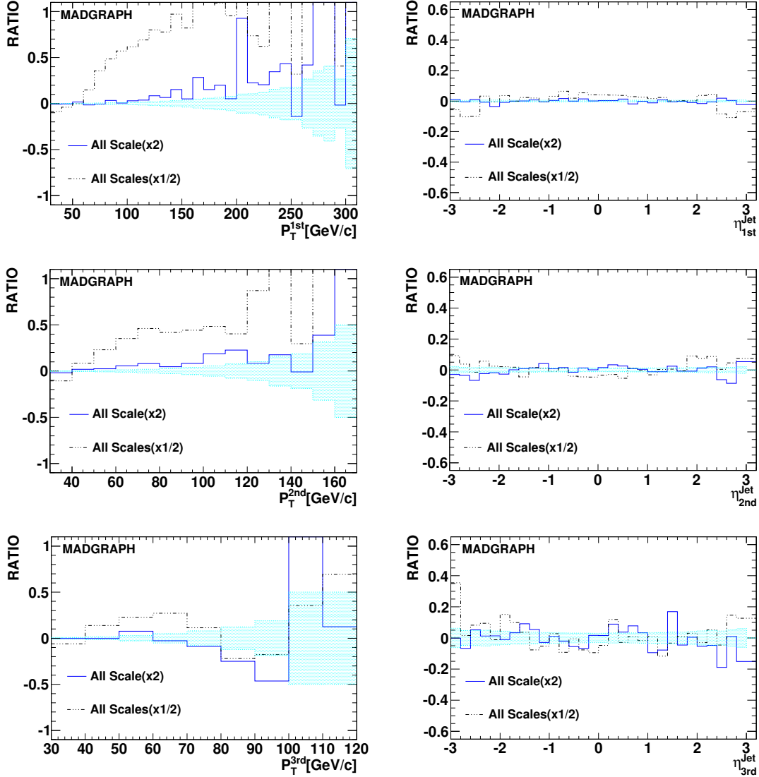
Figure 5.28: The ratio P_T (left) and \eta (right) distribution of the three leading jets systematics for the inclusive Madgraph W(l\nu)+\text{jets} production ( l = e, \mu, \tau ). Ratio: relative differences of various Madgraph settings with respect to Madgraph default.
