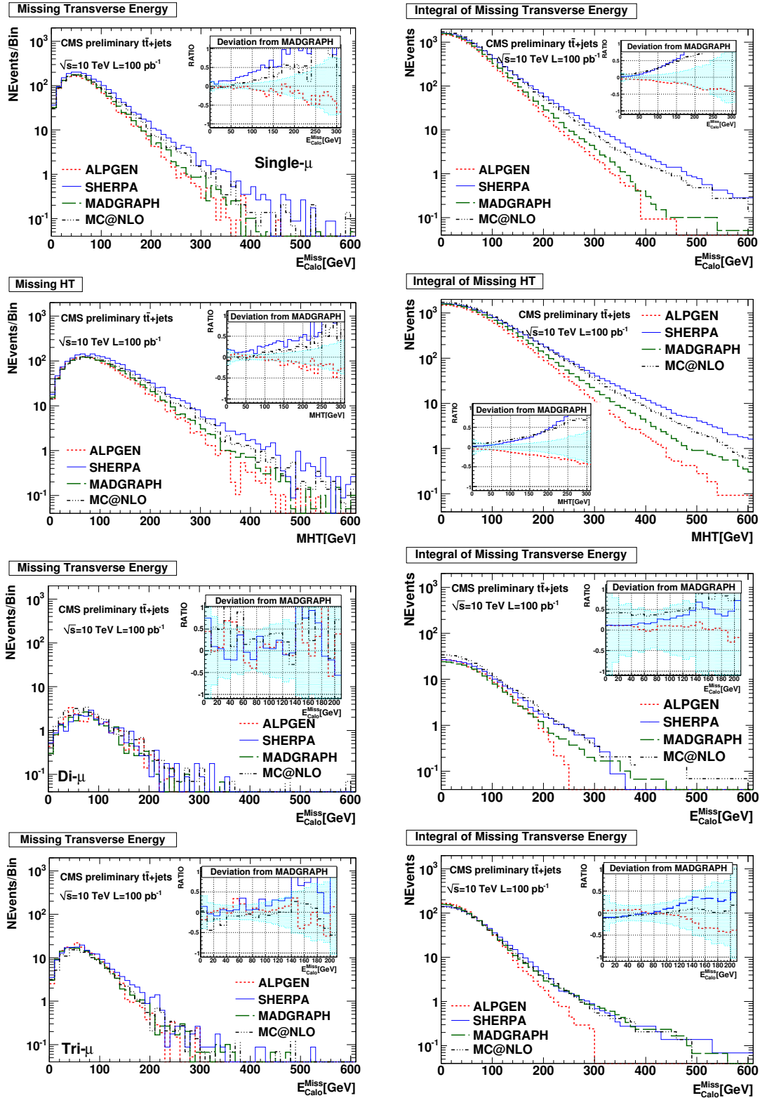
Figure 6.23: Differential (left) and integral (right) E_{\text{Calo}}^{\text{Miss}} and MHT (second-row) distribution for t\bar{t}+\text{jets} production simulated with Alpgen, Sherpa, Madgraph and MC@NLO after applying the muon selection step. Ratio: relative differences of Alpgen, Sherpa and MC@NLO with respect to Madgraph.
