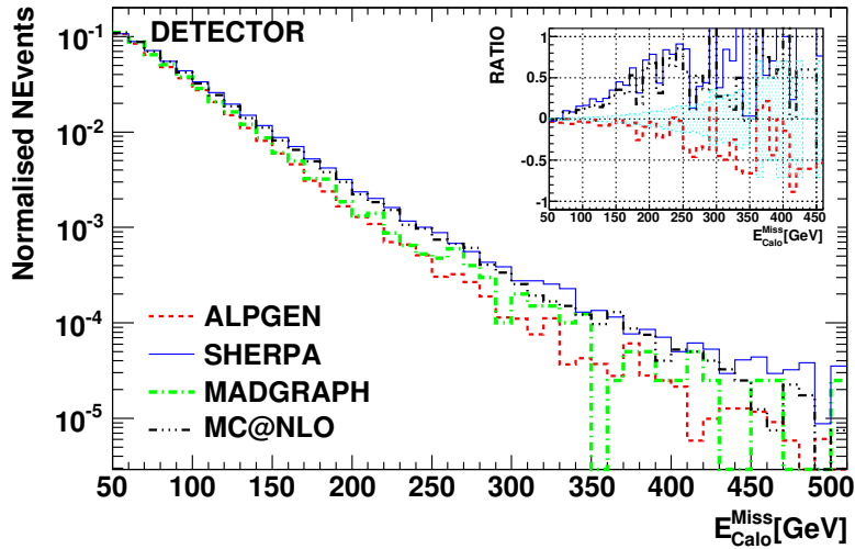
Figure 5.19: Detector level E_{Calo}^{Miss} > 50 GeV distribution for the inclusive t\bar{t} +jets production simulated with Alpgen, Sherpa, MC@NLO and Madgraph. Ratio: relative differences of Alpgen, Sherpa and MC@NLO with respect to Madgraph.
