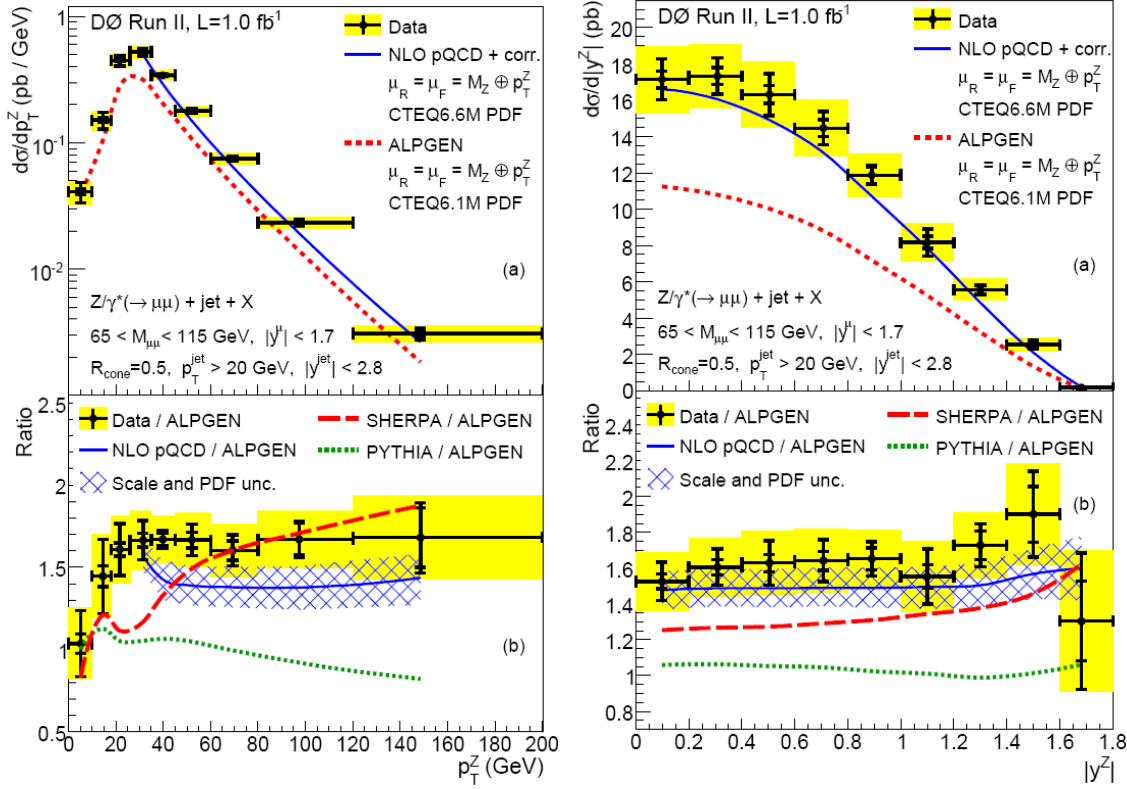
Figure 4.11: Upper: The measured cross section in bins of the leading jet P_T^Z and rapidity for Z^0(\rightarrow \mu\mu)/\gamma^* + \text{jets} + X events. Predictions from NLO and Alpgen are compared to the data. Lower: The ratio of data and predictions from NLO corrections, Sherpa and Pythia to the prediction from Alpgen [28].
