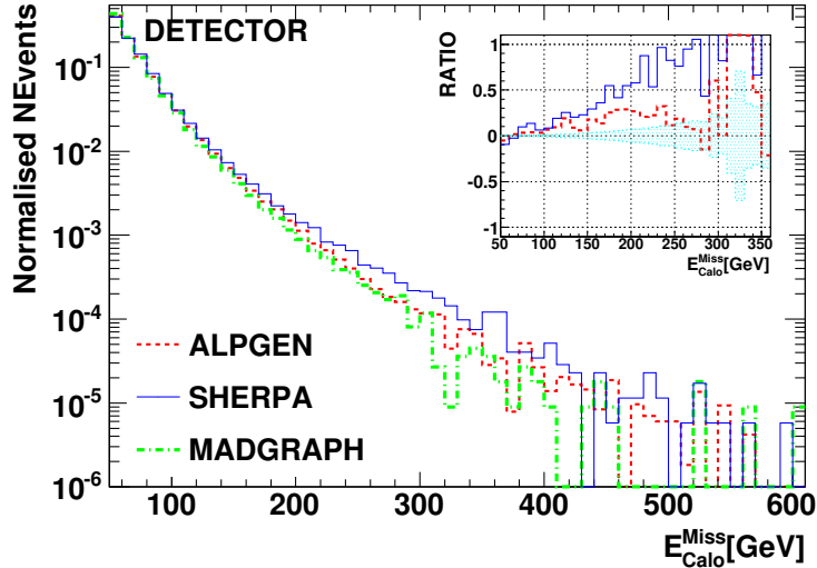
Figure 5.15: Detector level E_{Calo}^{Miss} > 50 GeV distribution for the inclusive W(l\nu) +jets ( l = e, \mu, \tau ) production simulated with Alpgen, Sherpa and Madgraph. Ratio: relative differences of Alpgen and Sherpa with respect to Madgraph.
