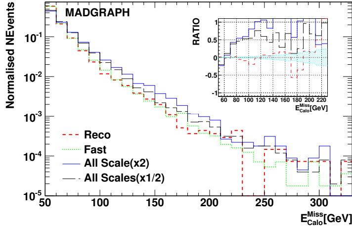
Figure 5.8: Detector level E_{Calo}^{Miss} > 50 GeV distribution for the inclusive Z(l\bar{l}) +jets ( l = e, \mu, \tau ) production simulated with various Madgraph settings. Ratio: relative differences of various Madgraph settings with respect to Madgraph (fast).
