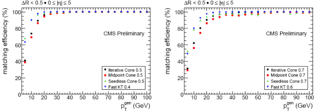
Figure 3.12: Matching efficiency vs P_T^{\text{gen}} for R = 0.5 / D = 0.4 (left) and R = 0.7 / D = 0.6 (right). Matching efficiency is defined as the ratio of number of particle jets matched to the calorimeter jet within the the corresponding \Delta R and the total number of particle jets. The efficiencies of jets reconstructed with the Fast k_T and SiSCone algorithms indicate better performance [103].
