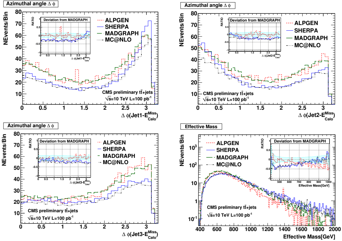
Figure 6.18: Azimuthal angle \Delta\phi between three leading jets and missing transverse energy (top and lower-left) and effective mass M_{\text{eff}} = E_{\text{Calo}}^{\text{Miss}} + \sum_{i=5}^n P_T^{j_i} (lower-right) are shown for t\bar{t} +jets before the final selection step. Ratio: relative differences of Alpgen, Sherpa and MC@NLO with respect to Madgraph.
