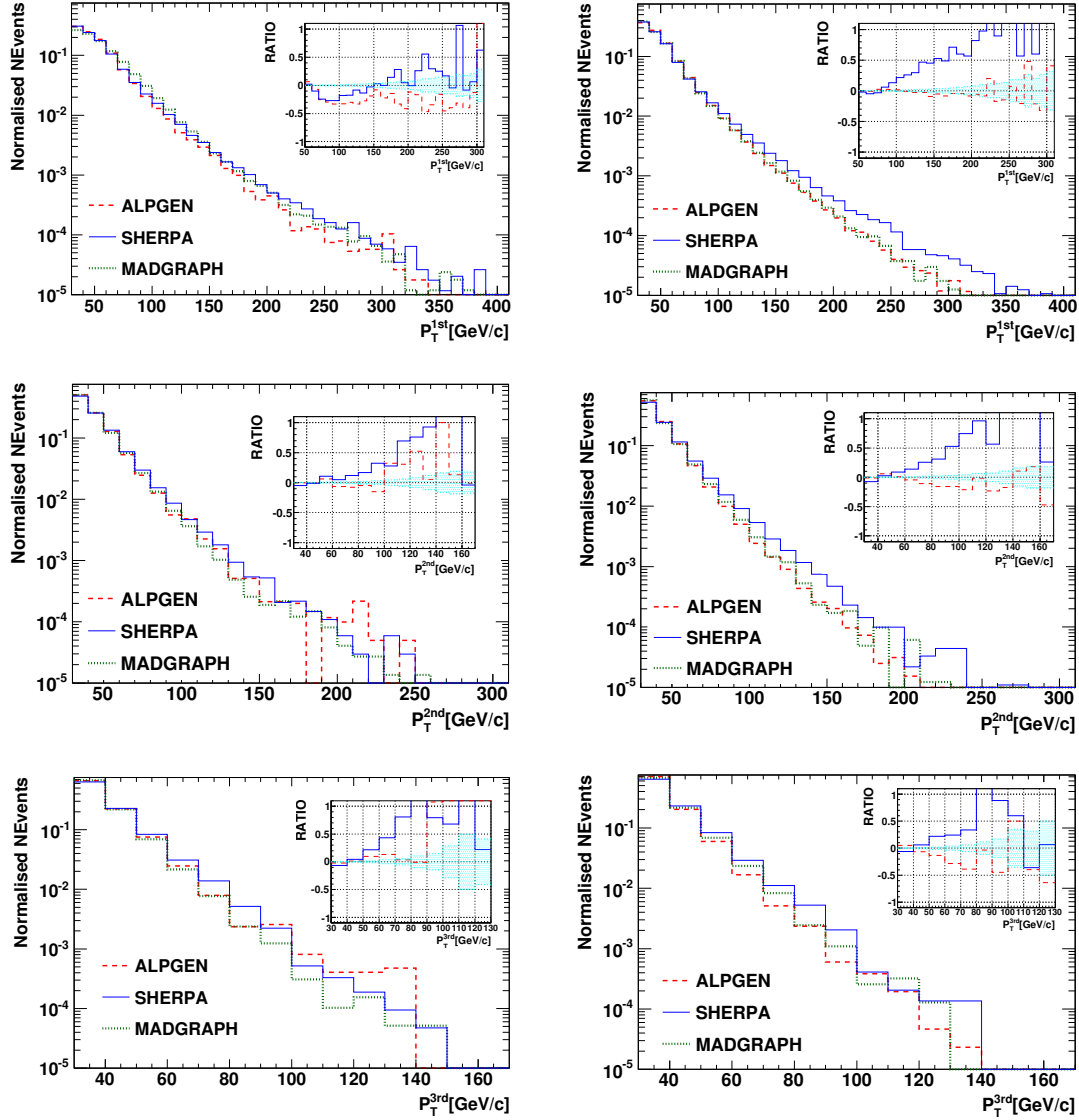
Figure 5.26: P_T distribution of the three leading jets for the inclusive Alpgen, Sherpa and Madgraph Z(l\bar{l}) +jets (left) and W(l\nu) +jets (right) ( l = e, \mu, \tau ) production at detector level. Ratio: relative differences of Alpgen and Sherpa with respect to Madgraph. The (blue) shaded area represents the statistical uncertainty.
