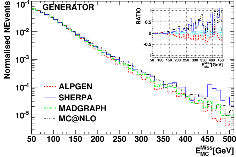
Figure 5.18: Generator level E_{MC}^{Miss} > 50 GeV distribution for the inclusive t\bar{t} +jets production simulated with Alpgen, Sherpa, MC@NLO and Madgraph. Ratio: relative differences of Alpgen, Sherpa and MC@NLO with respect to Madgraph. The (blue) shaded area represents the statistical uncertainty.
