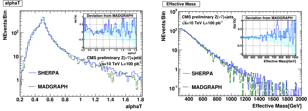
Figure 6.12: \alpha_T (left) and effective mass M_{\text{eff}} = E_{\text{Calo}}^{\text{Miss}} + \sum_{i=5}^n P_T^{j_i} distribution for the Zinvisible+jets production simulated with Sherpa and Madgraph after applying the lepton-veto selection step. Ratio: relative differences of Sherpa with respect to Madgraph.
