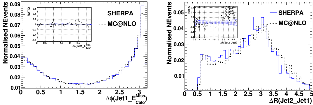
Figure 5.39: Left: Azimuthal angle ( \Delta\phi ) between leading jets and calorimeter missing transverse energy for the exclusive Z(\mu\bar{\mu})+1\text{jet} production at detector level. Right: \Delta R separations between reconstructed leading jets. Ratio: relative difference of MC@NLO with respect to Sherpa.
