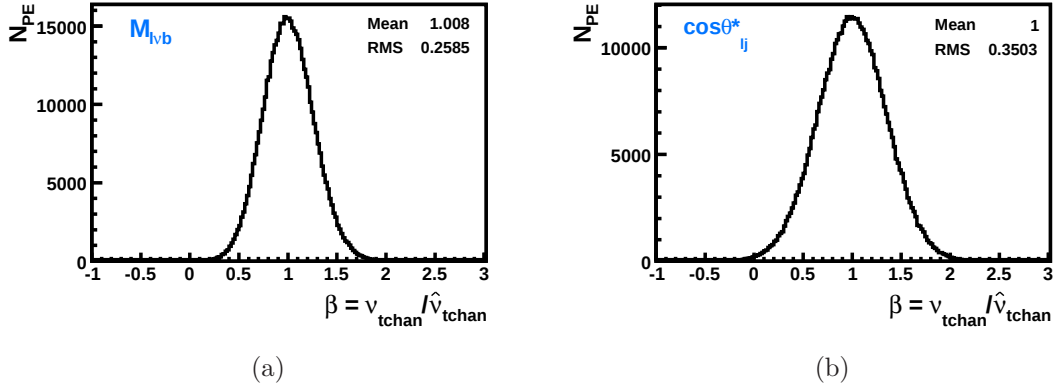
Figure 6.6: Distribution of the signal parameter \beta_1 as obtained from 500,000 pseudo-experiments for M_{l\nu b} in the S_1 scenario (a) and \cos\theta_{lj}^* in the S_{flat} scenario (b).
