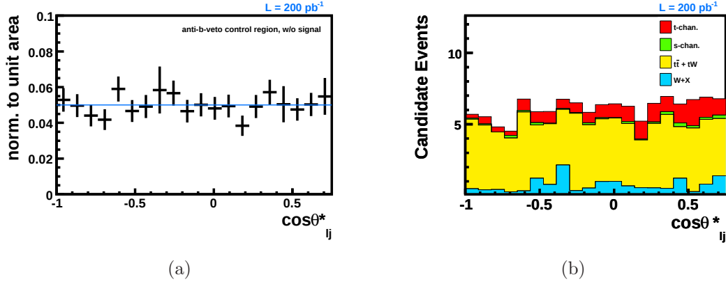
Figure 6.4: Distribution of the restricted \cos \theta_{lj}^* for events in the t\bar{t} -enriched control region, that is for events failing the second b -veto. The shape for these events except for the signal contribution is shown in (a), indicating a flat behavior. The expected distribution including the t -channel signal fraction and normalized to L = 200 \text{ pb}^{-1} is shown in (b).
