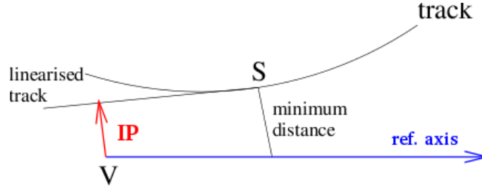
Figure 4.1: Schematic representation of the three-dimensional impact parameter (IP) calculation of a single track with respect to the vertex (V) in three dimensions [100].
