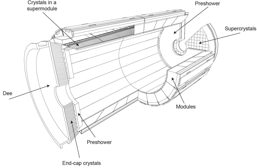
Figure 2.7: A sketch of the electromagnetic calorimeter [70]. The barrel region, where single crystals are combined to supermodules, is extended to \eta = 3.0 by the endcaps which consist of two so-called Dees on each side.
