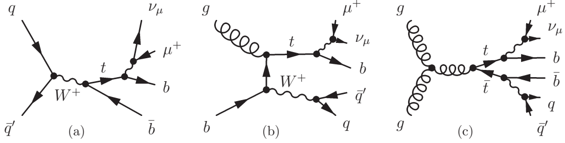
Figure 4.5: Feynman diagrams of s -channel (a) and associated (b) single top-quark production including the decay of the W bosons. Only decay channels with a muon in the final state contribute significantly as background. Subfigure (c) shows a Feynman diagram for a top-quark pair event, where one top quark decay is characterized by a leptonically decaying W boson, whereas the second top-quark decays fully hadronically.
