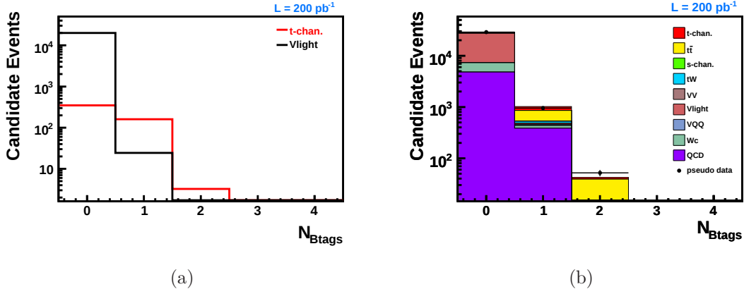
Figure 5.4: Number of b -tagged jets per event when requiring D_{\text{TCHP}} > 5.36 , for signal and Vlight events (a) and all processes (b), normalized to L = 200 \text{ pb}^{-1} .
