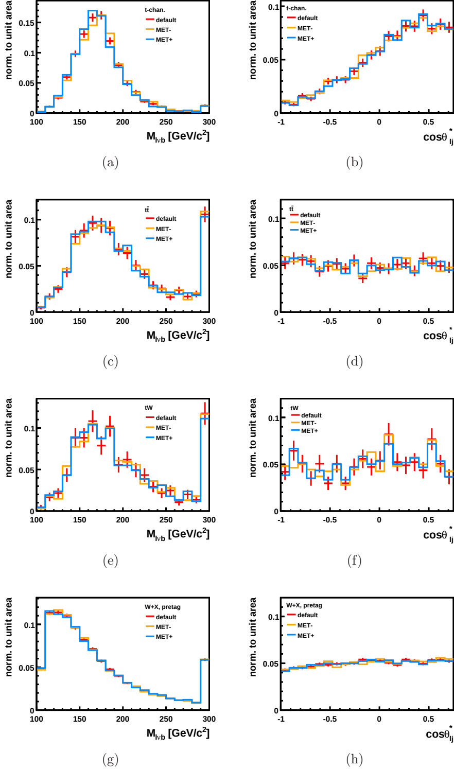
Figure 6.13: Shape comparisons for the invariant top-quark mass M_{lb} (left column) and the restricted \cos\theta_{lj}^* (right column), where the uncorrected E_T^{\text{miss}} fraction is rescaled with respect to the non-scaled default sample, for signal ((a), (b)), t\bar{t} ((c), (d)), tW ((e), (f)), and W+X ((g), (h)). The shapes of the top-quark processes are extracted from the sample having passed the standard selection, while the W+X shapes are obtained from pretag samples, where no b -tagging was applied in order to increase the number of events.
