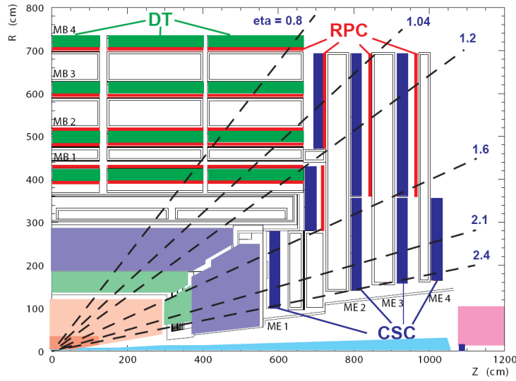
Figure 2.9: Layout of one quarter of the muon system [64]. In the barrel region DT chambers (green) and RPCs (red) are provided, in the endcaps the muons are detected by CSCs (blue) and RPCs.
