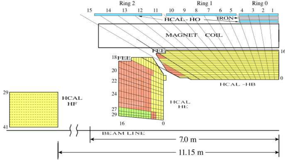
Figure 2.8: Transverse section through a quarter of the HCAL, showing the geometrical configuration [73]. The barrel and the endcap detectors are placed inside the solenoid, followed by the outer calorimeter. The HF modules are located at almost |z| = 11.2 m from the interaction point. The color code denotes the longitudinal segmentation of the read-out system, the location of the front-end electronic devices is indicated by the label FEE.
