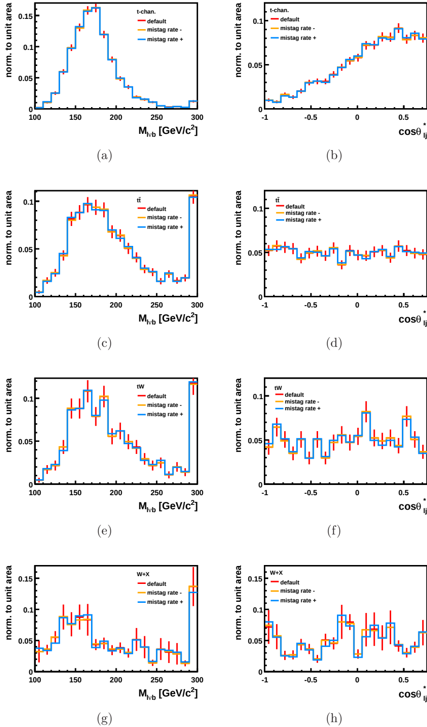
Figure 6.15: Shape comparisons for the invariant top-quark mass M_{lvb} (left column) and the restricted \cos\theta_{lj}^* (right column), where the applied discriminator working points are modified with respect to the expected uncertainty on the corresponding mistag rate ; for signal ((a), (b)), t\bar{t} ((c), (d)), tW ((e), (f)), and W+X ((g), (h)).
