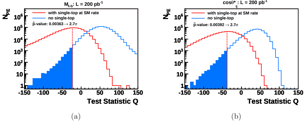
Figure 6.16: Q -value distributions for M_{l\nu b} fitted in the S_1 scenario (a) and for \cos\theta_{lj}^* fitted in the S_{\text{flat}} scenario (b), as expected for L = 200 \text{ pb}^{-1} , based on a signal rate as predicted by the SM. The resulting \hat{p} values, corresponding to the areas indicated in blue, are 3.63 \cdot 10^{-3} for M_{l\nu b} and 3.92 \cdot 10^{-3} for \cos\theta_{lj}^* . These values can be translated into a number of standard Gaussian deviations, yielding about 2.7\sigma for both M_{l\nu b} and \cos\theta_{lj}^* .
