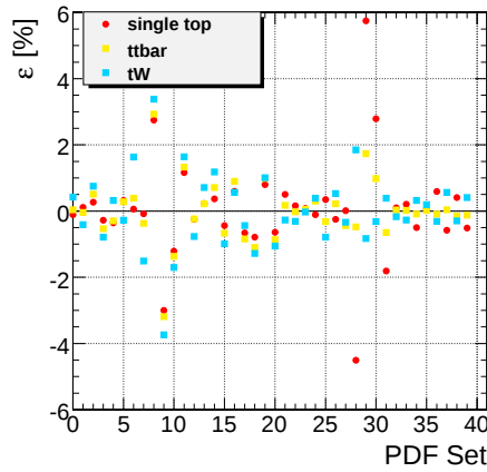
Figure 6.8: Relative variation (in %) of the selection efficiencies for signal, t\bar{t} , and tW , versus the PDF-set index in the CTEQ61 collection. [119]
