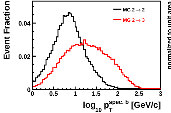
Figure 3.3: The transverse momentum distribution of the spectator b -quark. The x axis is plotted logarithmically in order to emphasize the difference due to the modeling of this parton in the two approaches. In the 2 \rightarrow 2 process, the spectator b -quark is modeled by the DGLAP evolution during the PS step, whereas in the 2 \rightarrow 3 simulation this parton is part of in the matrix-element calculation.
