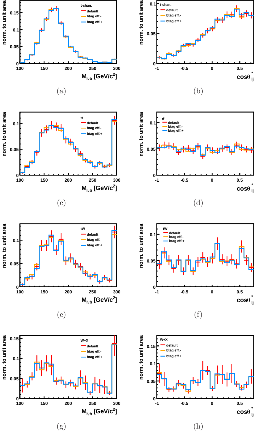
Figure 6.14: Shape comparisons for the invariant top-quark mass M_{l\nu b} (left column) and the restricted \cos\theta_{lj}^* (right column), where the applied discriminator working points are modified with respect to the expected uncertainty on the corresponding b -tagging efficiency ; for signal ((a), (b)), t\bar{t} ((c), (d)), tW ((e), (f)), and W+X ((g), (h)).
