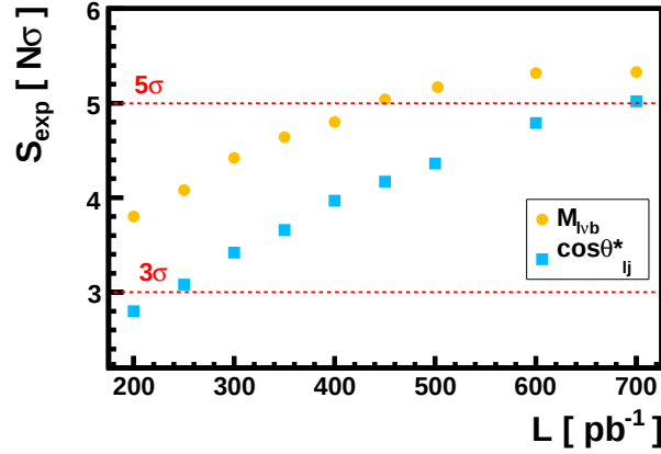
Figure 6.7: Evolution of the expected sensitivity with the integrated luminosity for M_{l\nu b} (yellow dots) and for \cos \theta_{lj}^* (blue rectangles) as obtained in the standard scenarios S_1 and S_{\text{flat}} , respectively. Statistical fluctuations of the method as well as uncertainties on the expected background rates are taken into account.
