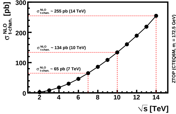
Figure 6.17: NLO cross-section of electroweakly produced top- and antitop-quarks in the t -channel as a function of the center-of-mass energy of the proton-proton collisions, calculated with ZTOP [90].
