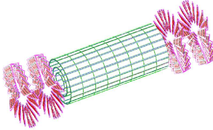
Figure 2.6: Sketch of the silicon pixel detector [64]. It is built of three barrel layers and two endcap disks which are assembled in a turbine-like geometry.
