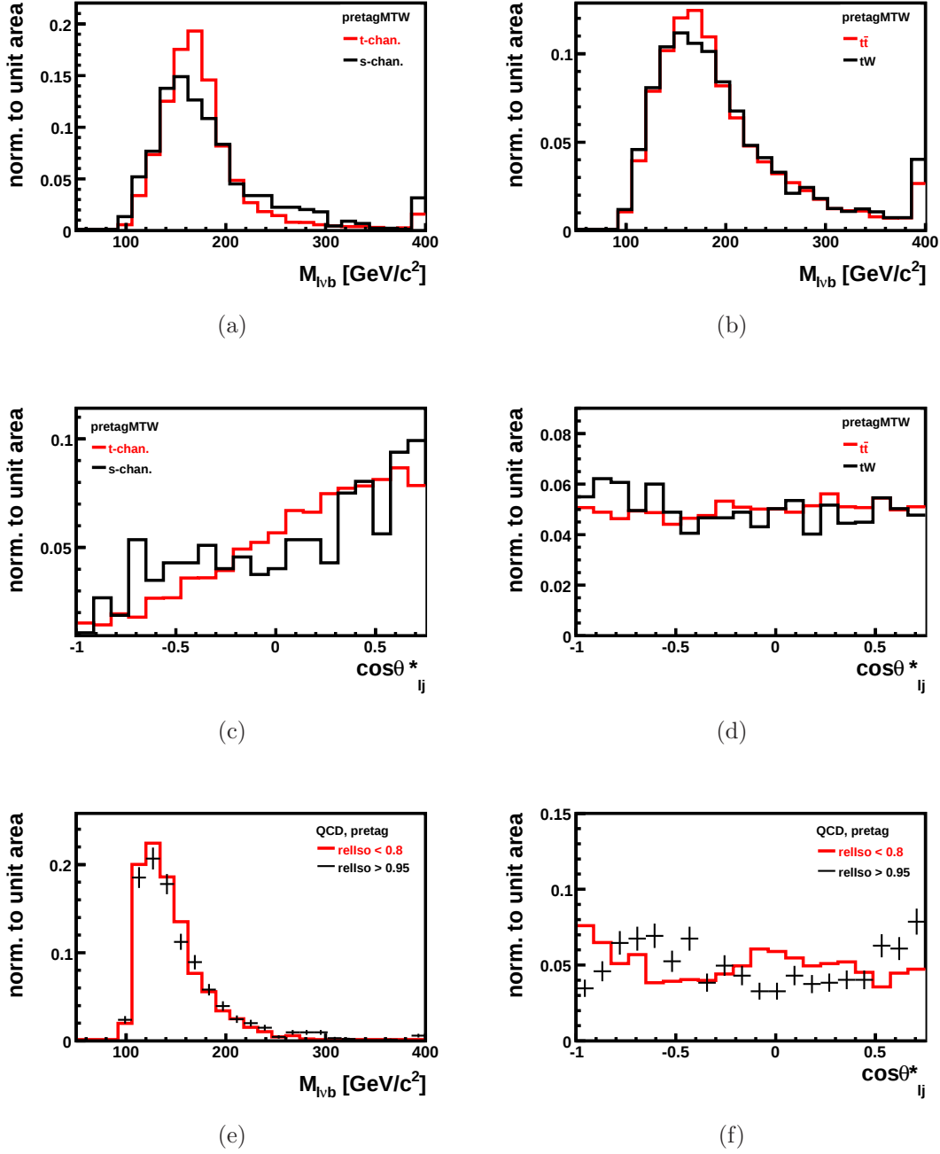
Figure 6.1: Comparison of M_{lvb} shapes for t - and s -channel single top-quark production (a), and t\bar{t} and tW production (b), and of the restricted \cos\theta^*_{lj} for t - and s -channel single top-quark production (c), and t\bar{t} and tW production (d). The comparison is performed for a selection without the b -tagging requirement in order to enhance the number of events while applying the cut on the transverse W -boson mass. This particular candidate-event sample is referred to as “pretagMTW”. The lower row shows the shape for QCD events with anti-isolation ( \text{relIso} < 0.8 ) compared to the distribution obtained with the standard isolation ( \text{relIso} > 0.95 ) for M_{lvb} (e) and the restricted \cos\theta^*_{lj} distribution (f).
