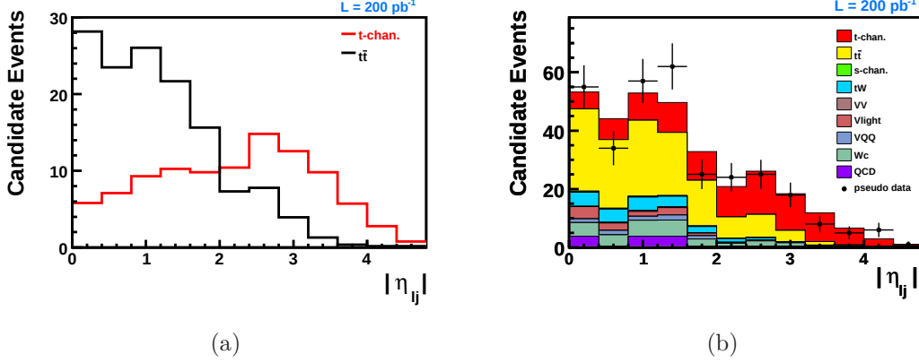
Figure 5.13: Pseudorapidity distribution of the untagged jet after having passed the full event selection. Subfigure (a) shows a comparison between top-quark pair and signal events, (b) shows the pseudorapidity distribution as expected in a selected data sample normalized to L = 200 \text{ pb}^{-1} . The pseudo data distribution is obtained from a bin-by-bin smearing of the total event yield following Poisson statistics.
