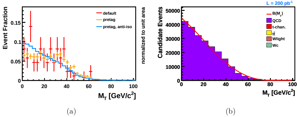
Figure 5.8: Comparison of the M_T distribution of QCD events in different control regions obtained from modified selection cuts (a). In order to increase the statistics, the b -tagging is omitted, yielding the so-called pretag sample, and in addition the isolation cut is modified to \text{relIso} < 0.8 , which is labeled as “anti-iso”. Subfigure (b) shows the expected M_T distribution in the QCD-enriched control region, normalized to 200 \text{ pb}^{-1} . The shape of the QCD background, which dominates the phase space of the anti-isolated muon, is extracted by fitting a polynomial of rank four as indicated by the red line.
