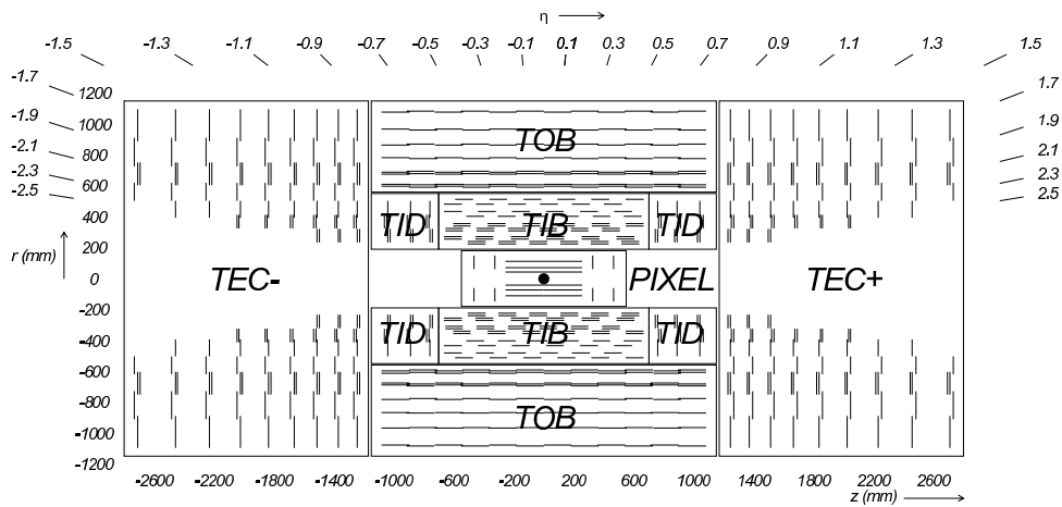
Figure 2.5: Schematic overview of the CMS tracking system [66]. The silicon pixel detector in the center is surrounded by the silicon strip detector which consists of endcaps and different barrel components.
