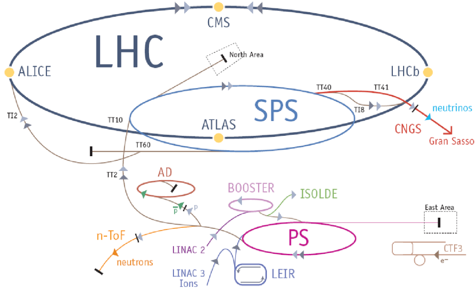
Figure 2.2: Sketch of the accelerator chain [58] used to fill the LHC with pre-accelerated protons or lead ions. On their way to the LHC, protons traverse the chain LINAC 2, Booster (PSB), PS, SPS, whereas lead ions coming from the LINAC 3 are sent through LEIR, PS, and SPS. As one can see in the sketch, many parallel experiments are supplied with beam taken out of different acceleration levels, which is not discussed here.
