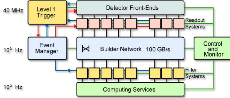
Figure 2.10: Sketch of the general architecture of the CMS DAQ system [64]. After the accept signal from the L1 trigger, the detector information fragments are passed to the readout units (RU, pink boxes). The event manager is responsible for the data flow in the RUs and their memory occupancy. The information is processed further through the builder network by the builder units (yellow boxes), which defragment the information of the events and passes them to the filter system of the HLT. The control and monitoring system is responsible for the configuration control and monitoring of all the elements.
