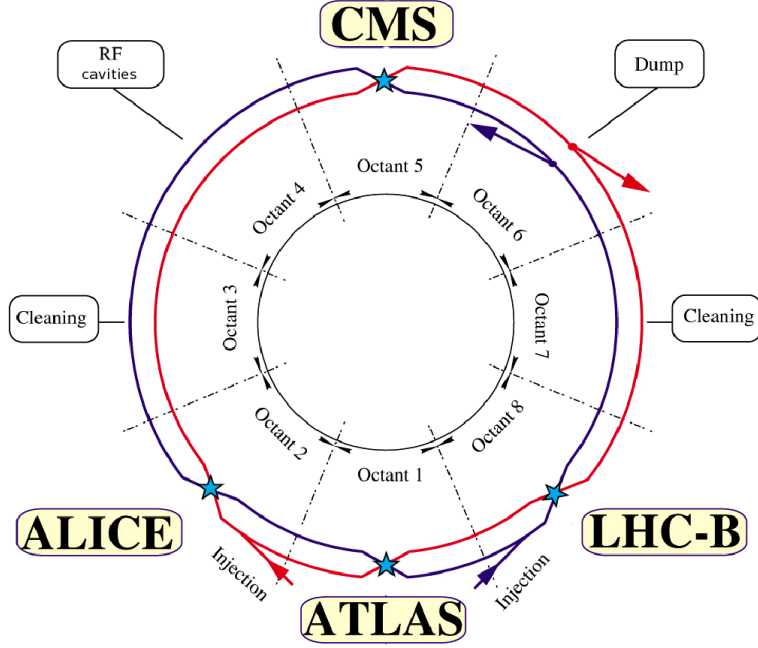
Figure 2.3: Sketch of the LHC [63]: the ring is organized in octants, distinguished by the different tasks which are performed. An octant starts from the middle of an arc and ends in the middle of the following arc and thus spans a full insertion. A section is defined as the part of the machine between two insertion midpoints. The straight sections which are located at the center of an octant are not explicitly shown here.
