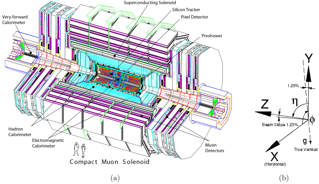
Figure 2.4: (a) Schematic overview of the CMS detector [64] where one quarter of the detector was removed to open the view onto the inner components. The interaction point in the center of the detector is enclosed by the inner tracking system, followed by the electromagnetic and the main hadronic calorimeter, which are all hosted inside the superconducting solenoid. The solenoidal magnet is surrounded by an outer hadron calorimeter and the voluminous muon systems. (b) The right-handed coordinate system of CMS: the x -axis points radially inwards to the center of the LHC ring, the y -axis points upwards, and the z -axis points towards the Jura. Since the plane of the LHC ring has a slight slope of 1.23% with respect to the horizontal by construction, the coordinate system of CMS is tilted accordingly.
