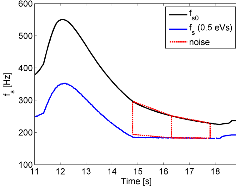
Figure 5.2: Noise excitation (red dashed lines) and synchrotron frequency spread at the end of the cycle, calculated for low intensities and for a bunch of 0.5 eVs.
