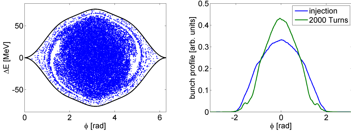
Figure 4.14: Particle distribution in the SPS longitudinal phase space (left) and its line density (right) after 2000 turns. The initial distribution is shown in Fig. 4.11. Note the high frequency pattern in the tails of the bunch. Here it is not very strong (compared to operation conditions) because of the low voltages, V_{200} = 1 MV and V_{800} = 0.25 MV. No intensity effects are included.
