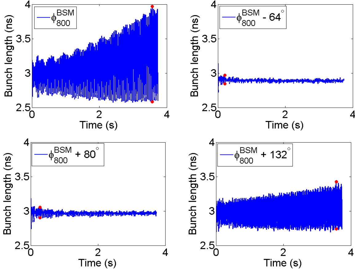
Figure 4.8: Bunch length evolution along the flat bottom for different values of \phi_{800} , V_{200} = 1 MV and V_{800} = 0.25 MV. Bunch with intensity \sim 1 \times 10^{11} and \varepsilon_\ell \simeq 0.25 eVs.
