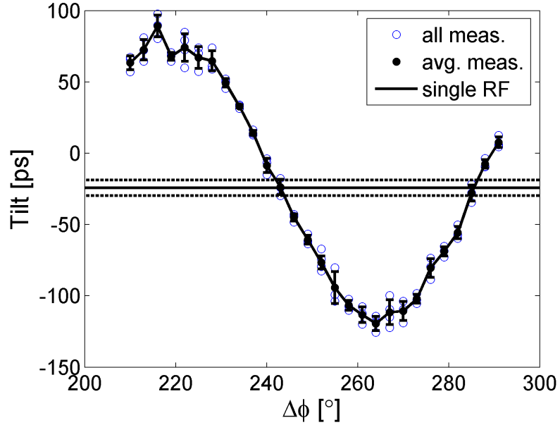
Figure 4.4: Measured bunch tilt versus relative phase (in deg at 200 MHz, unknown offset), 26 GeV/c, V_r = 0.25 and V_{200} = 2 MV.
