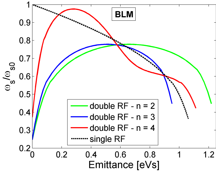
Figure 3.9: Relative synchrotron frequency distribution inside the bunch for different harmonic ratios n = h_2/h_1 and voltage ratio V_1/V_2 = n for the BLM. Example for the 100 MHz voltage V_1 = 0.6 MV, 26 GeV/c.
