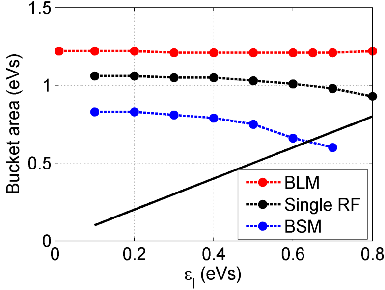
Figure 3.8: Bucket area versus emittance for a double RF (BLM - red, BSM - blue) and a single RF (black) in the cases corresponding to the N_{th} in Fig. 3.4. The black straight line is the limit where \varepsilon_\ell is equal to the bucket area.
