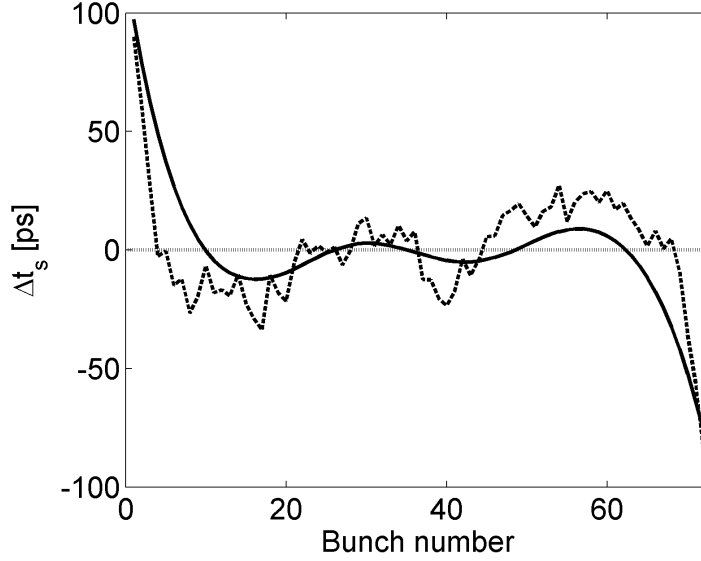
Figure 5.21: Bunch position variation (in ps) along the batch at the time in the cycle before the noise excitation. V_{200} = 4.5 MV and V_{800} = 0.5 MV. The beam parameters are the same as in Fig. 5.10.
