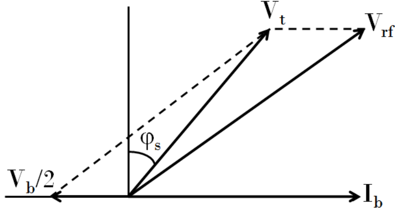
Figure 5.7: Vector diagram of a single-bunch passage through a resonant cavity.
