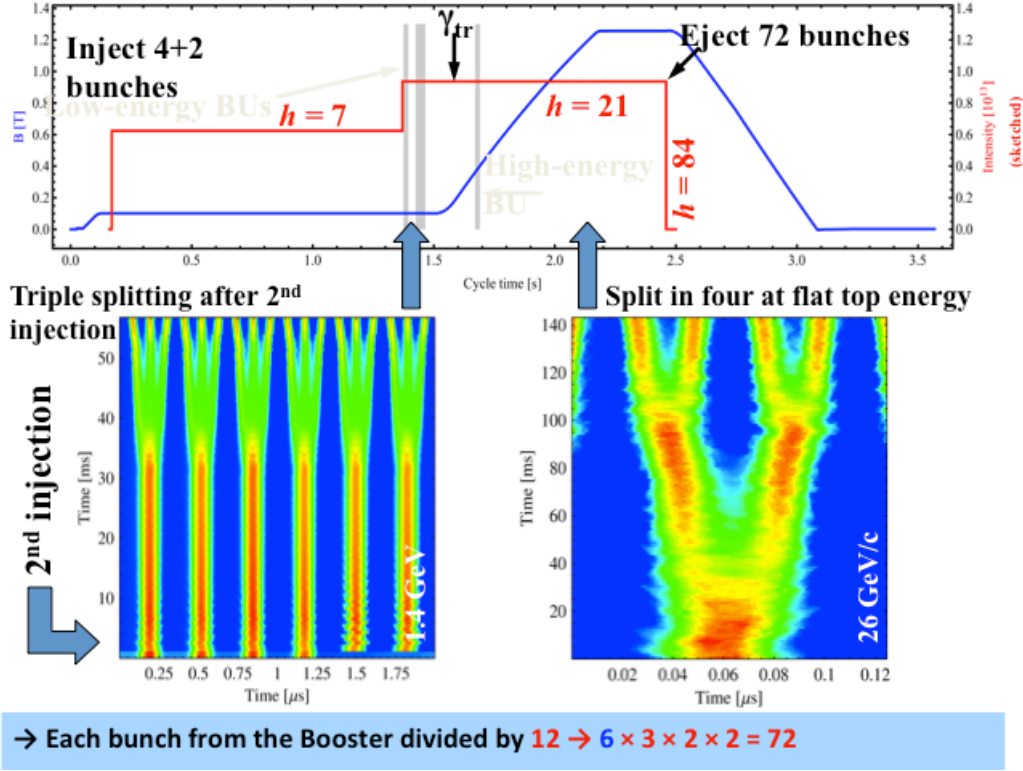
Figure 1.2: Schematic representation of the production of the LHC 25 ns beam in the CERN PS [26].
