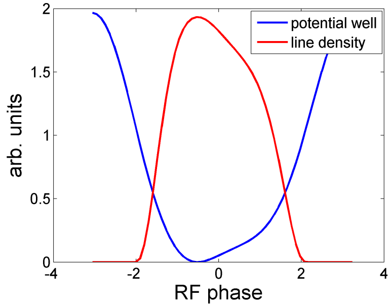
Figure 3.7: Potential well (blue curve) and line density (red curve) in the case of BLM with \varepsilon_\ell = 0.65 eVs and a phase shift of -20^\circ . Bunch intensity of 1 \times 10^{11} .
