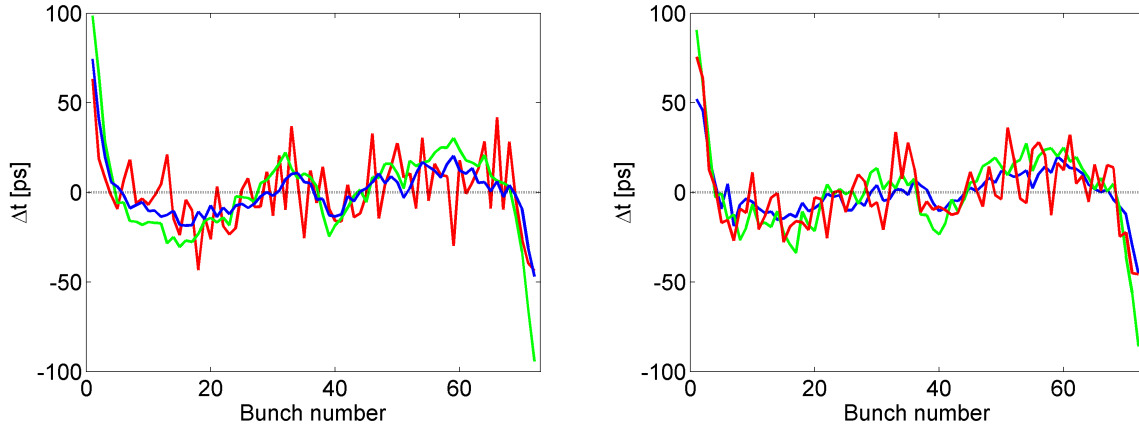
Figure 5.4: Longitudinal bunch position shift with respect to the equidistant positions along the batch. The data correspond to those of Fig. 5.3.
