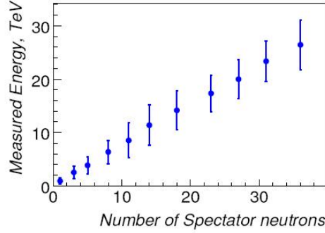
Figure 2.10: Energy measured by a 33\text{cm}^2 area centered on the spectator neutron cluster vs. the known number of spectator neutrons in the cluster. Error bars correspond to the rms of measured energy fluctuations. See text for details [1].
