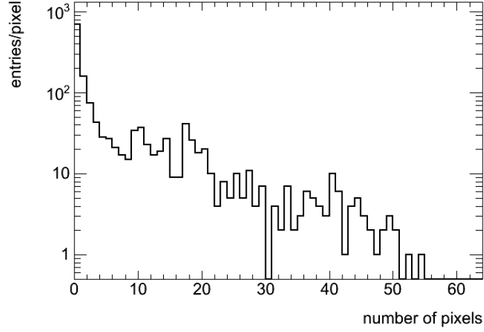
Figure 3.4: Number of pixels of the EM module with an energy higher than the threshold per event from Run 177682 at 7 TeV of center of mass energy.
