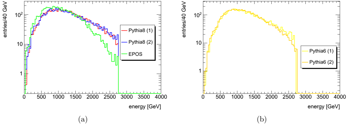
Figure 4.10: Distribution of reconstructed energy of the \pi^0 obtained from the simulated detector response with Pythia8 A2CTEQ6L1 (1), Pythia8 MSTW2008LO (2) and EPOS and with Pythia6 AUET24Minus (1) and Pythia6 Perugia2011 (2). The sharp cut at around 2.7 TeV corresponds to the rejection of events saturating the HG read-out of the ZDC.
