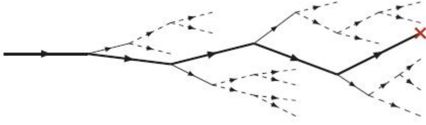
Figure 4.1: A representation of ISR. The thick line is the main parton taking part in the main interaction (the red X mark). Thin lines are partons that can not be recombined and dashed lines are further fluctuations that may or may not recombine. FSR has a similar representation.
