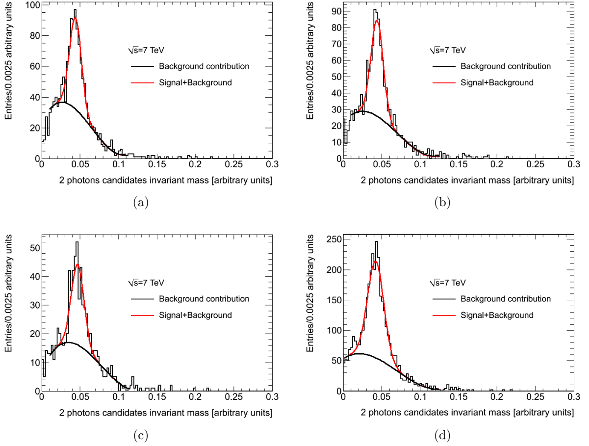
Figure 3.12: Uncalibrated invariant mass of \pi^0 candidates for pp collisions at 7 TeV in Run 177531 (a), 177540 (b), 177593 (c) and 177682 (d) reconstructed using the ZDC-C. The distribution is fitted using the sum of a gaussian distribution for the main \pi^0 peak and a third degree polynomial for the background events, whose contribution is shown by the black curve.
