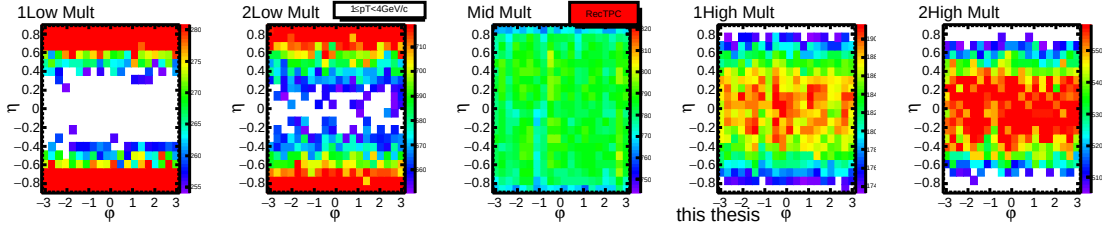
(c) Rec.MC, TPC event estimator, \phi and \eta distributions for the 5 multiplicity classes.
