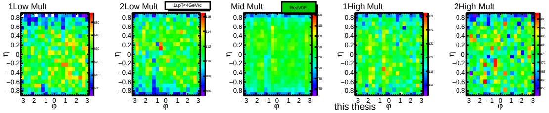
(d) Rec.MC, V0E event estimator, \phi and \eta distributions for the 5 multiplicity classes.
