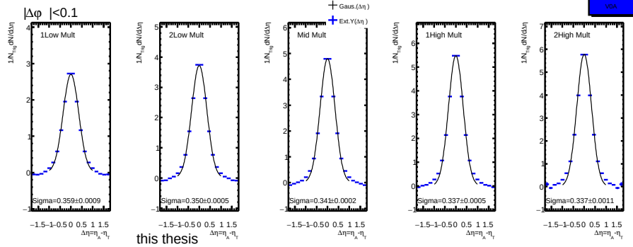
(a) ALICE experimental data, V0A event estimator.
